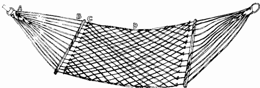
Detail of Hammock Assembly
