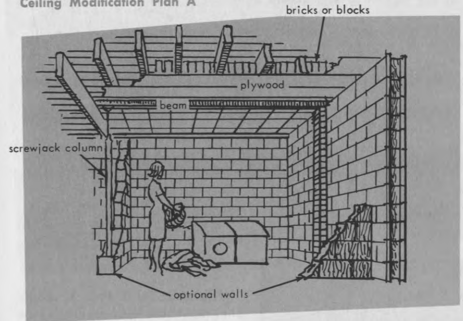
Ceiling Modification Plan A
