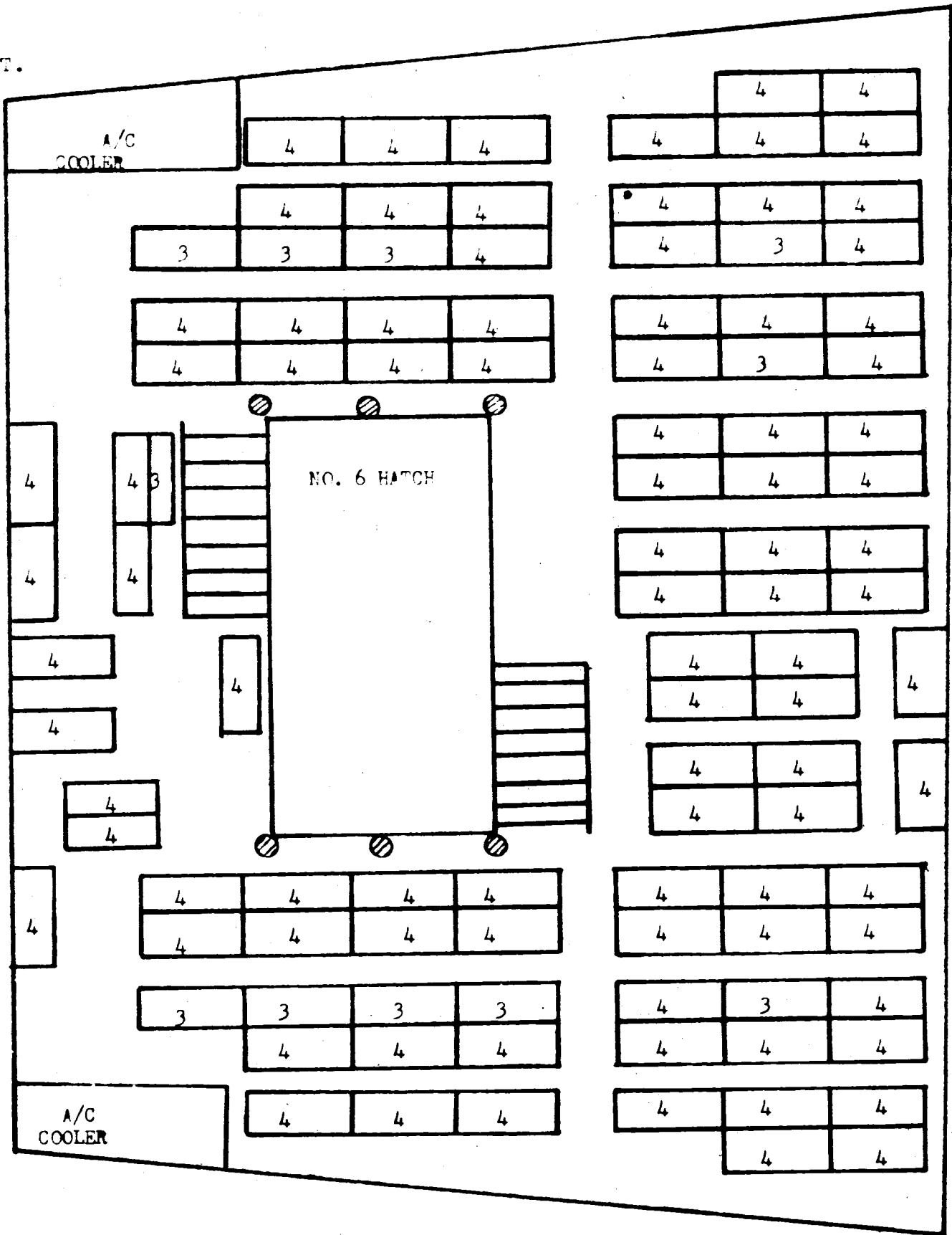
NO. 6 HATCH 4th. DECK COMPARTMENT 4-6
