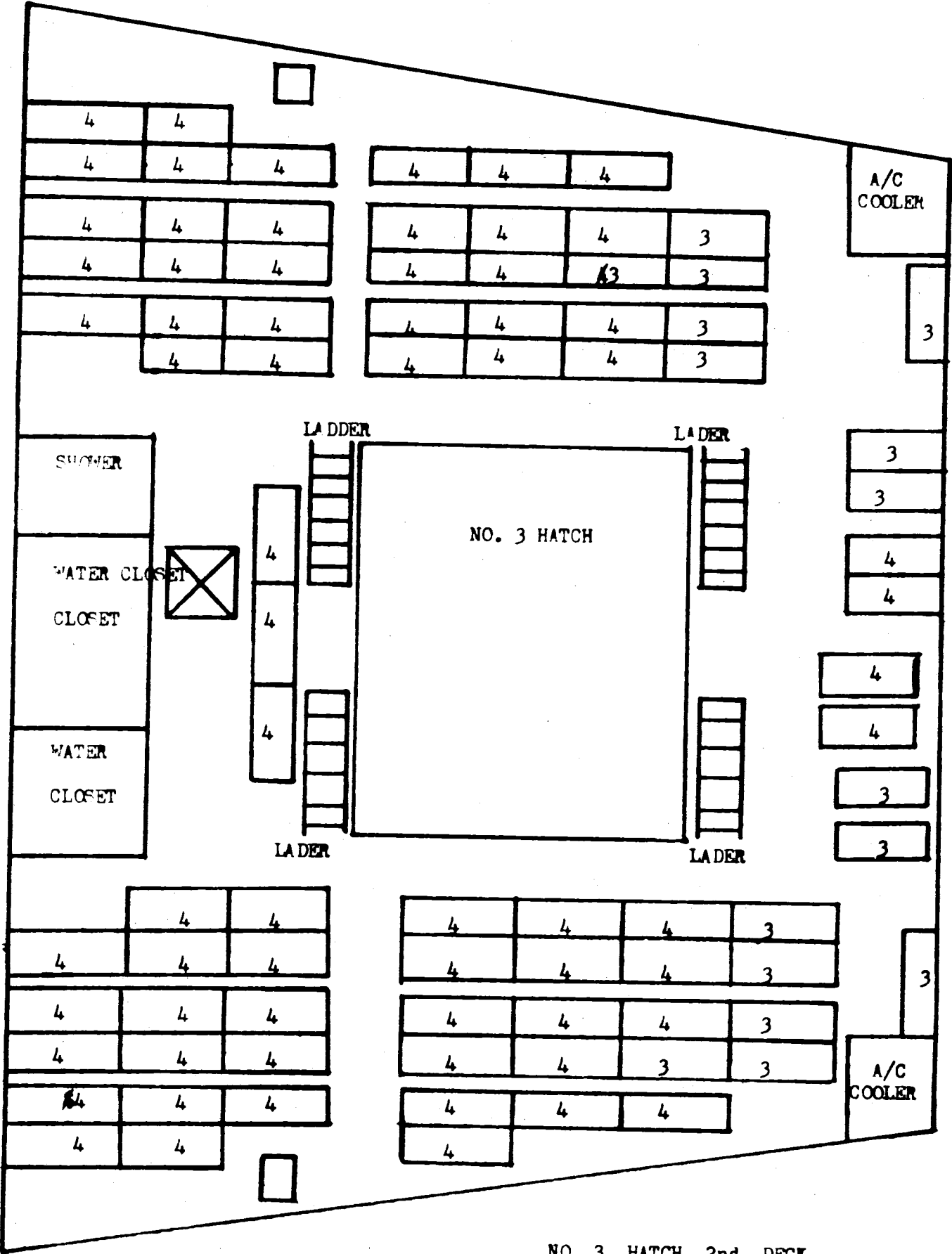
NO. 3 HATCH ,2nd. DECK
