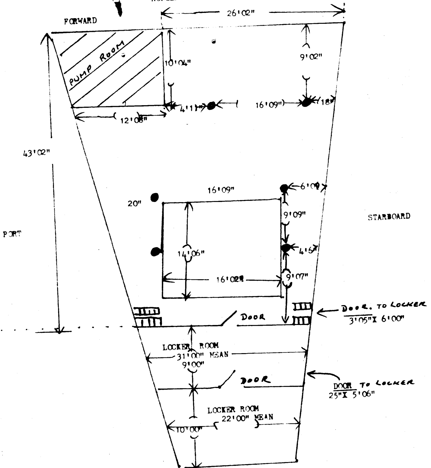
NO. 7 LOWER HOLD
