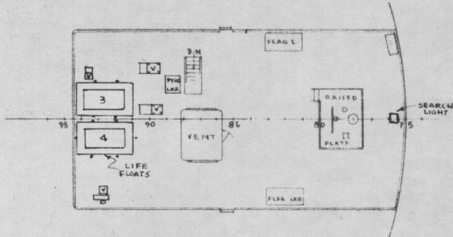
TOP OF NAV BRIDGE 04 LEVEL
