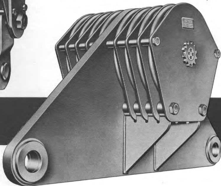
608-S, 30" 250 Ton Eight Sheave with special Hanger.
