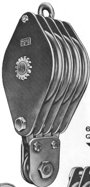
604-H, 30" 150 Ton Four Sheave Sling Hanger.
