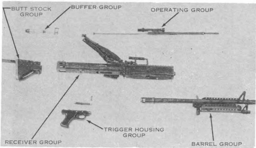
Figure 3. Machinegun, 7.62mm M60, disassembled into six major groups
