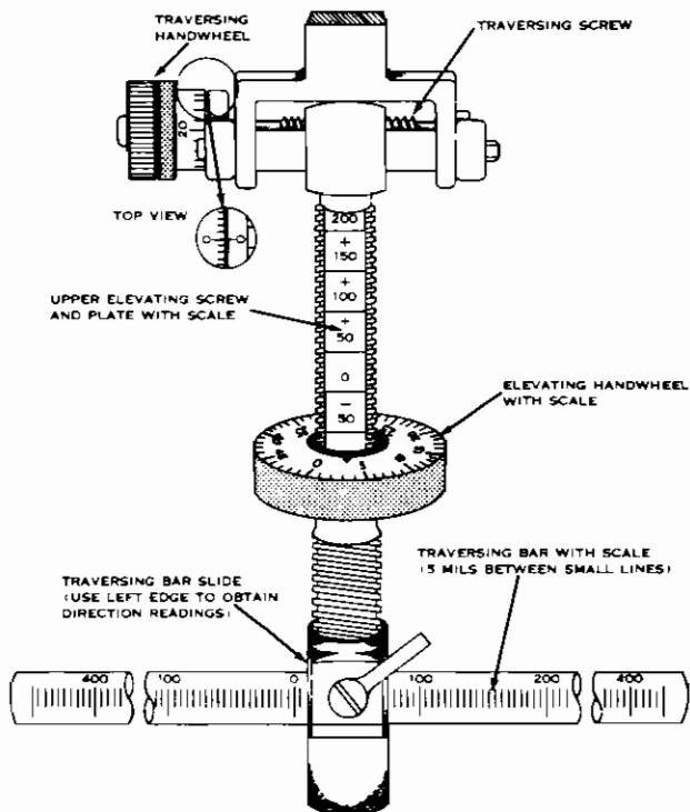
Figure 30. Traversing and elevating mechanism.
