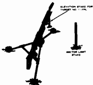
Figure 26. Sector limit and elevation stakes. (Eliminates use of light on gun position at night.) OVERHEAD FIRE
