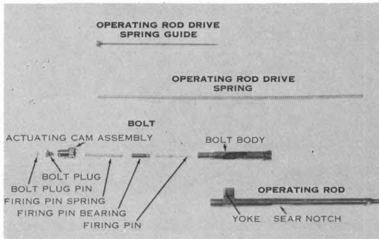
Figure 4. Operating group disassembled.
