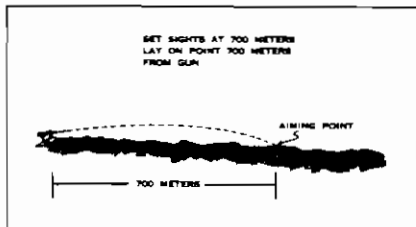
Figure 17. Grazing fire.
