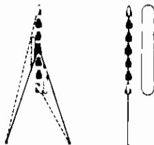
Figure 24. Searching fire.
