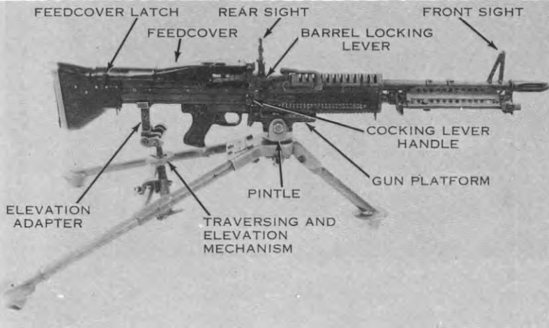
Figure 2. Machinegun, 7.62mm, M60 on M122 tripod mount.
