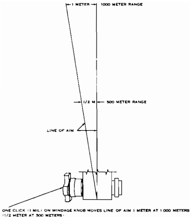
Figure 12. Mil relationship.
