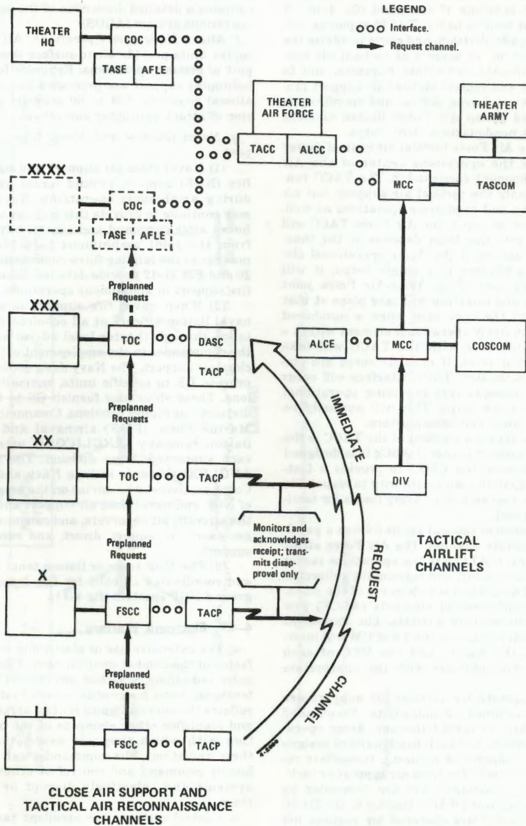
Figure 4-10. Tactical air support request channels.
