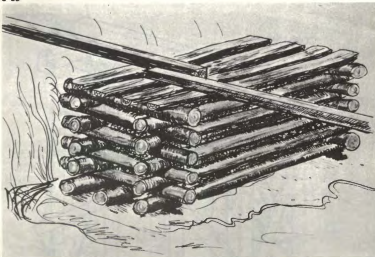
Figure 3-14. Typical crib pier.
