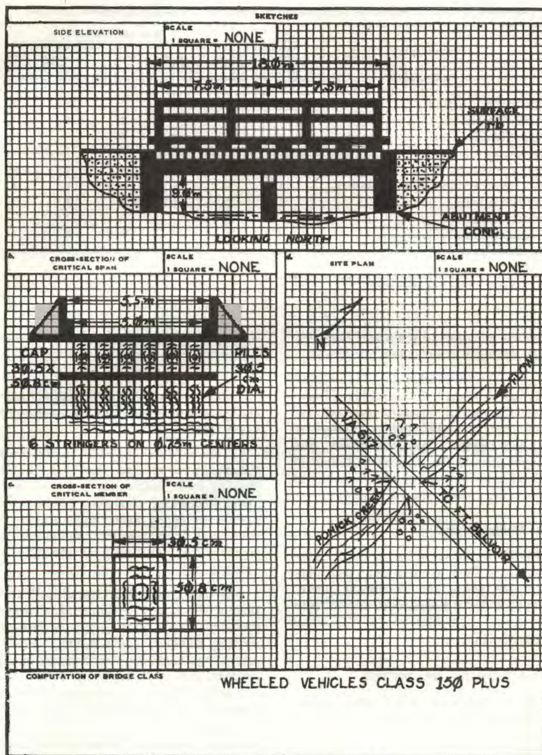
Figure 3-5. Example bridge sketch on back of reconnaissance report form.
