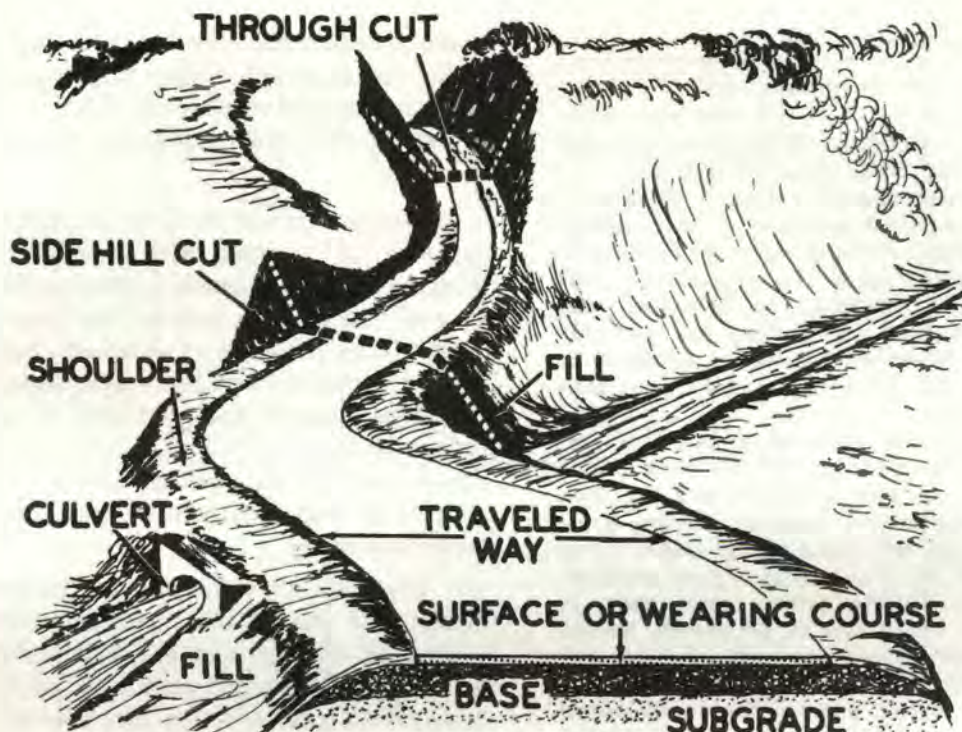
Figure 3-58. Road nomenclature.
