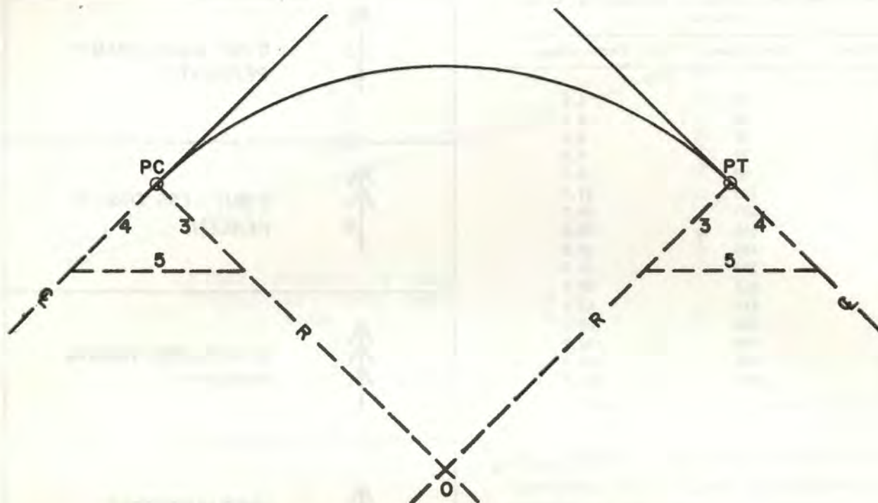
Figure 2-12. Radius of curvature by locating center of circle.
