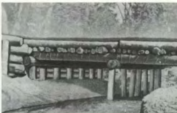
Figure 3-25. Simple stringer bridge with log stringers.
