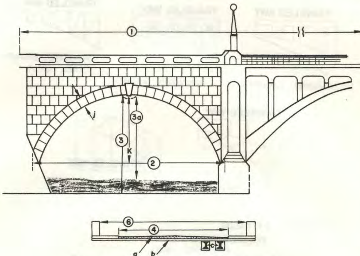
Figure 3-42. Standard dimension data guide for arch bridges.
