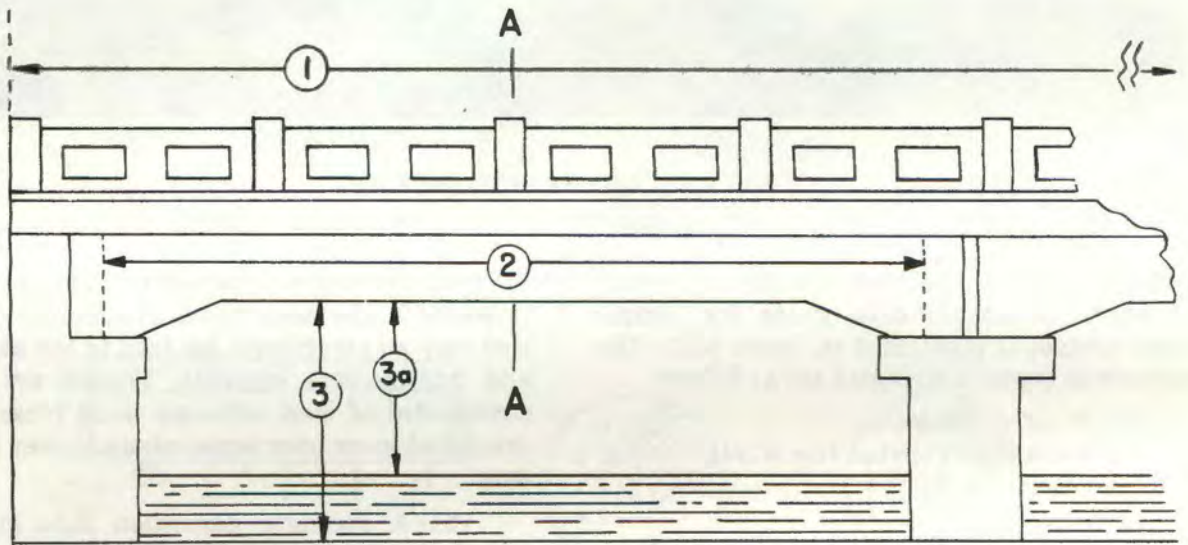
Figure 3-20. Typical cantilever bridge.
