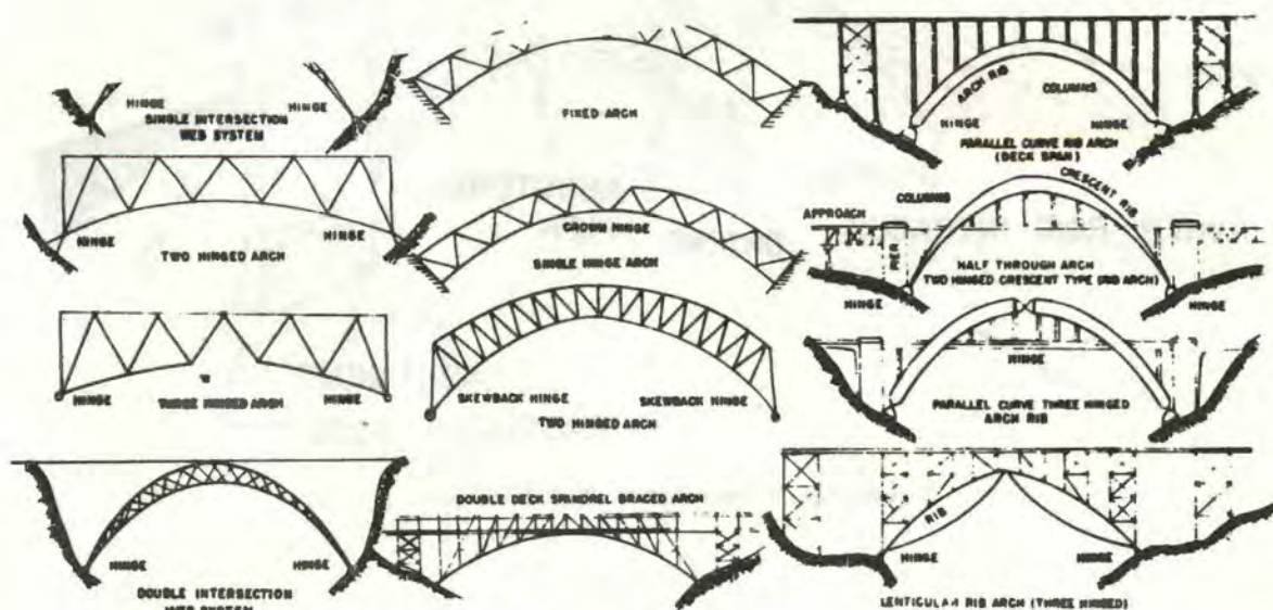
Figure 3-43. Common types of arch construction.
