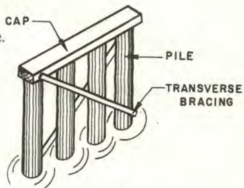
Figure 3-11. Pile bent.
