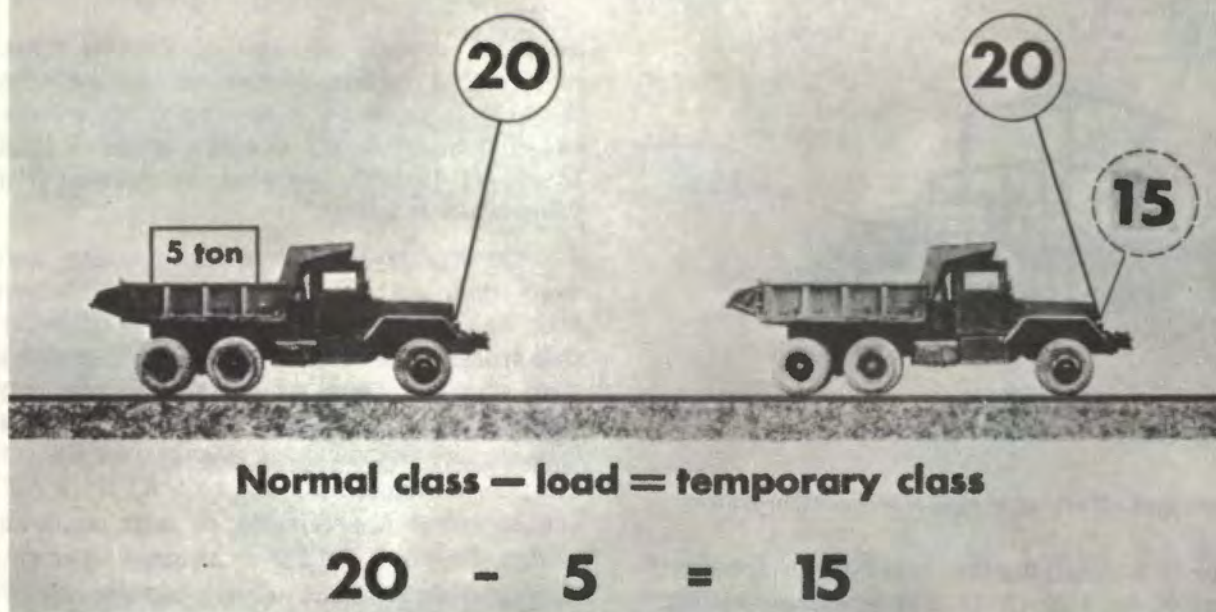
Figure 2-55. Example classification of an underload.
