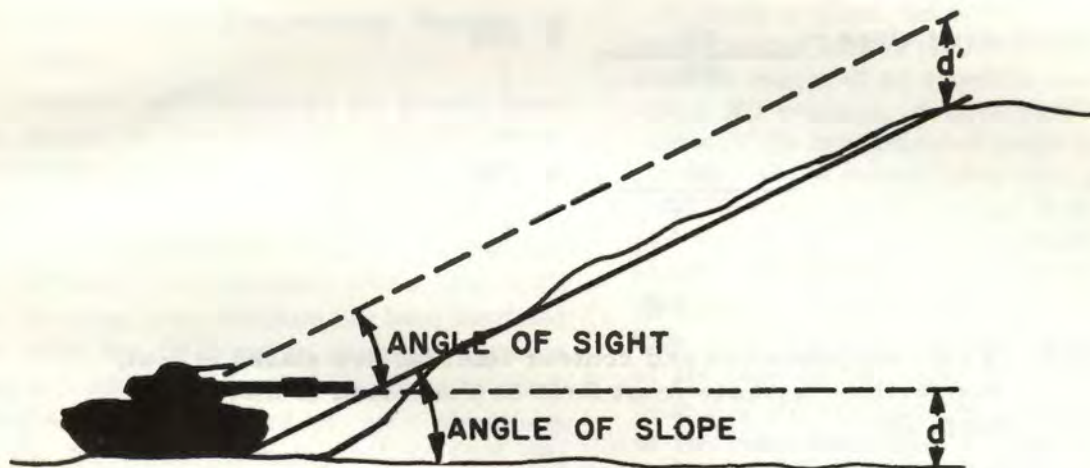
Figure 2-8. Determining percent of slope using line of sight and pace method.
