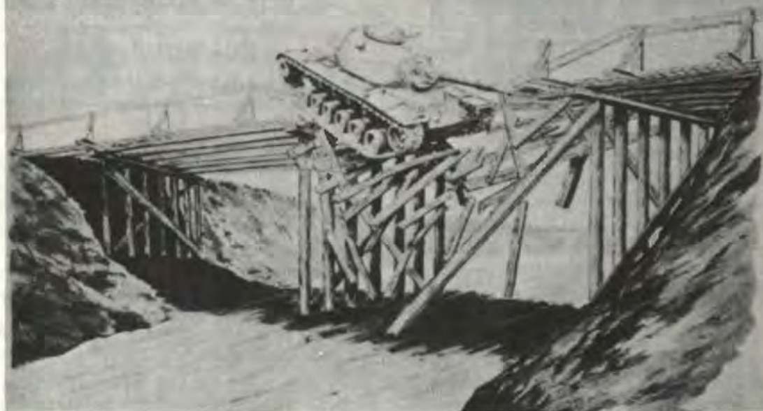
Figure 2-43. Example of a bridge failure.
