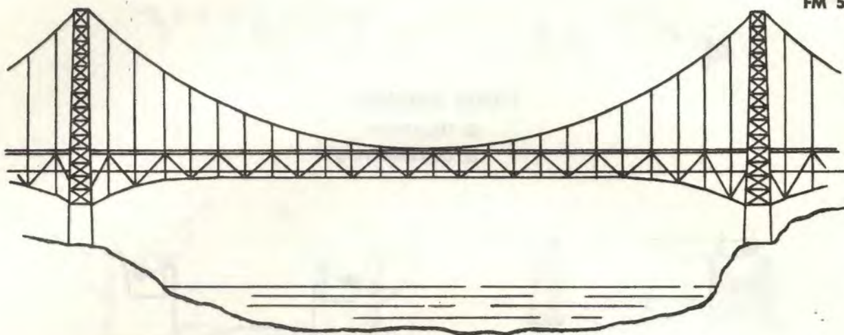
Figure 3-53. Bailey type suspension bridge.
