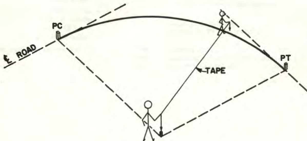
Figure 2-11. Radius of curvature by using tape.
