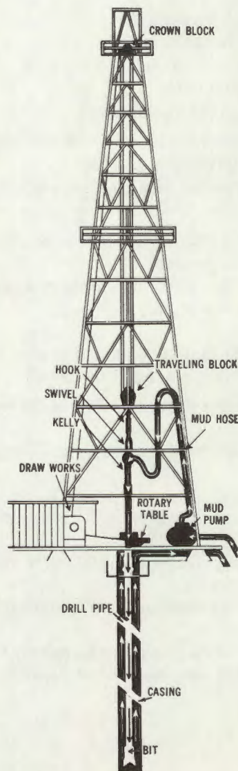
Figure 8-5. Rotary drilling.
