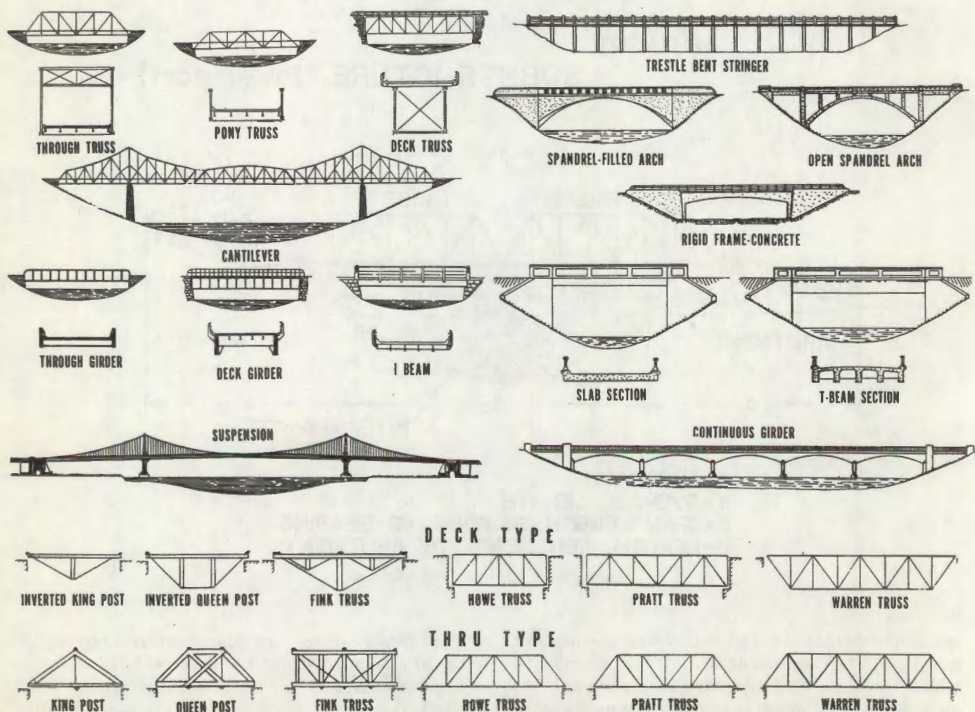
Figure 5-17. Fixed bridges.
