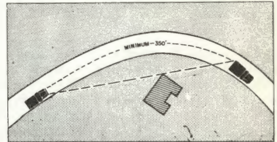
HORIZONTAL CURVE
