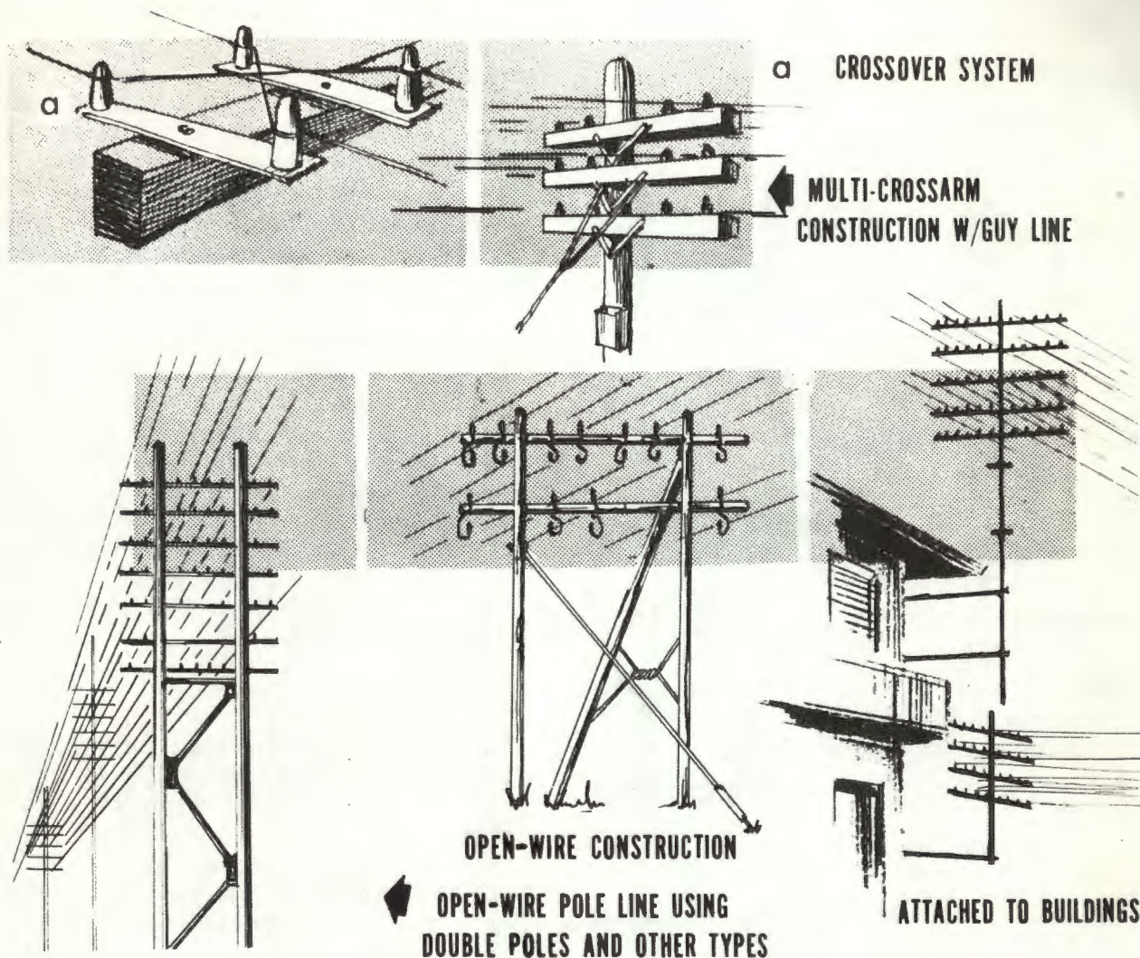
Figure 6-5. Types of telephone poles.
