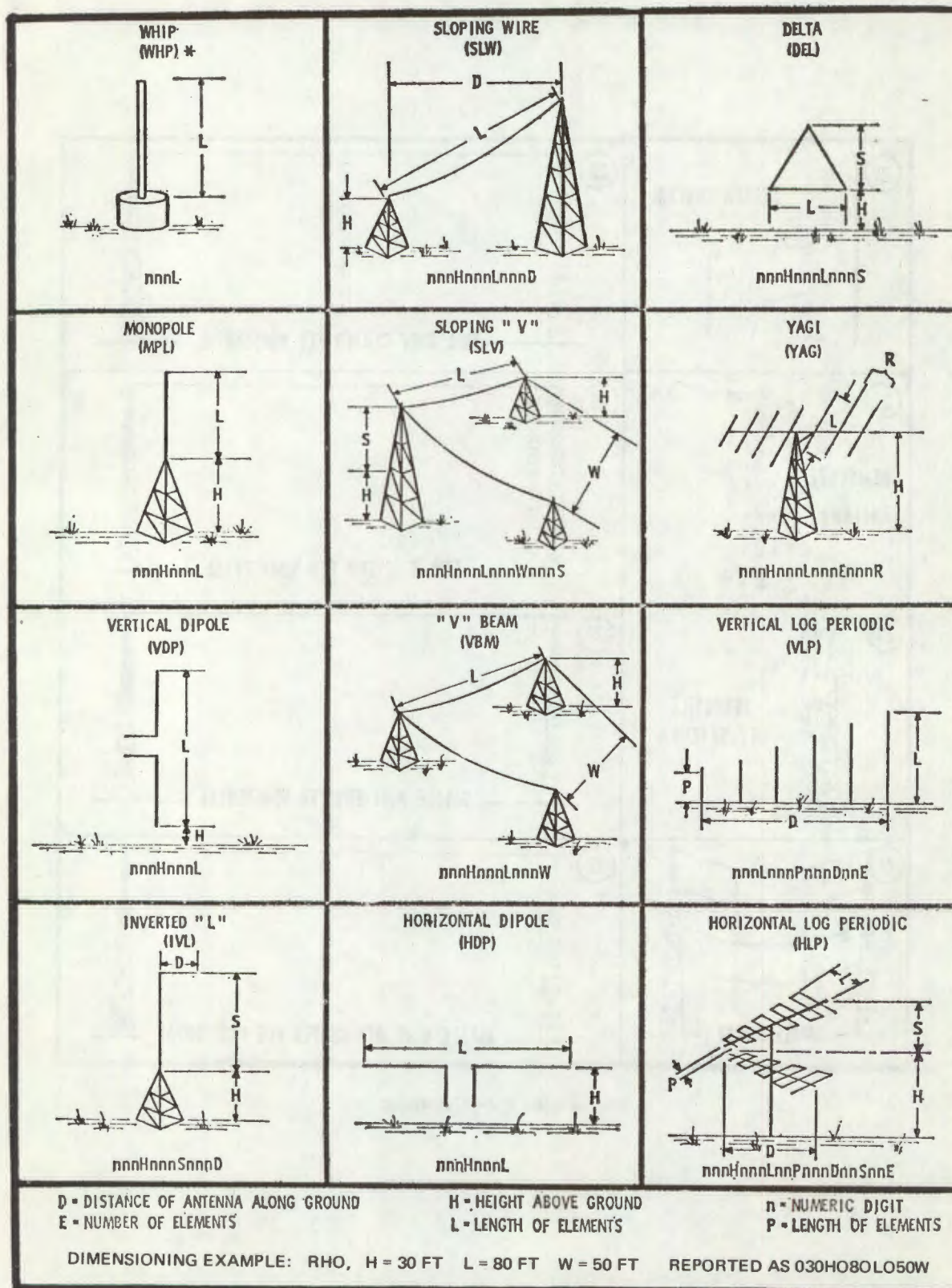
Figure 6-4. Standard method of dimensioning antennas.
