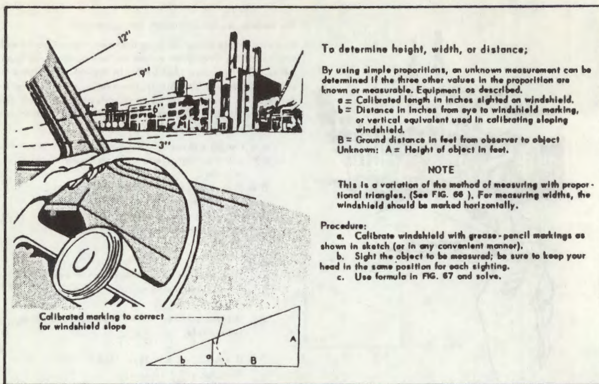
Figure 7-15. Windshield measurements.
