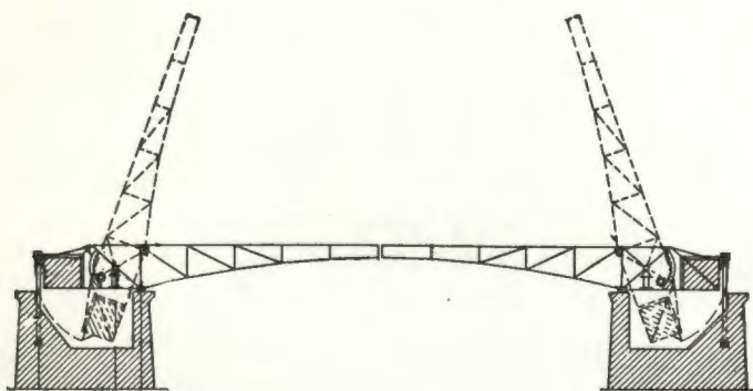
BASCULE DOUBLE-LEAF TRUNNION SPAN
