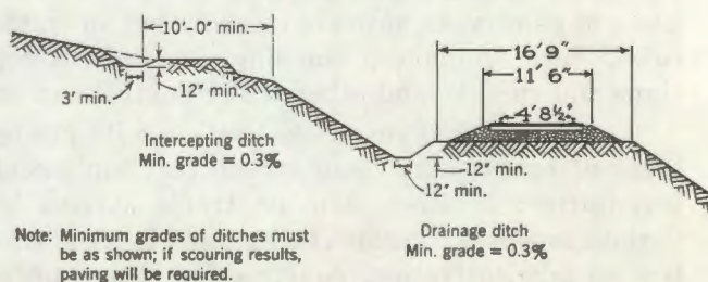
Figure 5-7. Typical roadbed cross section.
