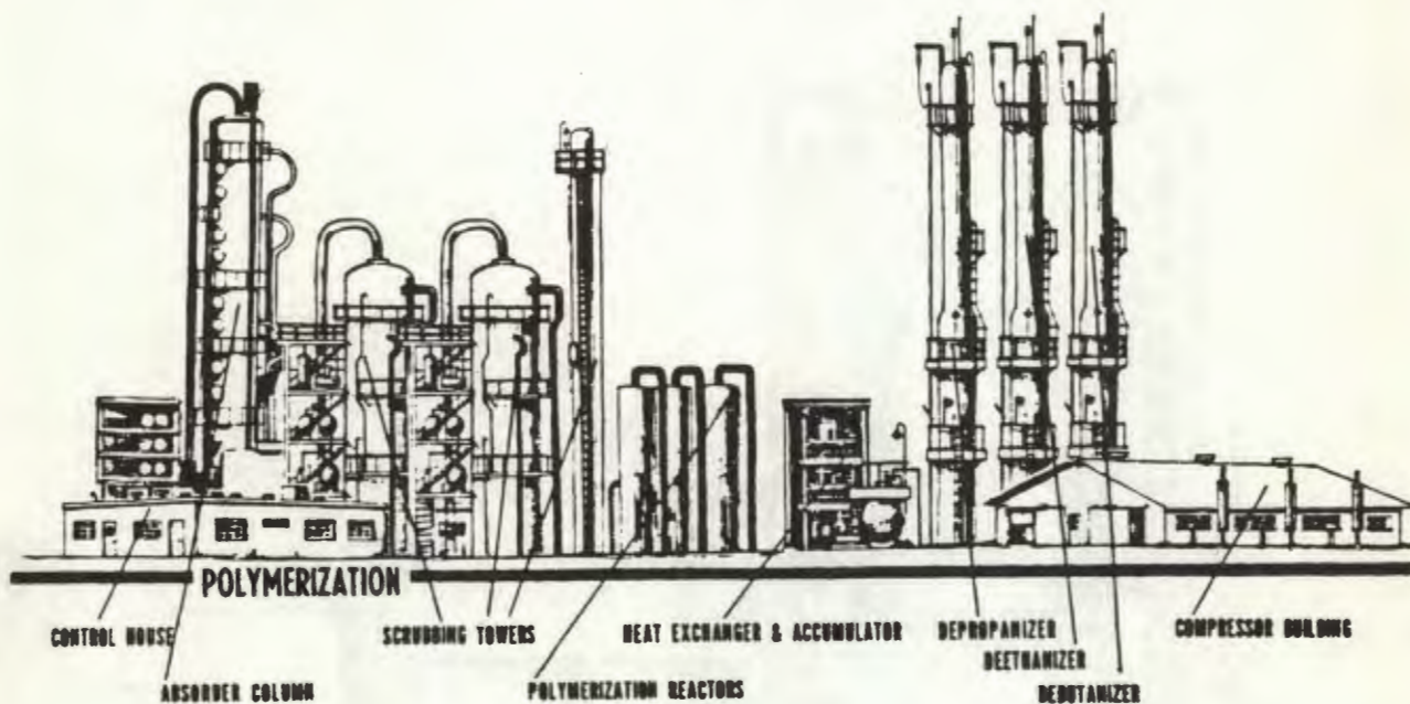
Figure 9-17. Sketch of petroleum polymerization process.
