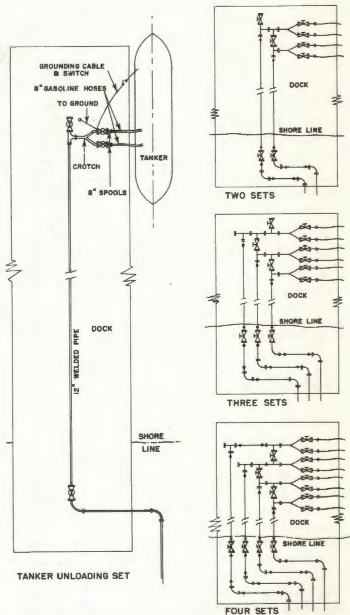
Figure 5-24. Layout of dock set for tanker unloading.
