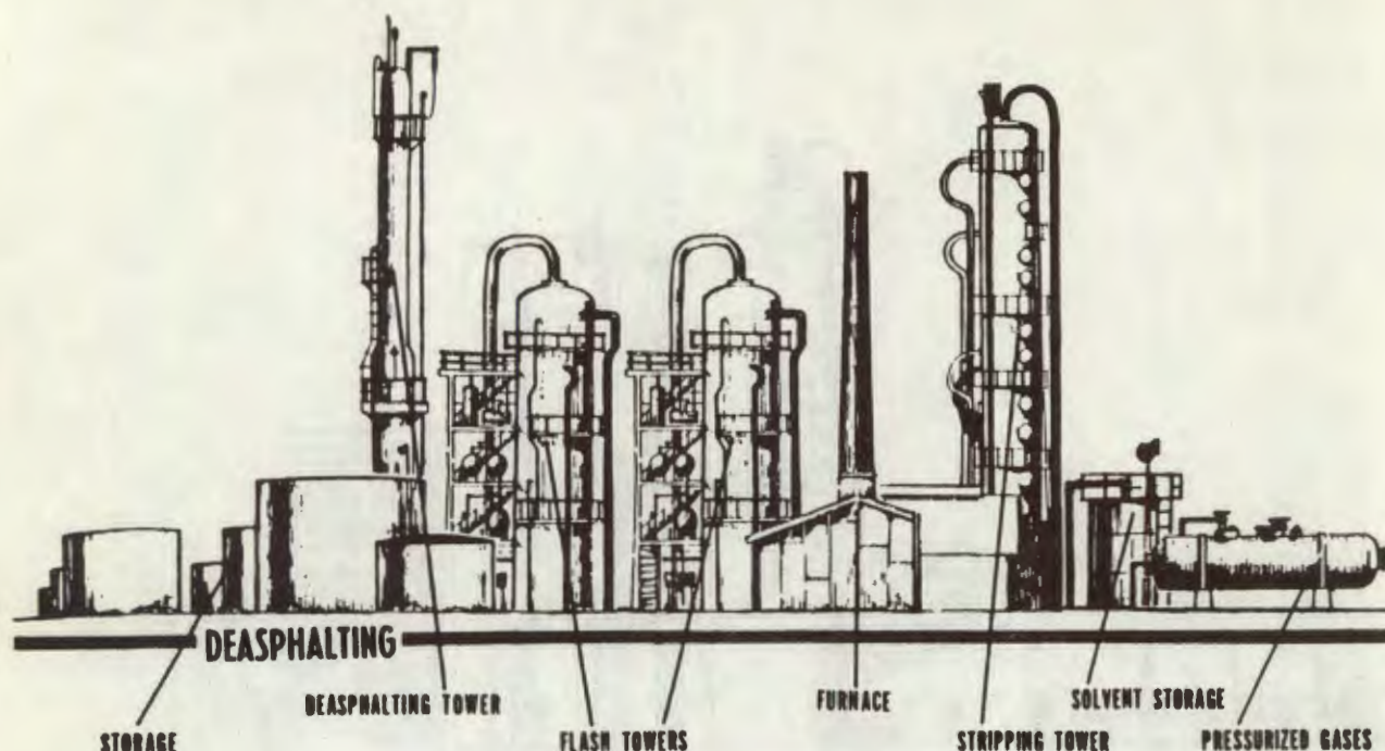
Figure 9-22. Sketch of petroleum deasphalting process.
