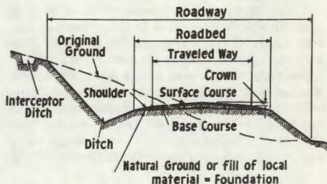
Figure 5-1. Typical cross section illustrating road nomenclature.
