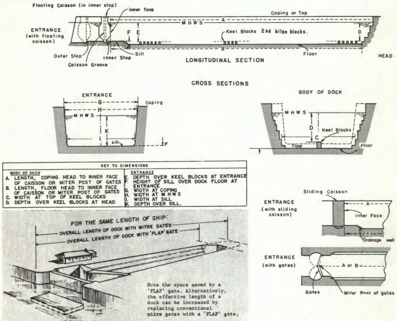
Figure 5-53. Graving dock.
