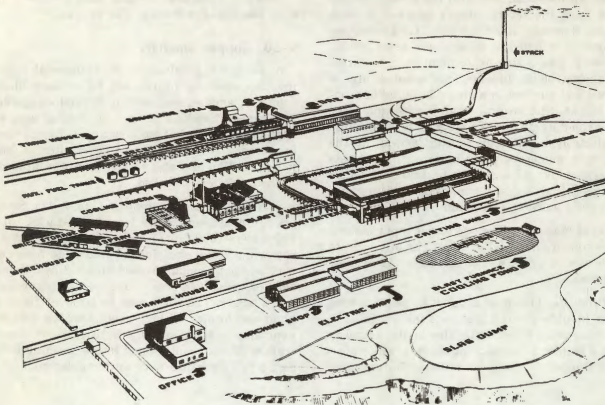
Figure 9-13. Layout sketch of typical copper smelter.
