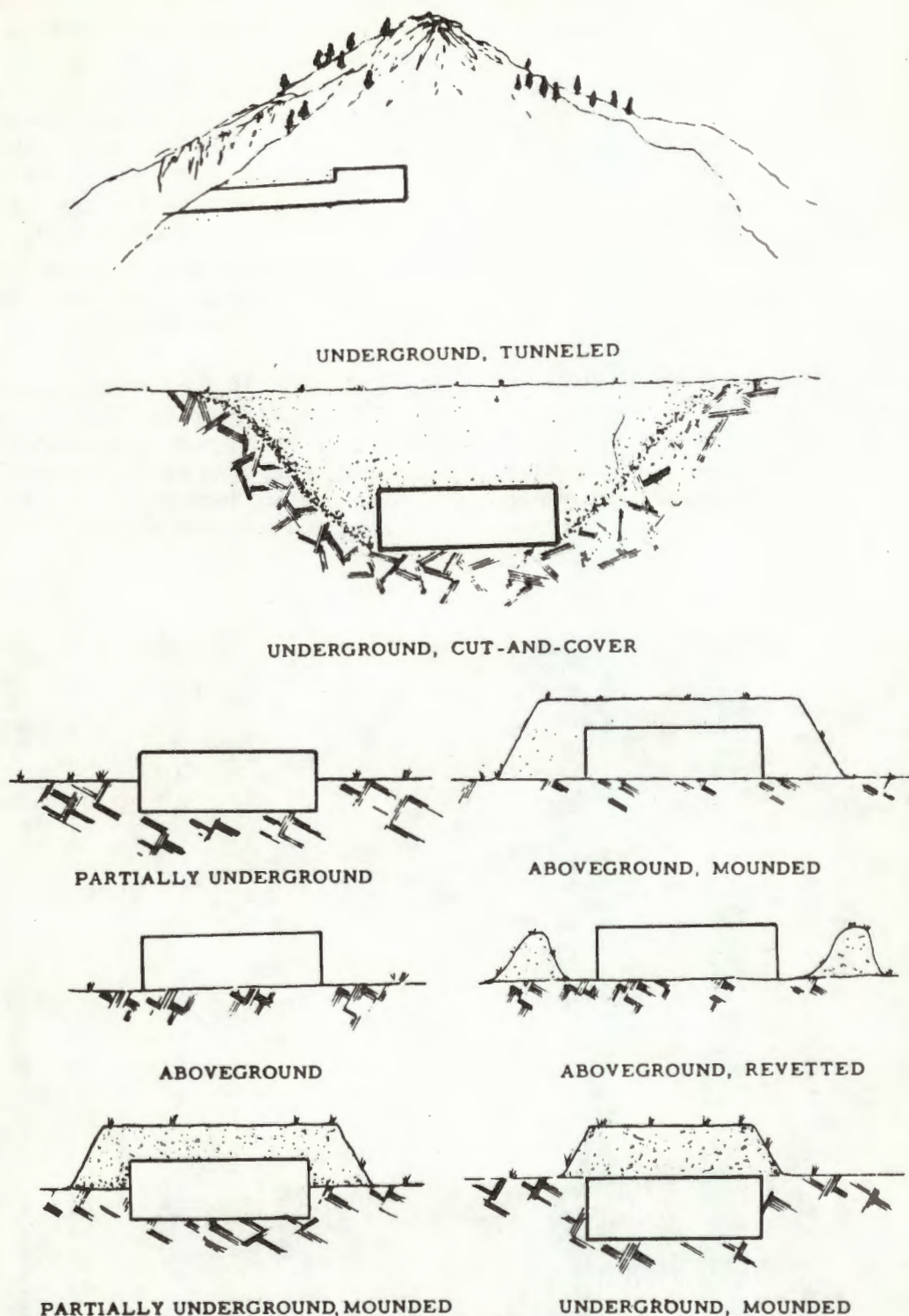
Figure 7-9. Structure situations.
