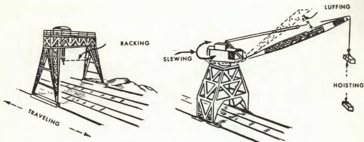
Figure 5-51. Basic motions of cranes.
