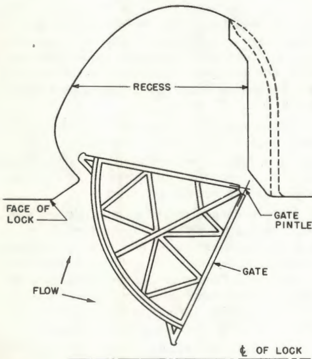
Figure 5-31. Schematic drawing of sector gate leaf.
