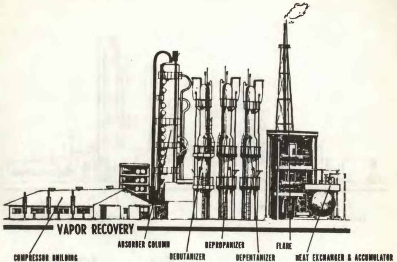
Figure 9-20. Sketch of petroleum vapor recovery process.
