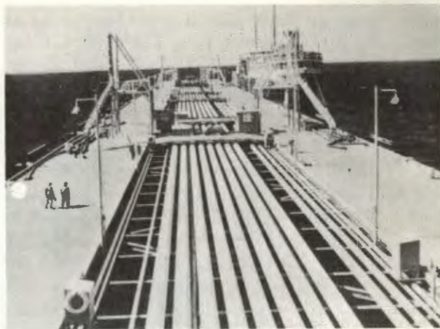
Figure 5-23. Oil loading lines.
