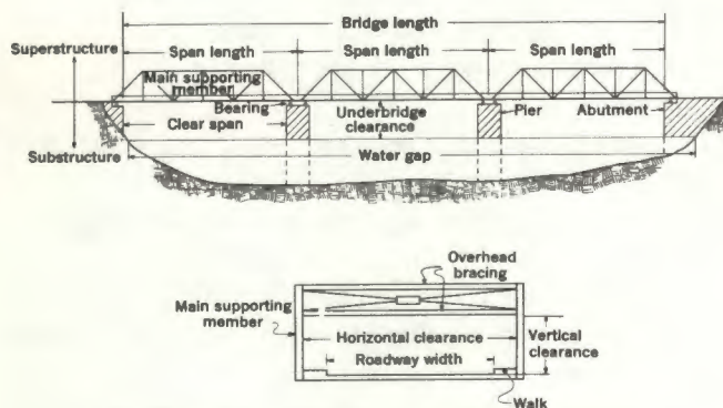
Figure 5-19. Principal bridge measurements.
