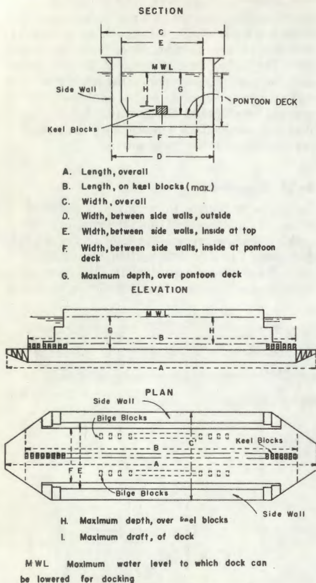
Figure 5-54. Floating drydock.
