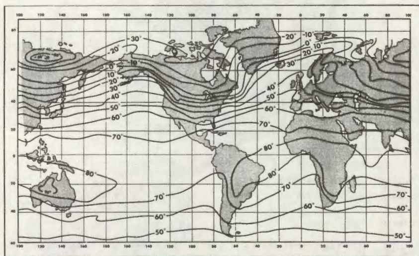
Figure 2-2. World temperatures in January.
