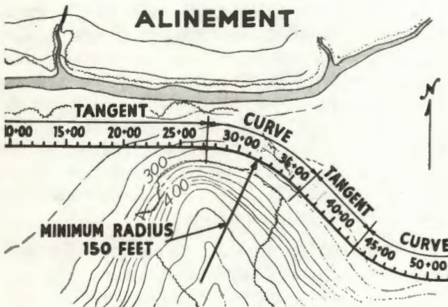
Figure 5-4. Alinement showing tangents and curves.
