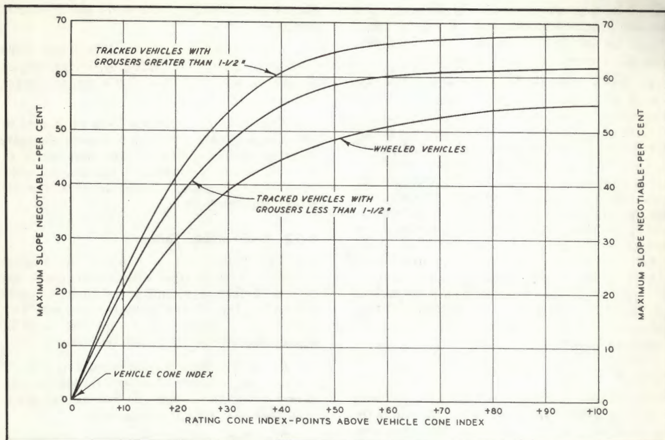
Figure 4-1. Criteria for self-propelled vehicles on fine-grained soils and sand with fines, poorly drained.
