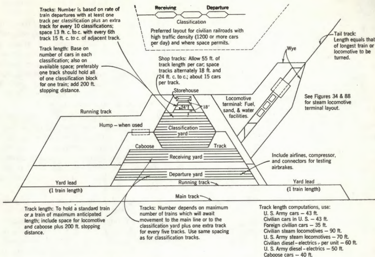
Figure 5-13. General layout of a major classification yard.
