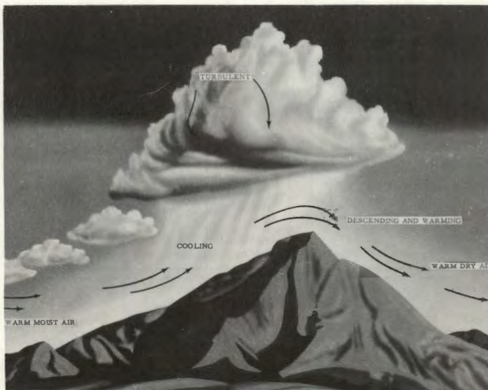
Figure 2-7. Chinook or foehn effect.
