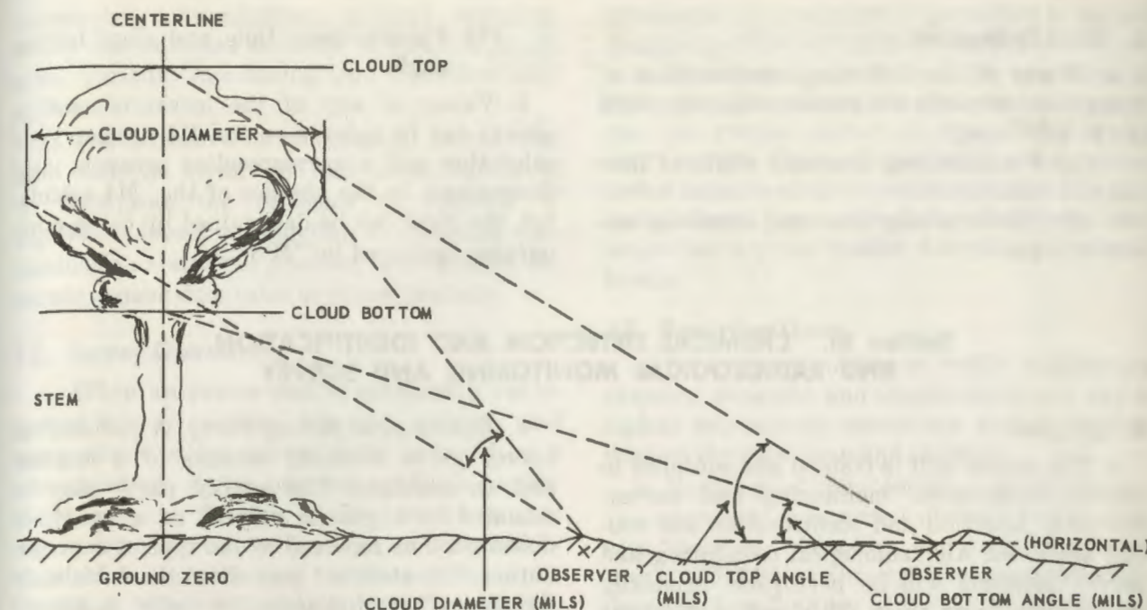
Figure 100. Cloud measurements.
