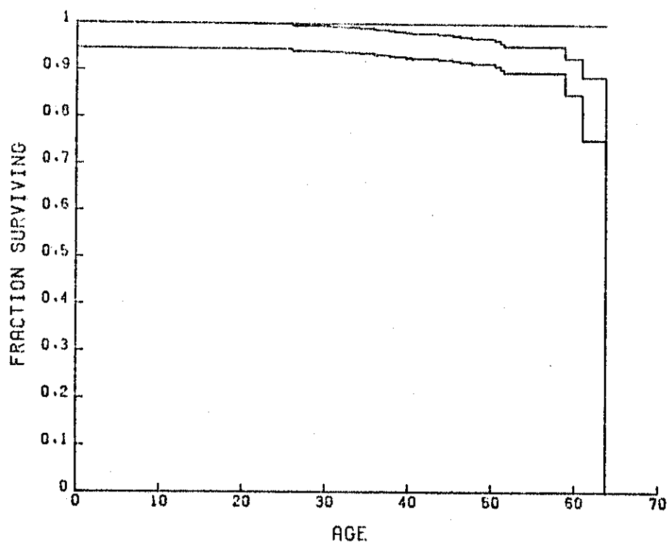
Figure 10 SURVIVAL CURVE ESTIMATE AND 95% CONFIDENCE BANDS FOR RANCH HAND FLYING PERSONNEL
