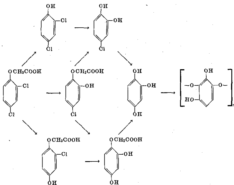
FIGURE 3 Proposed mechanism of 2,4-D photodecomposition After Crosby (4)
