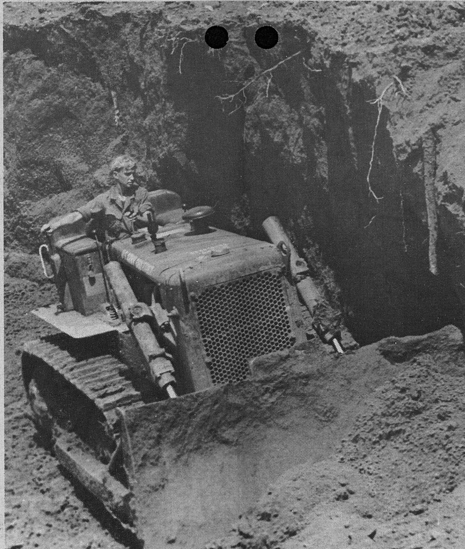
Specialist Five Steve Caldwell (right) uses his Cat to chew out a hillside for fill soil to cover the runway extension. During construction, 8th Engineer crews were often forced from the runway by daily air traffic (below) and enemy mortar barrages.
