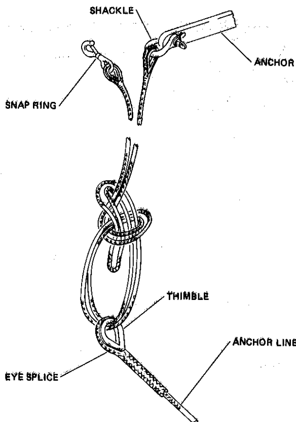
Figure 2-19. Method of Shortening the Anchor Line
