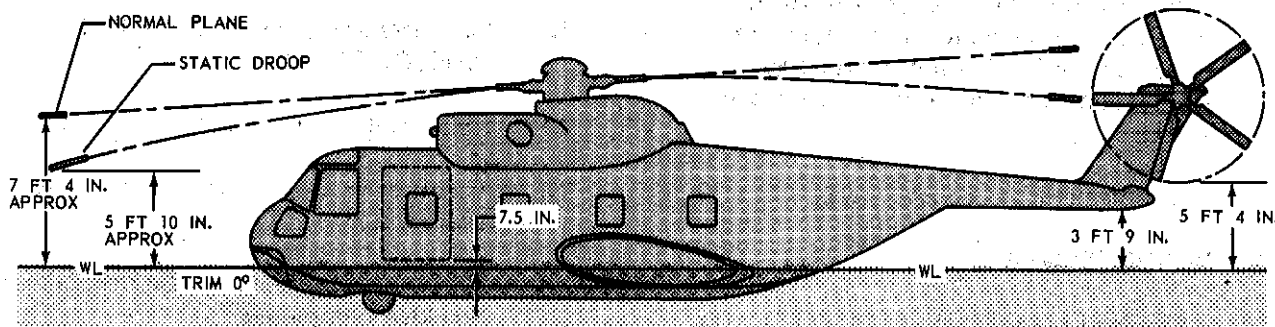
Figure 2-17. Water Clearance
