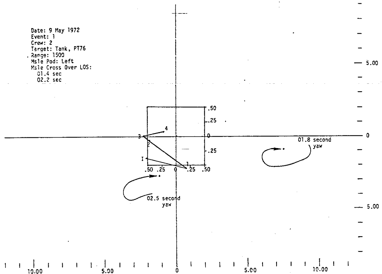
Figure B-46 (C; GDS) AIM ANGLE ERROR (TENTHS MIL) AND MAXIMUM MISSILE EXCURSION (MILS) DURING FLIGHT
