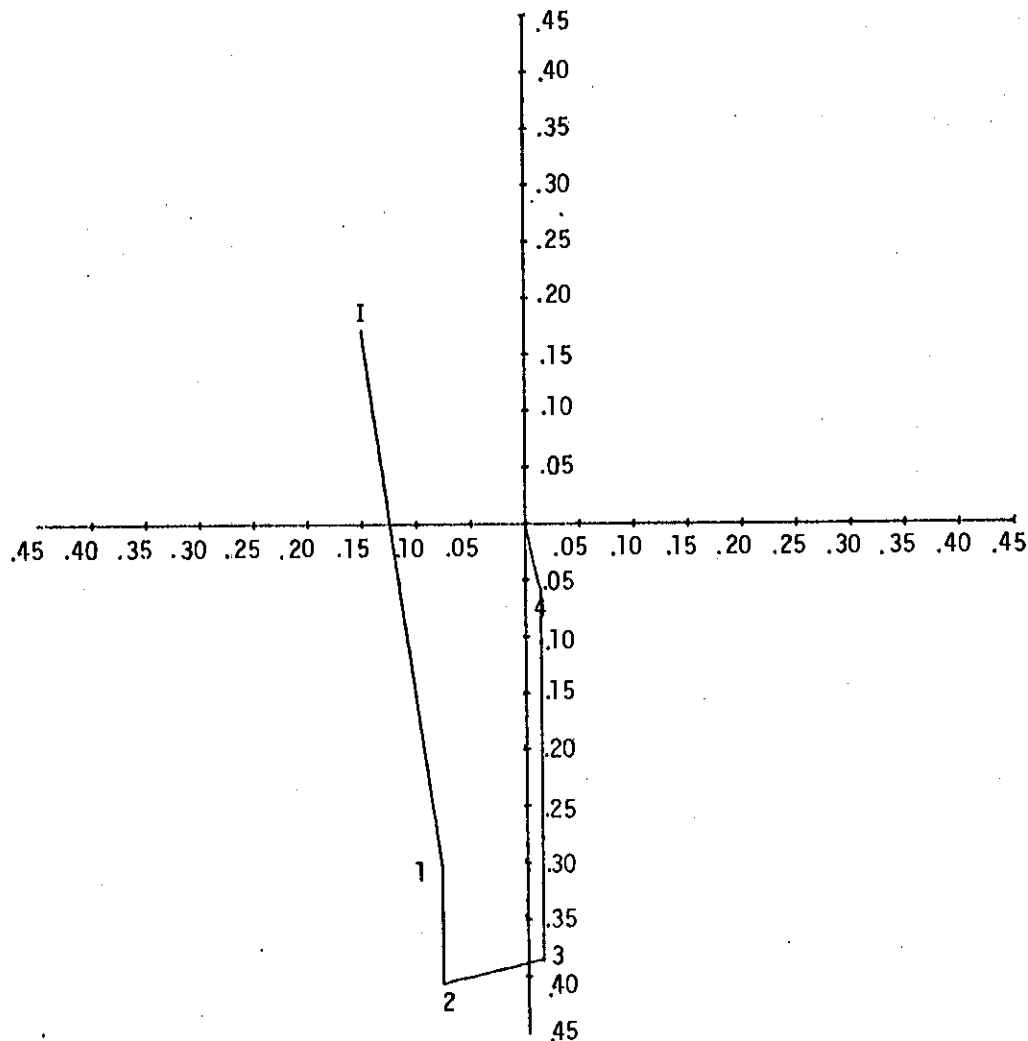
Figure B-21 (C; GDS) AIM ANGLE ERROR (TENTHS MIL) XM26 SYSTEM
