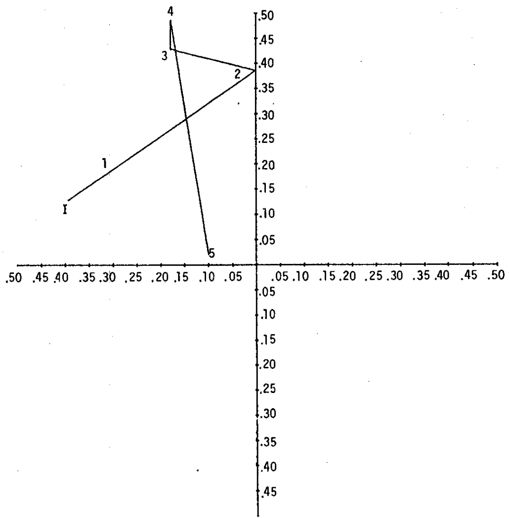
Figure B-22 (C; GDS) AIM ANGLE ERROR (TENTHS MIL) XM26 SYSTEM
