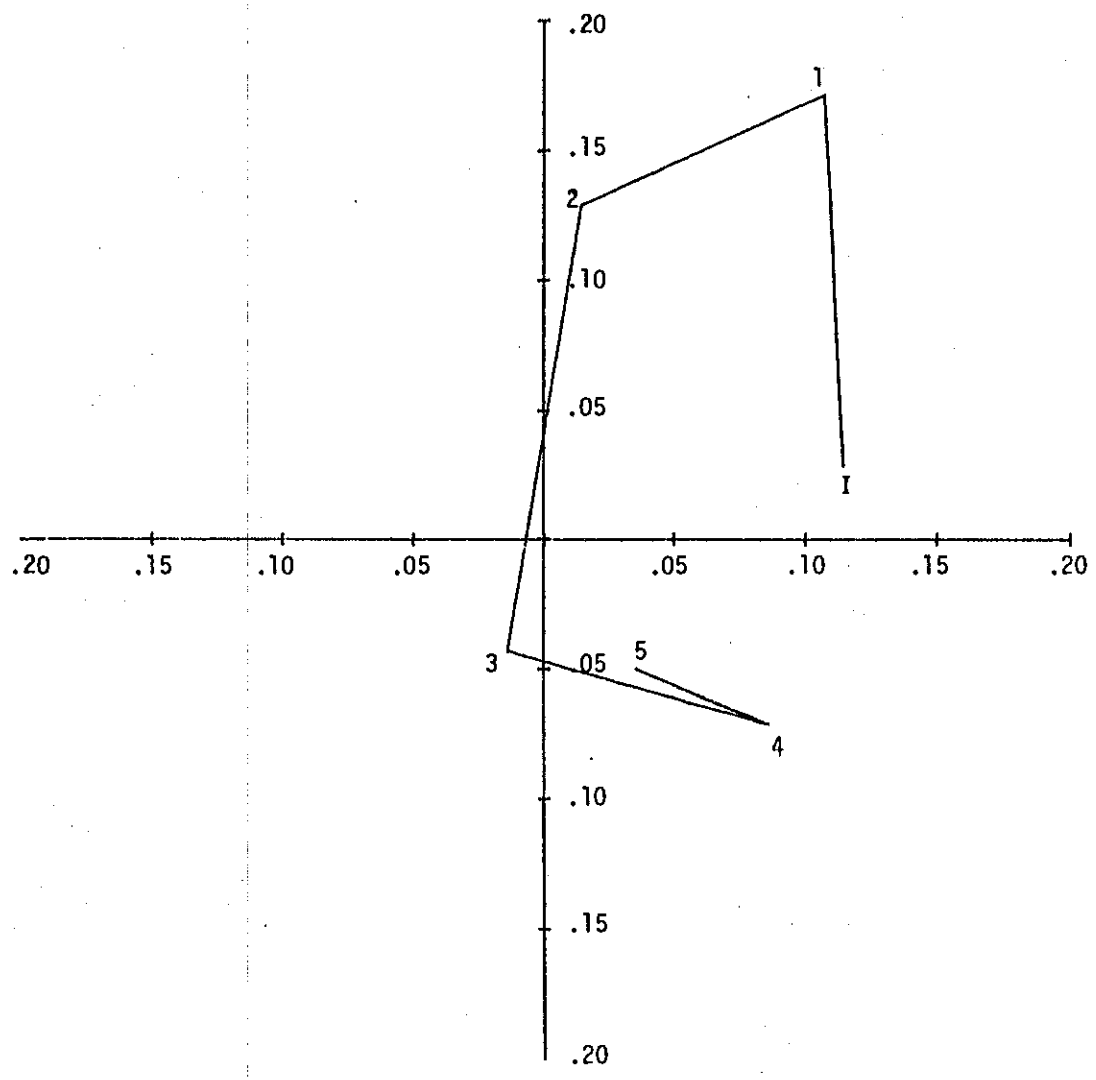
Figure B-31 (C; GDS) AIM ANGLE ERROR (TENTHS MIL) XM26 SYSTEM
