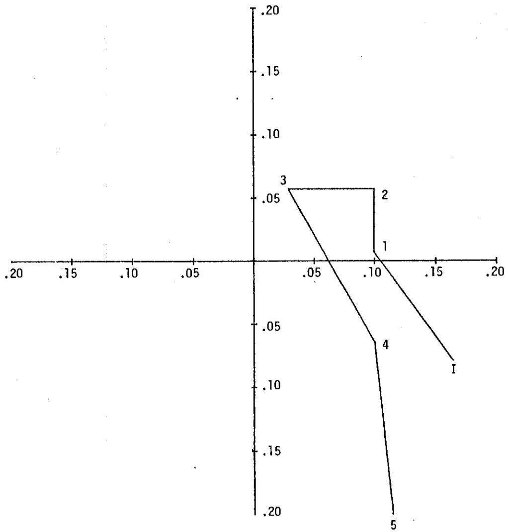
Figure B-25 (C; GDS) AIM ANGLE ERROR (TENTHS MIL) XM26 SYSTEM
