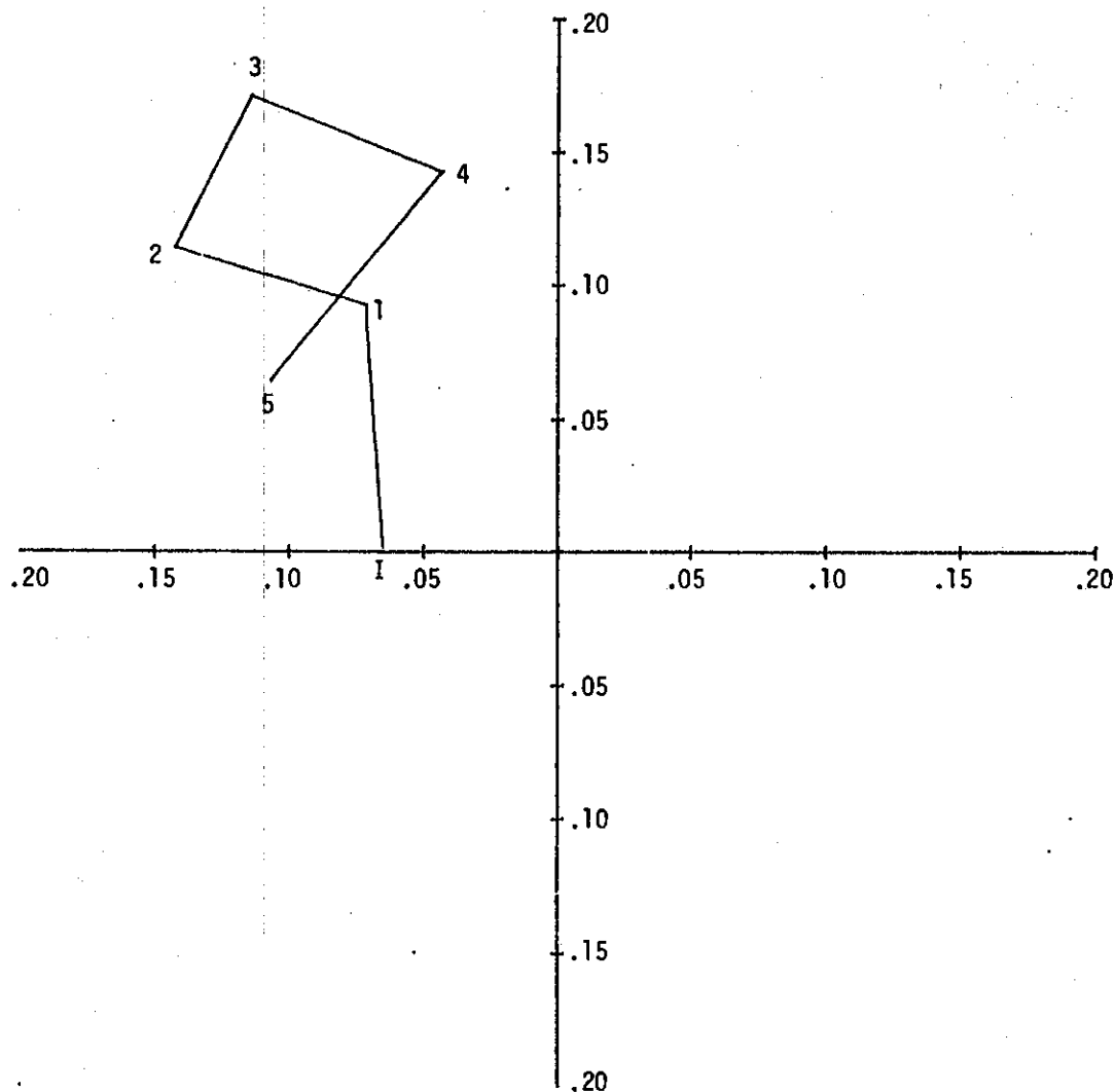
Figure B-32 (C; GDS) AIM ANGLE ERROR (TENTHS MIL) XM26 SYSTEM
