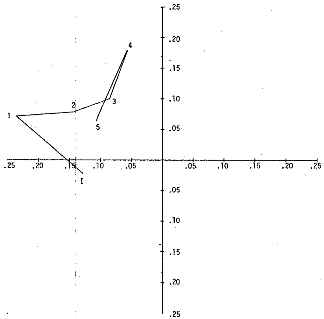
Figure B-34 (C; GDS) AIM ANGLE ERROR (TENTHS MIL) XM26 SYSTEM
