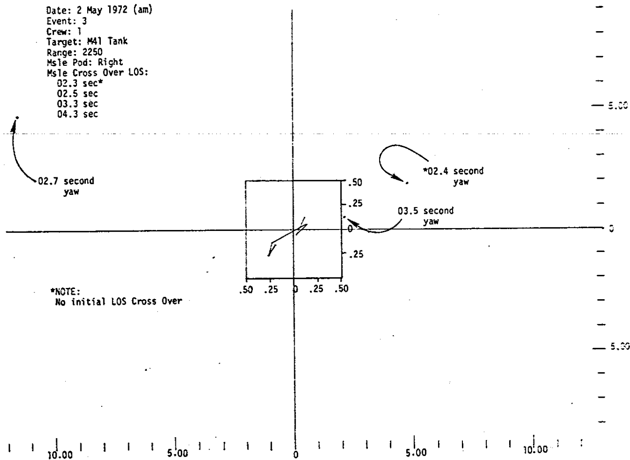
Figure B-38 (C; GDS) AIM Angle Error (TENTHS MIL) AND MAXIMUM MISSILE EXCURSION (MILS) DURING FLIGHT
