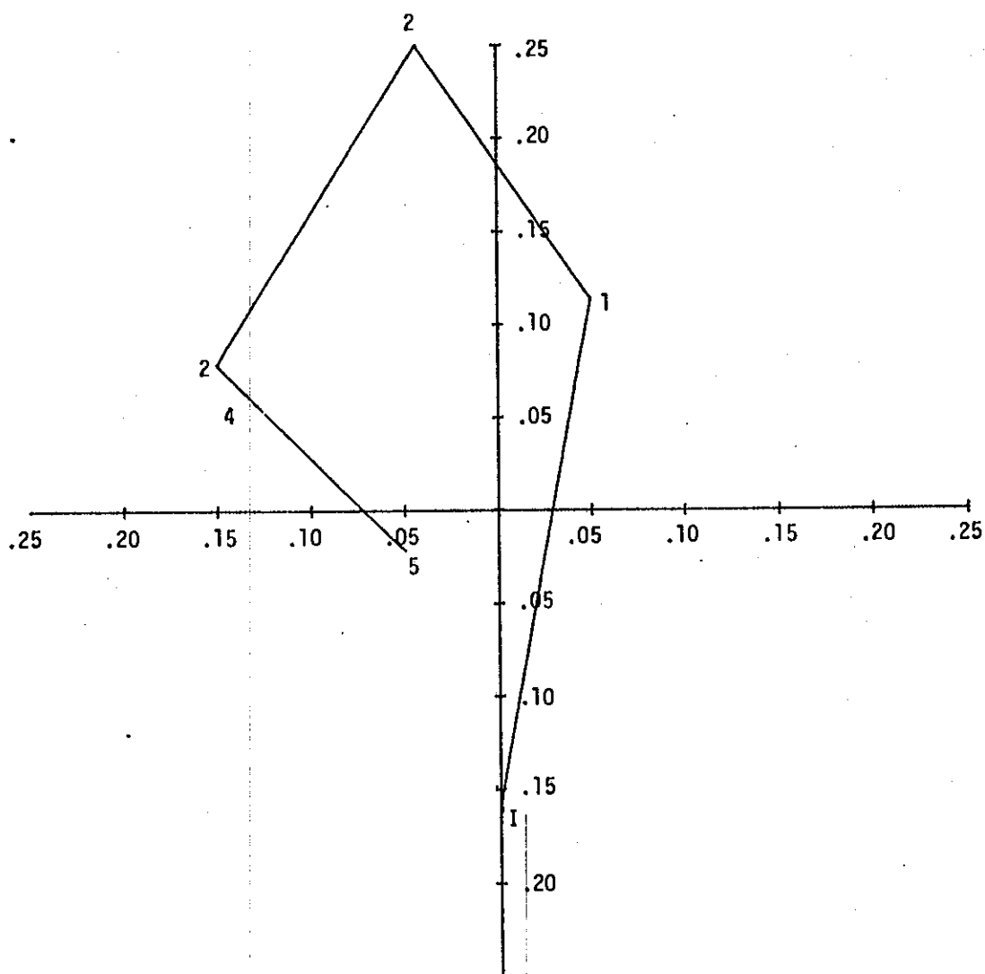
Figure B-30 (C; GDS) AIM ANGLE ERROR (TENTHS MIL) XM26 SYSTEM
