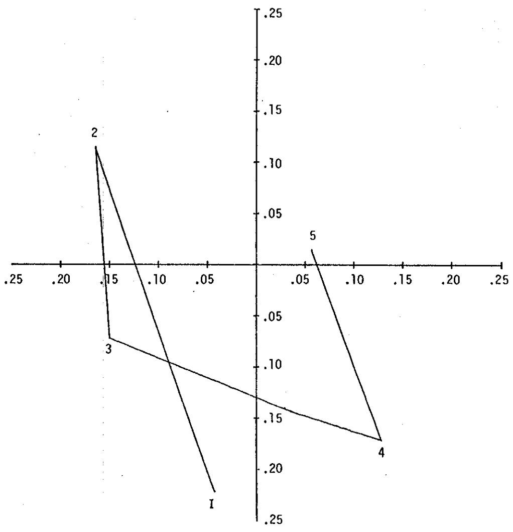
Figure B-27 (C; GDS) AIM ANGLE ERROR (TENTHS MIL) XM26 SYSTEM
