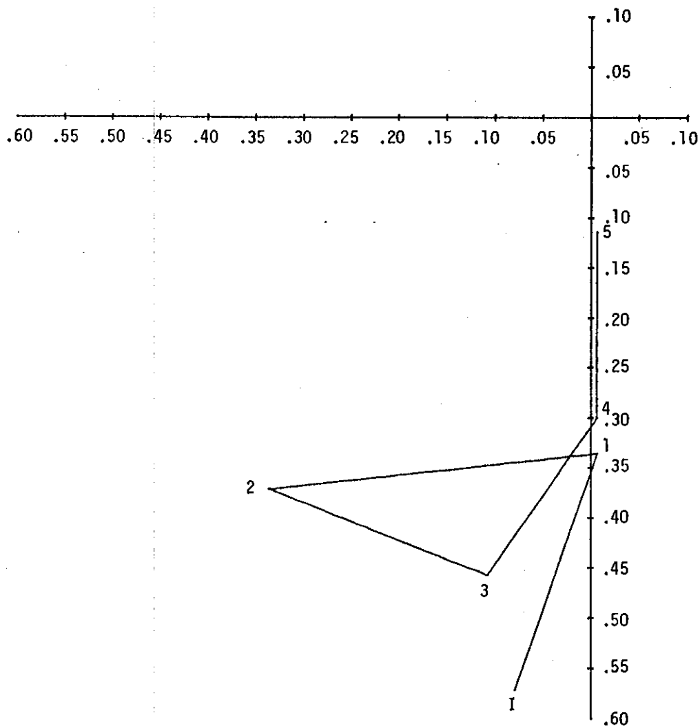
Figure B-35 (C; GDS) AIM ANGLE ERROR (TENTHS MIL) XM26 SYSTEM
