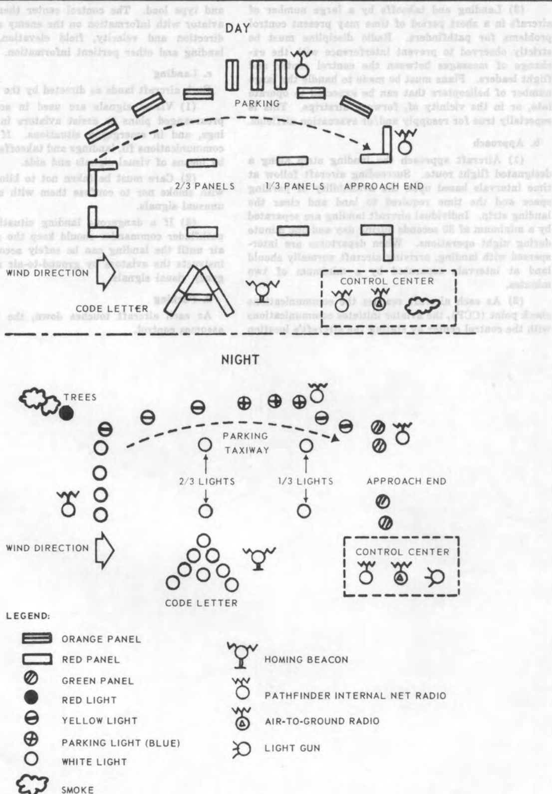
(Figure 4-7) FIXED WING AIRFIELD
