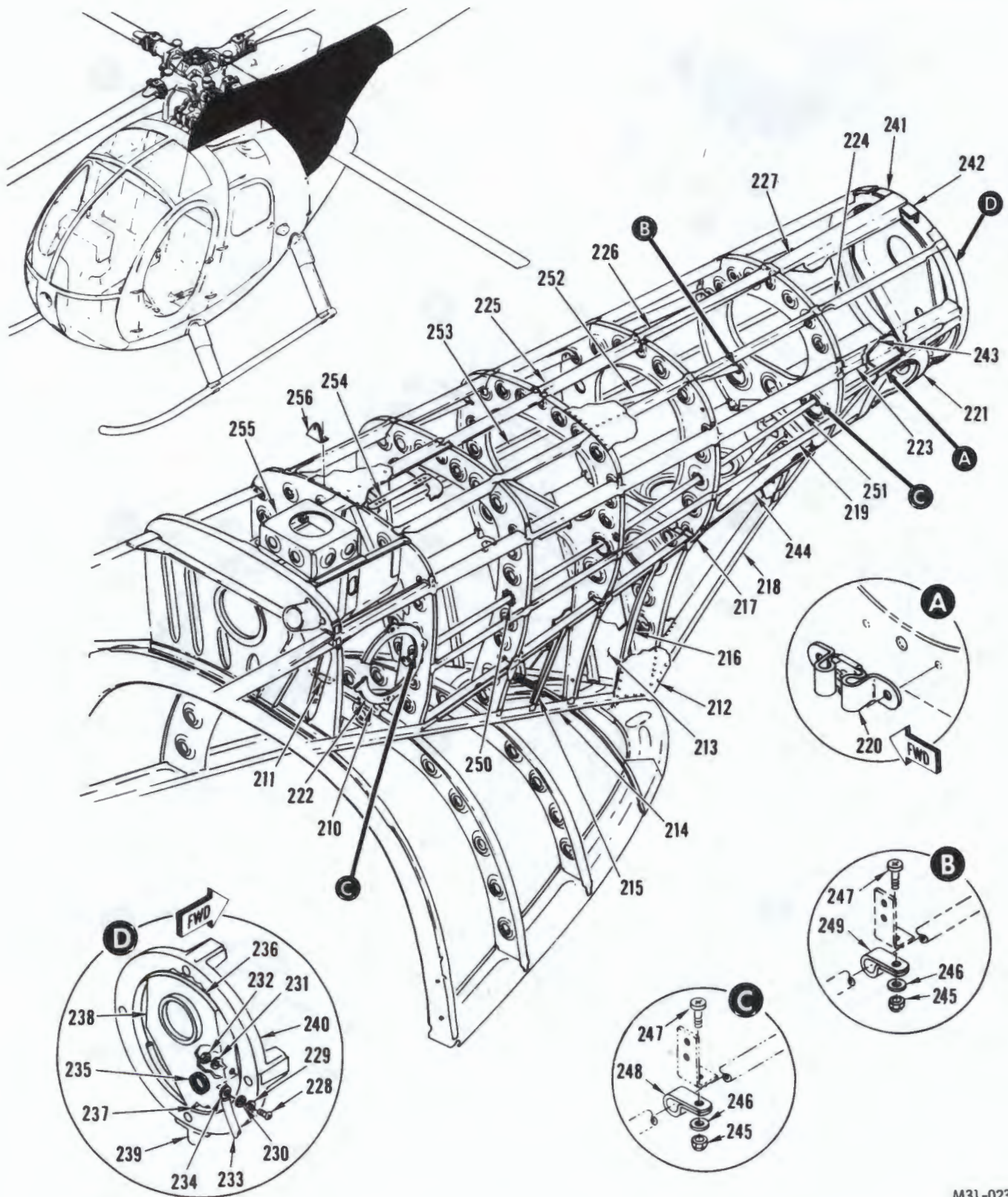
FIGURE 4. AFT SECTION INSTALLATION, FUSELAGE STRUCTURE (SHEET 7 OF 8)
