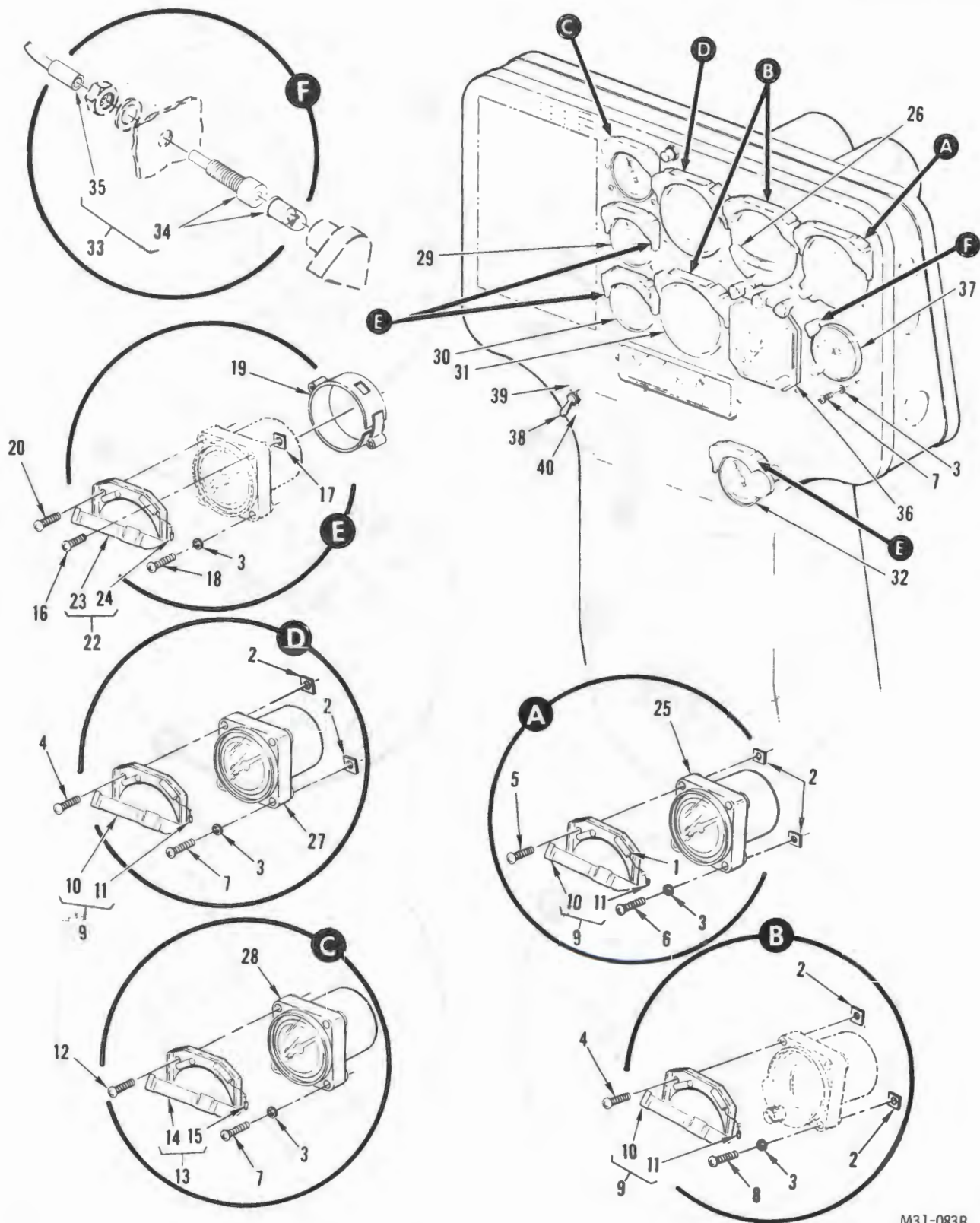
FIGURE 45. ELECTRICAL INSTALLATION (INSTRUMENTS, SERIES III) (SHEET 1 OF 2)
