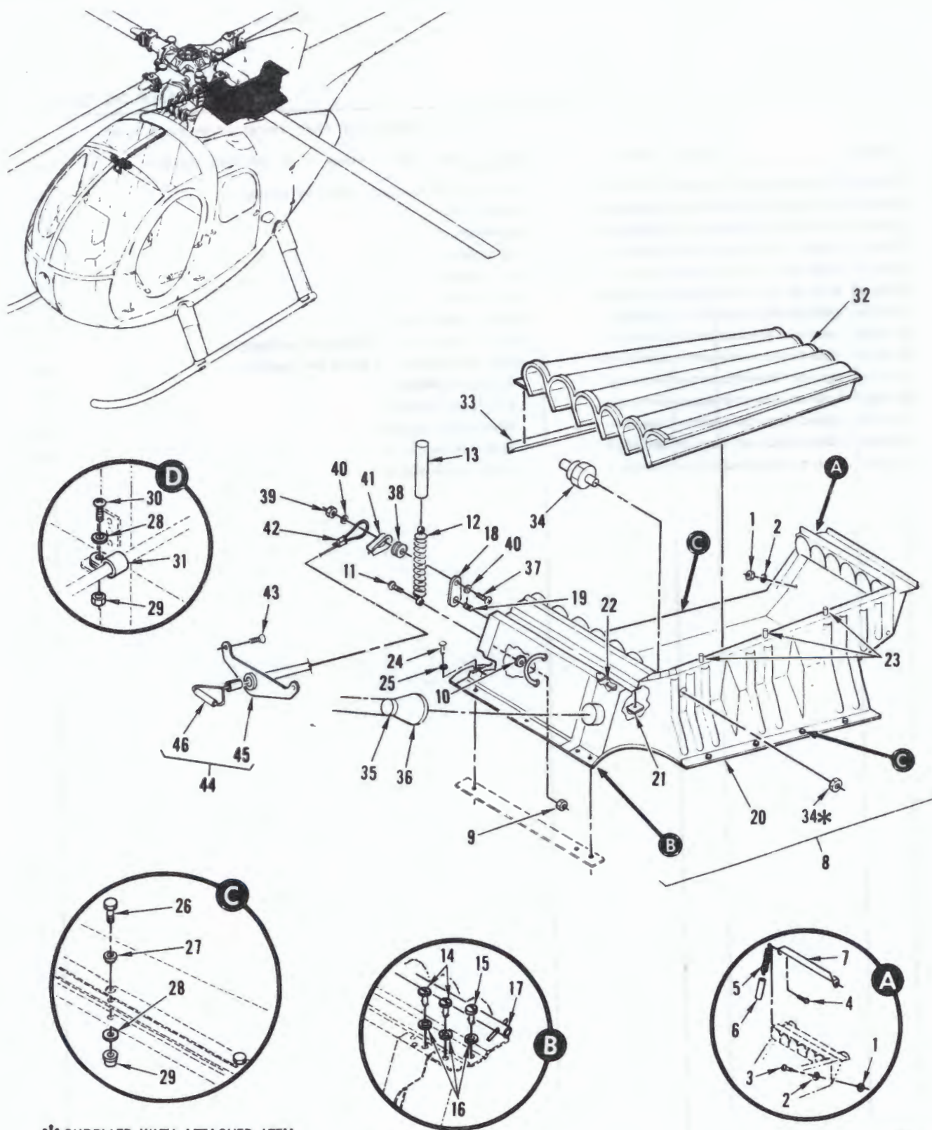
FIGURE 26. BARRIER FILTER
