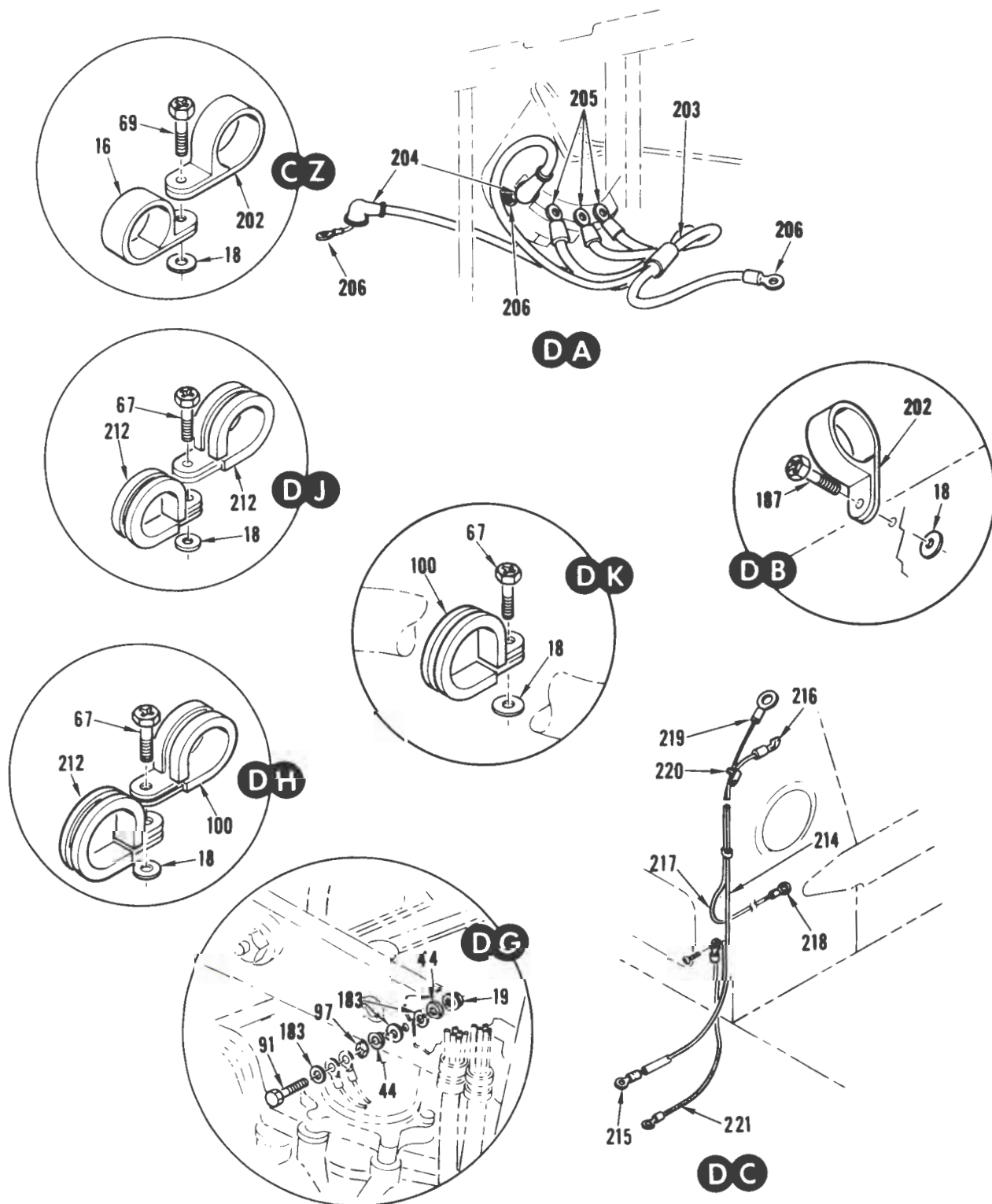
FIGURE 56. WIRE INSTALLATION, SERIES III (SHEET 15 OF 15)
