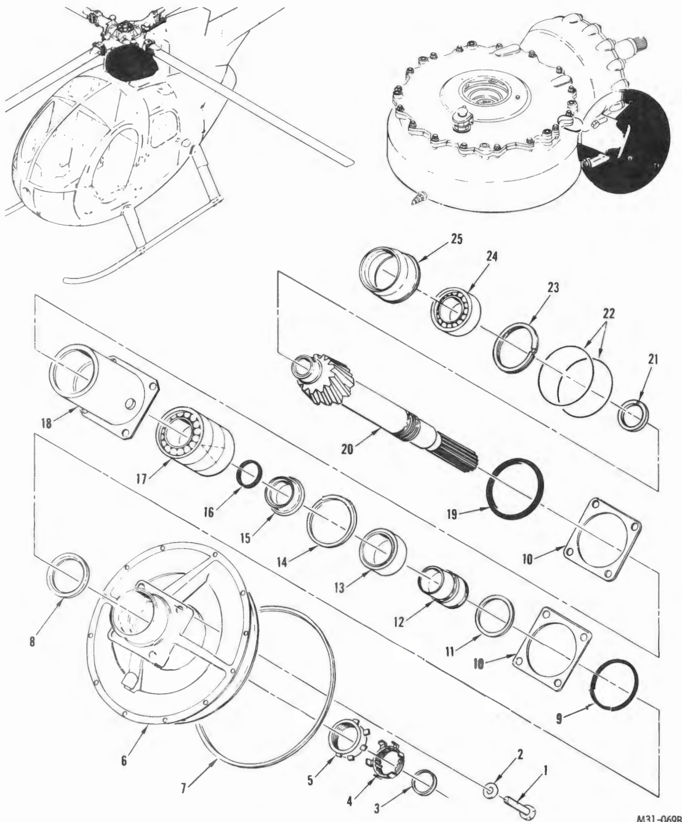
FIGURE 40. TRANSMISSION ASSEMBLY (DRIVES INSTALLATION) (SHEET 1 OF 3)
