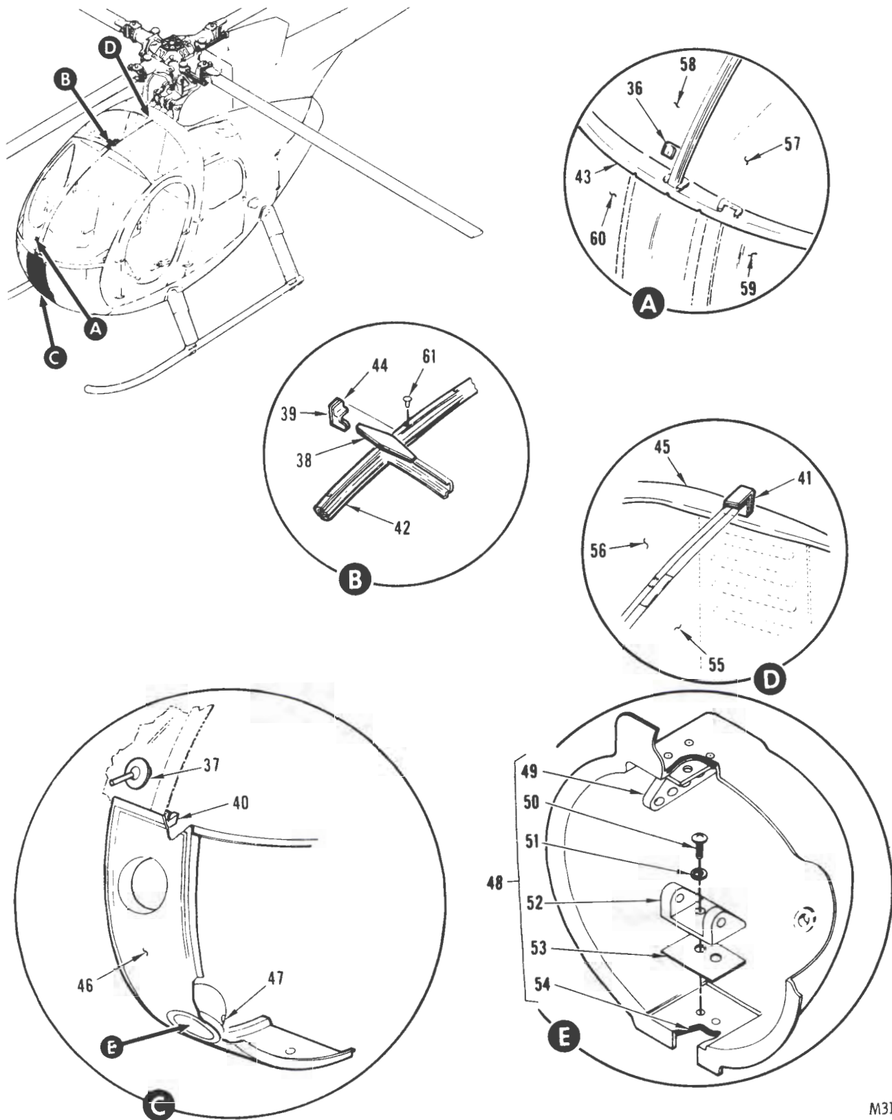
FIGURE 3. FORWARD SECTION INSTALLATION, FUSELAGE STRUCTURE (SHEET 2 OF 2)
