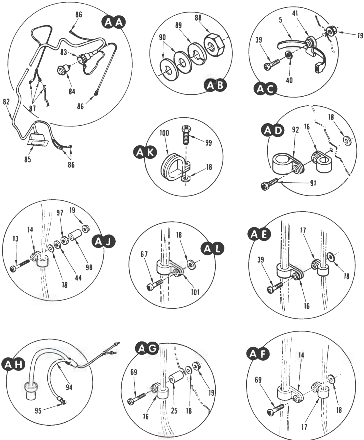
FIGURE 56. WIRE INSTALLATION, SERIES III (SHEET 8 OF 15)
