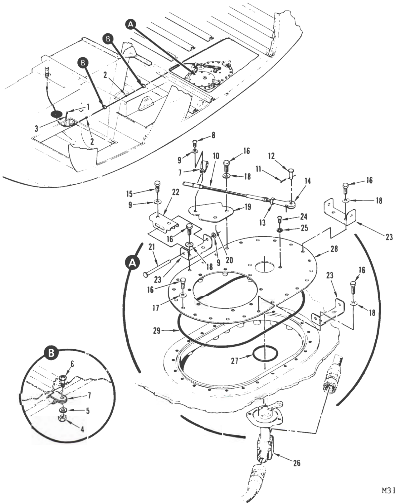
FIGURE 60. CRASHWORTHY FUEL SYSTEM – FUEL SHUTOFF AND FUEL QUANTITY TRANSMITTER (SHEET 1 OF 2)
