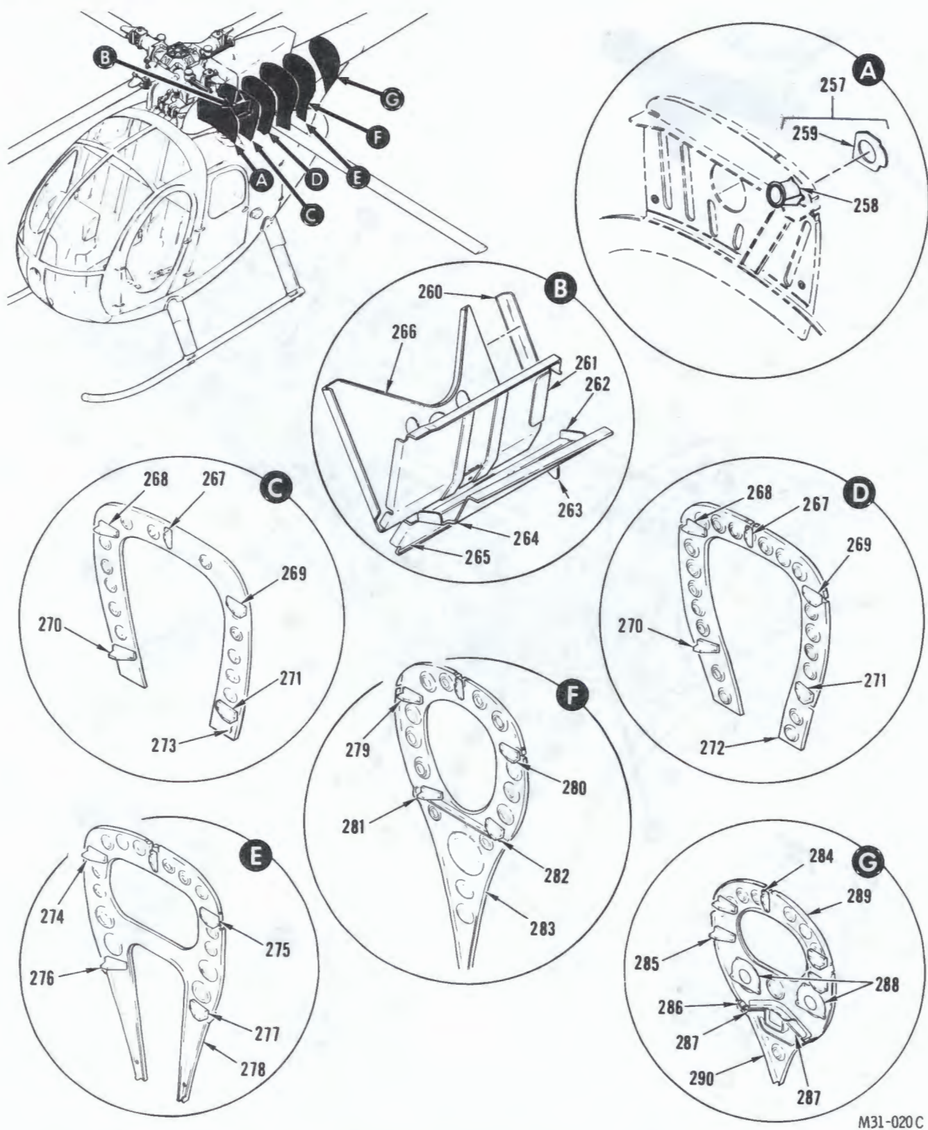
FIGURE 4. AFT SECTION INSTALLATION, FUSELAGE STRUCTURE (SHEET 8 OF 8)
