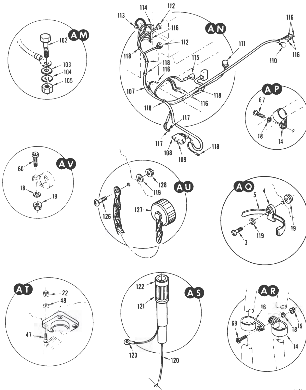
FIGURE 56. WIRE INSTALLATION, SERIES III (SHEET 9 OF 15)
