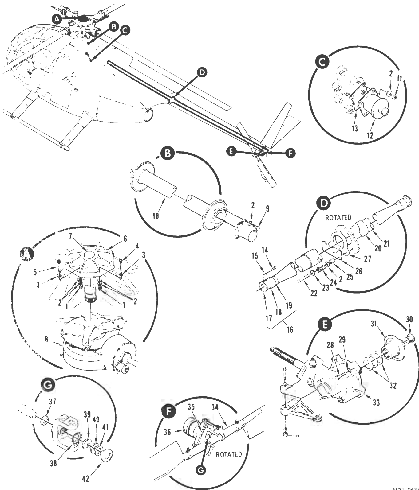
FIGURE 37. DRIVE SYSTEM INSTALLATION
