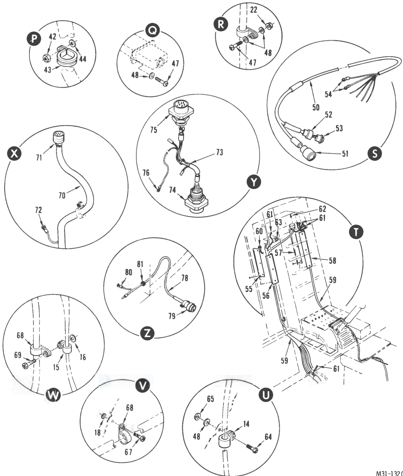
FIGURE 56. WIRE INSTALLATION, SERIES III (SHEET 7 OF 15)
