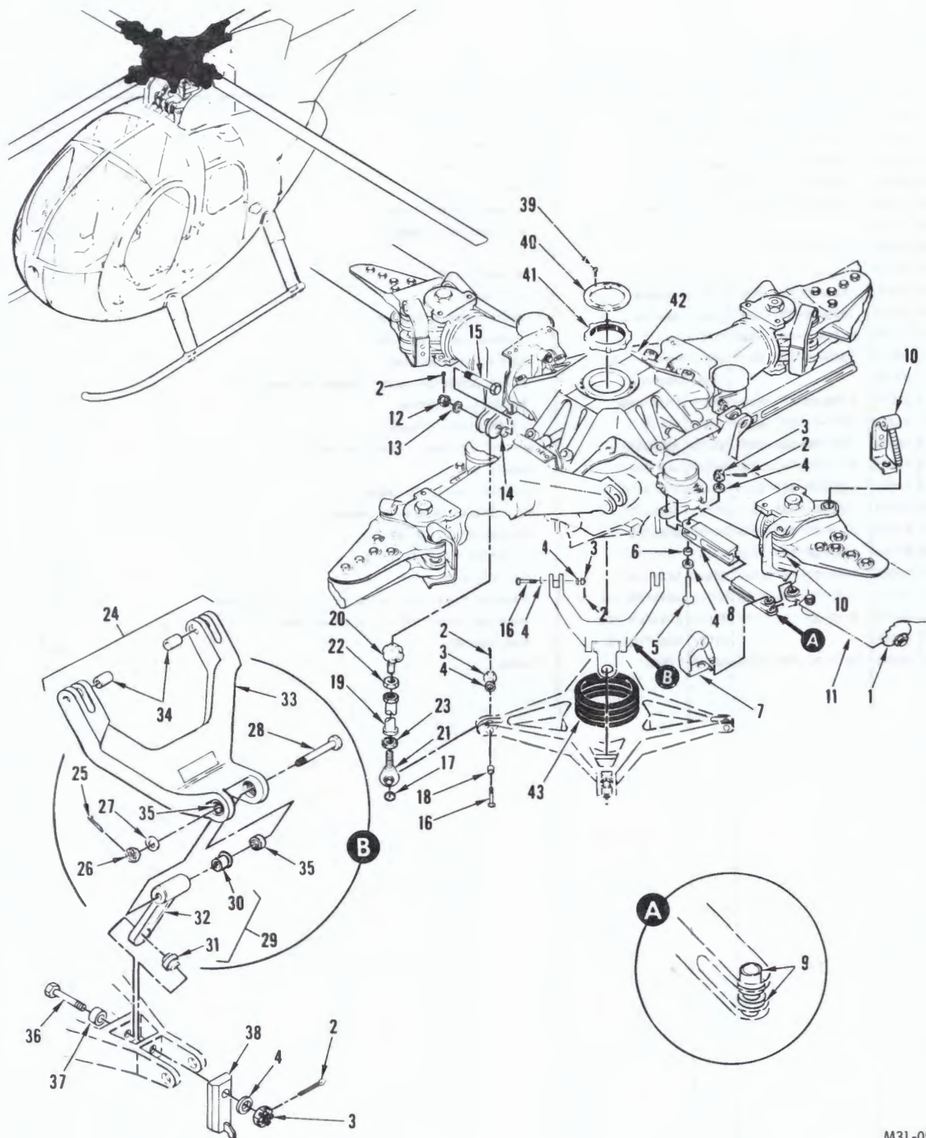
FIGURE 30. MAIN ROTOR INSTALLATION
