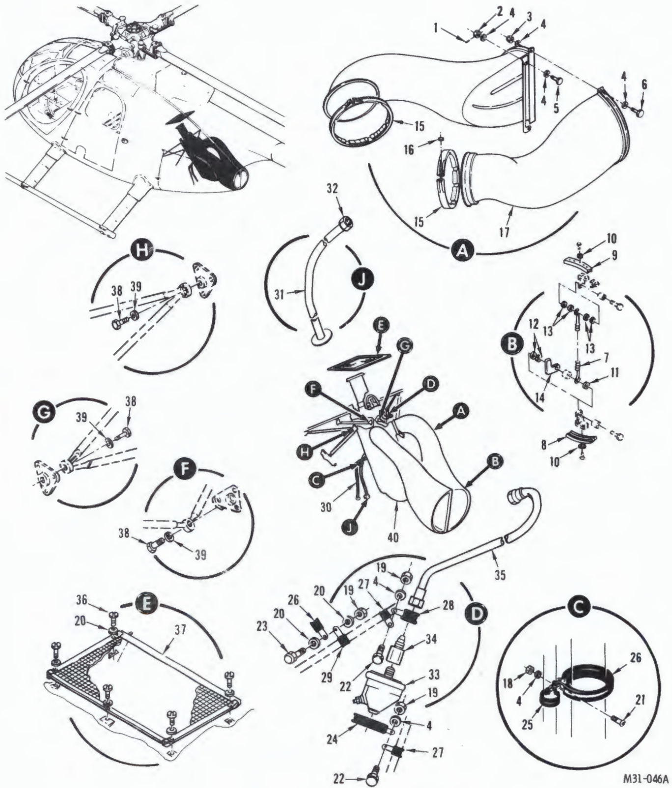
FIGURE 22. ENGINE INSTALLATION, HELICOPTER
