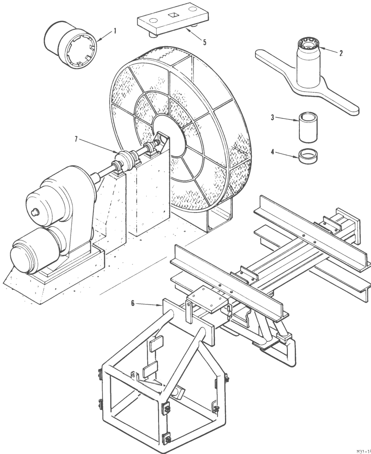
FIGURE A7. AIRFRAME TOOLS
