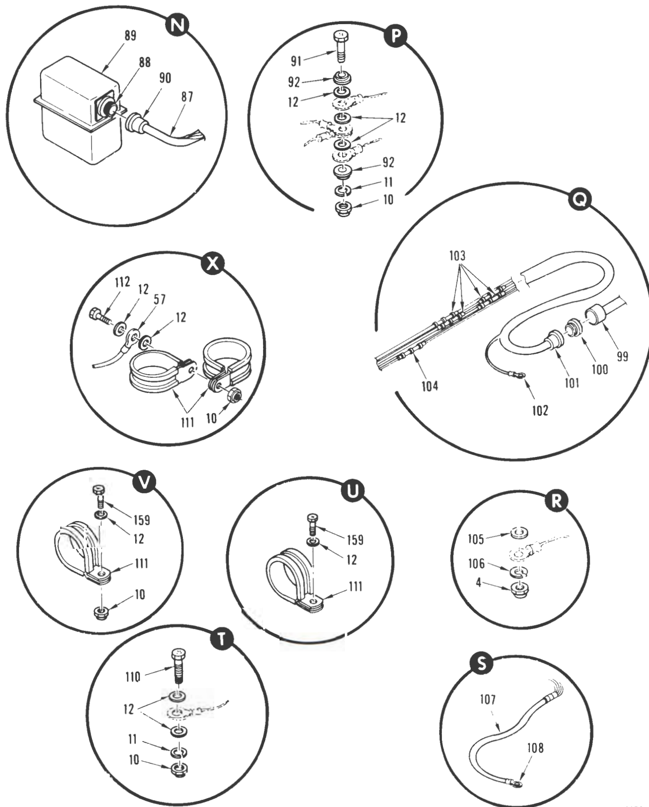
FIGURE 55. WIRE INSTALLATION, SERIES I AND II (SHEET 7 OF 9)
