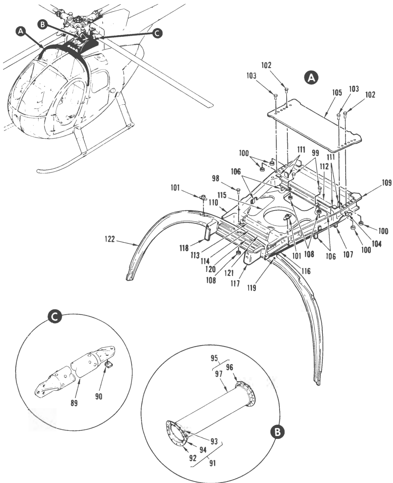
FIGURE 4. AFT SECTION INSTALLATION, FUSELAGE STRUCTURE (SHEET 4 OF 8)
