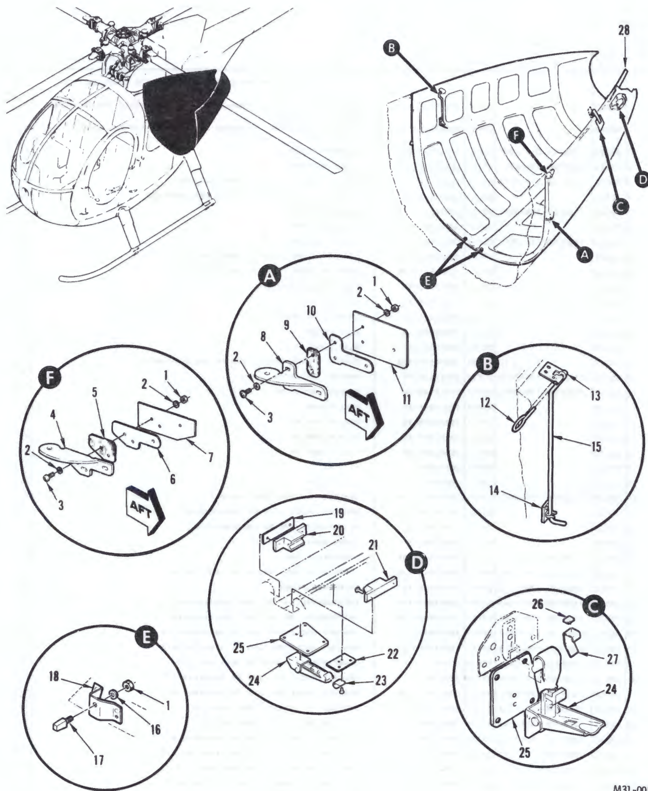
FIGURE 13. DOOR, ACCESS, ENGINE
