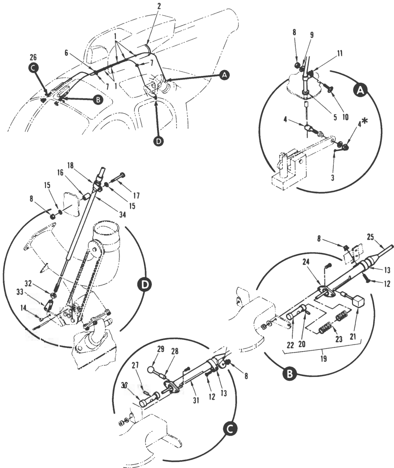
FIGURE 78. HEATING SYSTEM INSTALLATION (HEAT AND DE-ICER VALVE CONTROL)
