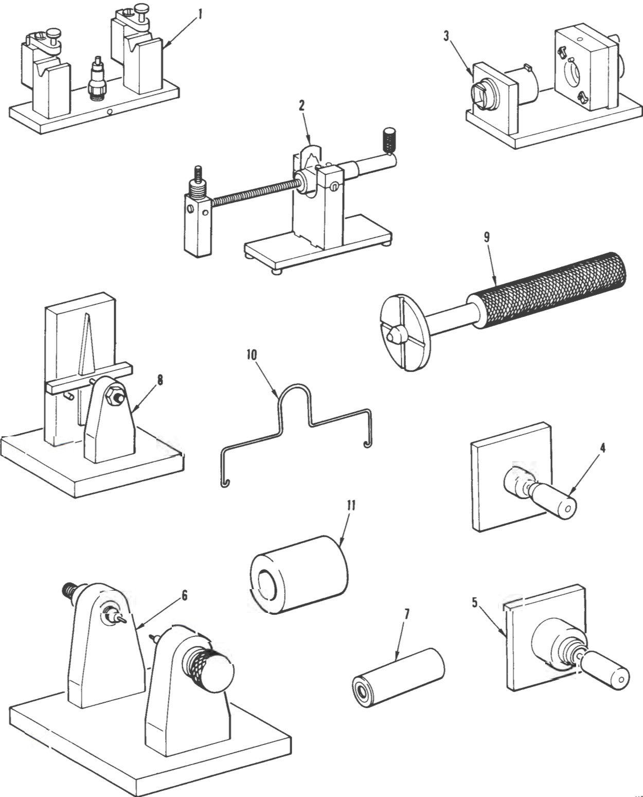
FIGURE A16. AIRFRAME TOOLS
