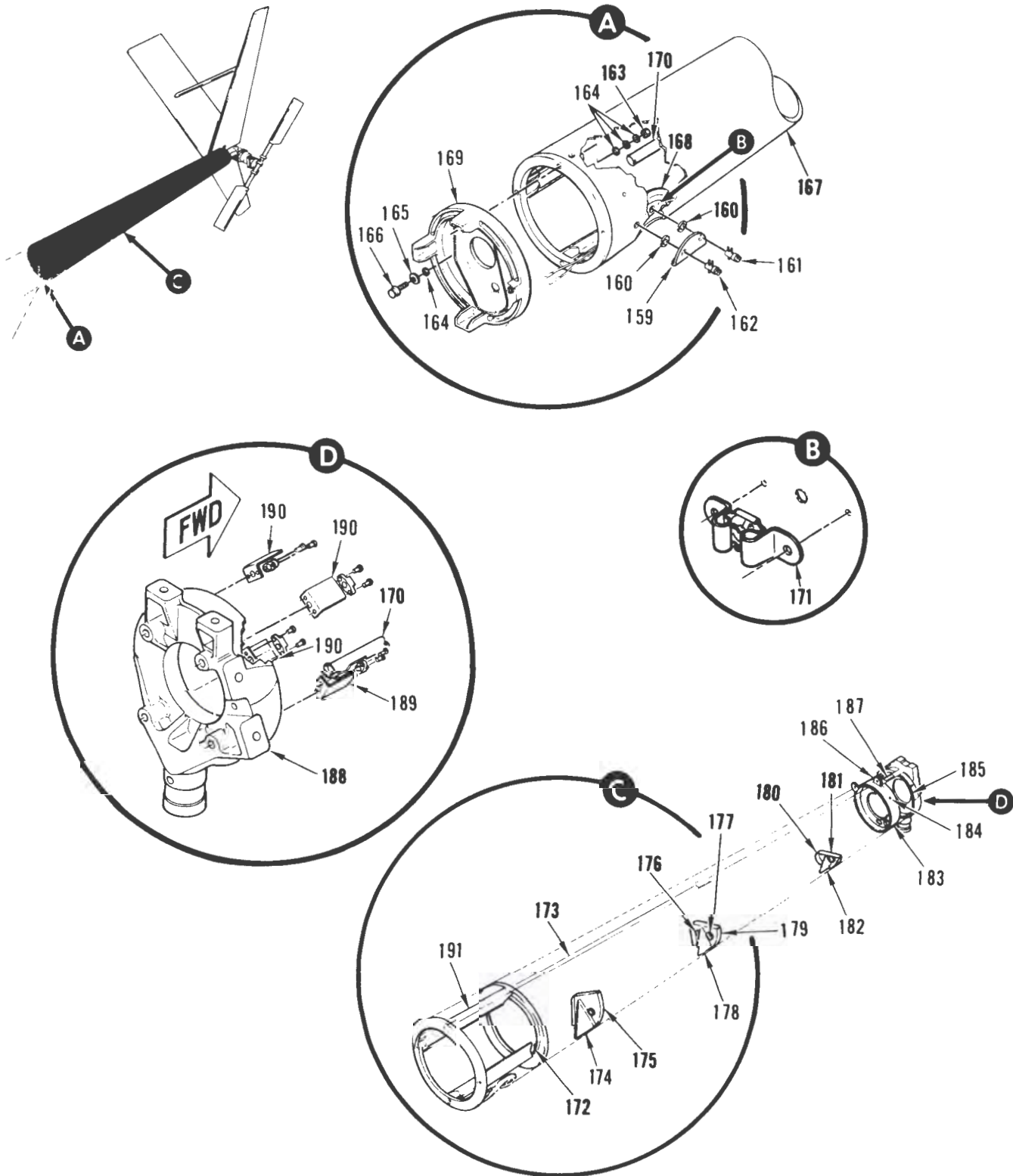
FIGURE 2. FUSELAGE STRUCTURE, COMPLETE (SHEET 7 OF 9)
