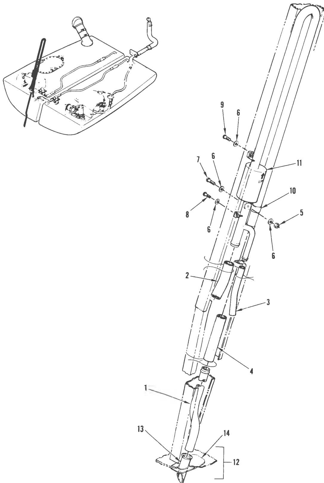
FIGURE 59. CRASHWORTHY FUEL SYSTEM - VENT (SHEET 1 OF 2)
