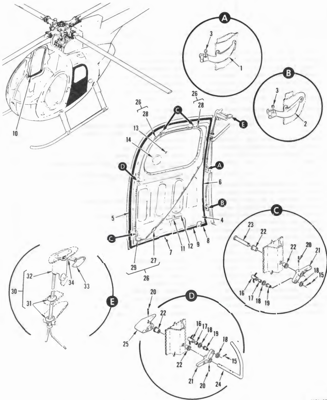
FIGURE 15. DOOR, PASSENGER
