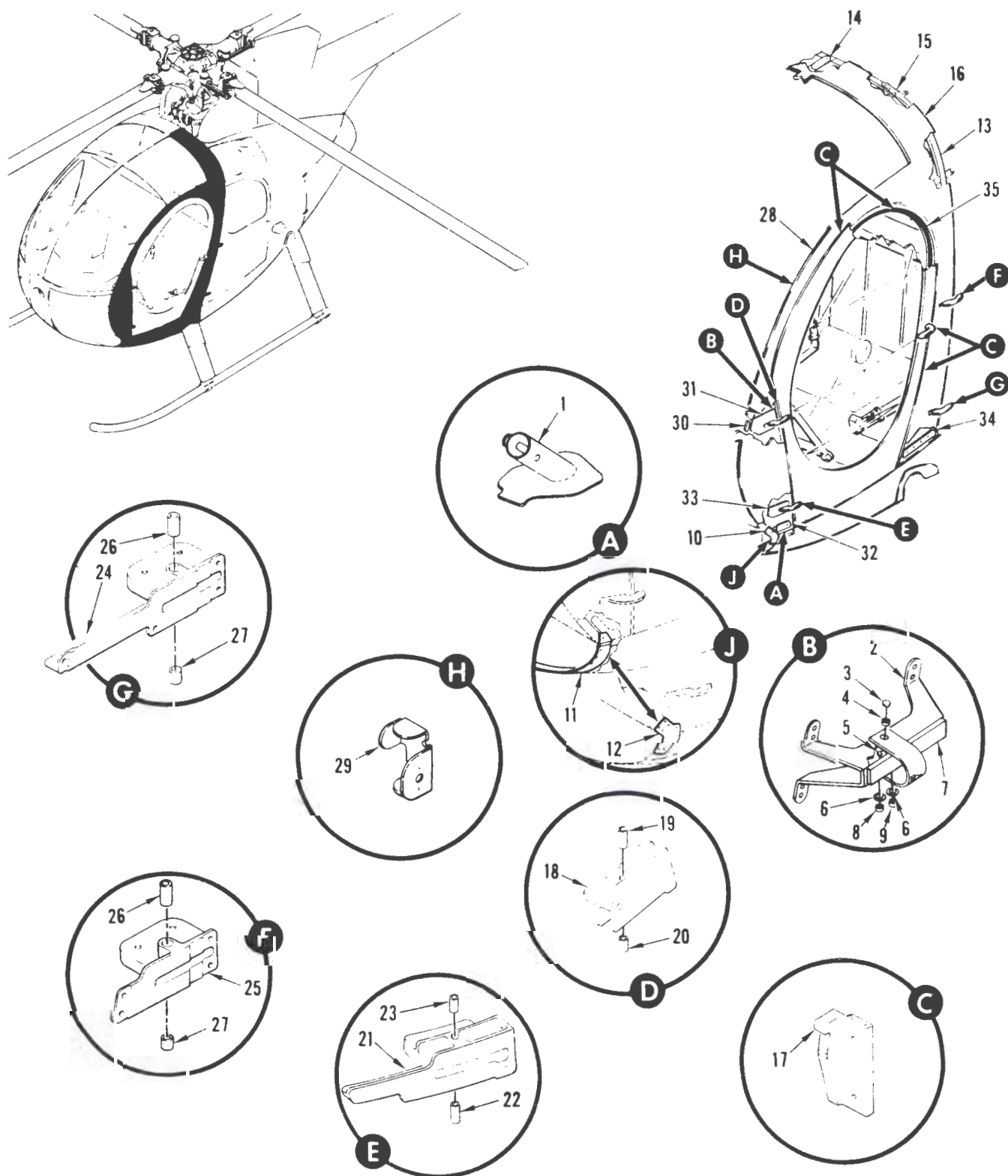
FIGURE 3. FORWARD SECTION INSTALLATION, FUSELAGE STRUCTURE (SHEET 1 OF 2)
