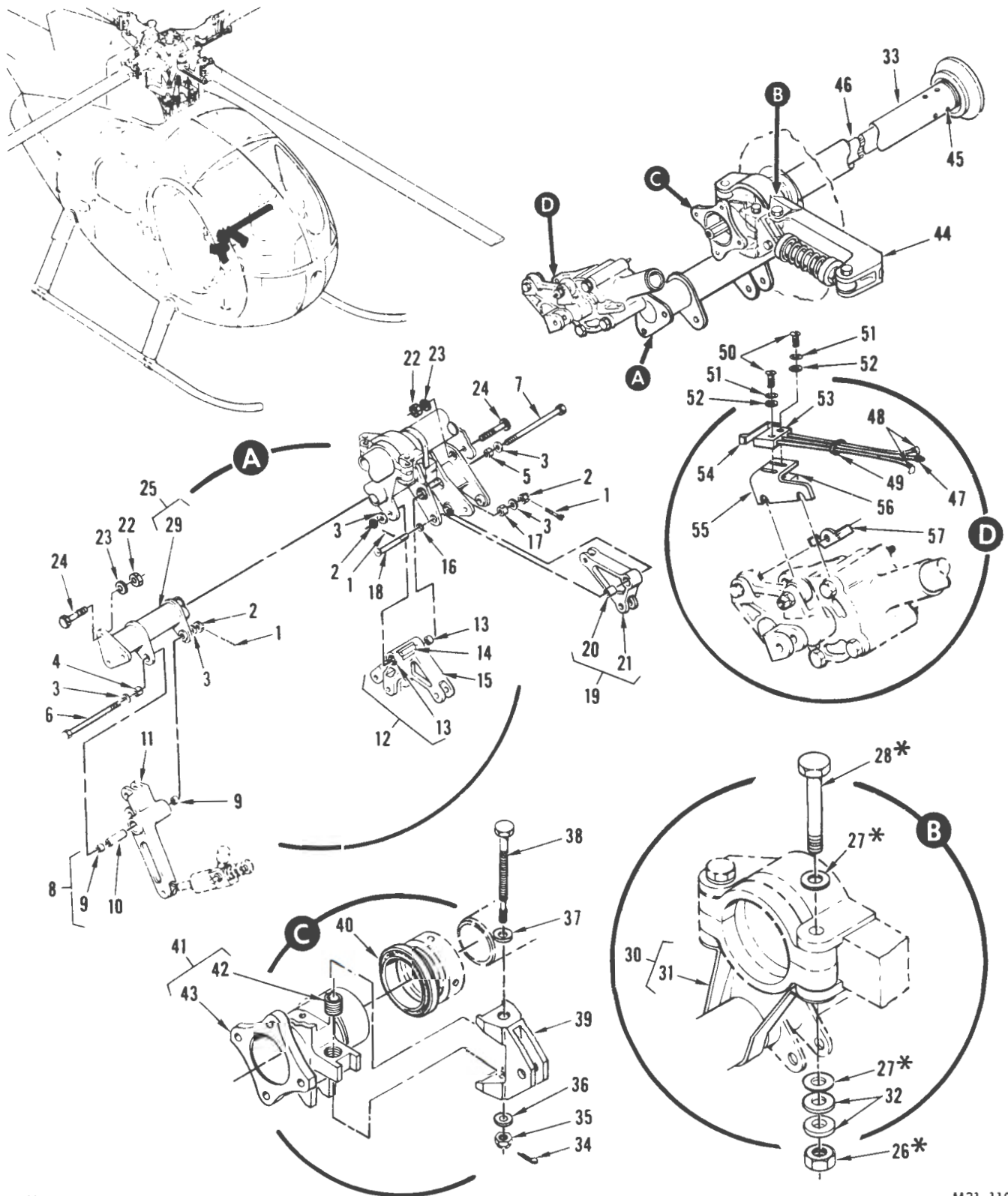
FIGURE 73. FORWARD CONTROLS INSTALLATION (PART II)
