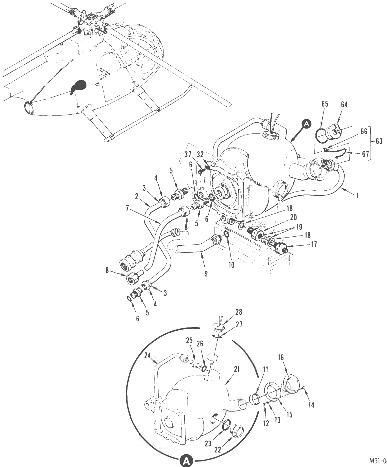
FIGURE 21. ENGINE OIL SYSTEM INSTALLATION (SHEET 1 OF 2)
