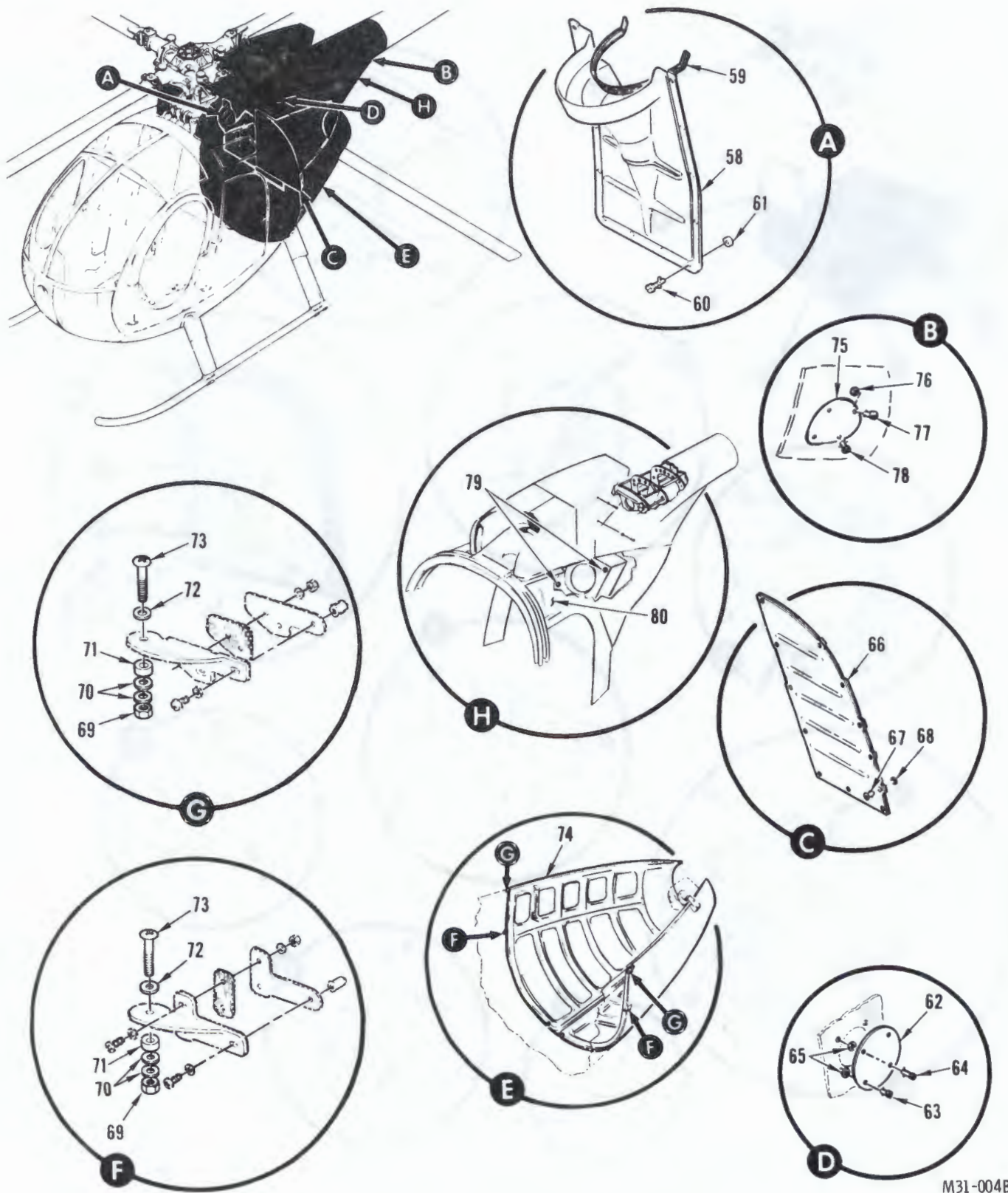
FIGURE 2. FUSELAGE STRUCTURE, COMPLETE (SHEET 3 OF 9)
