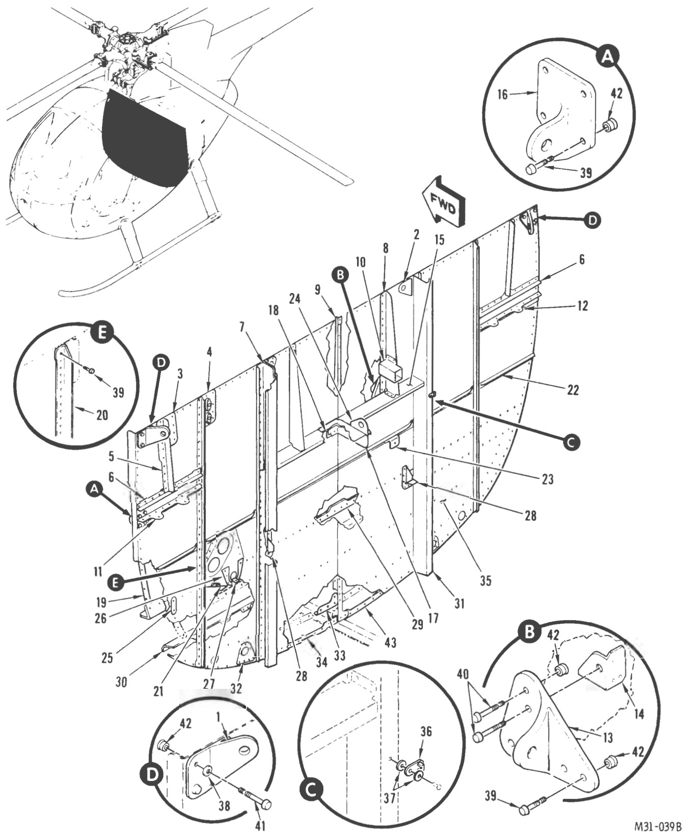
FIGURE 10. FRAME INSTALLATION, LOWER SECTION
