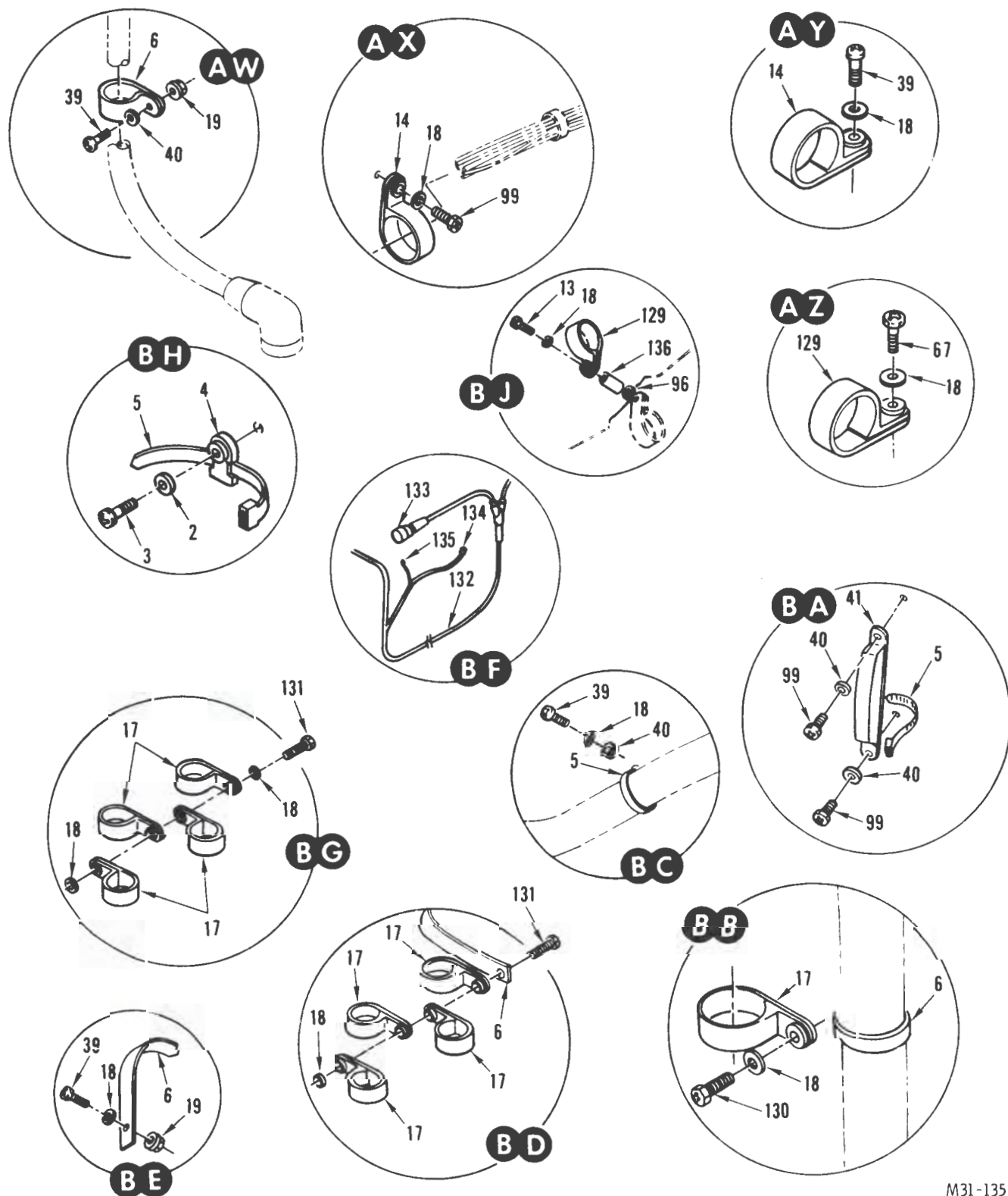
FIGURE 56. WIRE INSTALLATION, SERIES III (SHEET 10 OF 15)
