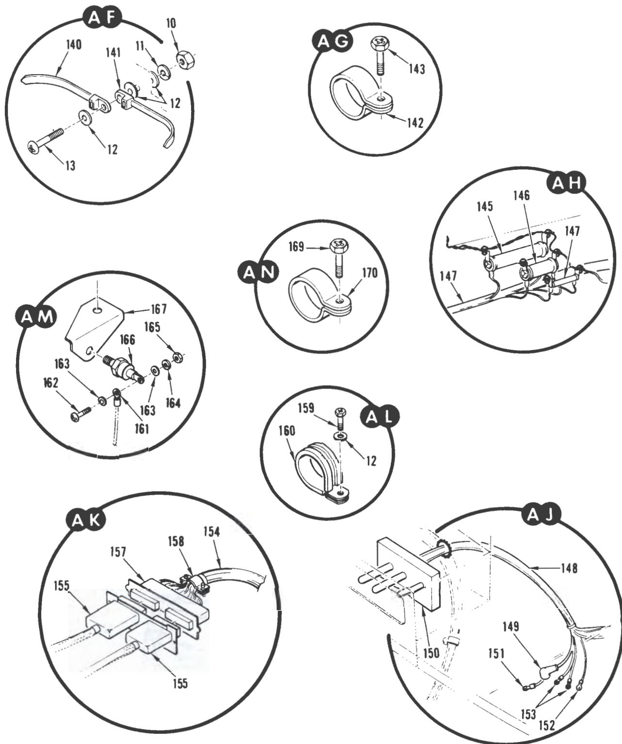
FIGURE 55. WIRE INSTALLATION, SERIES I AND II (SHEET 9 OF 9)
