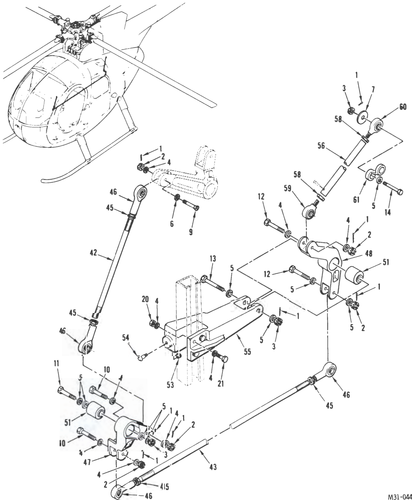
FIGURE 29. ENGINE CONTROLS INSTALLATION (SHEET 1 OF 4)
