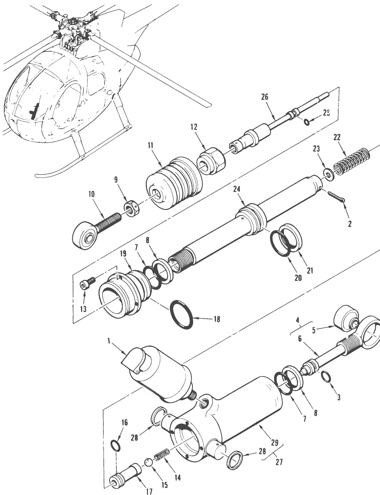
FIGURE 70. LOCK CONTROL SYSTEM, ONE-WAY
