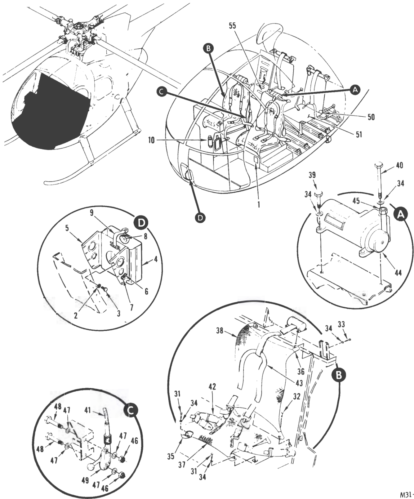
FIGURE 16. EQUIPMENT INSTALLATION (SHEET 2 OF 2)
