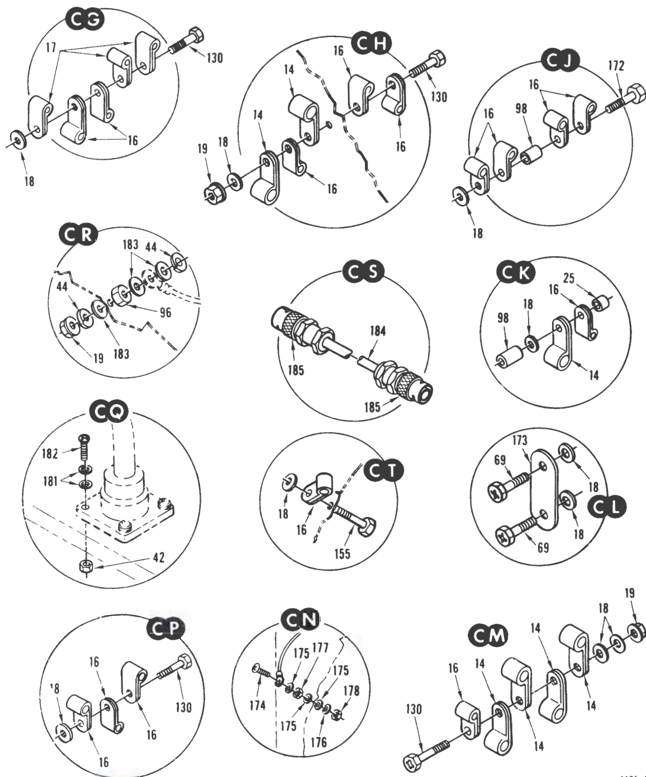
FIGURE 56. WIRE INSTALLATION, SERIES III (SHEET 13 OF 15)
