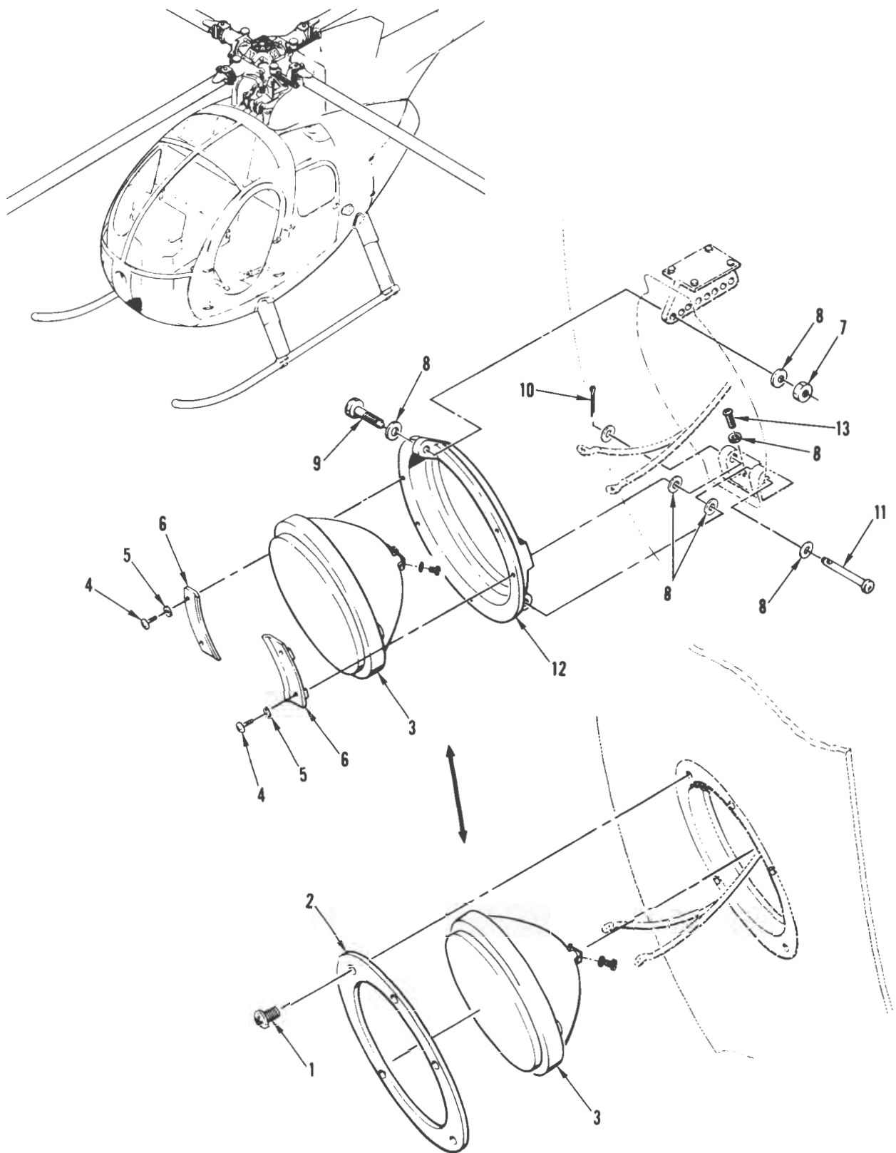
FIGURE 53. EXTERIOR LIGHTING INSTALLATION (SHEET 1 OF 2)
