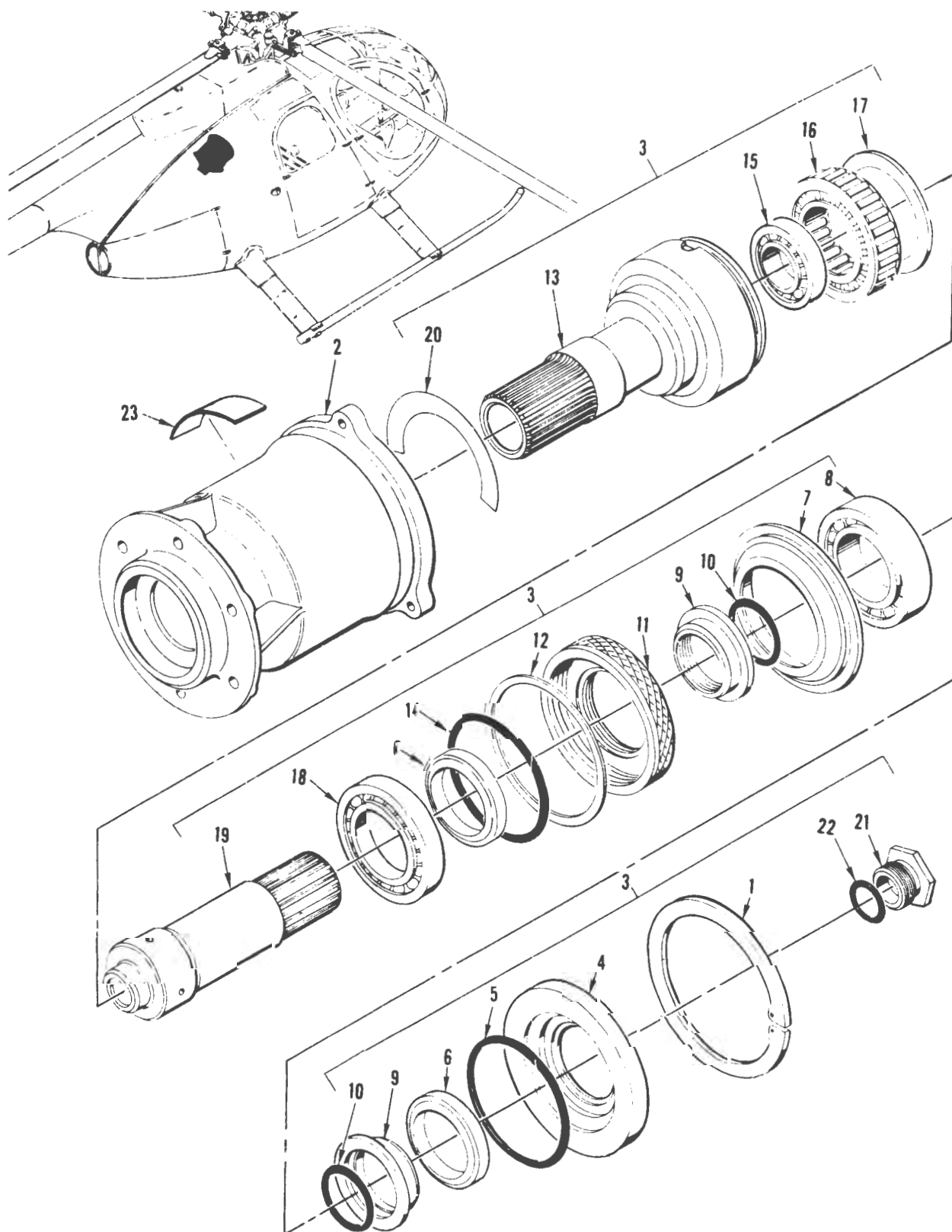
FIGURE 41. CLUTCH, TRANSMISSION
