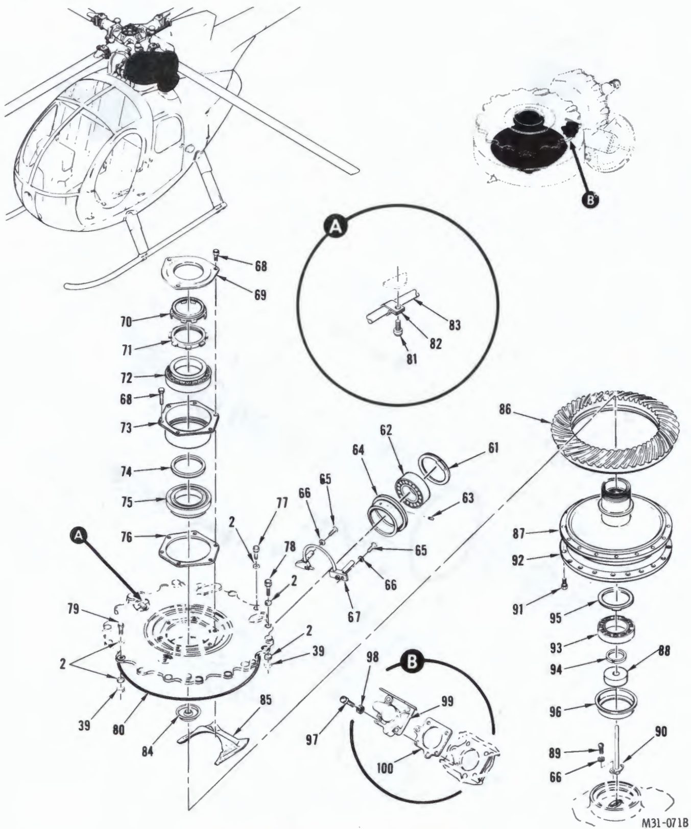
FIGURE 40. TRANSMISSION ASSEMBLY (DRIVES INSTALLATION) (SHEET 3 of 3)
