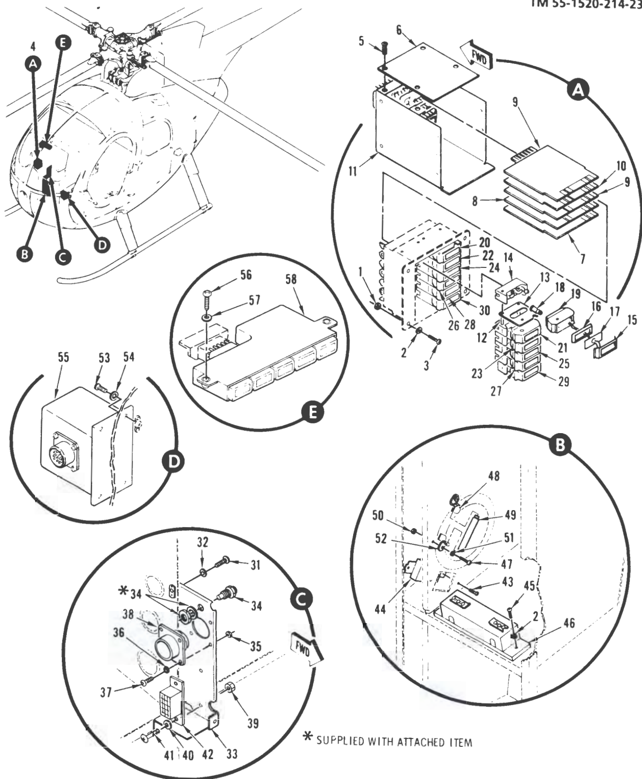
FIGURE 50. ELECTRICAL INSTALLATION (CONSOLE AND WARNING INDICATORS) (SHEET 1 OF 2)
