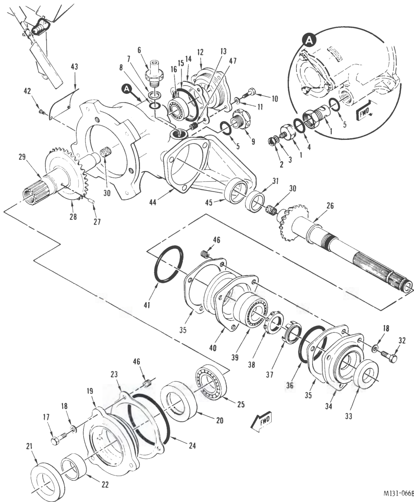
FIGURE 43. TRANSMISSION ASSEMBLY, TAIL ROTOR
