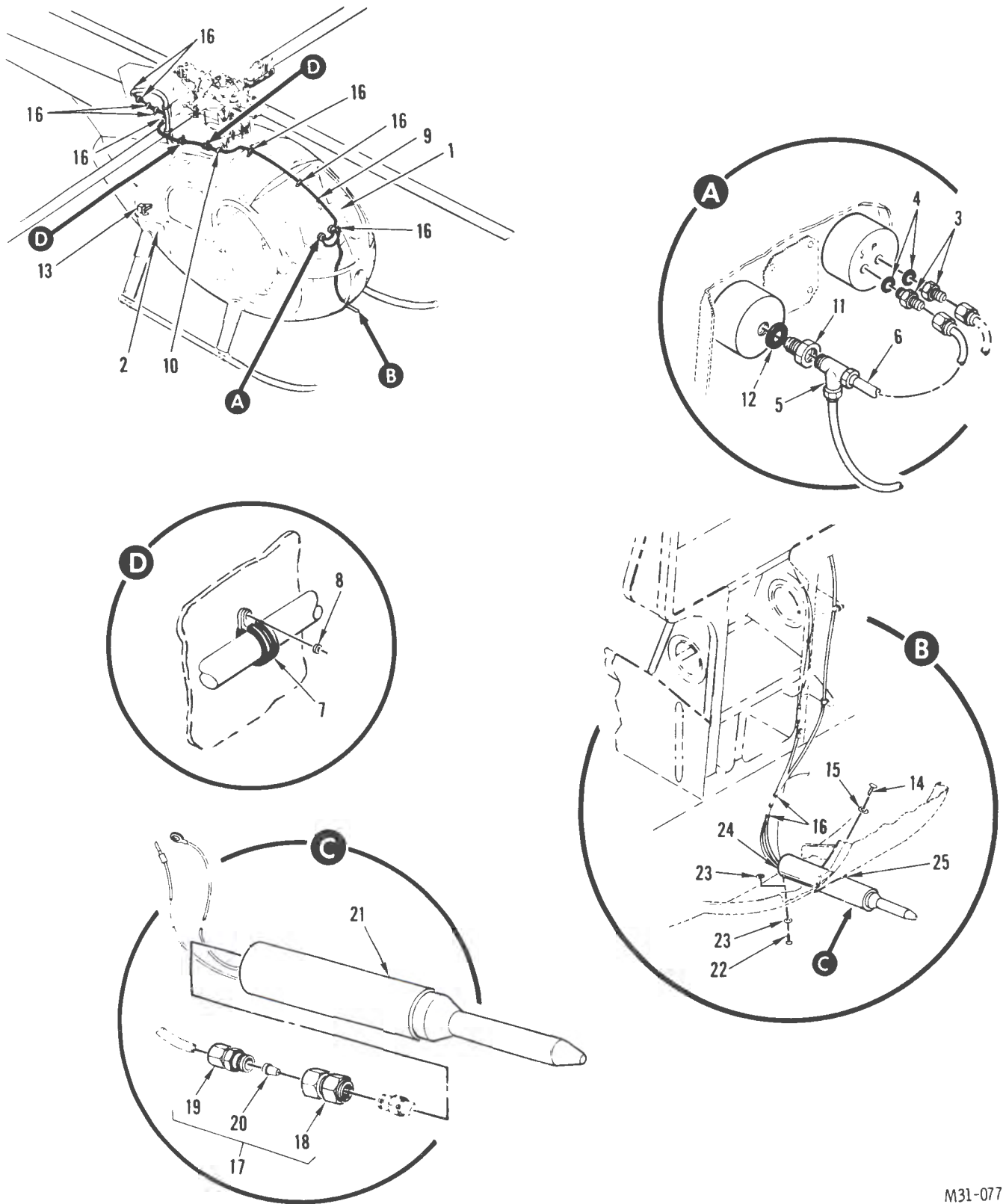
FIGURE 44. INSTRUMENT INSTALLATION, ELECTRICAL (SERIES I AND II) (SHEET 1 of 2)
