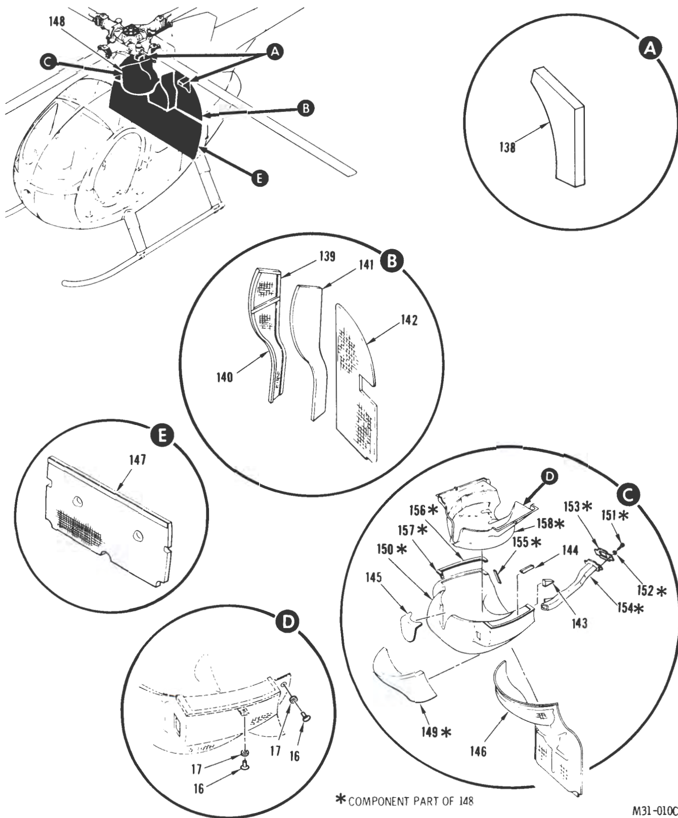
FIGURE 2. FUSELAGE STRUCTURE, COMPLETE (SHEET 6 OF 9)
