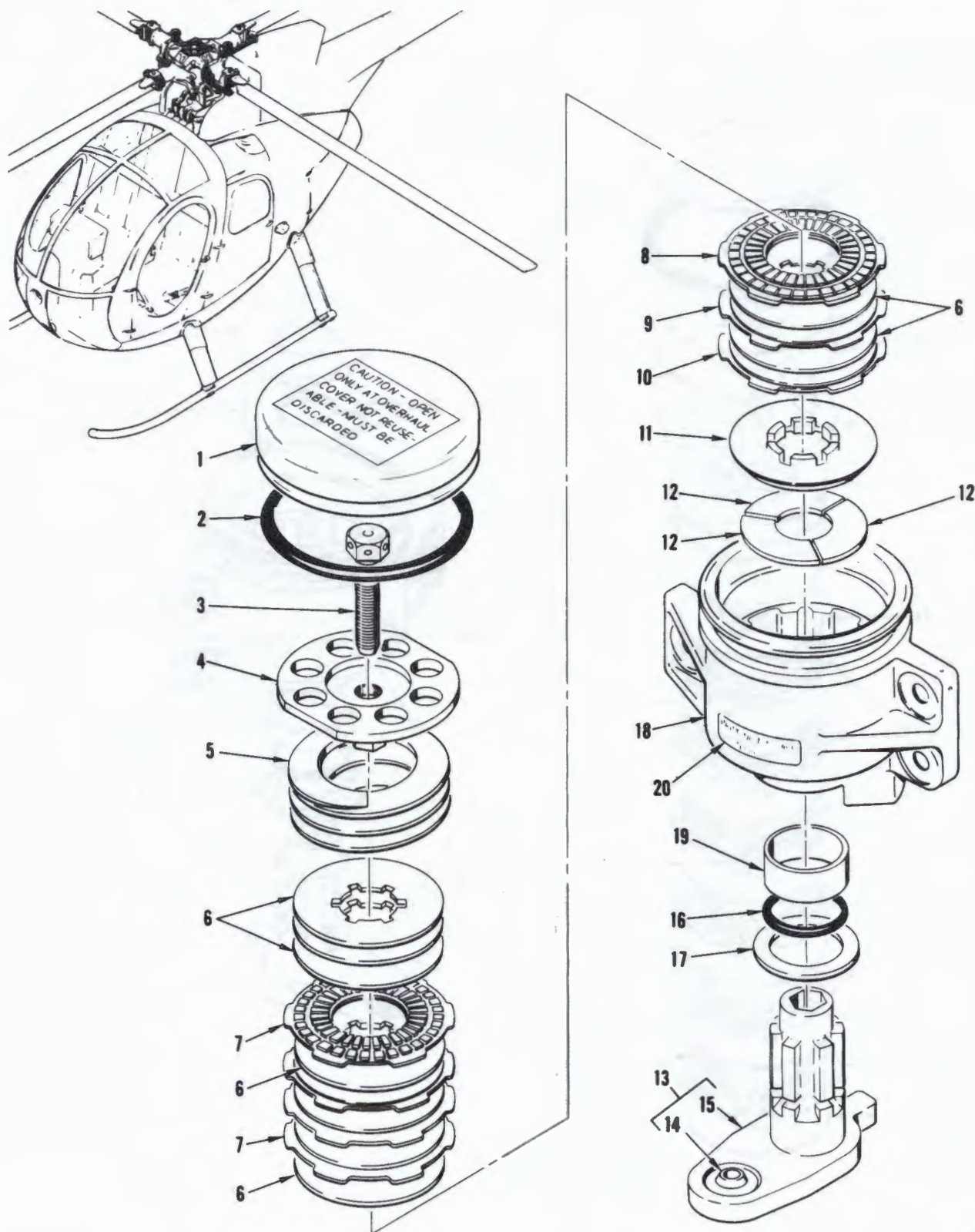
FIGURE 35. DAMPER ASSEMBLY, MAIN ROTOR BLADE (SHEET 1 OF 2)
