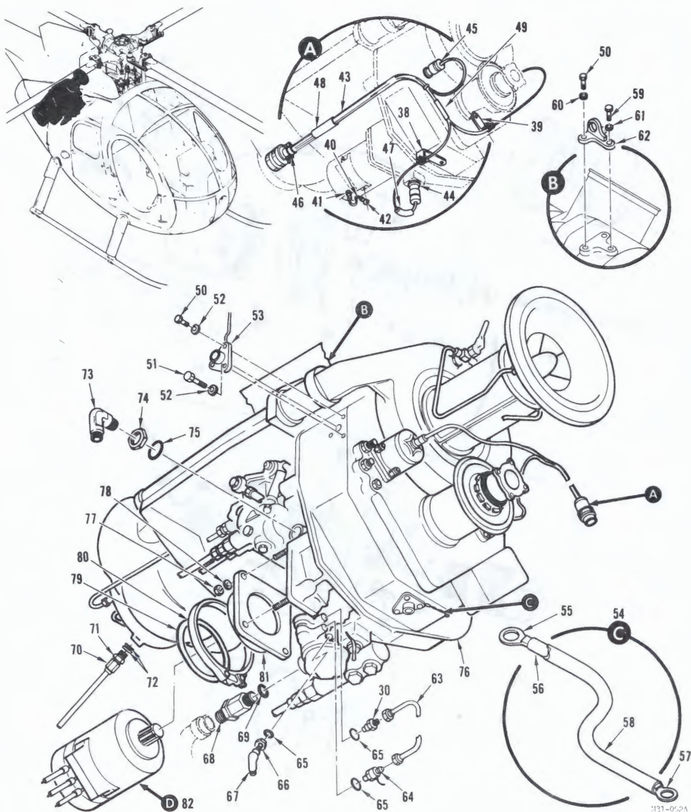
FIGURE 23. ENGINE BUILD-UP UNIT (SHEET 2 OF 3)
