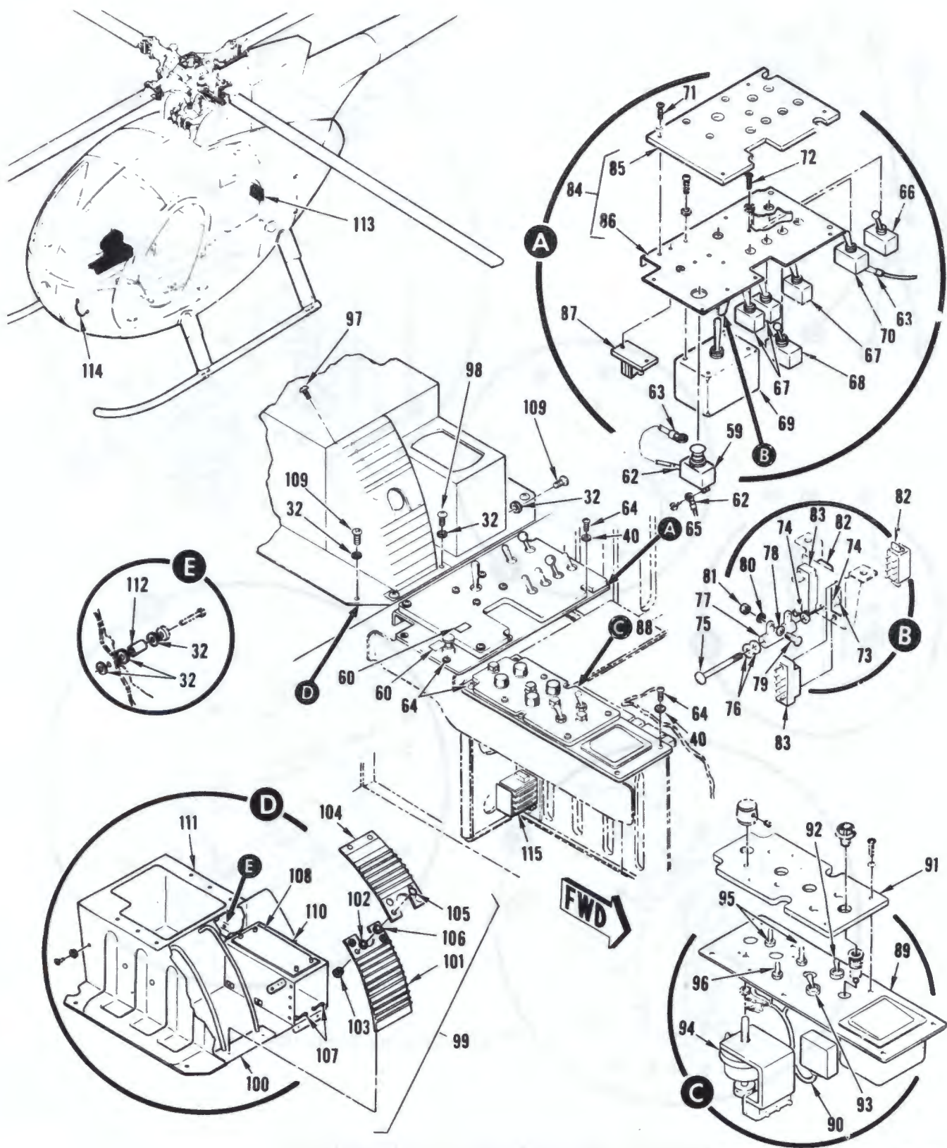
FIGURE 50. ELECTRICAL INSTALLATION (CONSOLE AND WARNING INDICATORS) (SHEET 2 OF 2)
