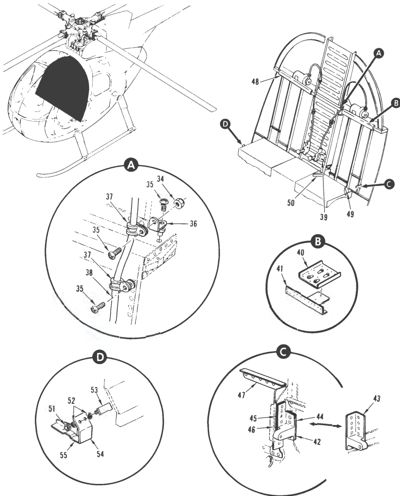
FIGURE 17. ARMOR INSTALLATION, SEATS (SHEET 2 OF 2)
