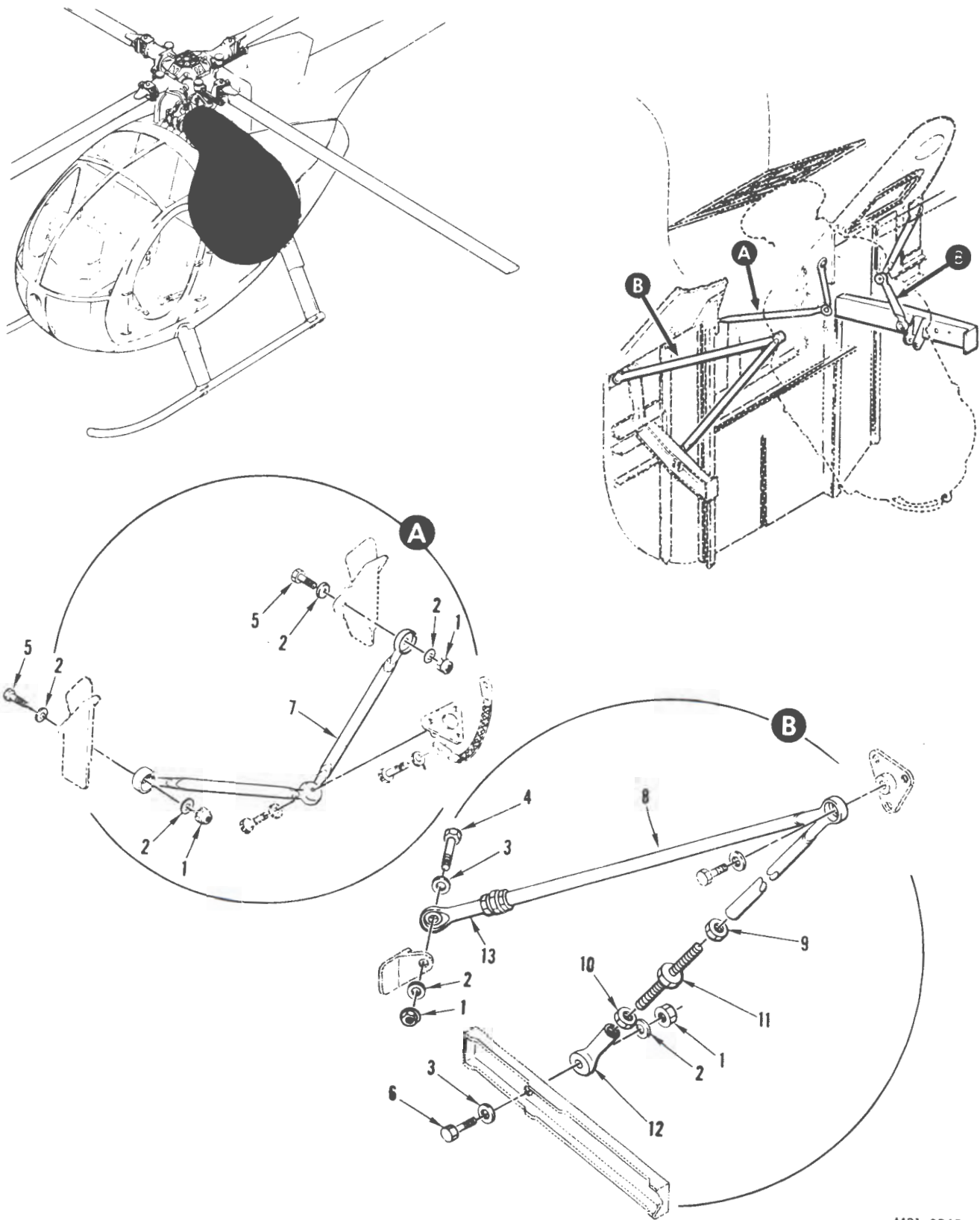
FIGURE 25. ENGINE MOUNT INSTALLATION, POWER PLANT
