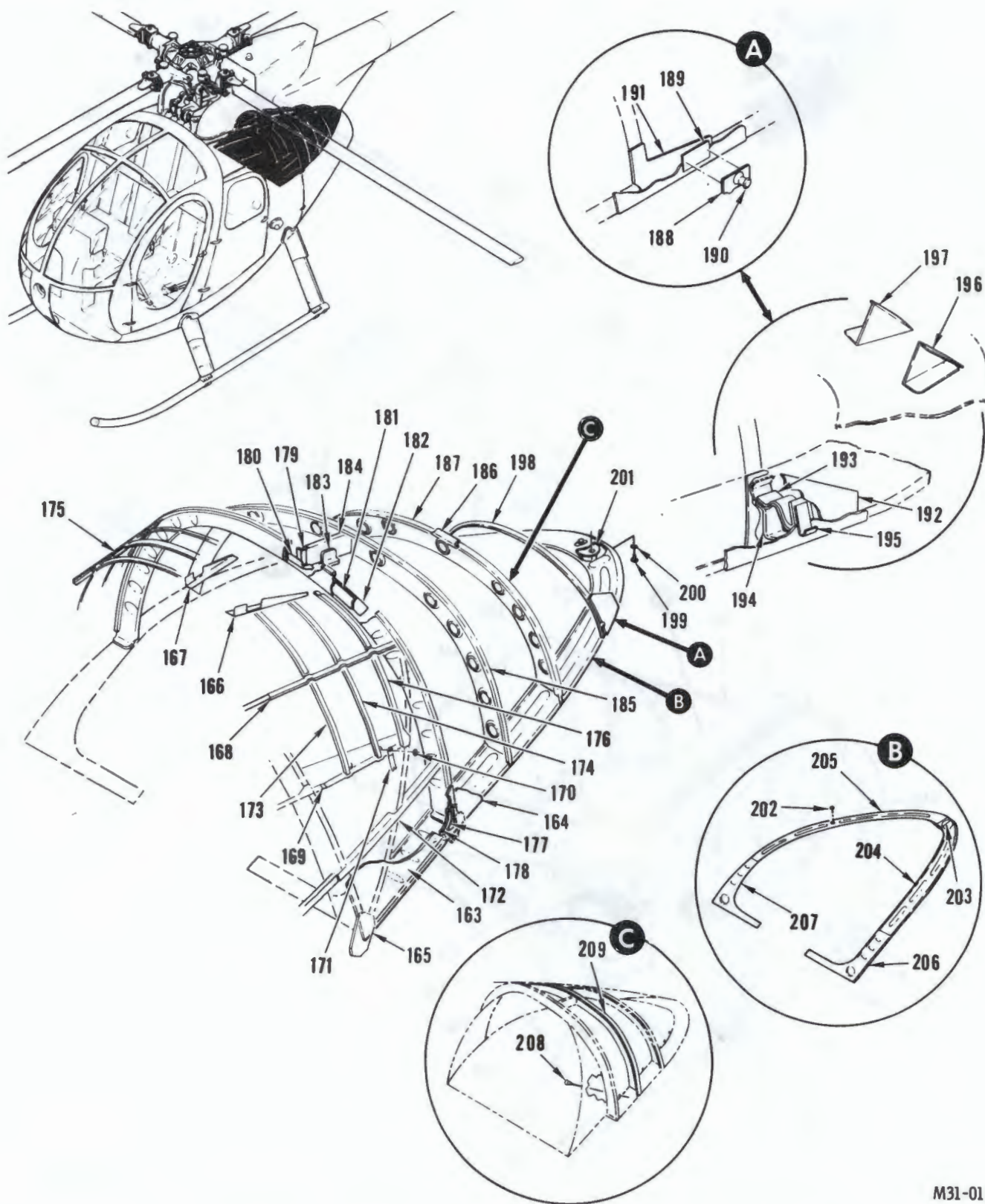
FIGURE 4. AFT SECTION INSTALLATION, FUSELAGE STRUCTURE (SHEET 6 OF 8)
