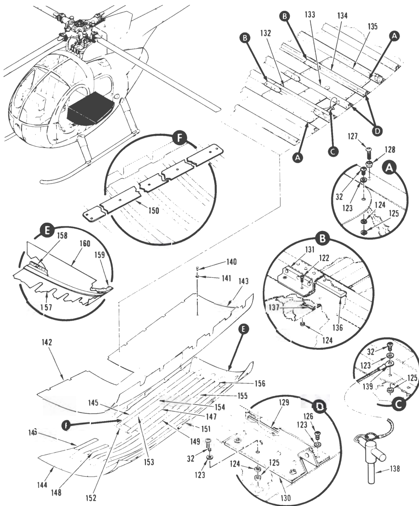
FIGURE 6. LOWER SECTION INSTALLATION, FUSELAGE STRUCTURE (SHEET 4 OF 5)
