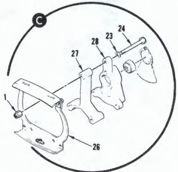
FIGURE 33. HUB ASSEMBLY, MAIN ROTOR (SHEET 1 OF 2)
