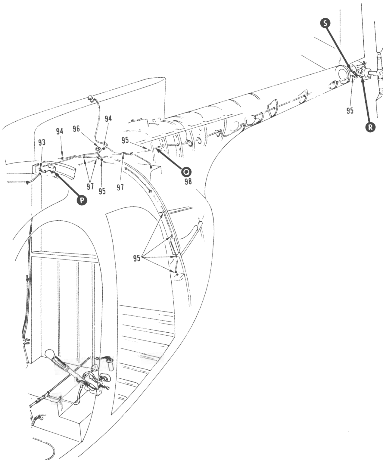
FIGURE 55. WIRE INSTALLATION, SERIES I AND II (SHEET 2 OF 9)
