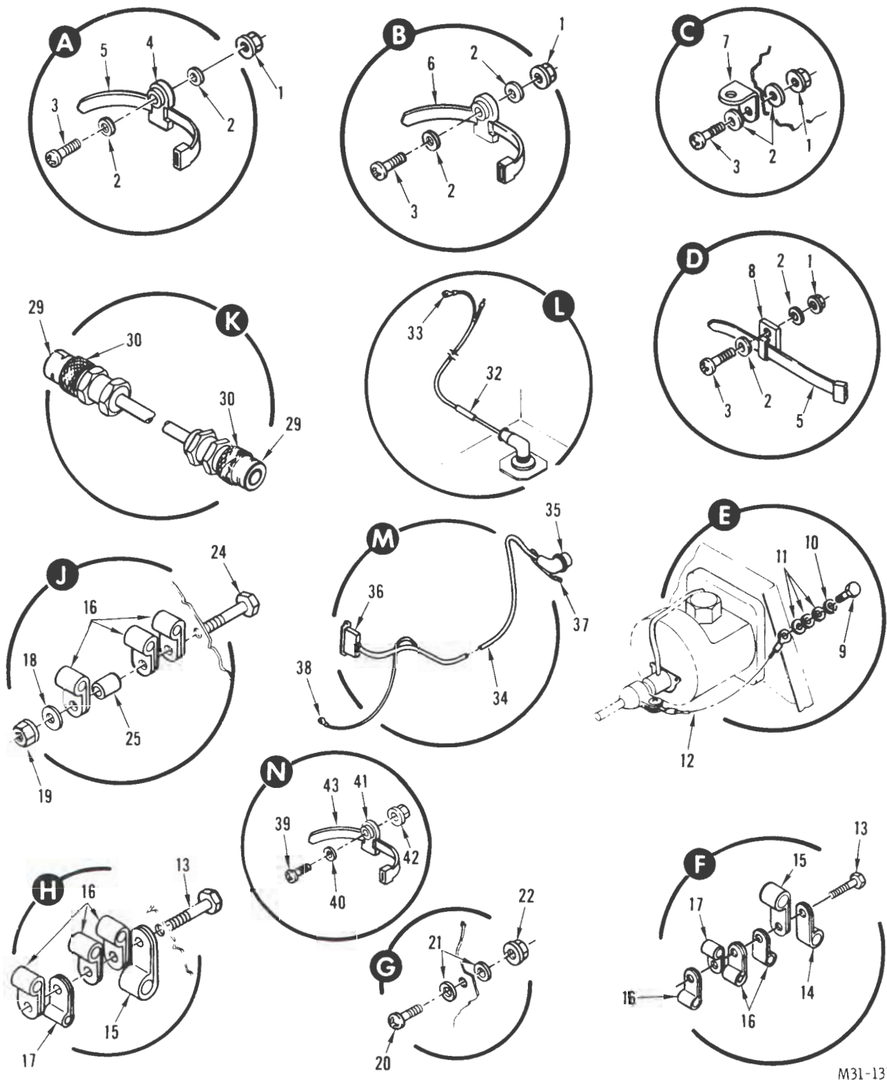
FIGURE 56. WIRE INSTALLATION, SERIES III (SHEET 6 OF 15)
