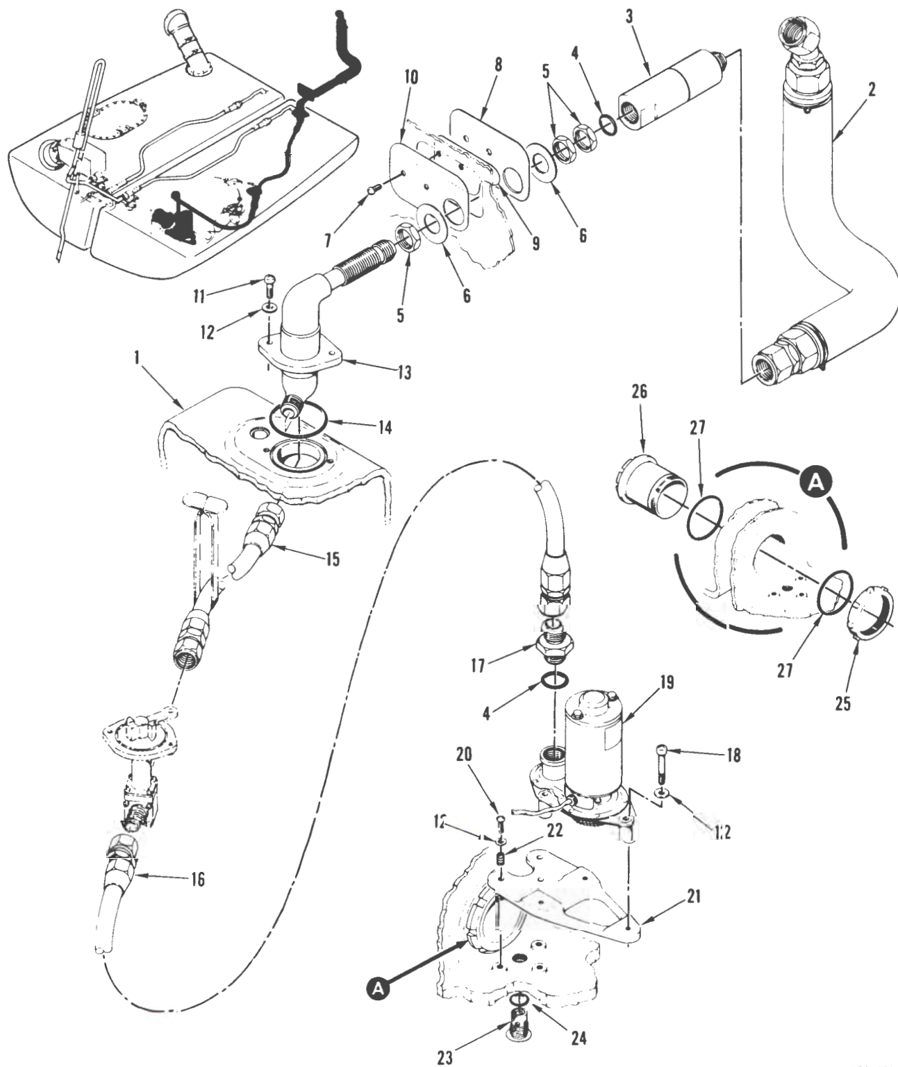
FIGURE 58. CRASHWORTHY FUEL SYSTEM – FUEL SUPPLY
