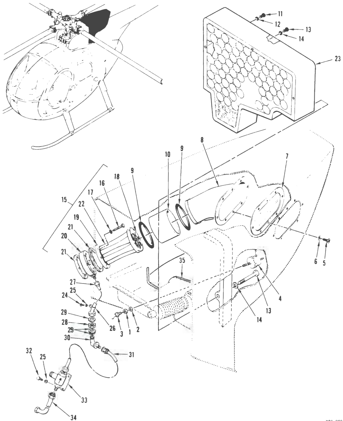
FIGURE 27. FILTER INSTALLATION, ENGINE AIR
