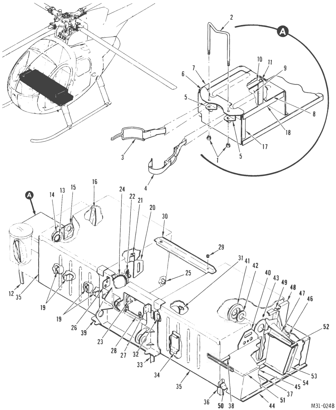
FIGURE 7. SEAT STRUCTURE INSTALLATION
