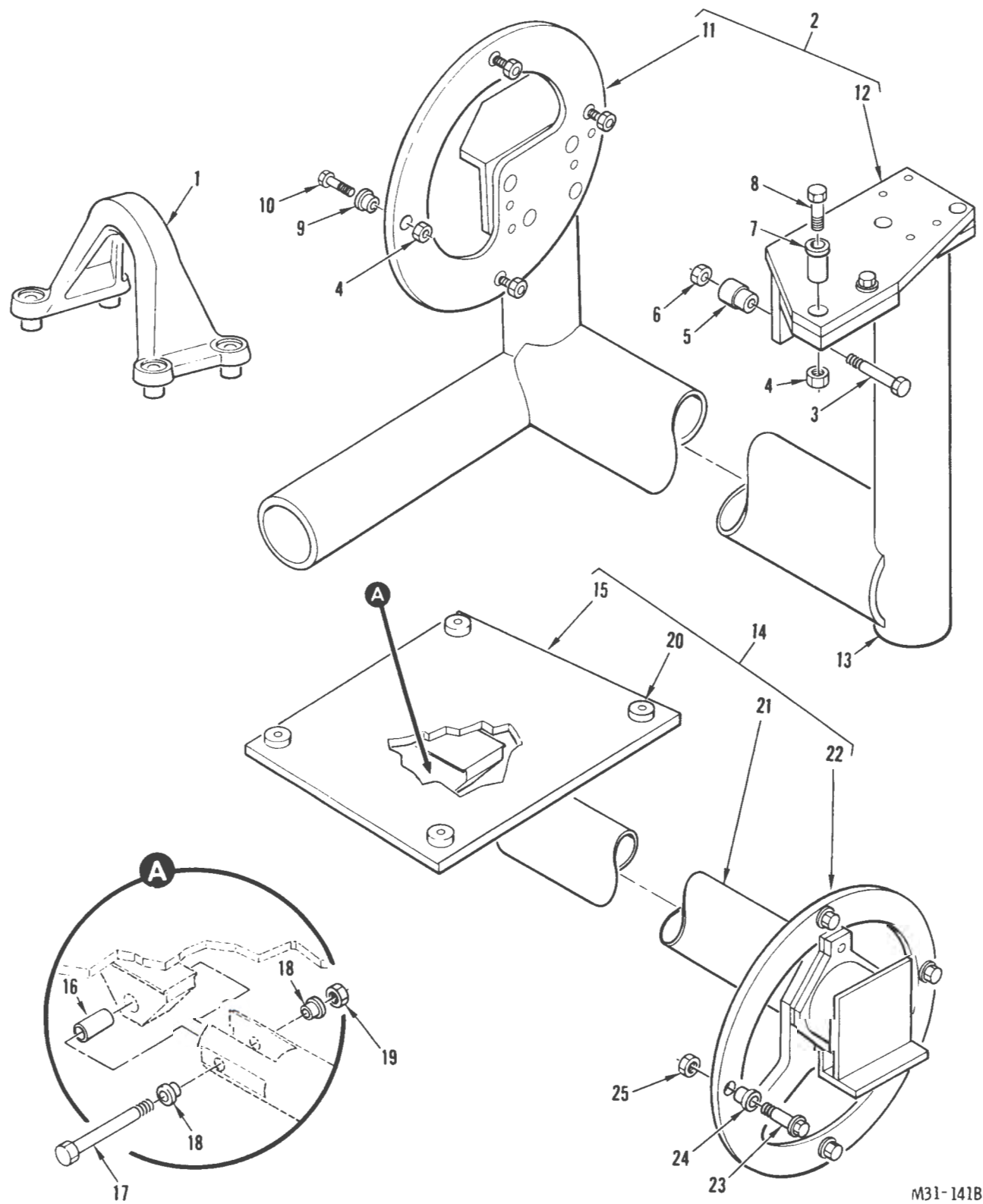
FIGURE A1. AIRFRAME TOOLS
