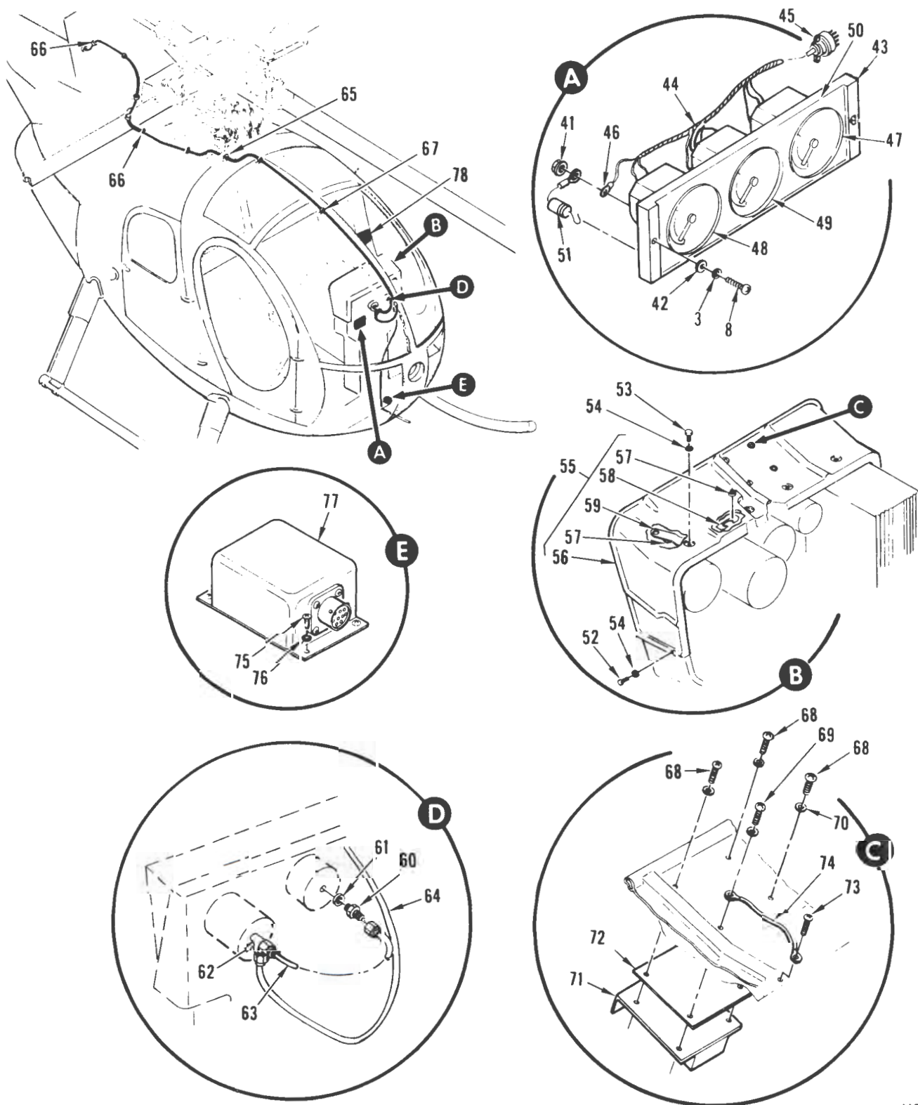
FIGURE 45. ELECTRICAL INSTALLATION (INSTRUMENTS, SERIES III) (SHEET 2 OF 2)
