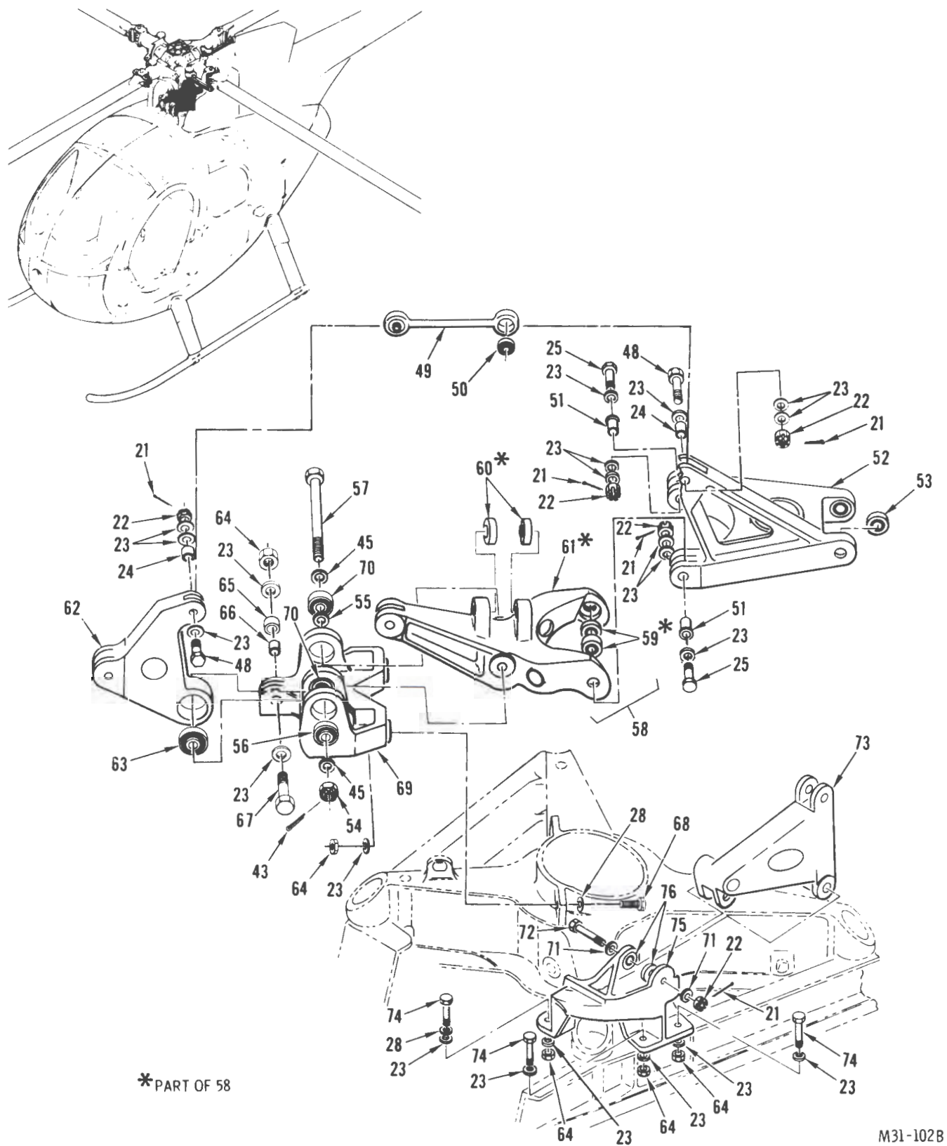
FIGURE 64. MIXER, SWASHPLATE AND ROTOR CONTROLS INSTALLATION (SHEET 2 OF 2)
