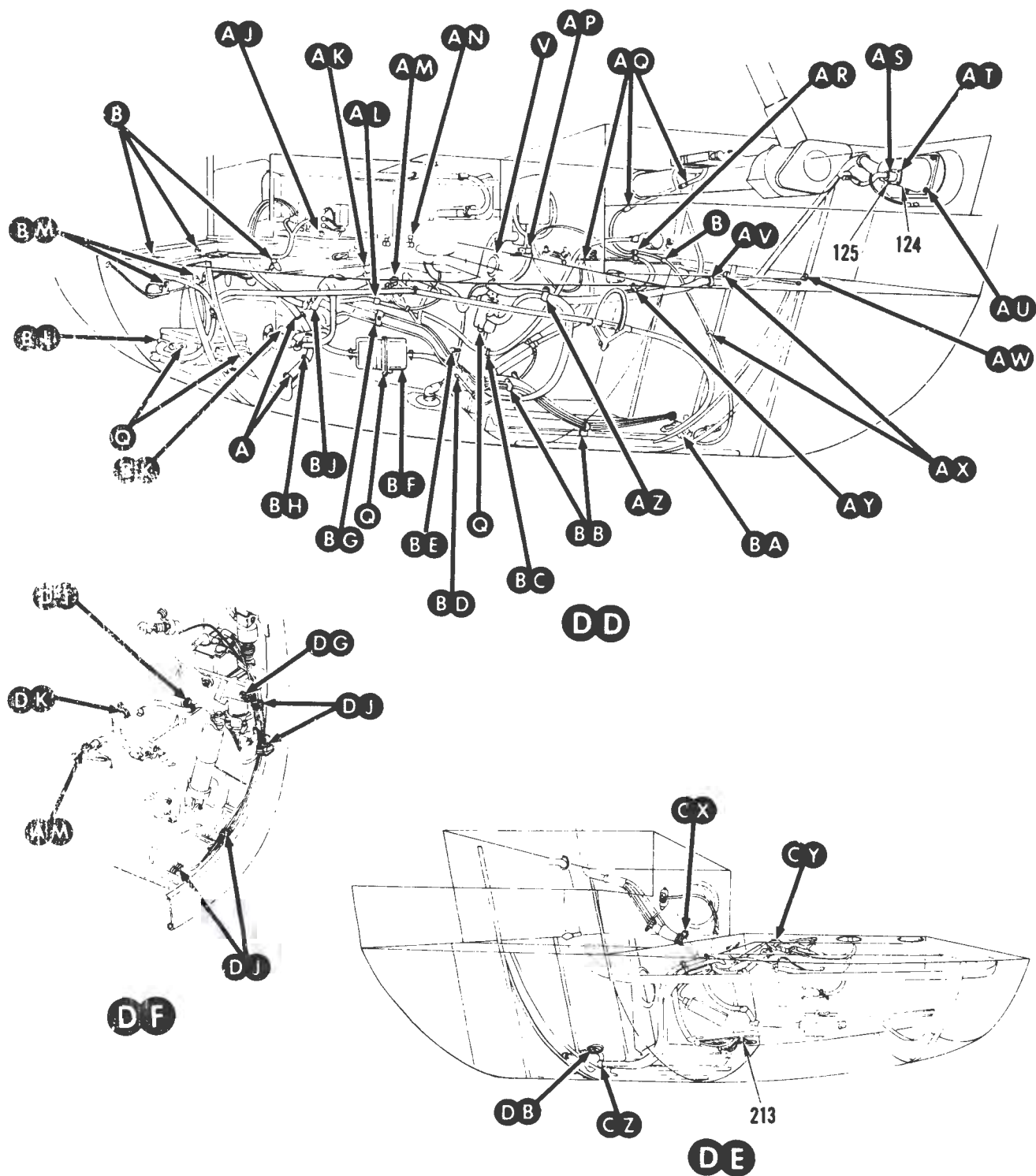
FIGURE 56. WIRE INSTALLATION, SERIES III (SHEET 5 OF 15)
