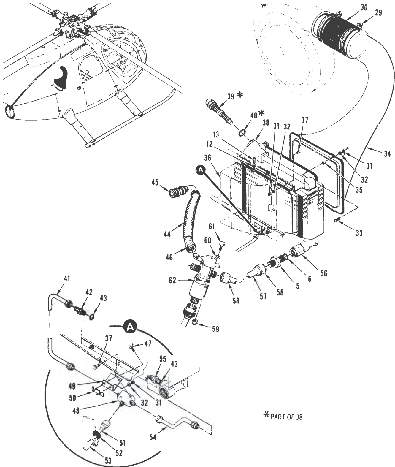
FIGURE 21. ENGINE OIL SYSTEM INSTALLATION (SHEET 2 OF 2)
