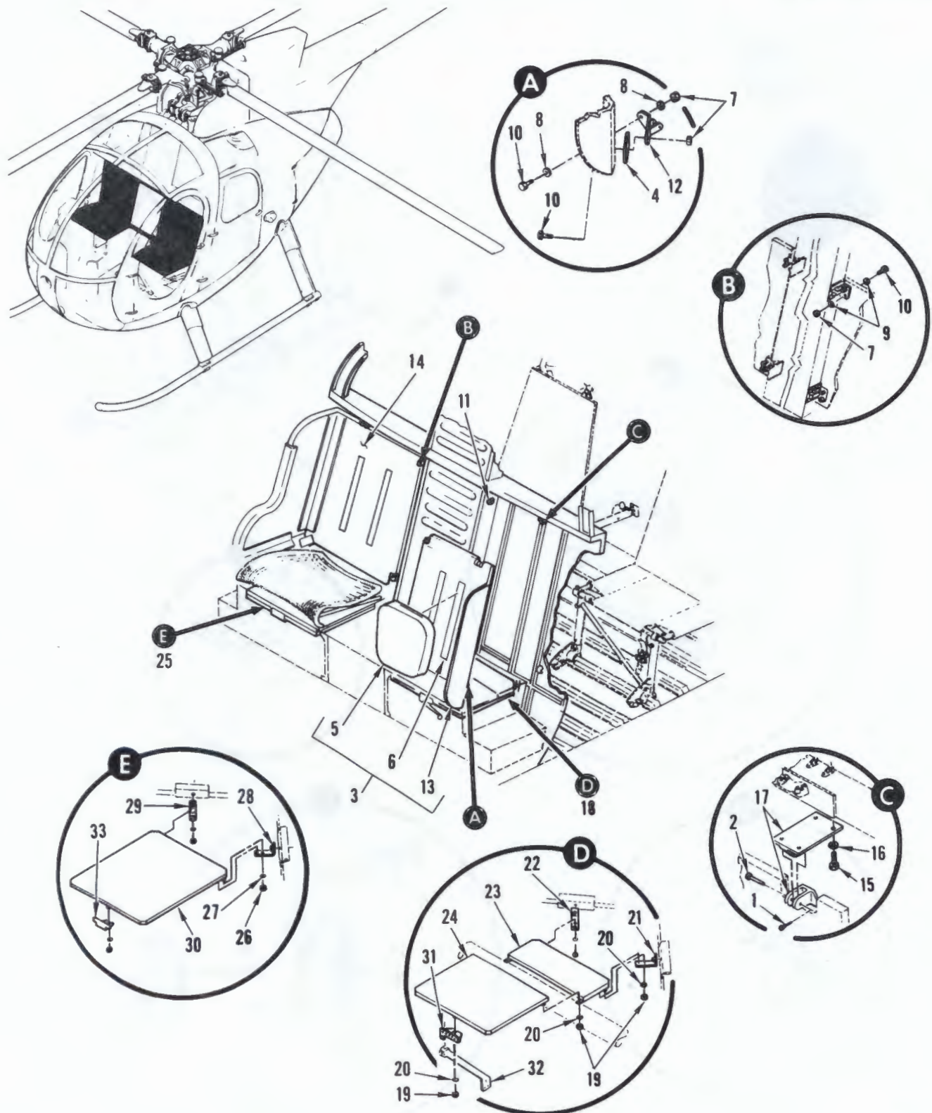
FIGURE 17. ARMOR INSTALLATION, SEATS (SHEET 1 OF 2)
