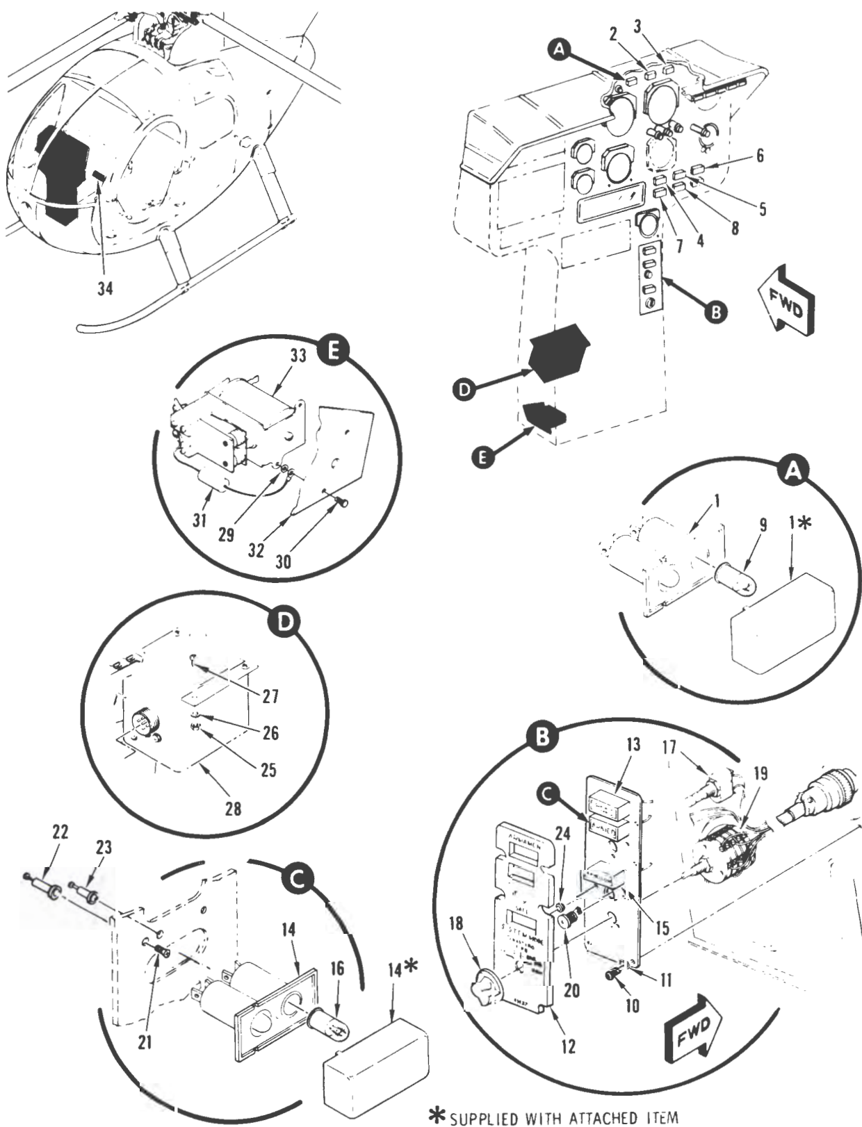
FIGURE 52. PANEL ASSEMBLY, COCKPIT INDICATOR (ARMAMENT ELECTRICAL CONTROLS) (SHEET 1 OF 2)
