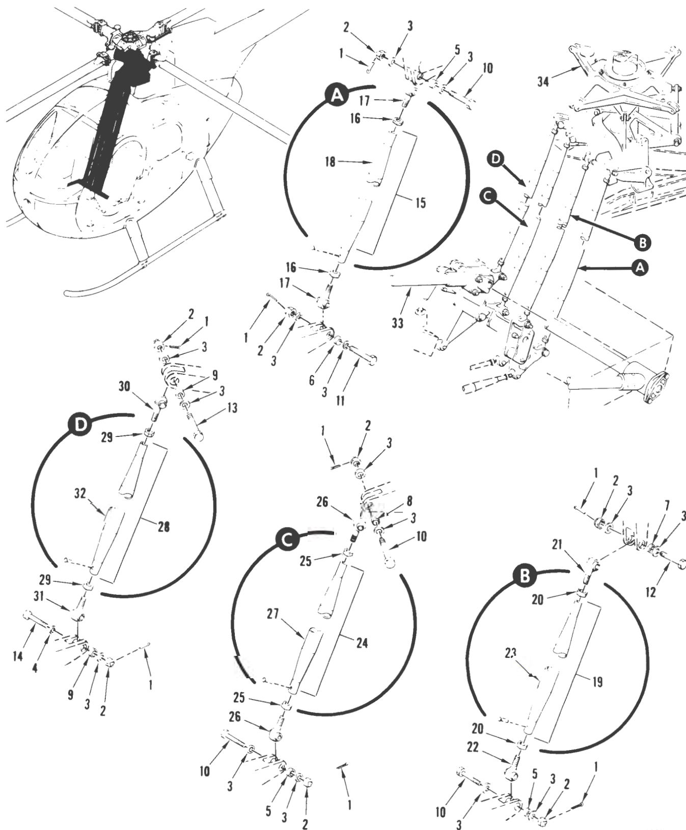
FIGURE 63. FLIGHT CONTROLS INSTALLATION (FORWARD) (SHEET 1 OF 2)
