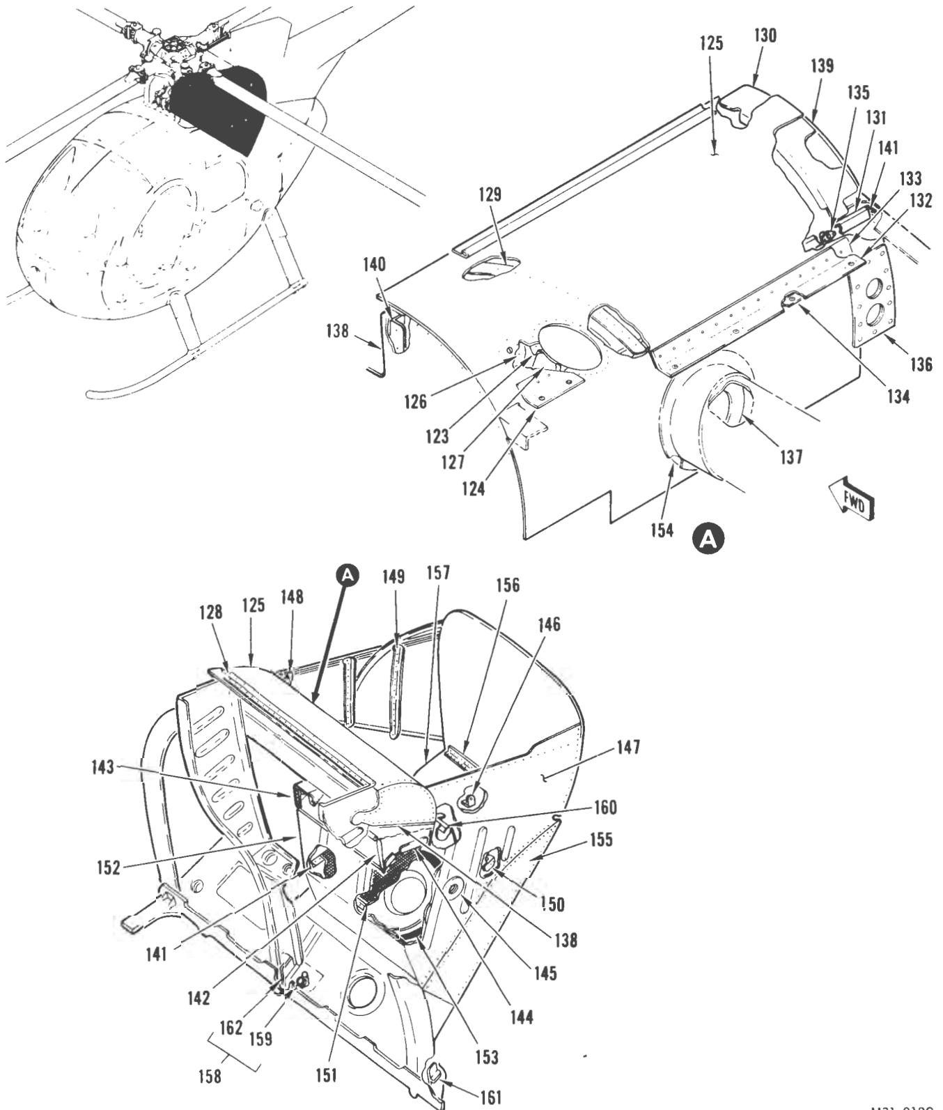
FIGURE 4. AFT SECTION INSTALLATION, FUSELAGE STRUCTURE (SHEET 5 OF 8)
