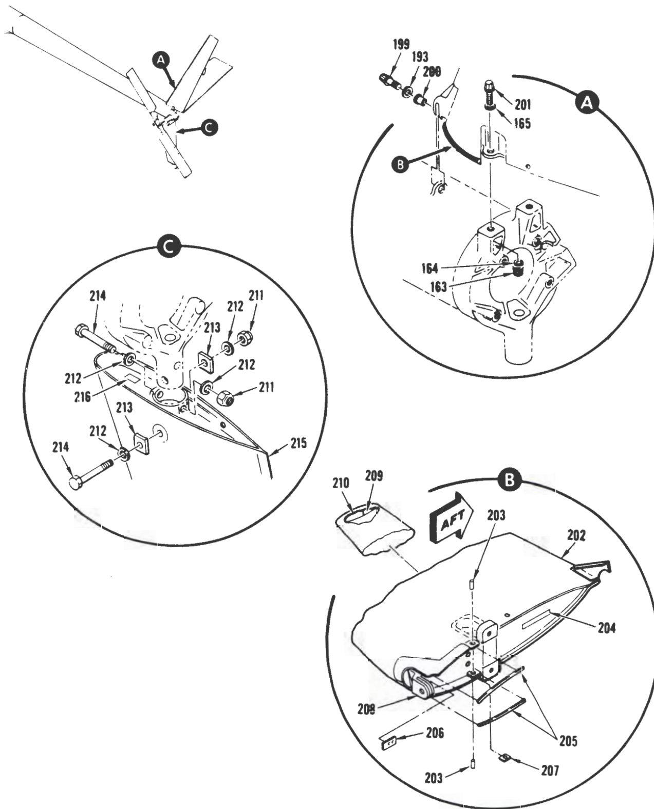
FIGURE 2. FUSELAGE STRUCTURE, COMPLETE (SHEET 9 OF 9)
