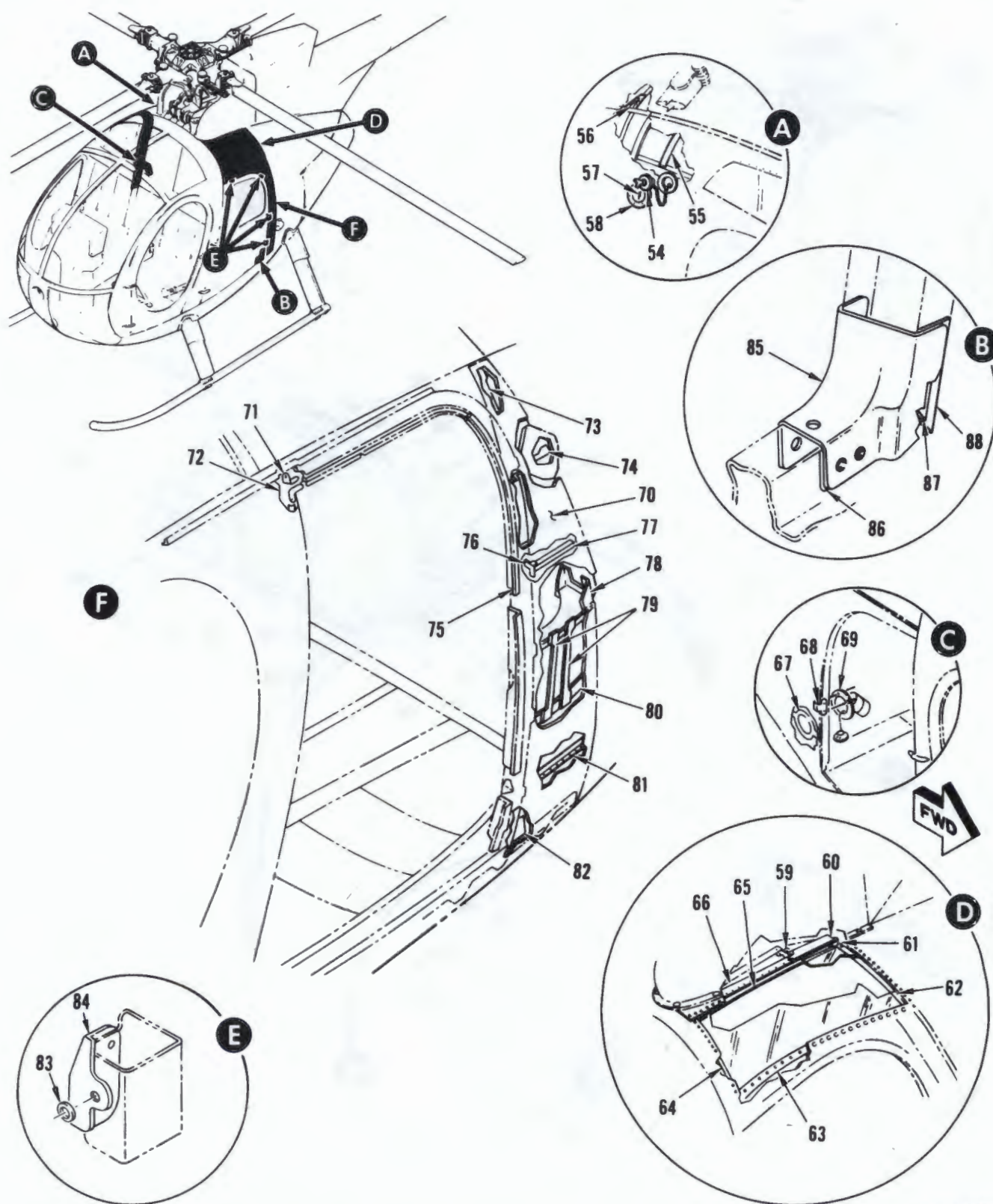
FIGURE 4. AFT SECTION INSTALLATION, FUSELAGE STRUCTURE (SHEET 3 OF 8)
