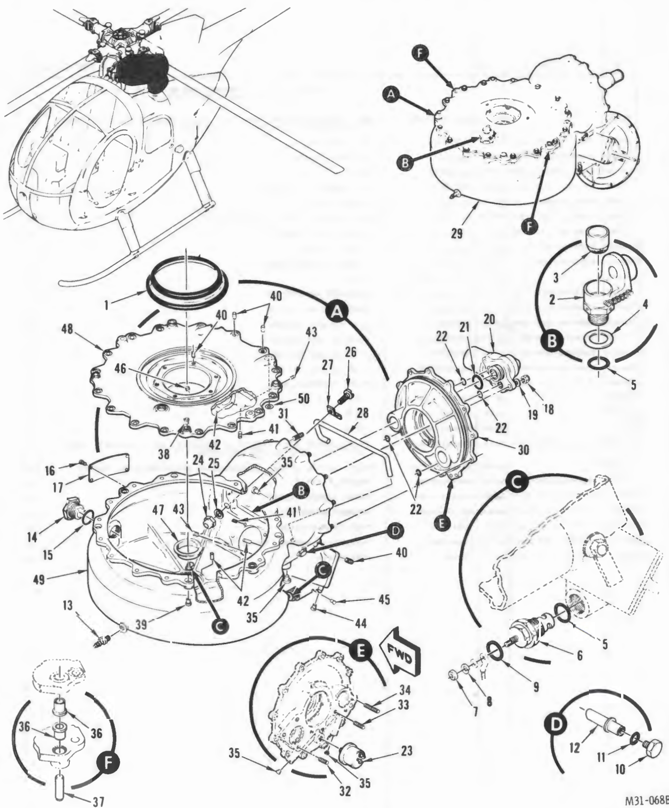
FIGURE 39. TRANSMISSION ASSEMBLY, MAIN (EXTERIOR COMPONENTS AND MAIN HOUSING)
