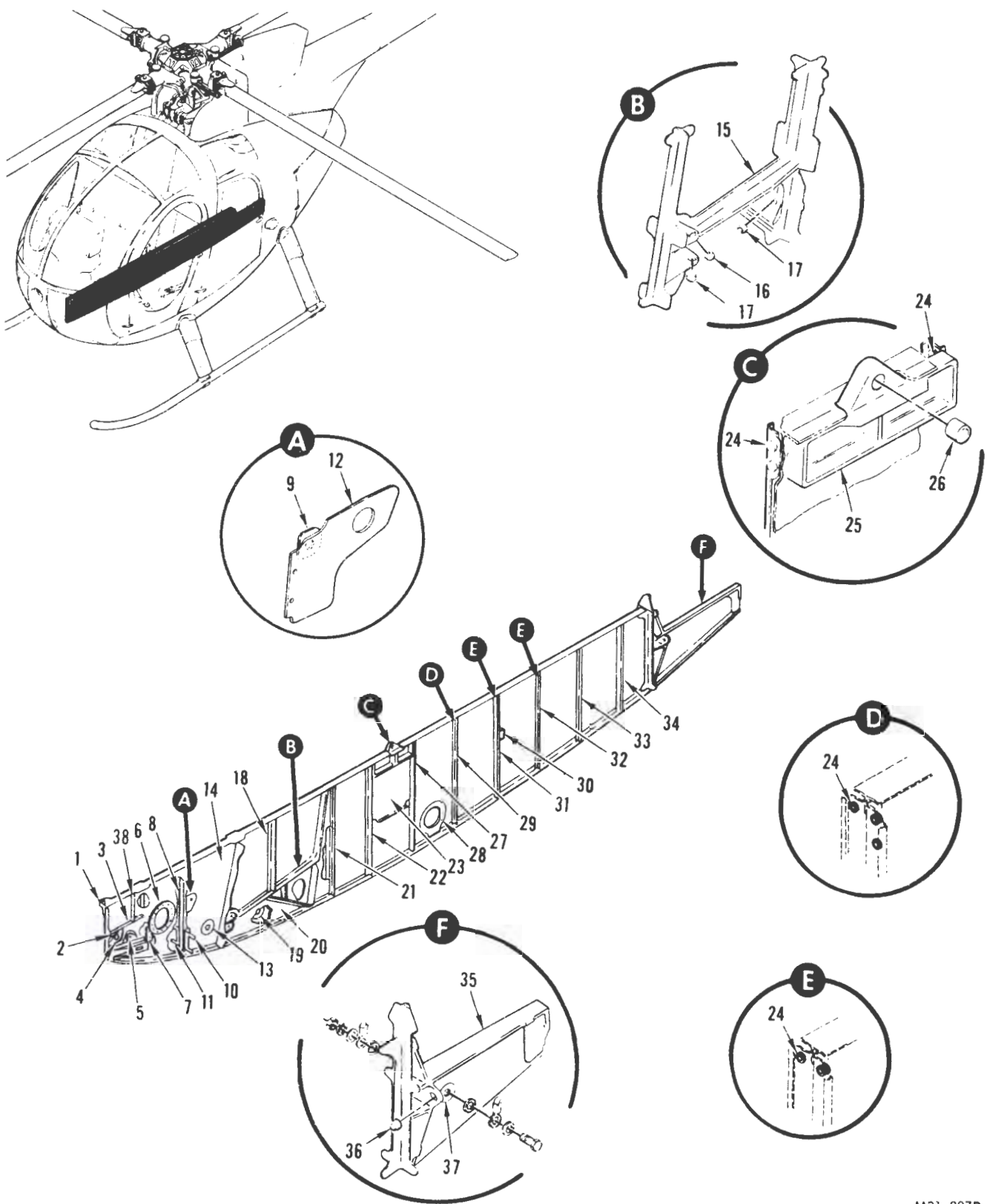
FIGURE 8. CENTER BEAM ASSEMBLY
