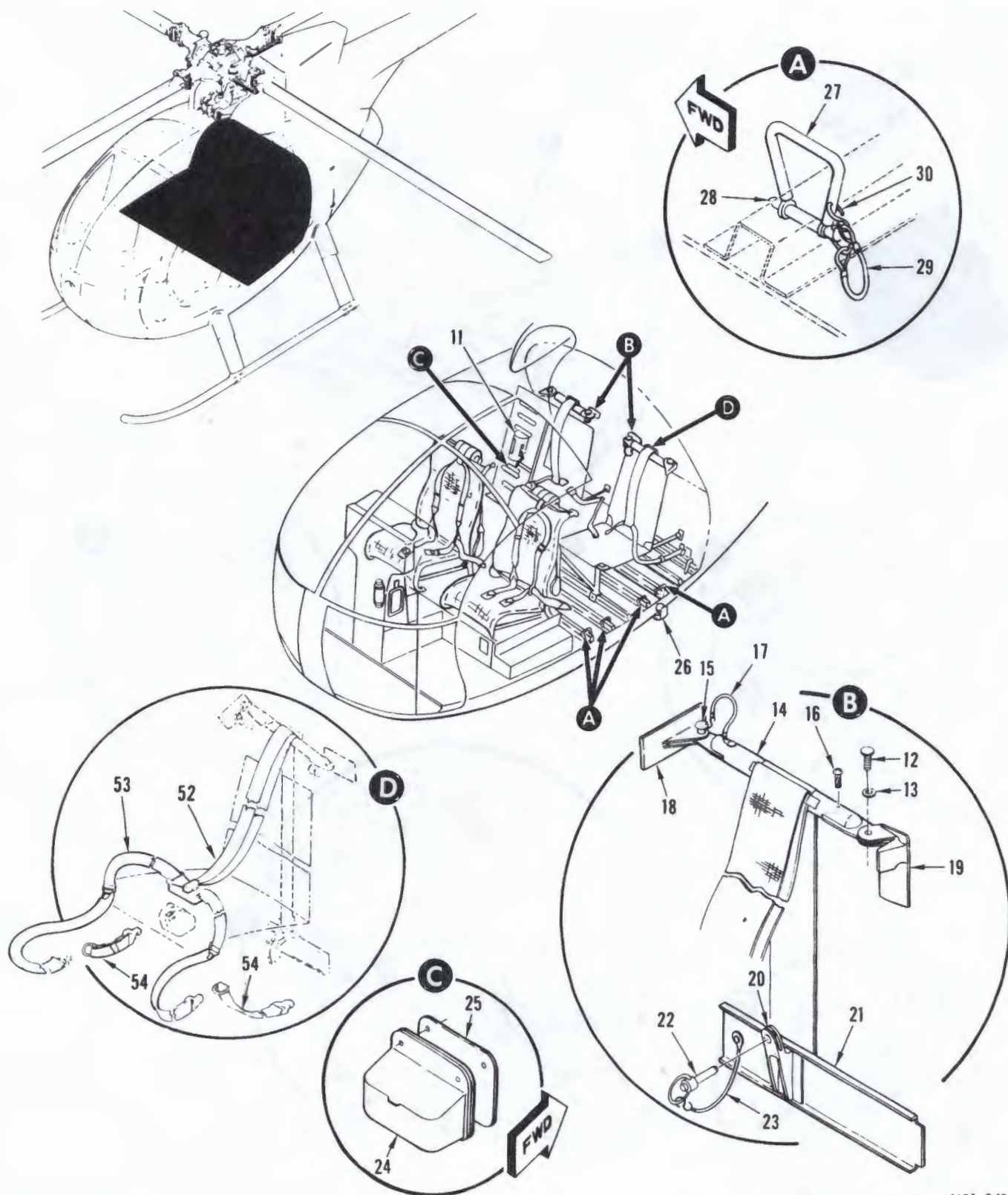
FIGURE 16. EQUIPMENT INSTALLATION (SHEET 1 OF 2)
