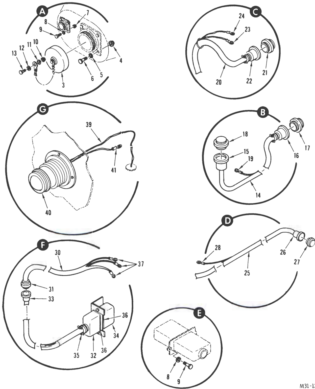
FIGURE 55. WIRE INSTALLATION, SERIES I AND II (SHEET 5 OF 9)
