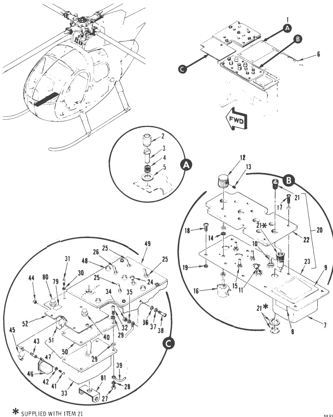
FIGURE 49. CONSOLE ASSEMBLY, CONTROL, ELECTRICAL (SHEET 1 of 2)
