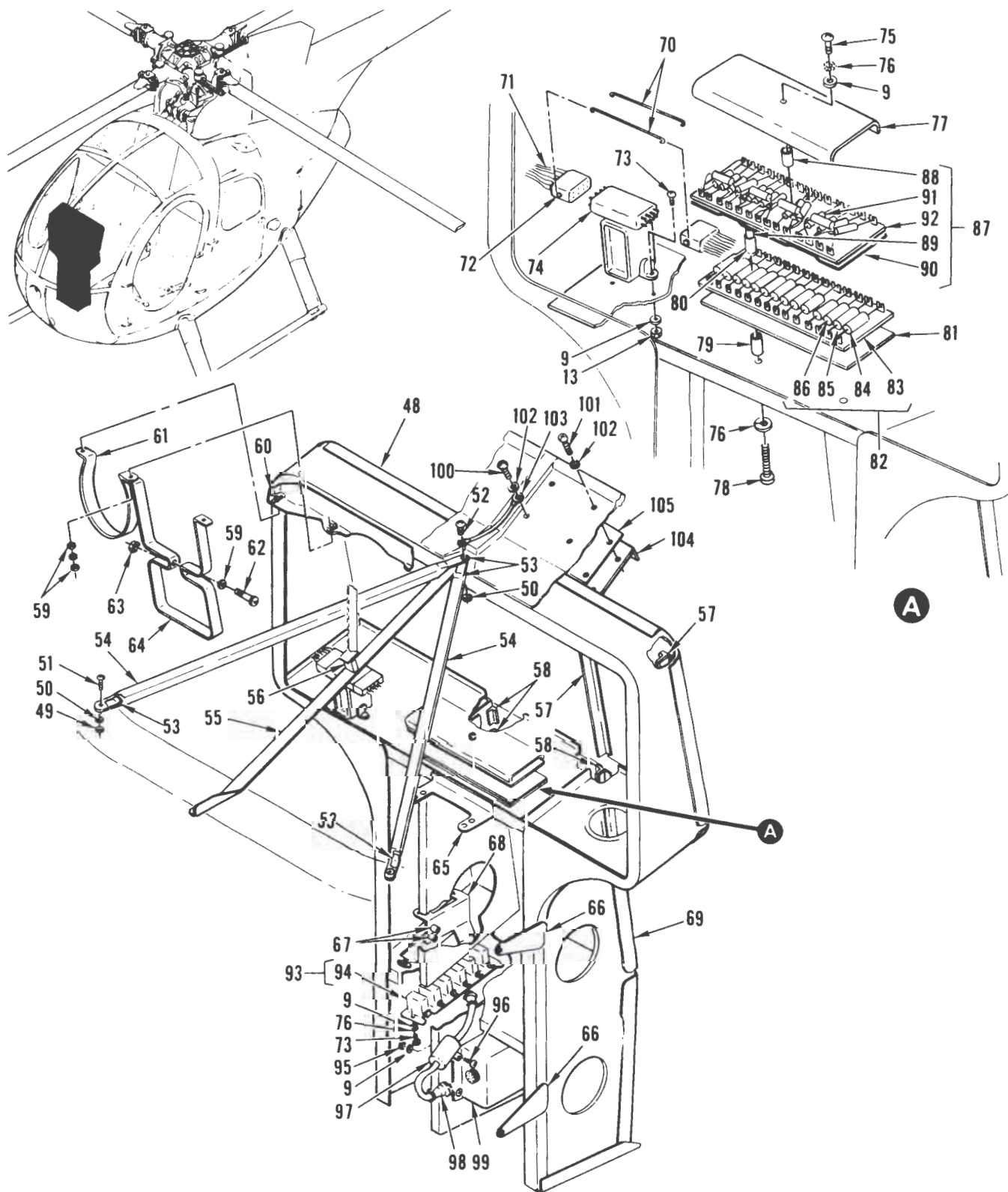
FIGURE 47. PANEL ASSEMBLY, COCKPIT INDICATOR (SHEET 2 OF 2)
