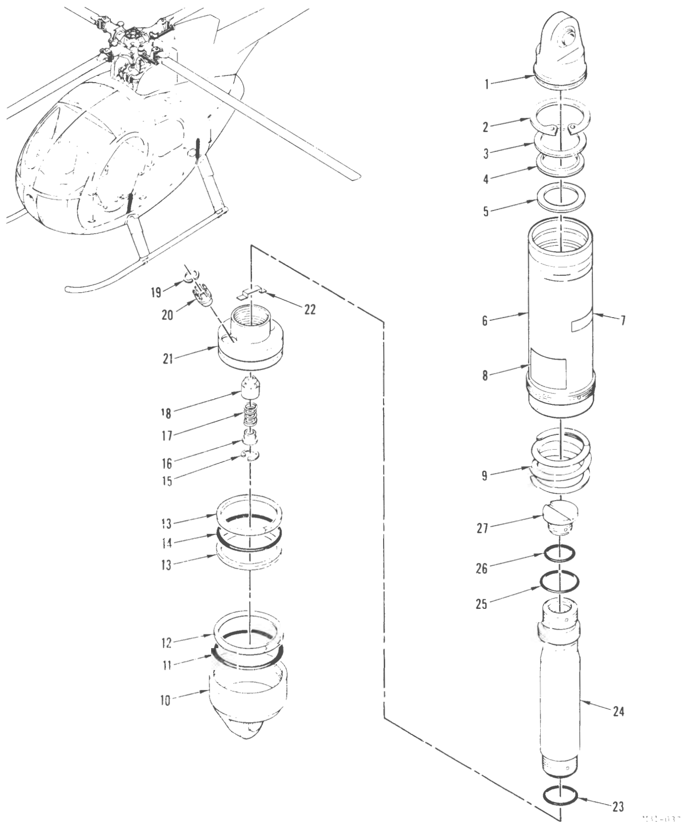
FIGURE 19. DAMPER ASSEMBLY, LANDING GEAR
