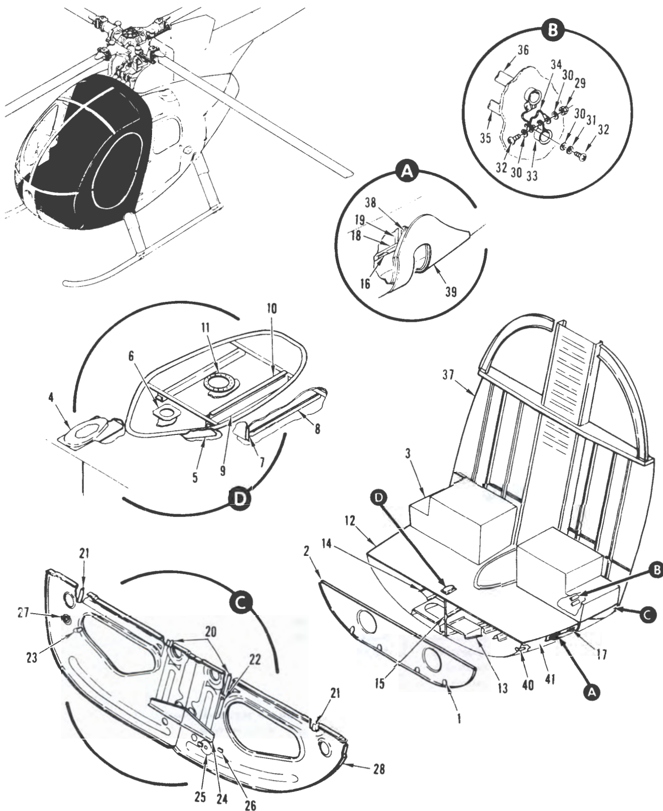
FIGURE 6. LOWER SECTION INSTALLATION, FUSELAGE STRUCTURE (SHEET 1 OF 5)
