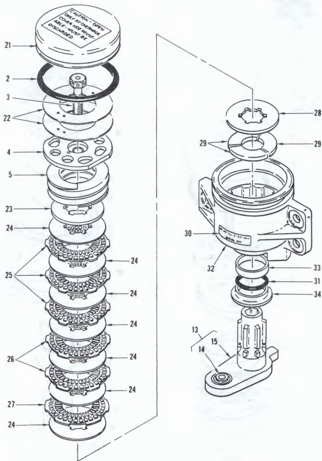
FIGURE 35. DAMPER ASSEMBLY, MAIN ROTOR BLADE (SHEET 2 OF 2)
