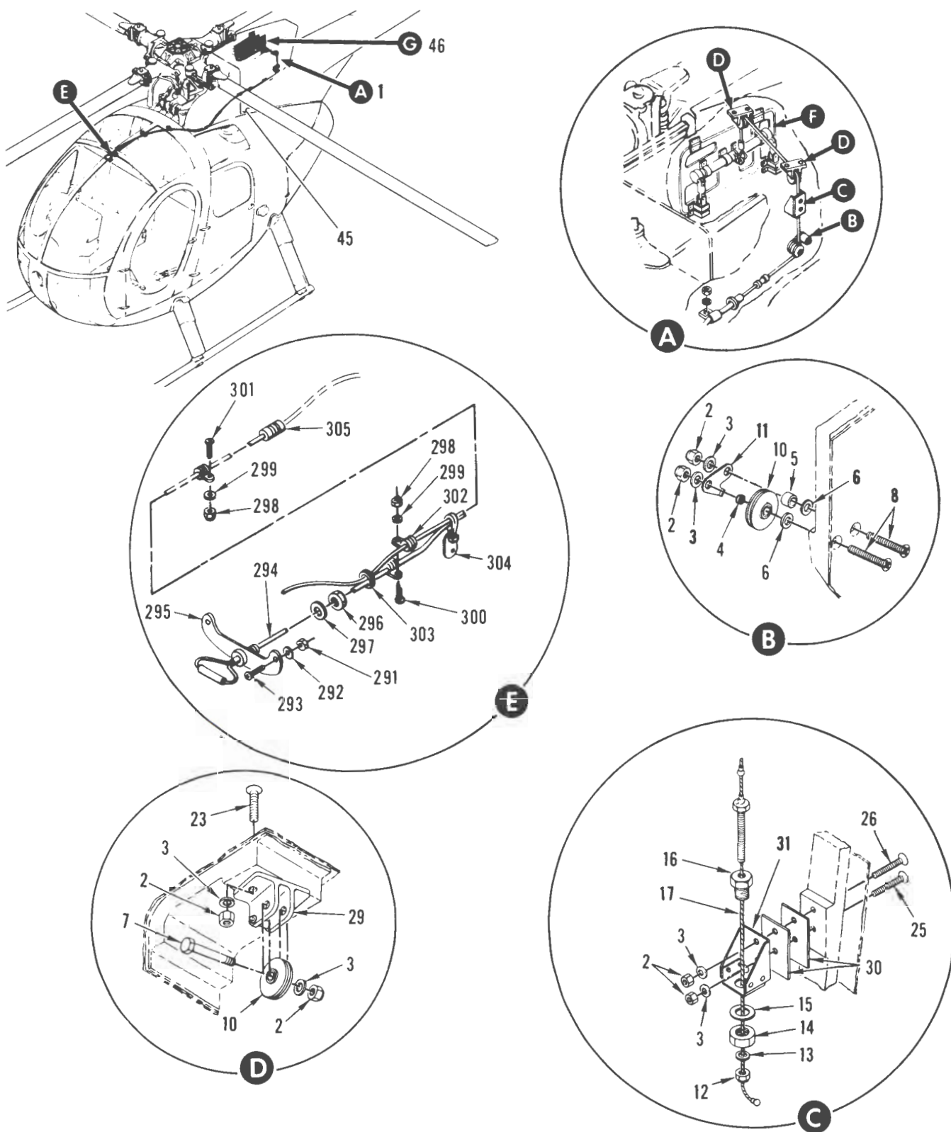
FIGURE 4. AFT SECTION INSTALLATION, FUSELAGE STRUCTURE (SHEET 1 OF 8)
