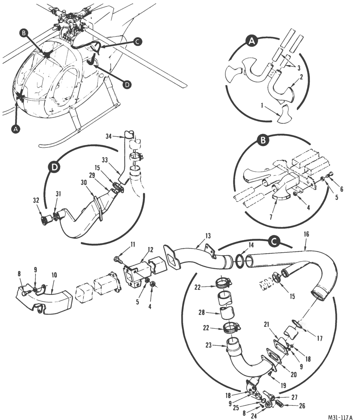
FIGURE 76. HEATING SYSTEM INSTALLATION (CABIN DISTRIBUTION)
