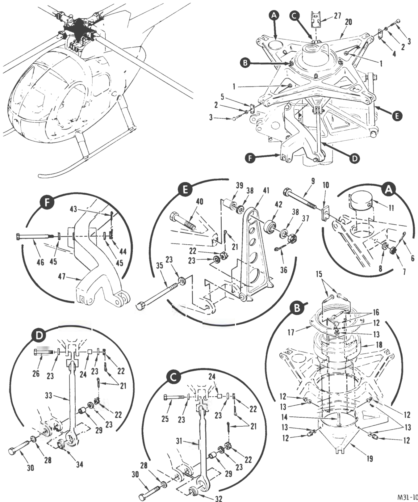
FIGURE 64. MIXER, SWASHPLATE AND ROTOR CONTROLS INSTALLATION (SHEET 1 of 2)
