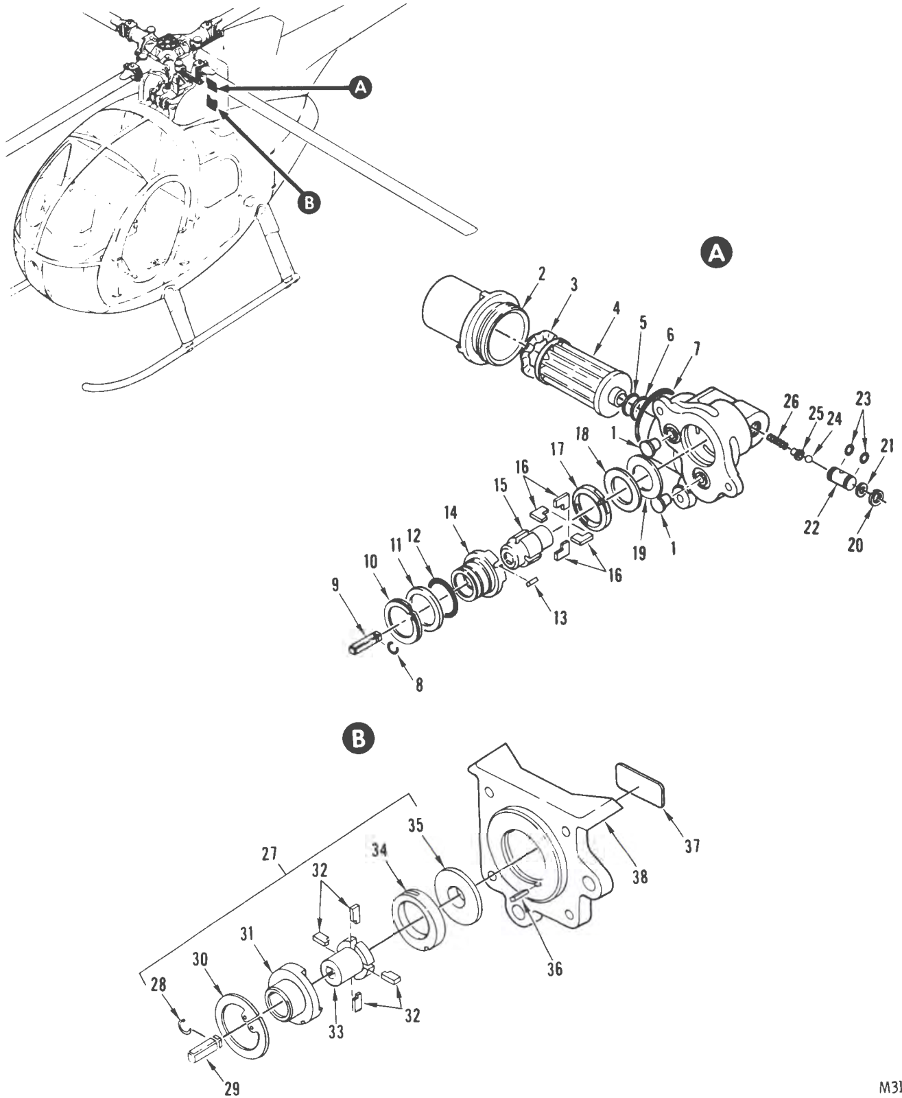
FIGURE 42. PUMP, ROTARY
