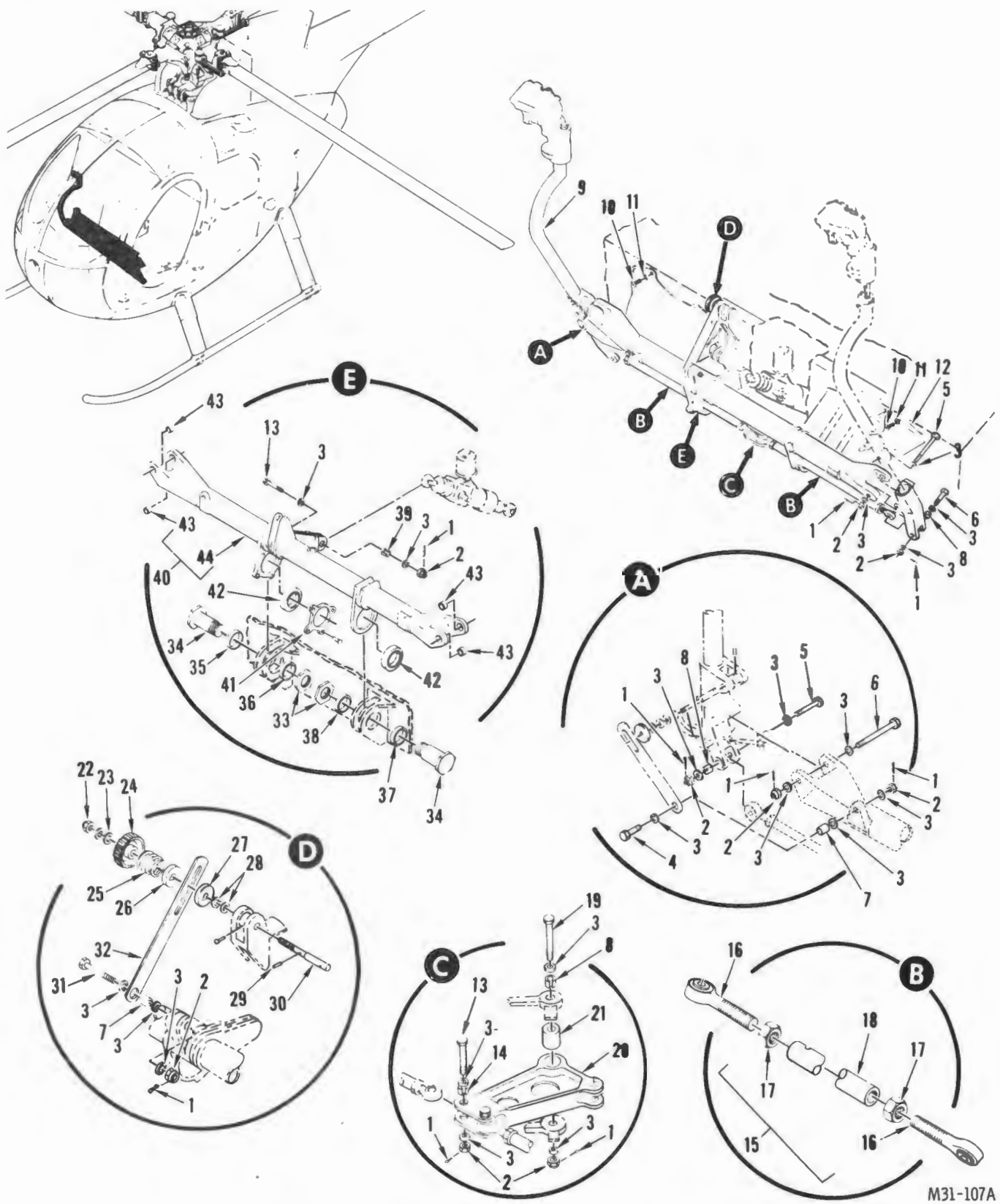
FIGURE 65. FORWARD CYCLIC CONTROL INSTALLATION
