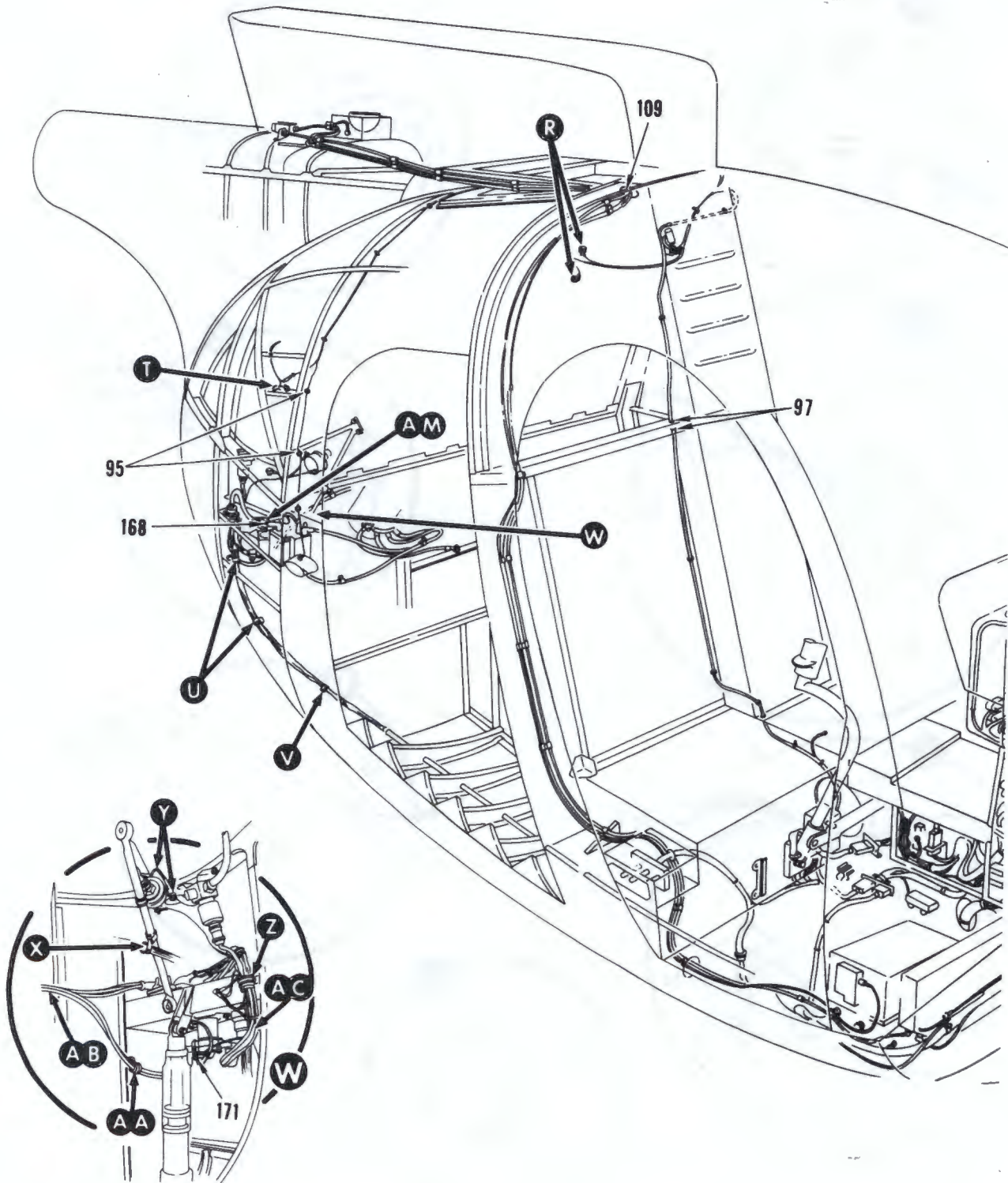
FIGURE 55. WIRE INSTALLATION, SERIES I AND II (SHEET 4 OF 9)
