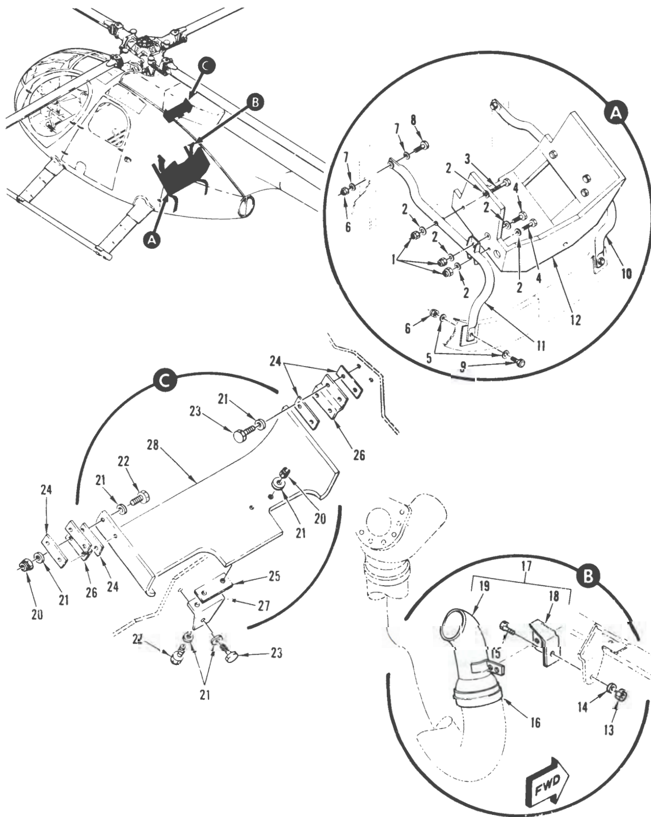
FIGURE 28. ARMOR ASSEMBLY, ENGINE
