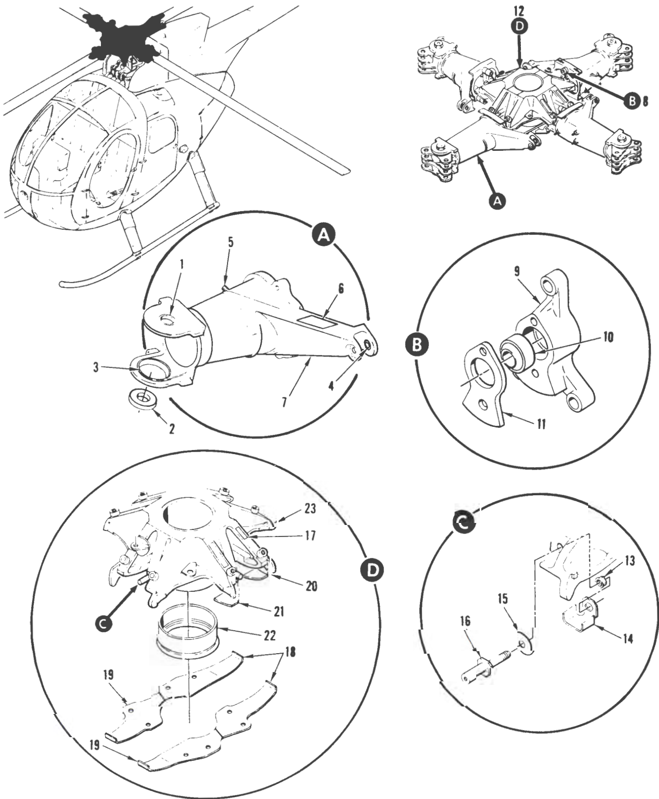
FIGURE 34. HUB SUBASSEMBLIES, MAIN ROTOR
