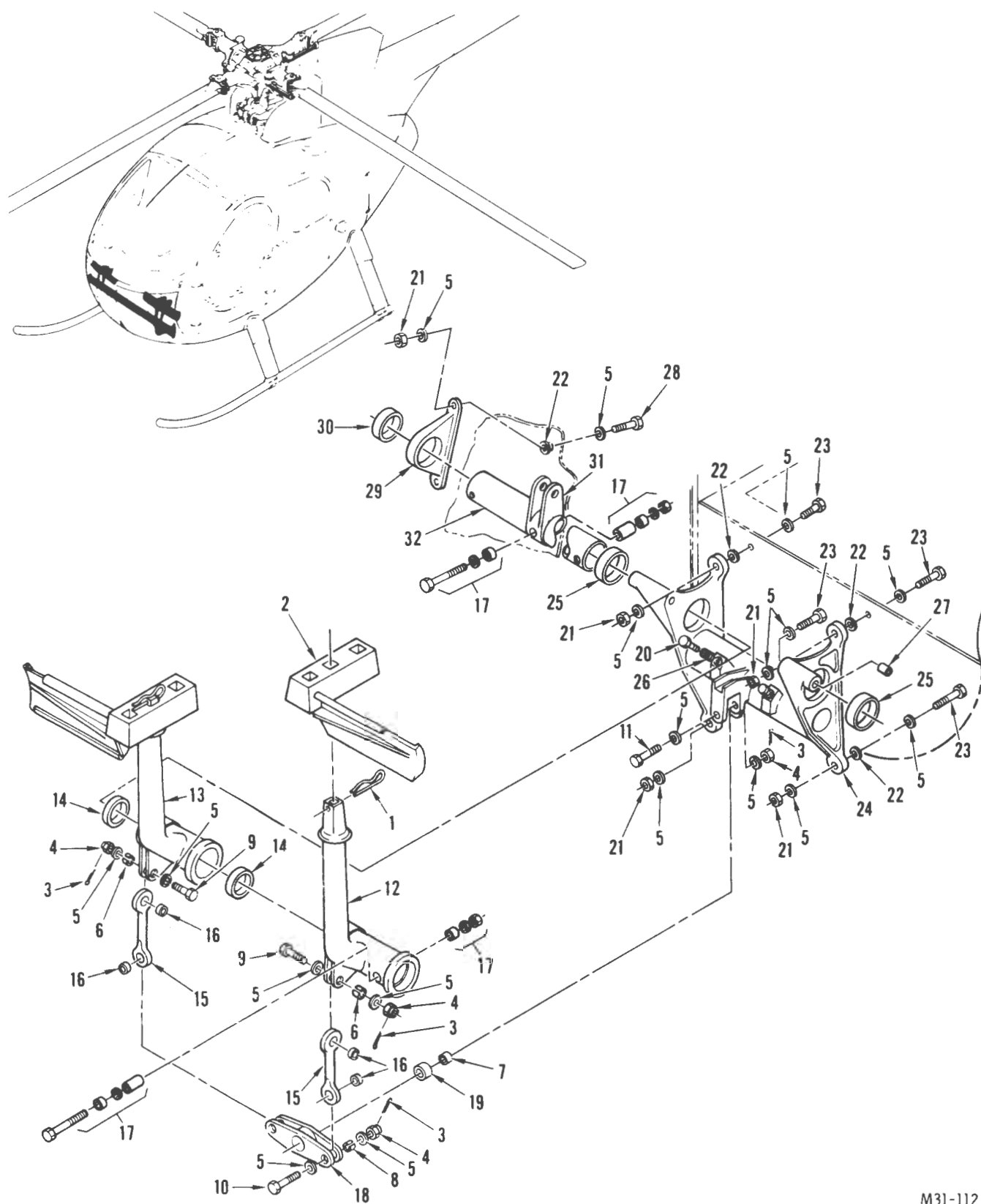
FIGURE 74. FOOT PEDAL INSTALLATION, ROTOR CONTROL
