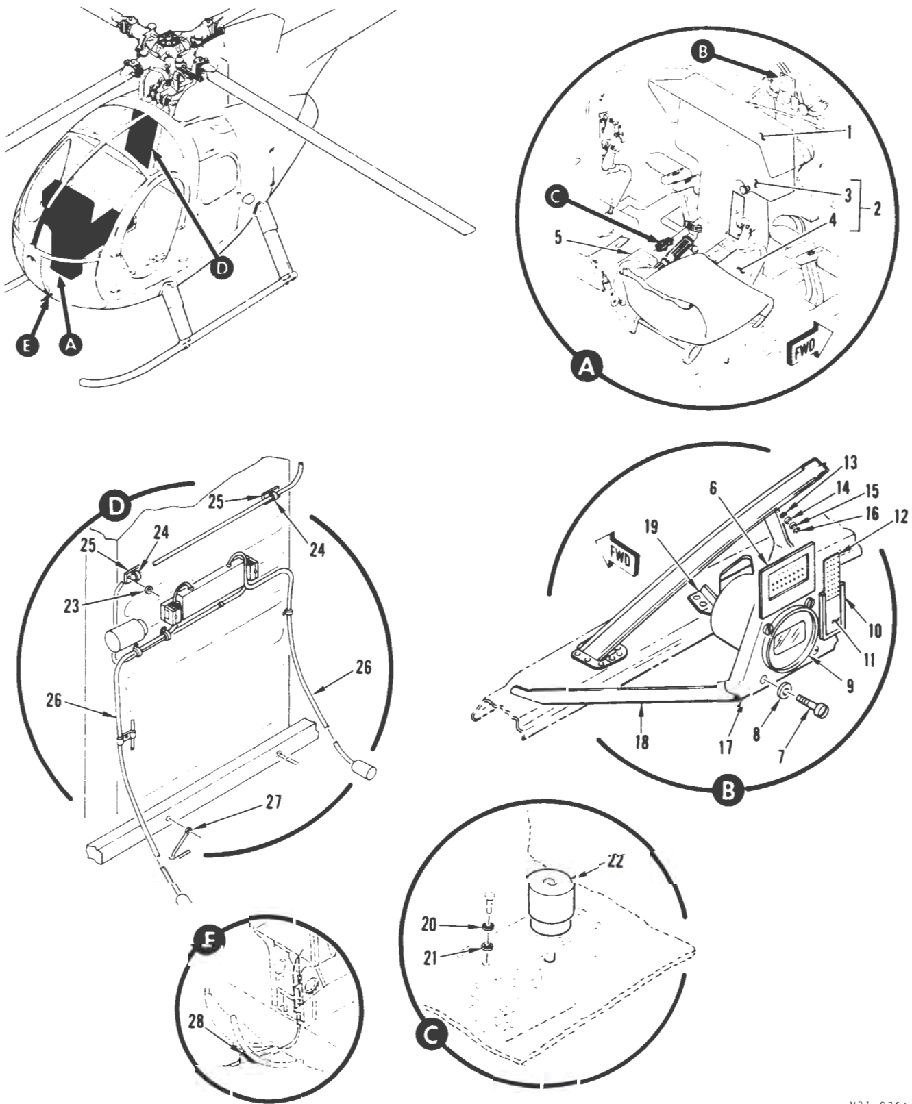
FIGURE 46. CONSOLE, COCKPIT INSTRUMENT, ELECTRICAL INSTALLATION
