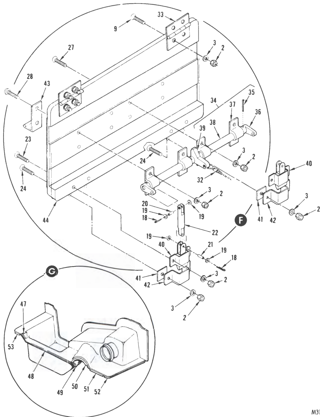
FIGURE 4. AFT SECTION INSTALLATION, FUSELAGE STRUCTURE (SHEET 2 OF 8)
