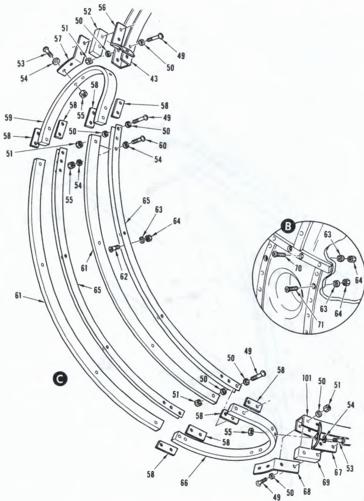
FIGURE 17A. WIRE STRIKE PROTECTION SYSTEM (SHEET 2 OF 3)
