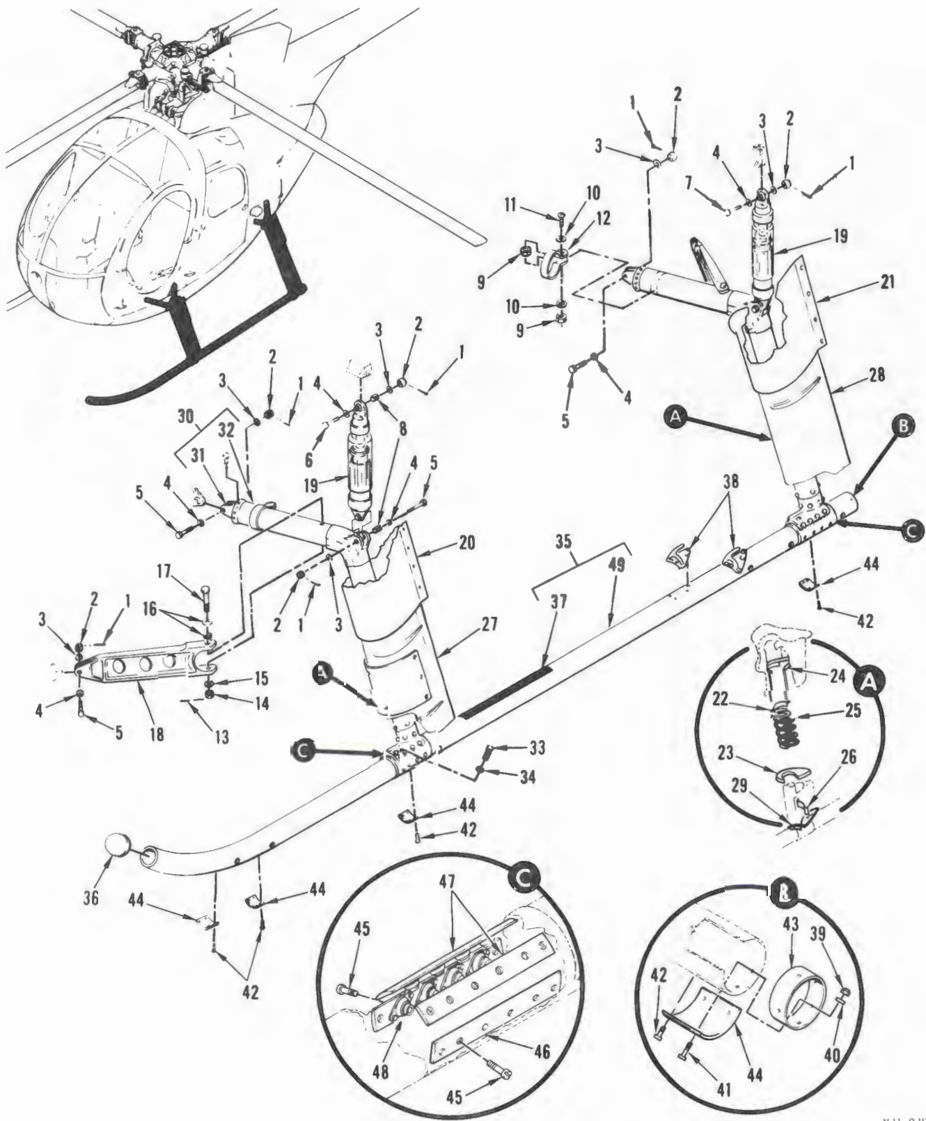
FIGURE 18. LANDING GEAR INSTALLATION
