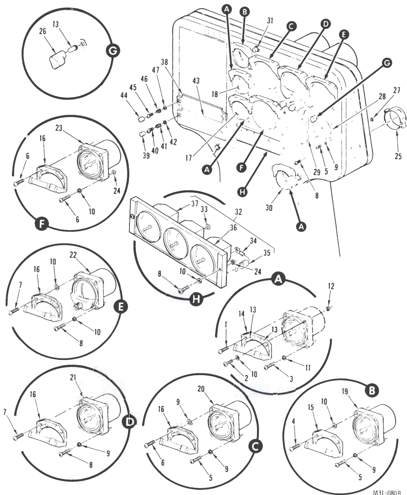
FIGURE 47. PANEL ASSEMBLY, COCKPIT INDICATOR (SHEET 1 of 2)
