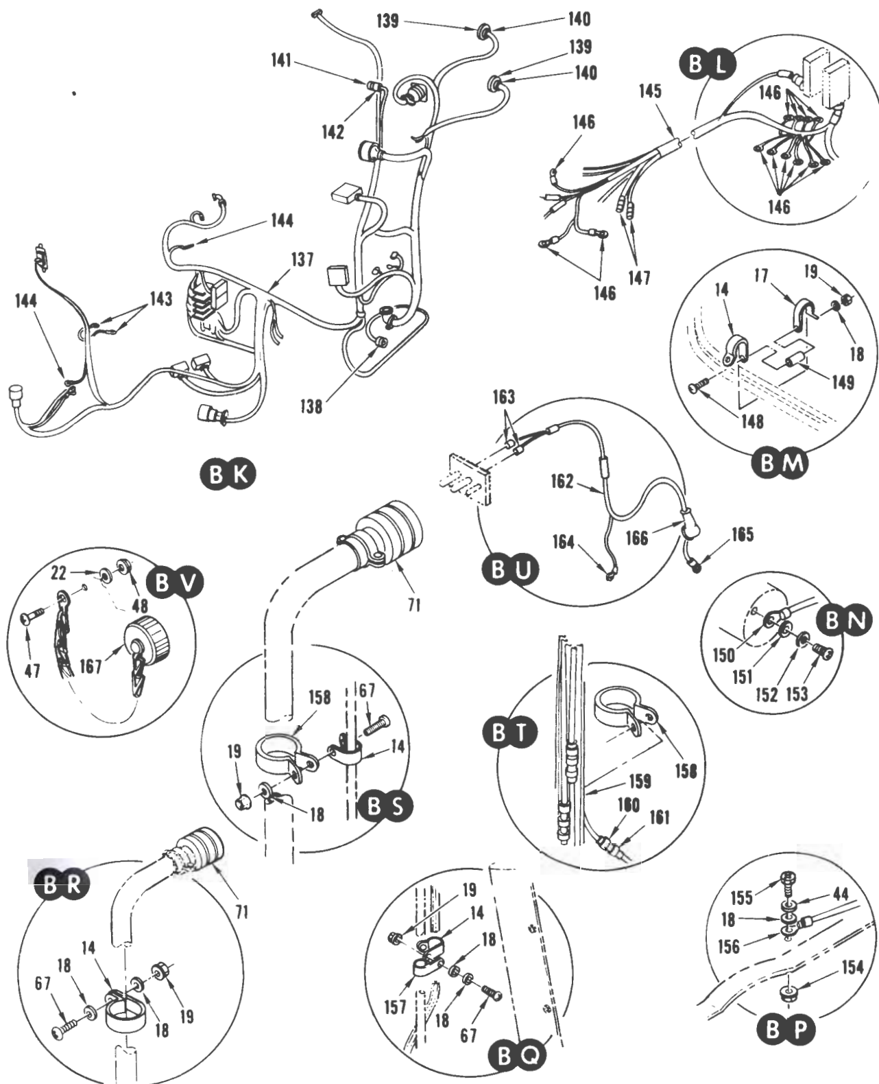
FIGURE 56. WIRE INSTALLATION, SERIES III (SHEET 11 OF 15)
