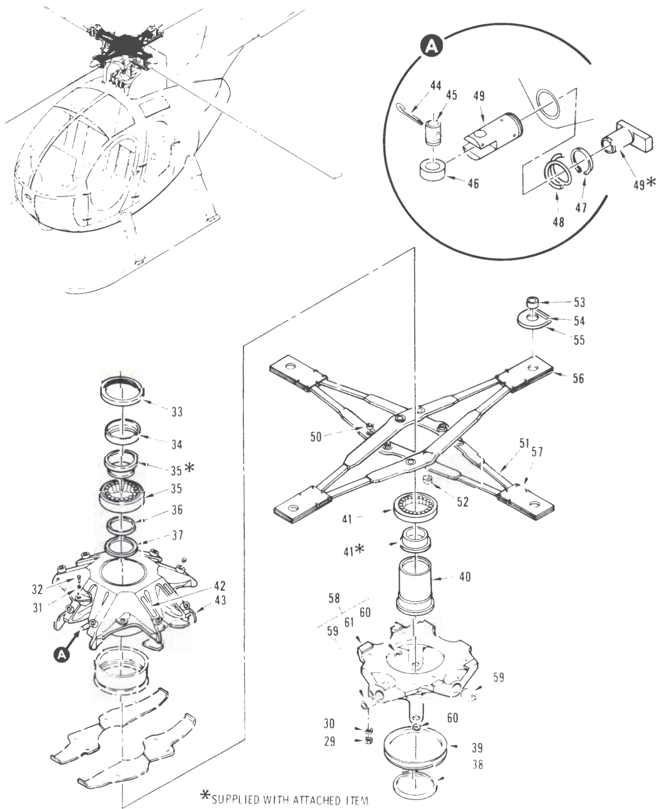
FIGURE 33. HUB ASSEMBLY, MAIN ROTOR (SHEET 2 OF 2)
