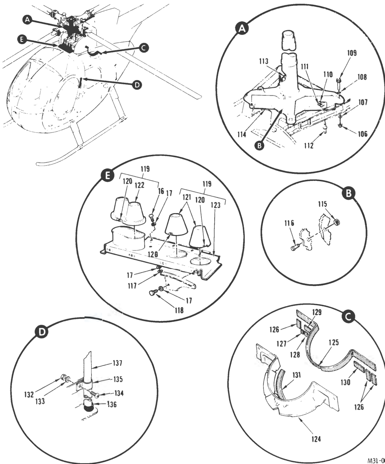
FIGURE 2. FUSELAGE STRUCTURE, COMPLETE (SHEET 5 OF 9)
