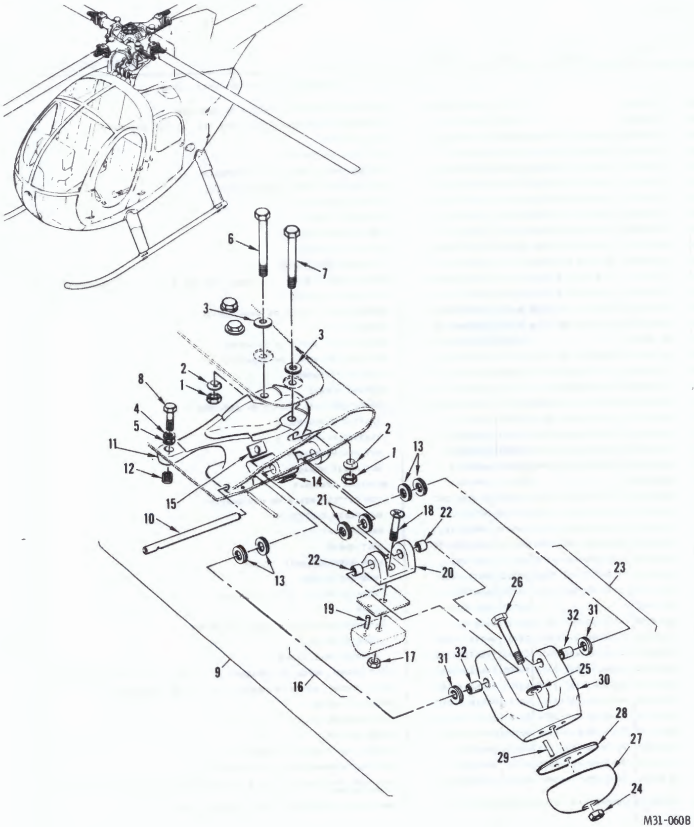
FIGURE 31. VIBRATION ABSORBER INSTALLATION
