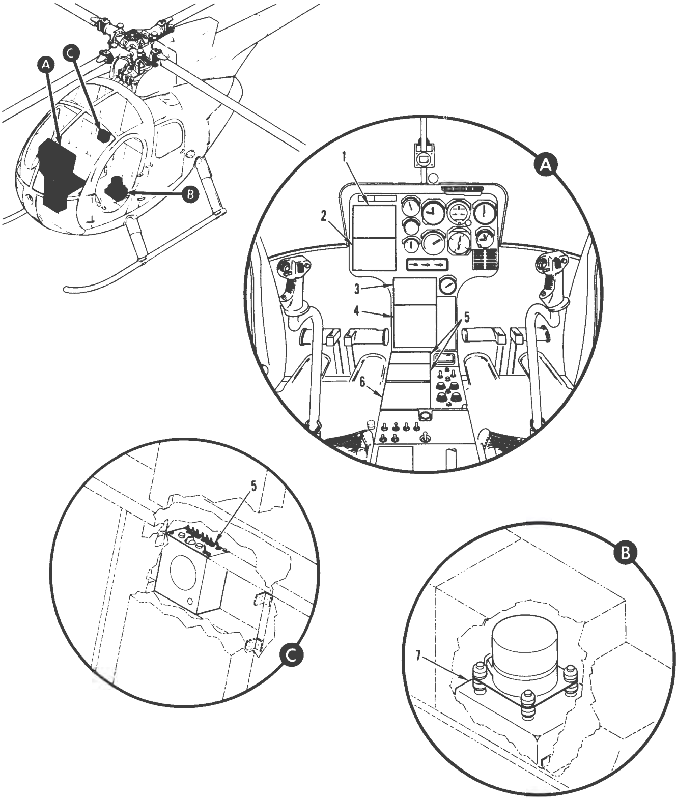
FIGURE 81. AVIONICS EQUIPMENT, SERIES III
