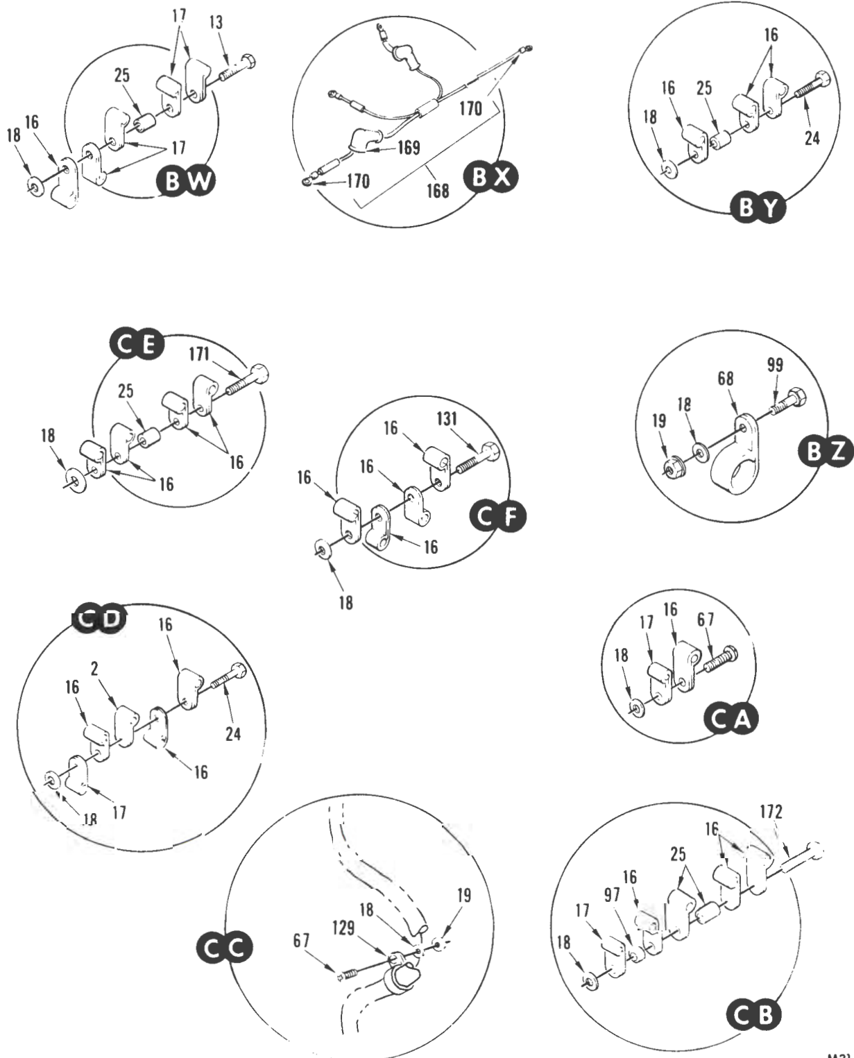
FIGURE 56. WIRE INSTALLATION, SERIES III (SHEET 12 OF 15)
