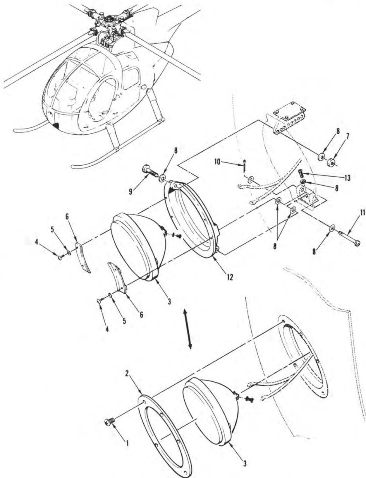
FIGURE 53. EXTERIOR LIGHTING INSTALLATION (SHEET 1 OF 2)
