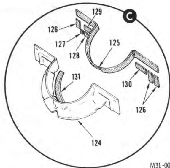
FIGURE 2. FUSELAGE STRUCTURE, COMPLETE (SHEET 5 OF 9)
