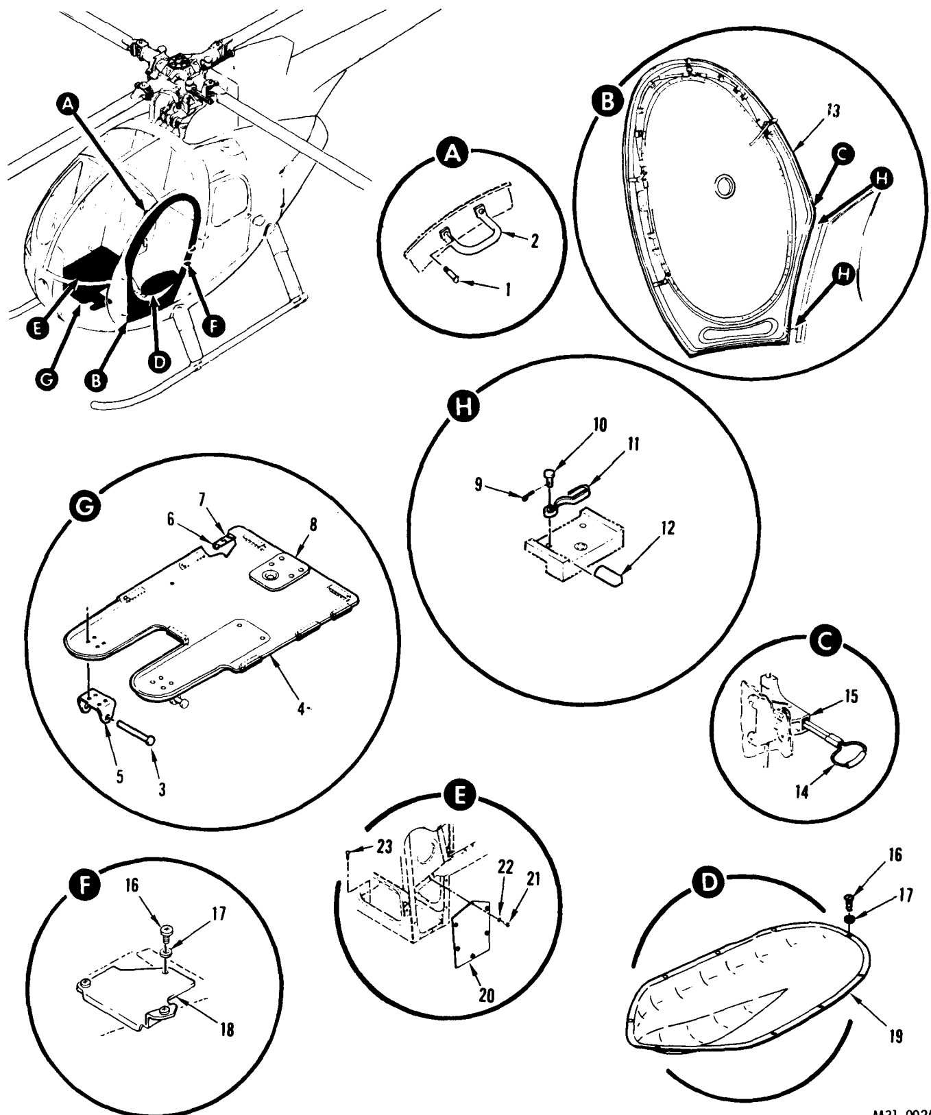
FIGURE 2. FUSELAGE STRUCTURE, COMPLETE (SHEET 1 OF 9)
