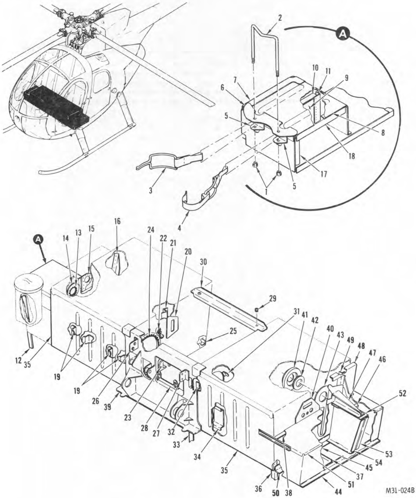
FIGURE 7. SEAT STRUCTURE INSTALLATION
