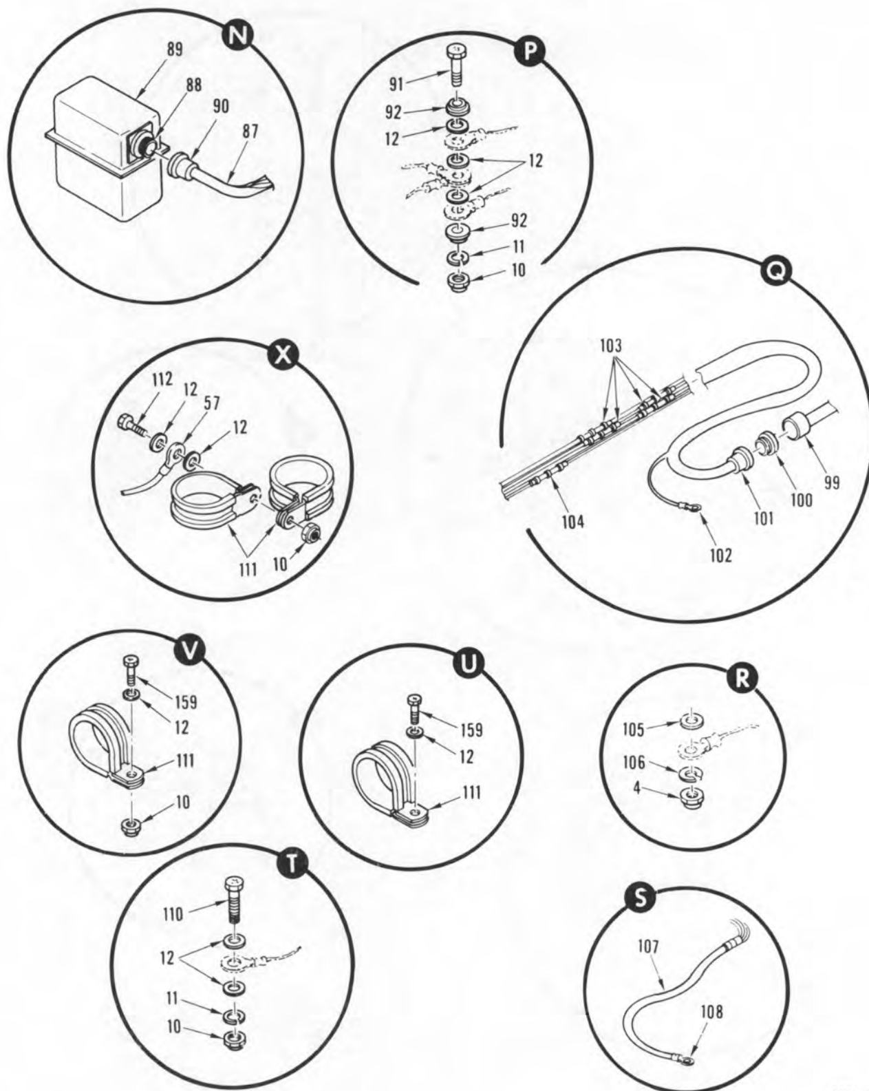
FIGURE 55. WIRE INSTALLATION, SERIES I AND II (SHEET 7 OF 9)
