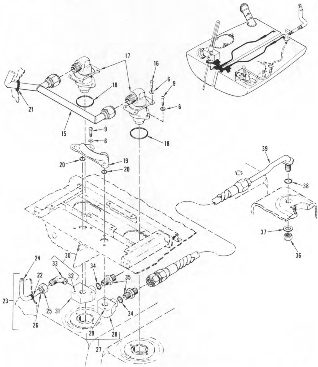
FIGURE 59. CRASHWORTHY FUEL SYSTEM - VENT (SHEET 2 OF 2)
