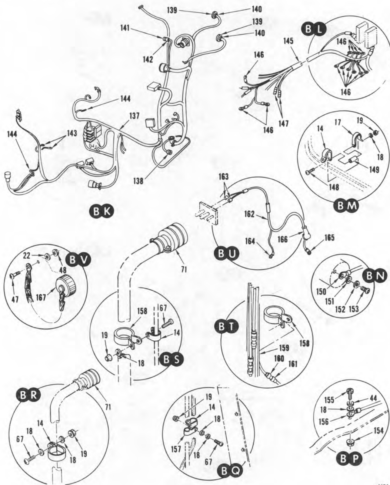
FIGURE 56. WIRE INSTALLATION, SERIES III (SHEET 11 OF 15)
