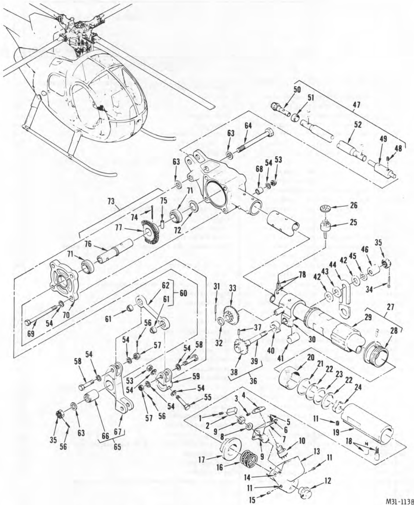
FIGURE 72. CONTROL STICK, AIRCRAFT, PILOT COLLECTIVE
