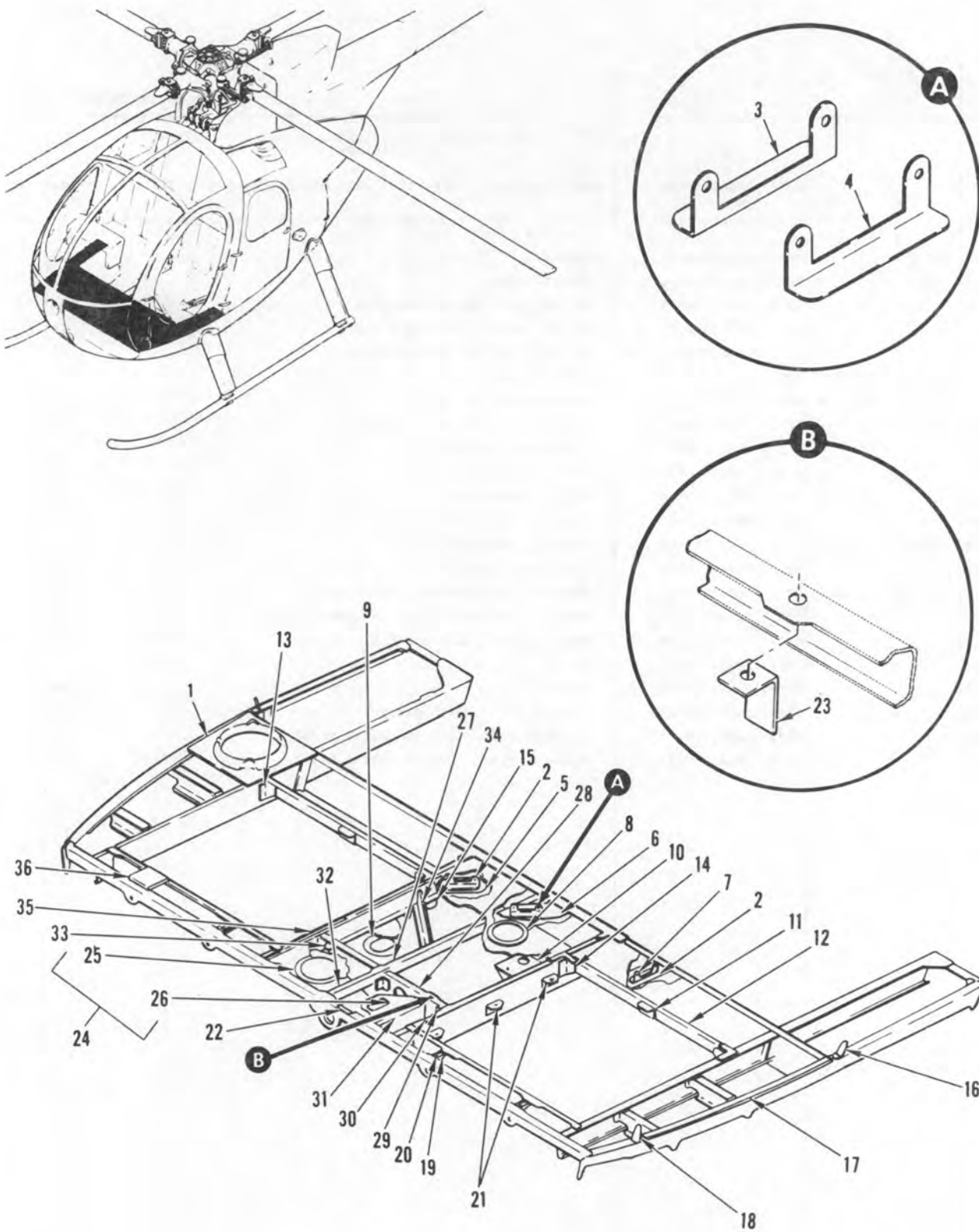
FIGURE 12. FLOOR INSTALLATION, PILOTS, LOWER SECTION
