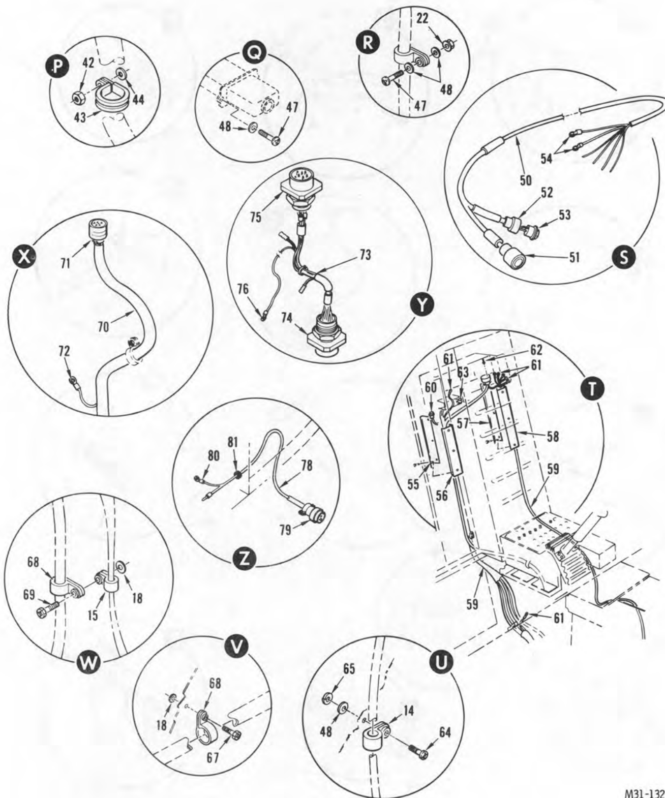
FIGURE 56. WIRE INSTALLATION, SERIES III (SHEET 7 OF 15)
