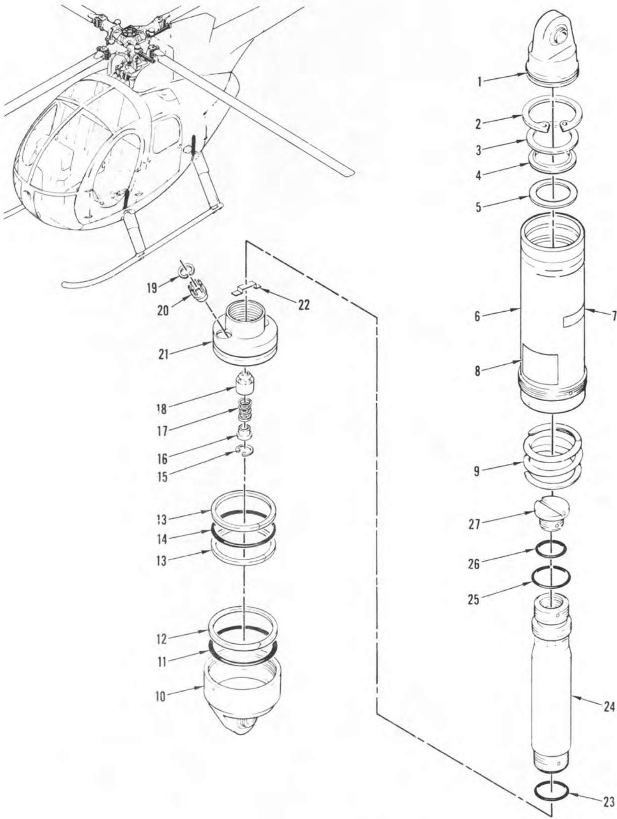
FIGURE 19. DAMPER ASSEMBLY, LANDING GEAR
