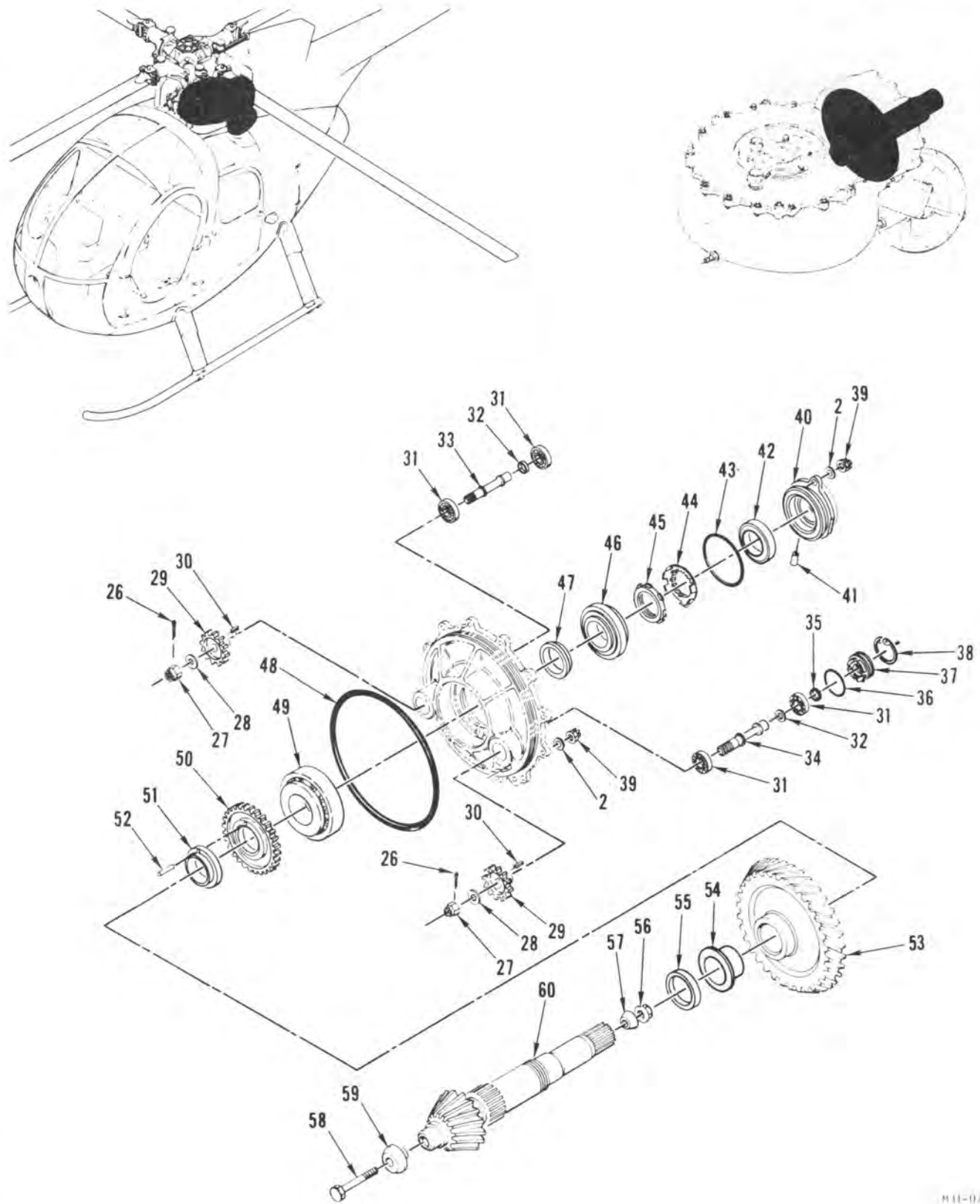
FIGURE 40. TRANSMISSION ASSEMBLY (DRIVES INSTALLATION) (SHEET 2 OF 3)
