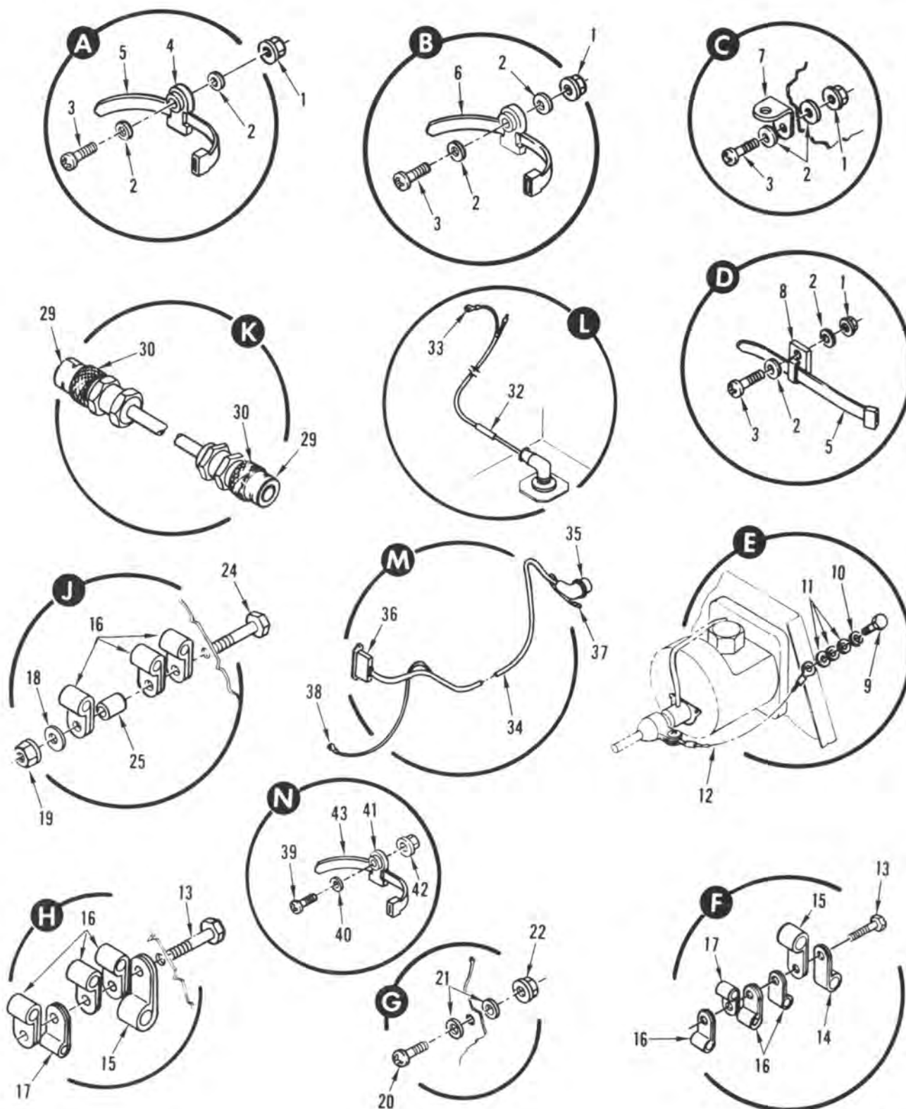
FIGURE 56. WIRE INSTALLATION, SERIES III (SHEET 6 OF 15)
