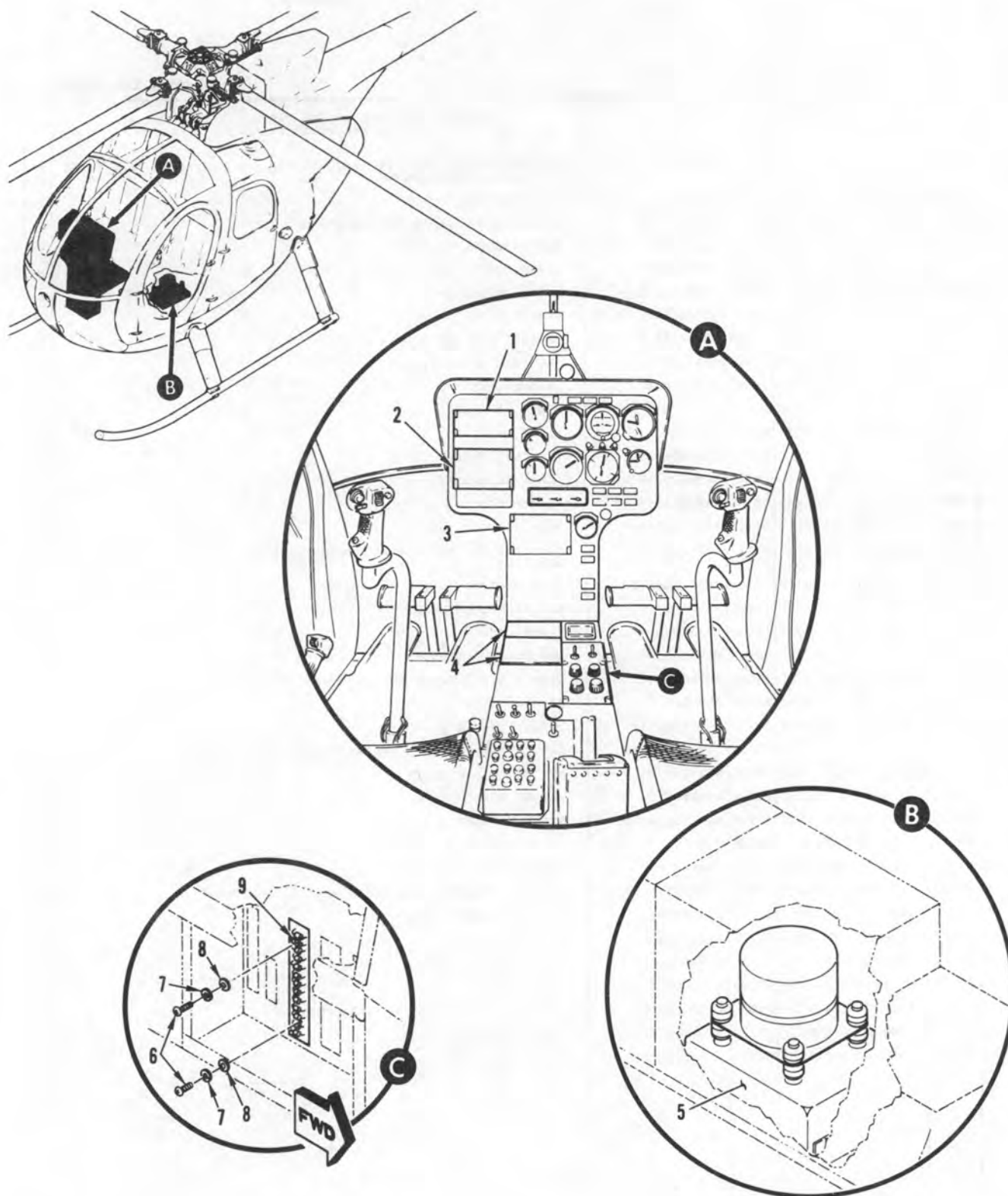
FIGURE 80. AVIONICS EQUIPMENT, SERIES I AND II
