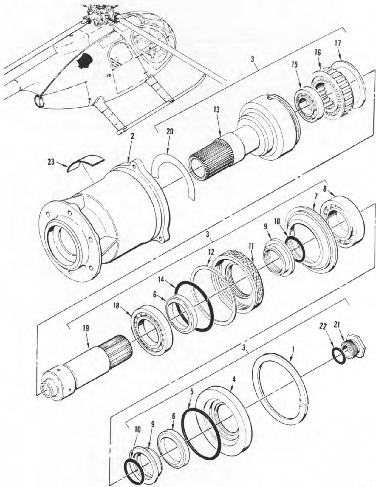
FIGURE 41. CLUTCH, TRANSMISSION
