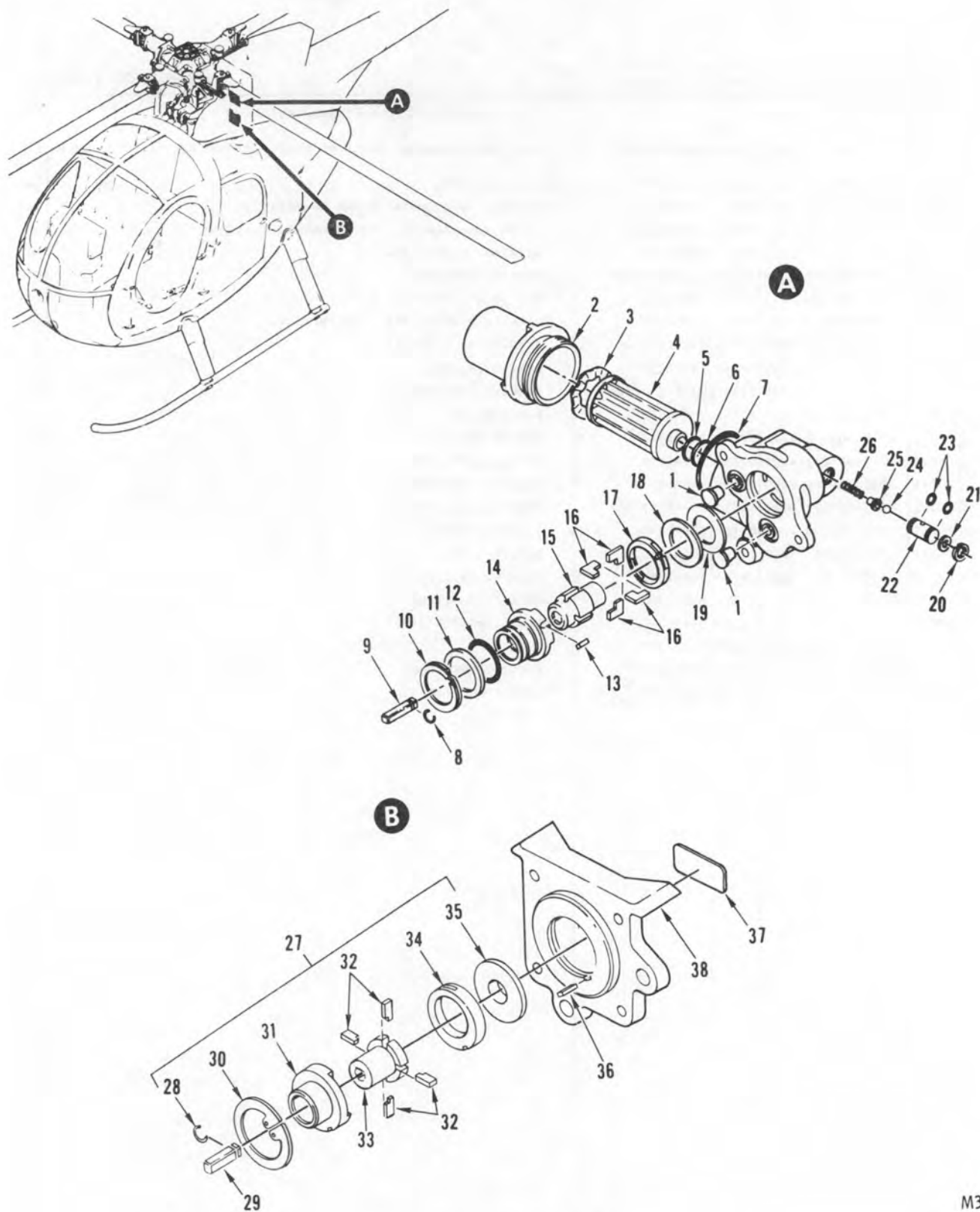
FIGURE 42. PUMP, ROTARY
