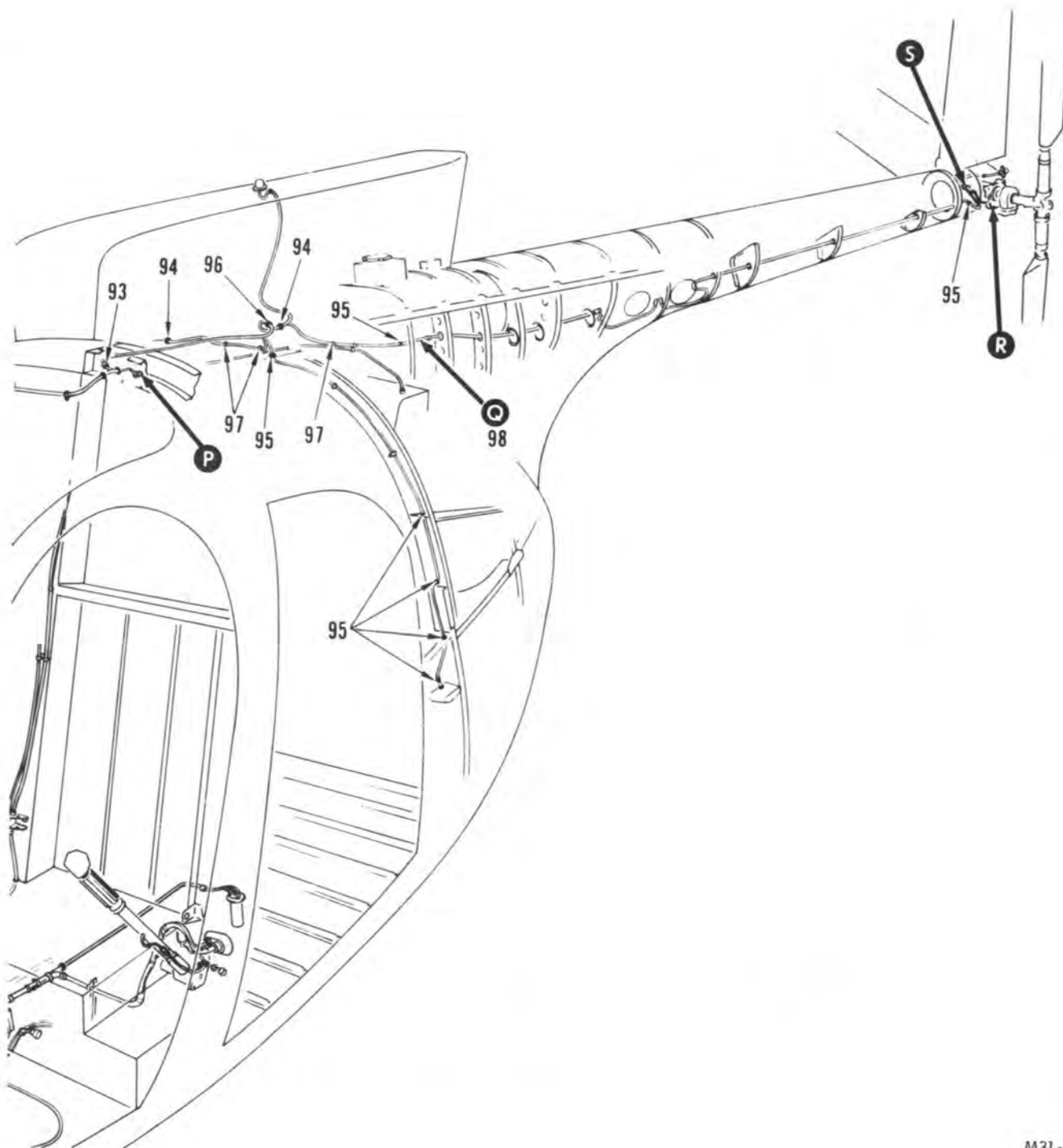
FIGURE 55. WIRE INSTALLATION, SERIES I AND II (SHEET 2 OF 9)
