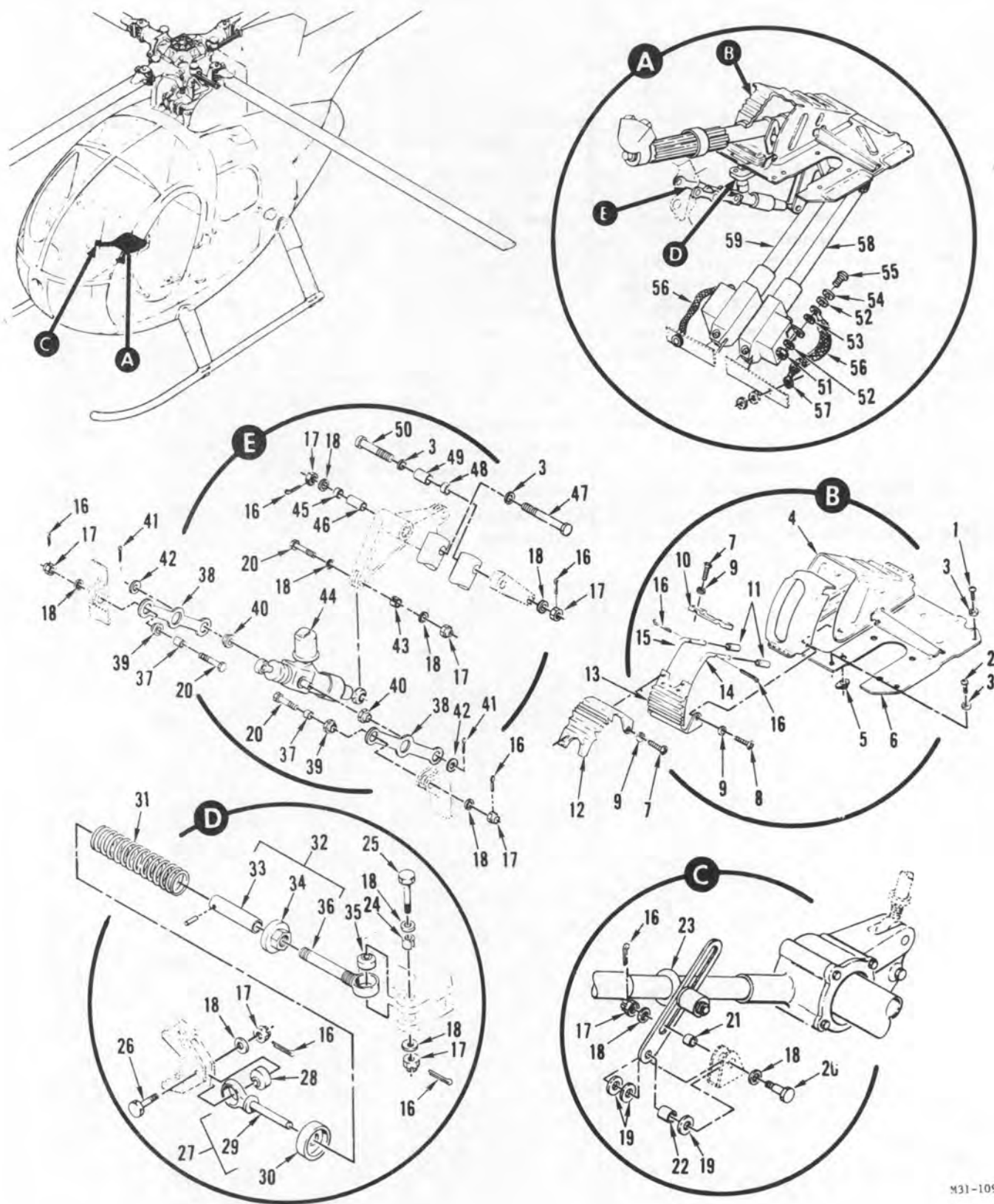
FIGURE 68. FORWARD CONTROLS INSTALLATION (PART I)
