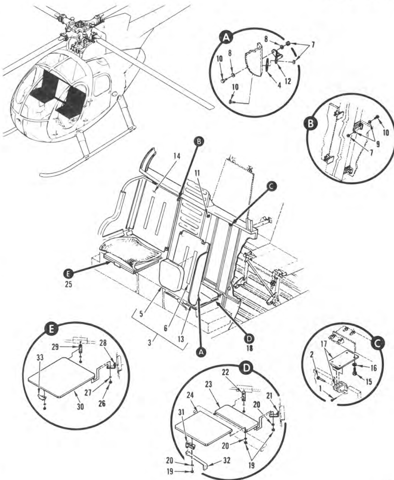
FIGURE 17. ARMOR INSTALLATION, SEATS (SHEET 1 OF 2)
