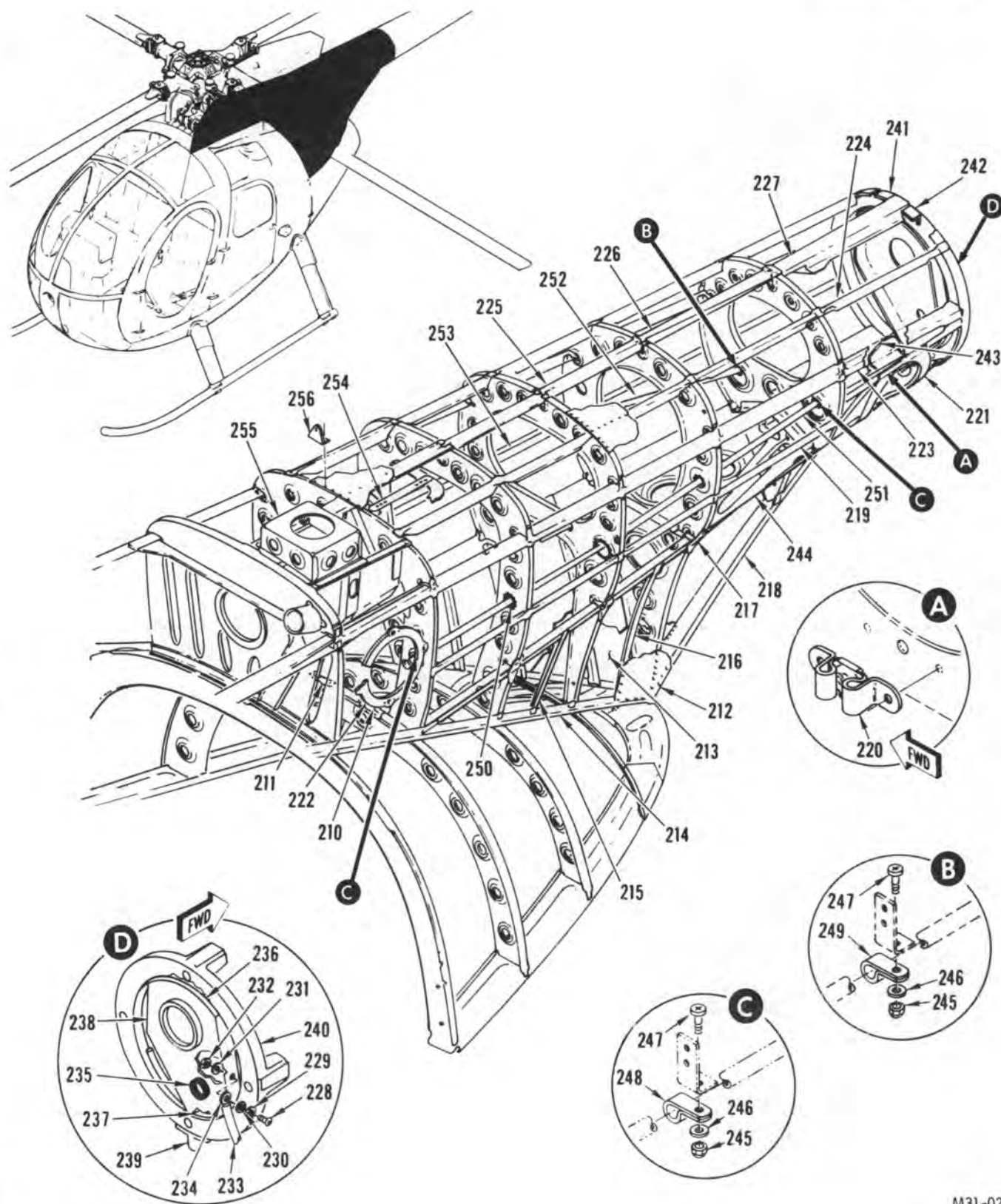
FIGURE 4. AFT SECTION INSTALLATION, FUSELAGE STRUCTURE (SHEET 7 OF 8)
