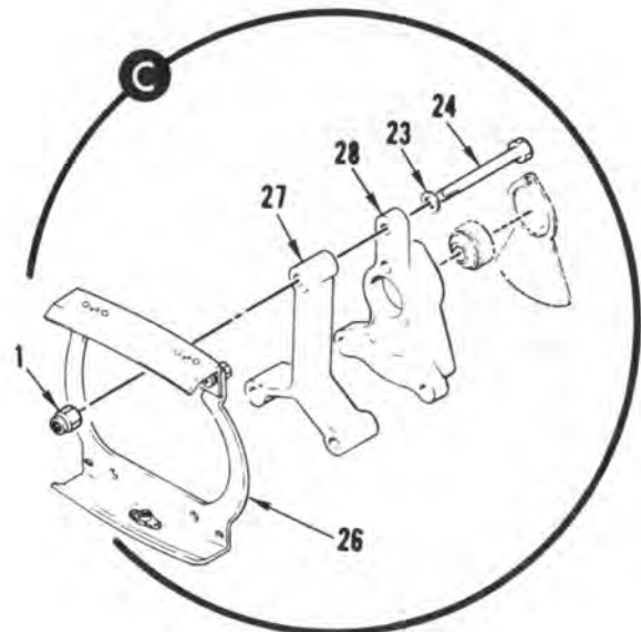
FIGURE 33. HUB ASSEMBLY, MAIN ROTOR (SHEET 1 OF 2)
