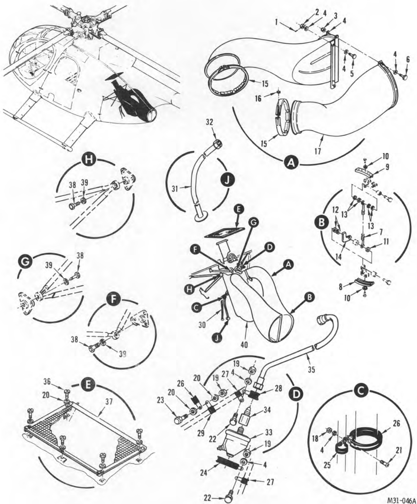
FIGURE 22. ENGINE INSTALLATION, HELICOPTER
