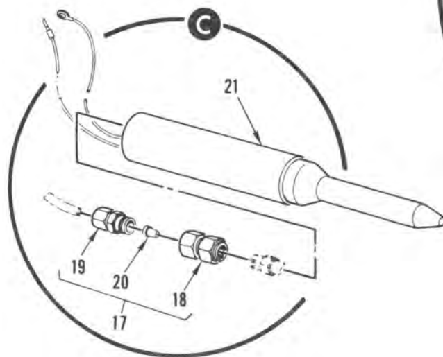
FIGURE 44. INSTRUMENT INSTALLATION, ELECTRICAL (SERIES I AND II) (SHEET 1 of 2)
