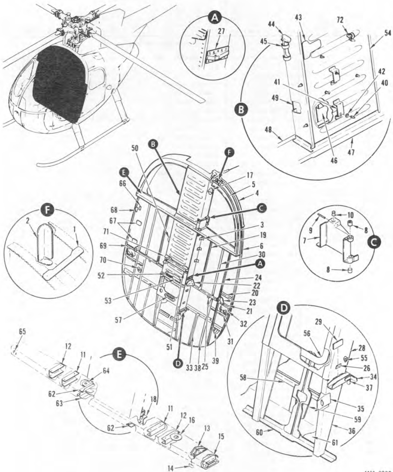
FIGURE 9. FRAME INSTALLATION, CANTED
