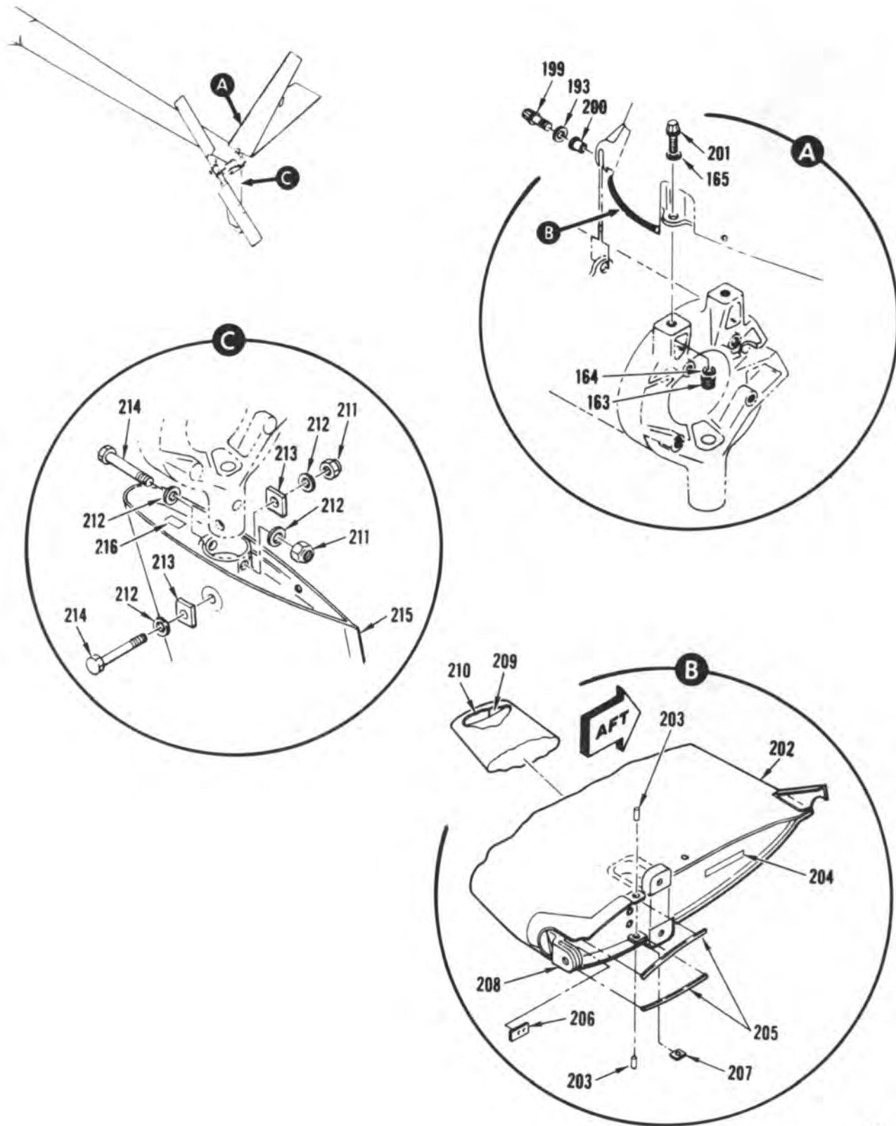
FIGURE 2. FUSELAGE STRUCTURE, COMPLETE (SHEET 9 OF 9)
