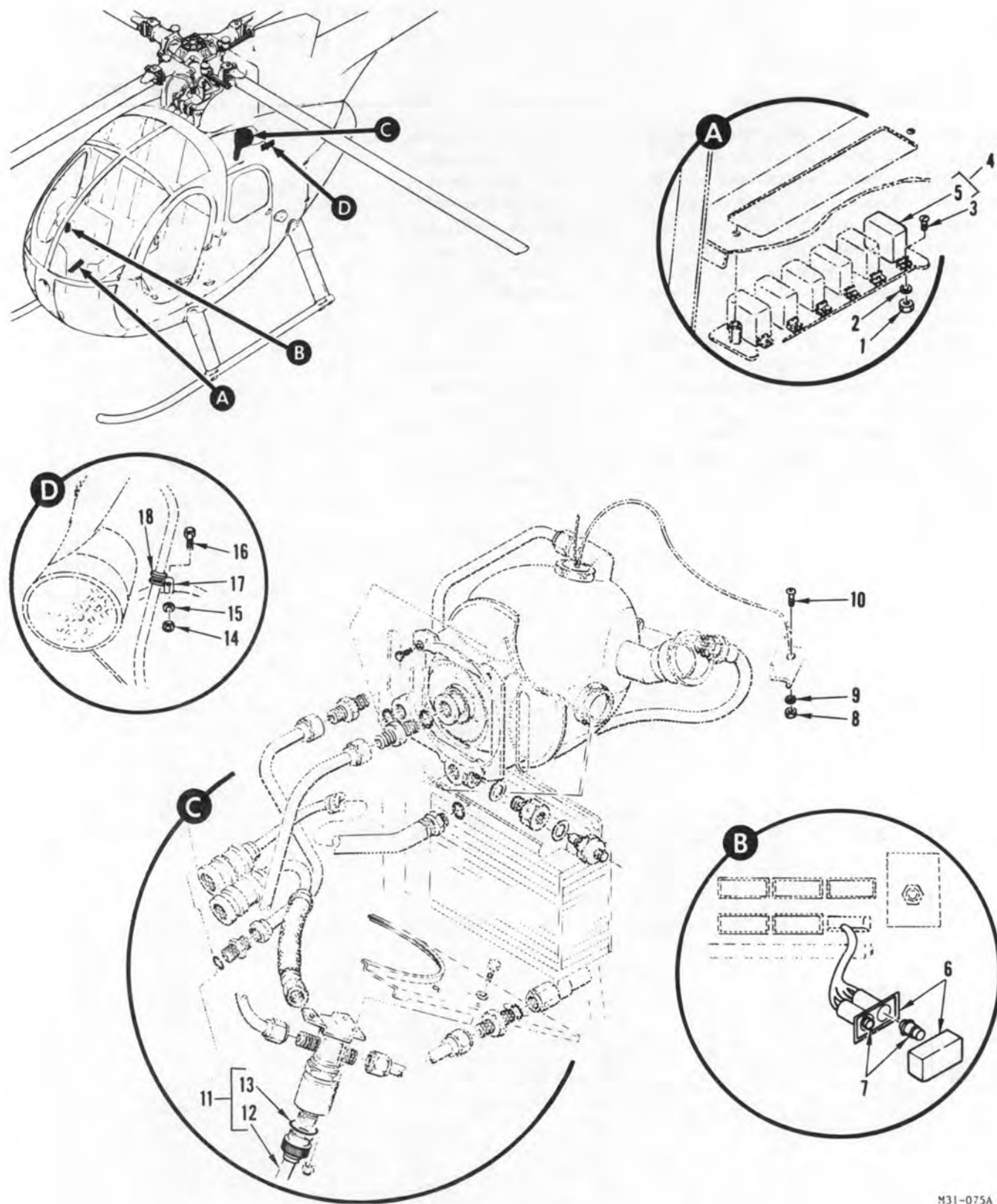
FIGURE 51. ELECTRICAL SYSTEM INSTALLATION, ARMOR
