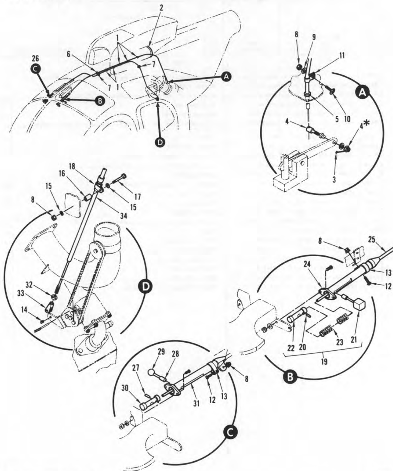
FIGURE 78. HEATING SYSTEM INSTALLATION (HEAT AND DE-ICER VALVE CONTROL)
