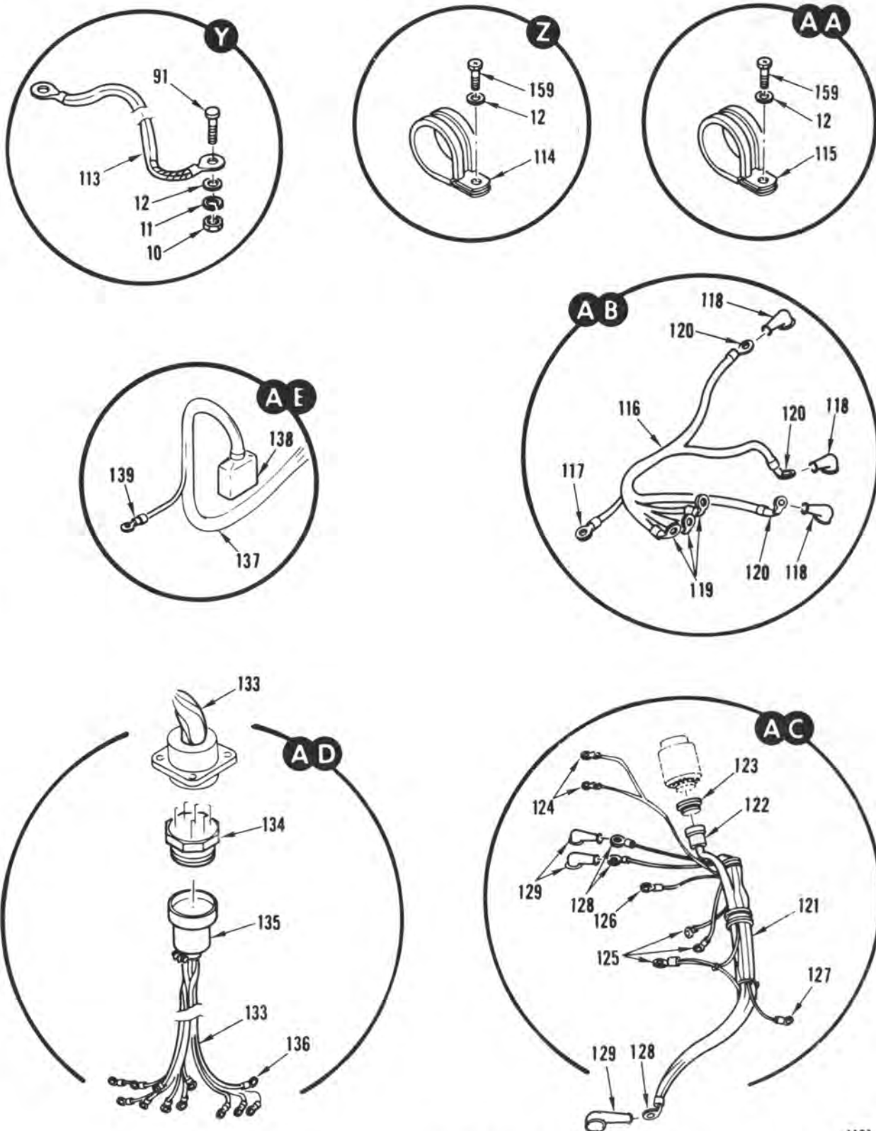
FIGURE 55. WIRE INSTALLATION, SERIES I AND II (SHEET 8 OF 9)
