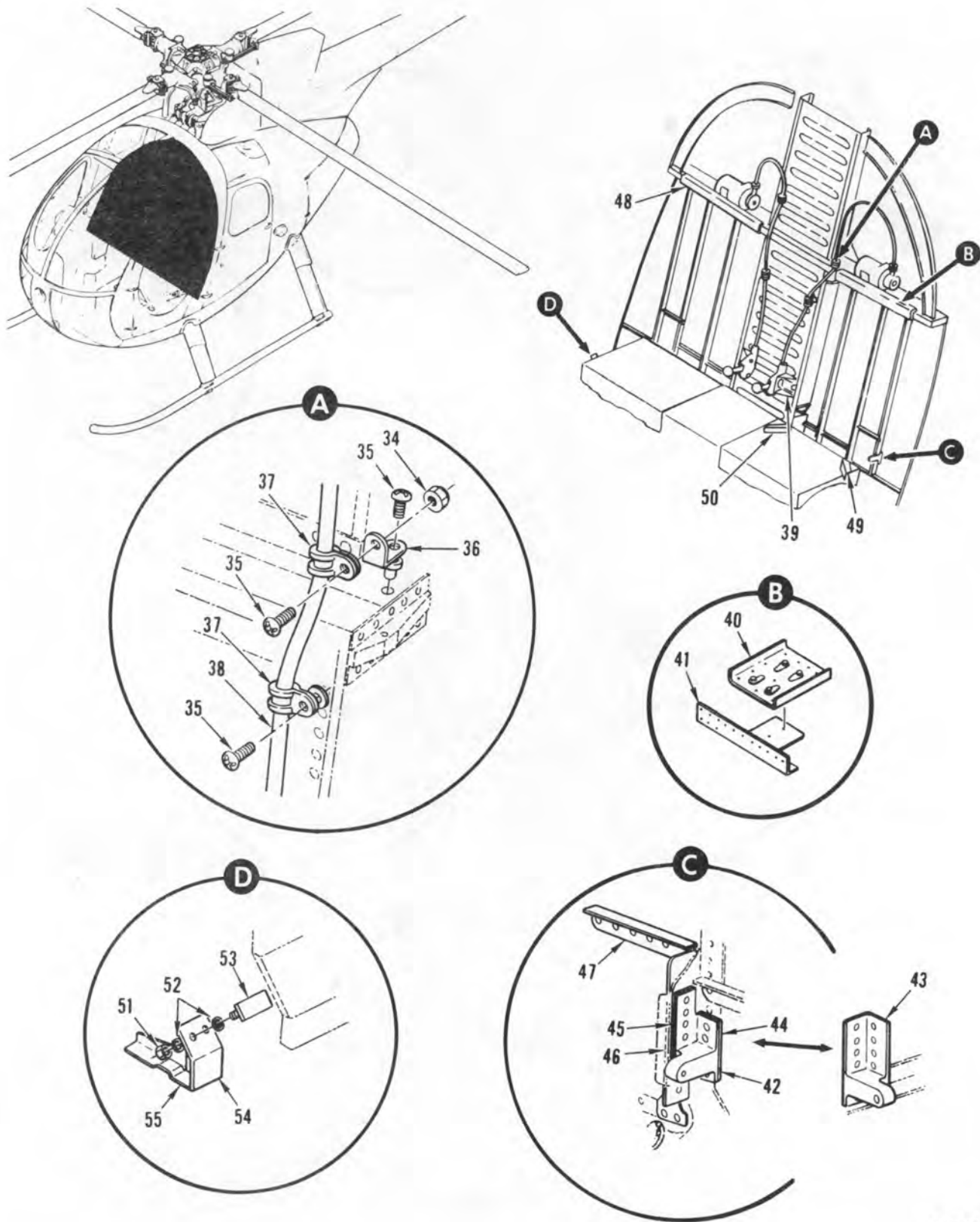
FIGURE 17. ARMOR INSTALLATION, SEATS (SHEET 2 OF 2)
