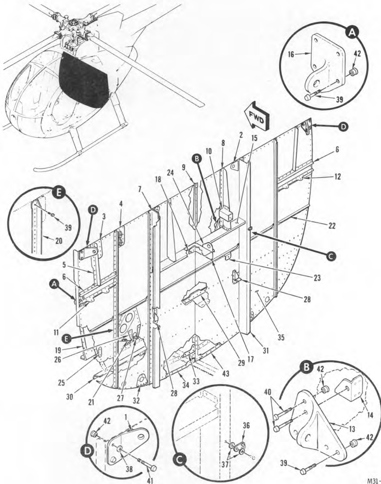
FIGURE 10. FRAME INSTALLATION, LOWER SECTION
