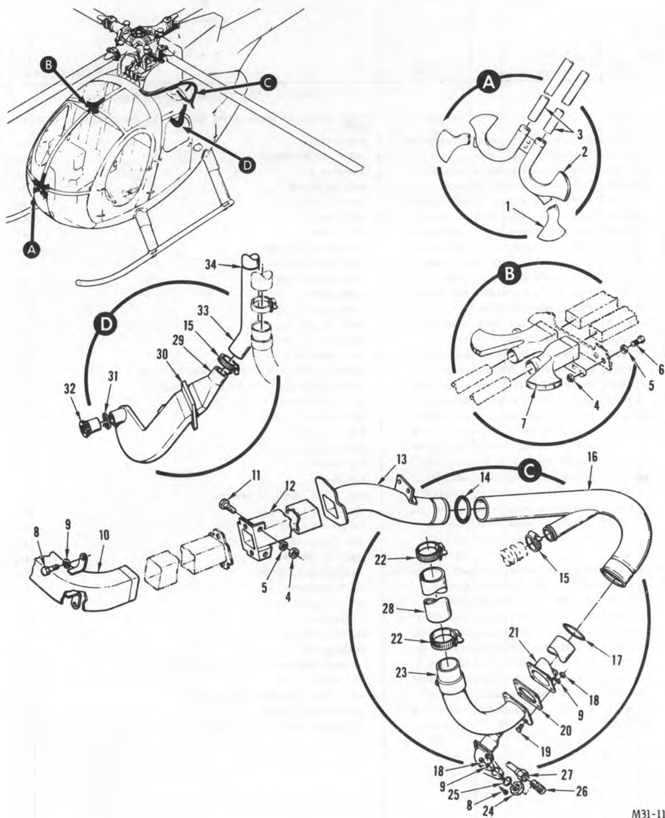
FIGURE 76. HEATING SYSTEM INSTALLATION (CABIN DISTRIBUTION)
