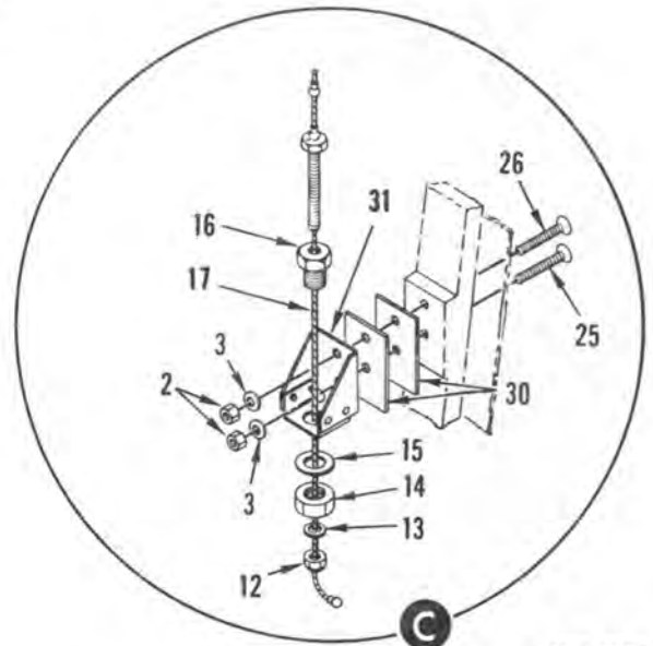
FIGURE 4. AFT SECTION INSTALLATION, FUSELAGE STRUCTURE (SHEET 1 OF 8)
