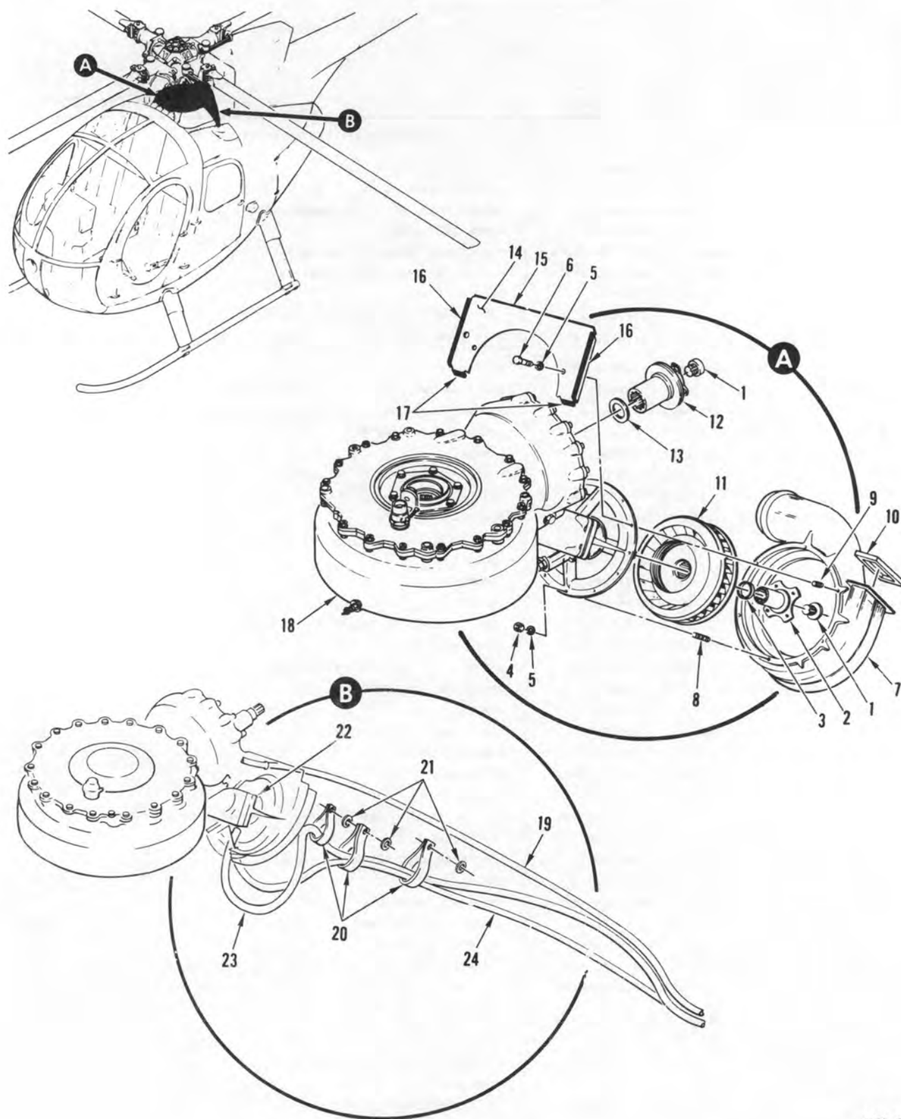
FIGURE 38. MAIN TRANSMISSION BUILD-UP UNIT AND DRAIN UNIT INSTALLATION
