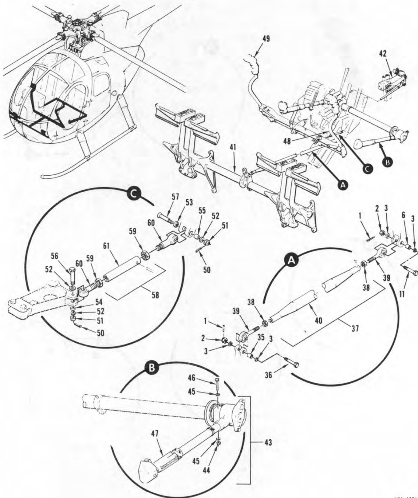
FIGURE 63. FLIGHT CONTROLS INSTALLATION (FORWARD) (SHEET 2 OF 2)
