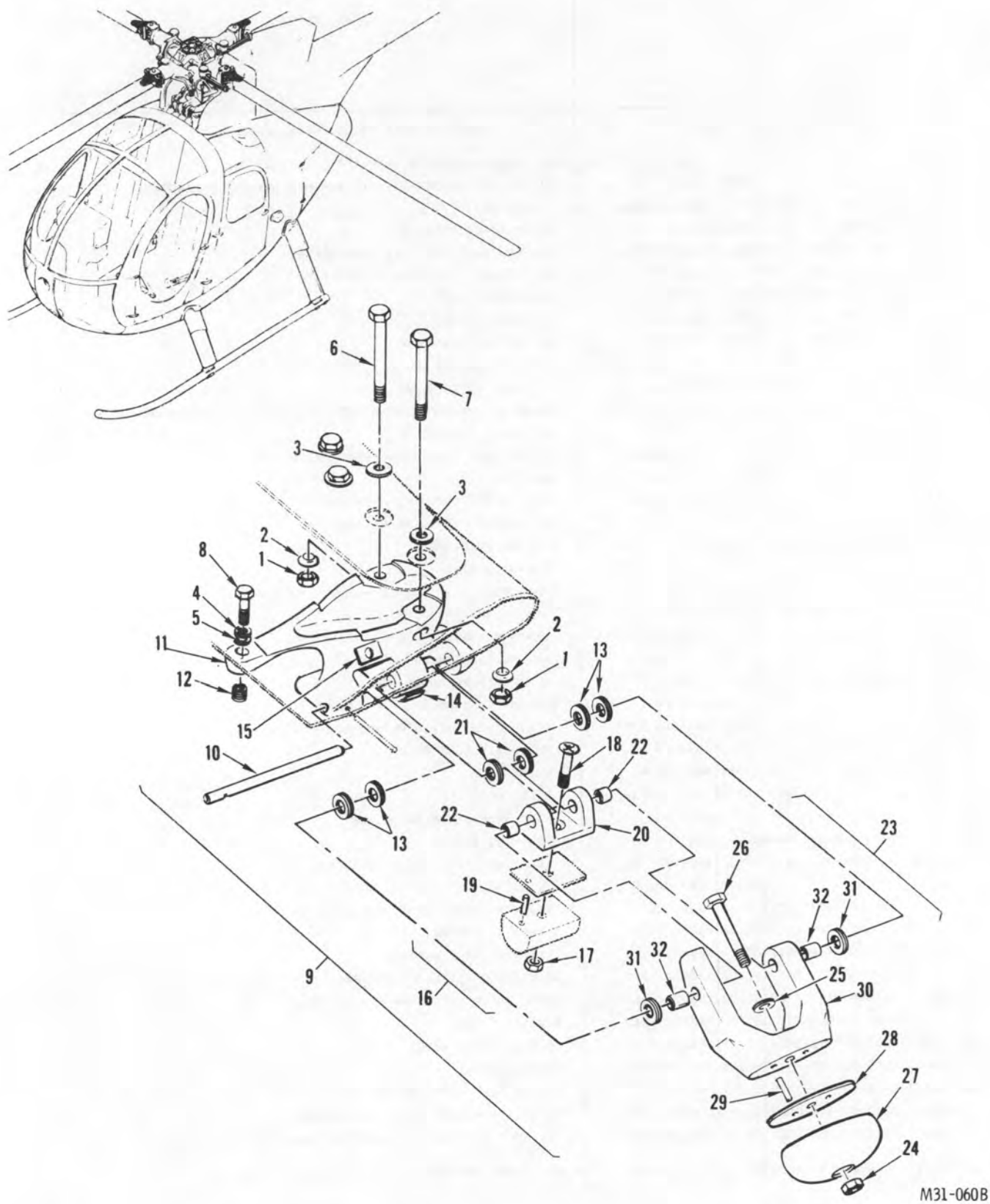
FIGURE 31. VIBRATION ABSORBER INSTALLATION
