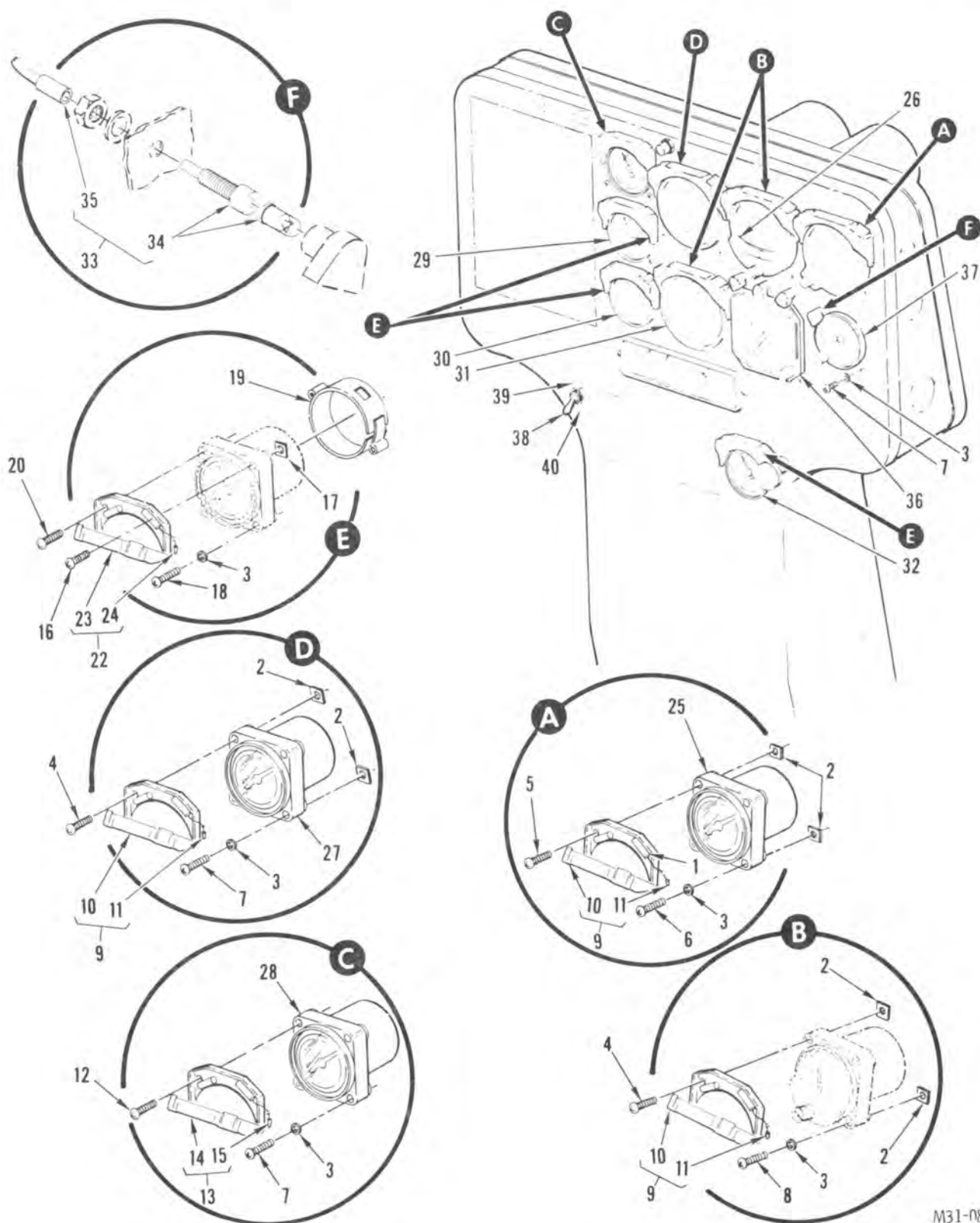
FIGURE 45. ELECTRICAL INSTALLATION (INSTRUMENTS, SERIES III) (SHEET 1 OF 2)
