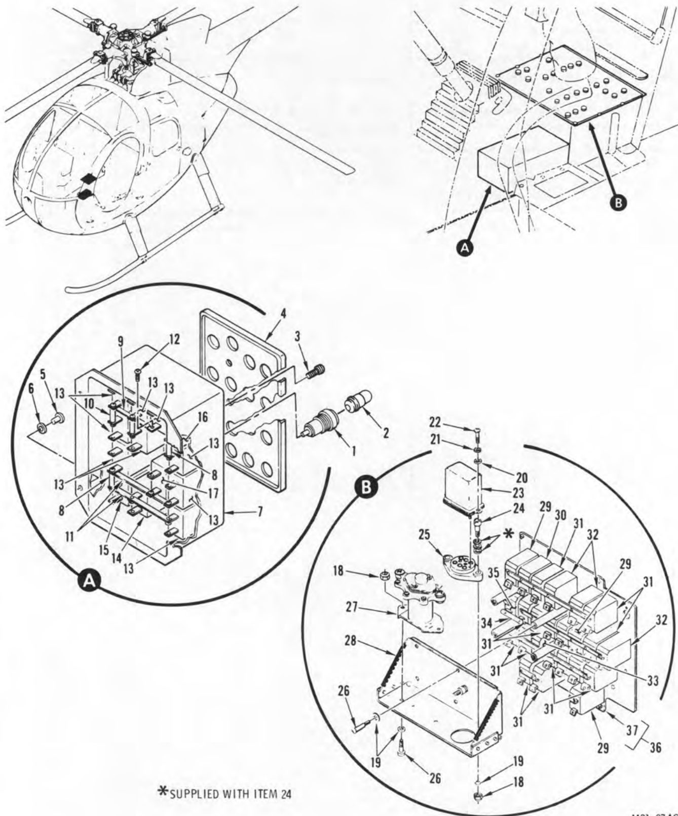
FIGURE 48. CIRCUIT BREAKER ASSEMBLY, ELECTRICAL EQUIPMENT
