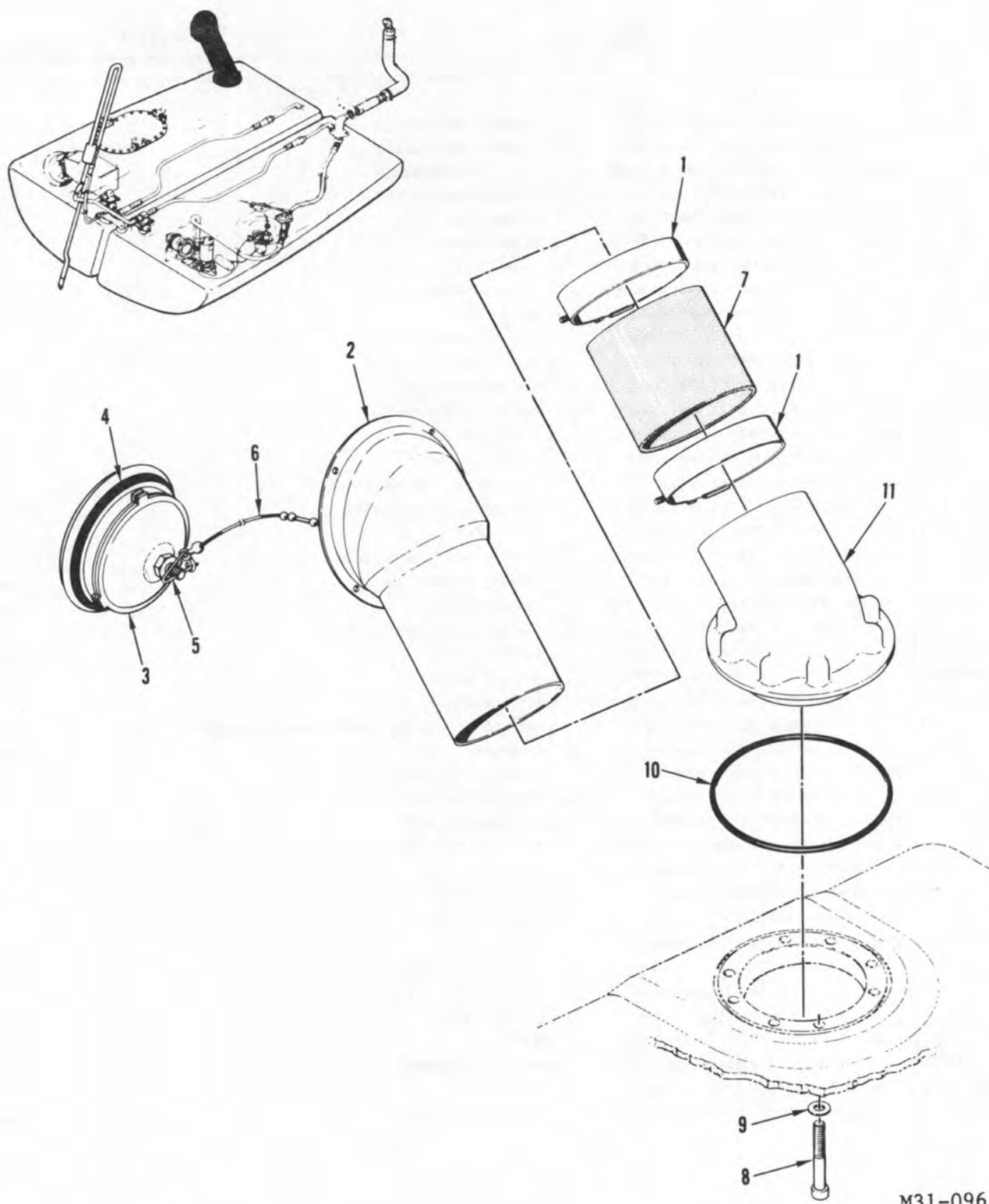
FIGURE 61. CRASHWORTHY FUEL SYSTEM - GRAVITY FILLER
