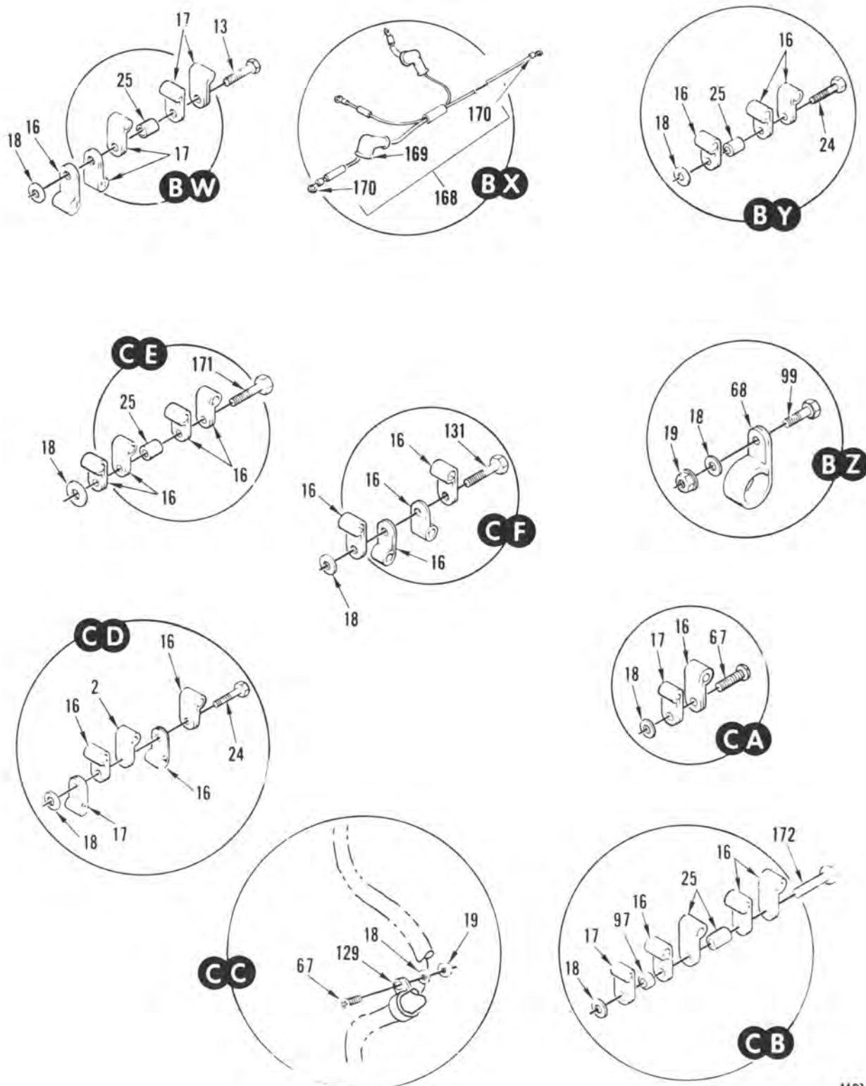
FIGURE 56. WIRE INSTALLATION, SERIES III (SHEET 12 OF 15)
