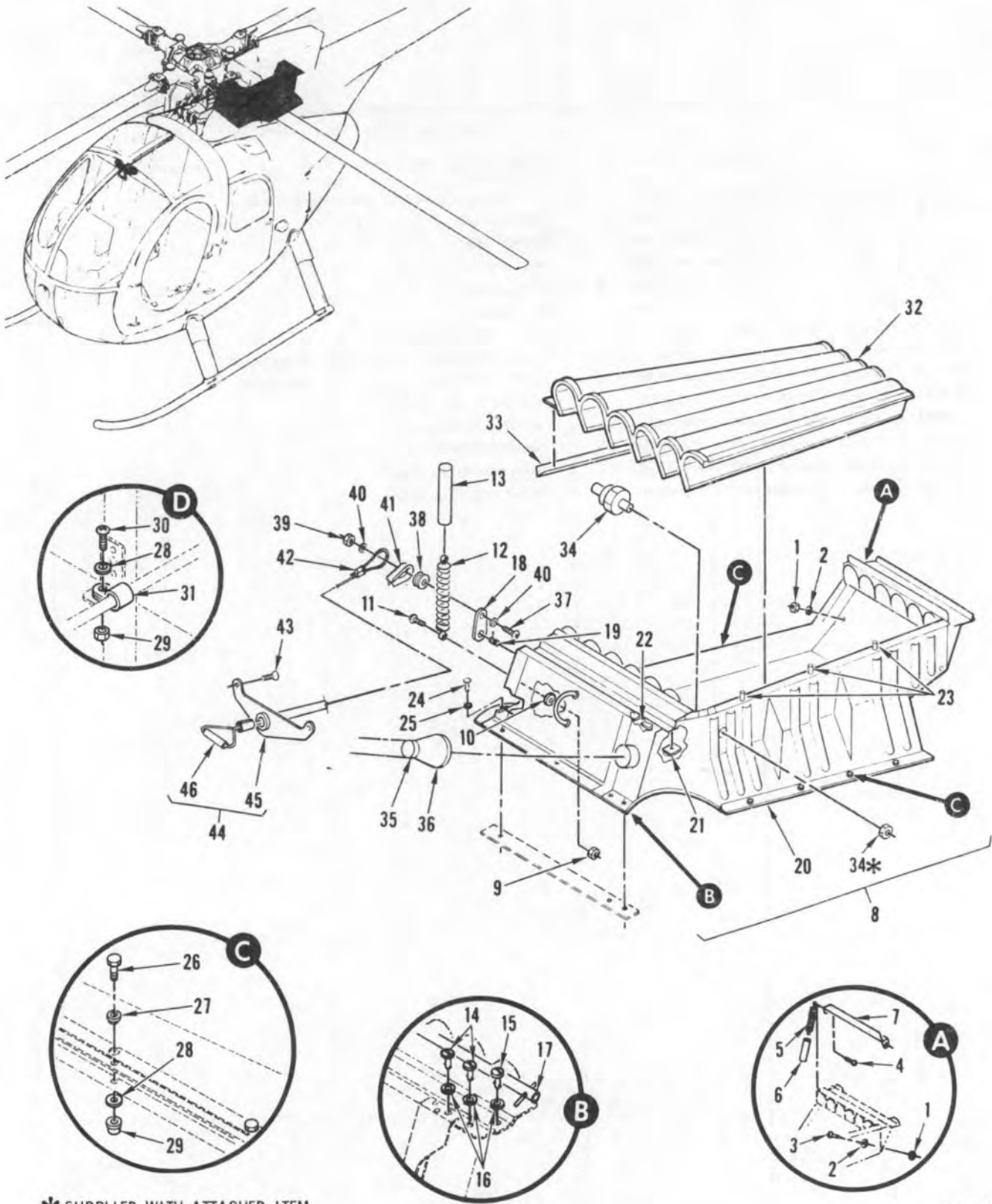
FIGURE 26. BARRIER FILTER
