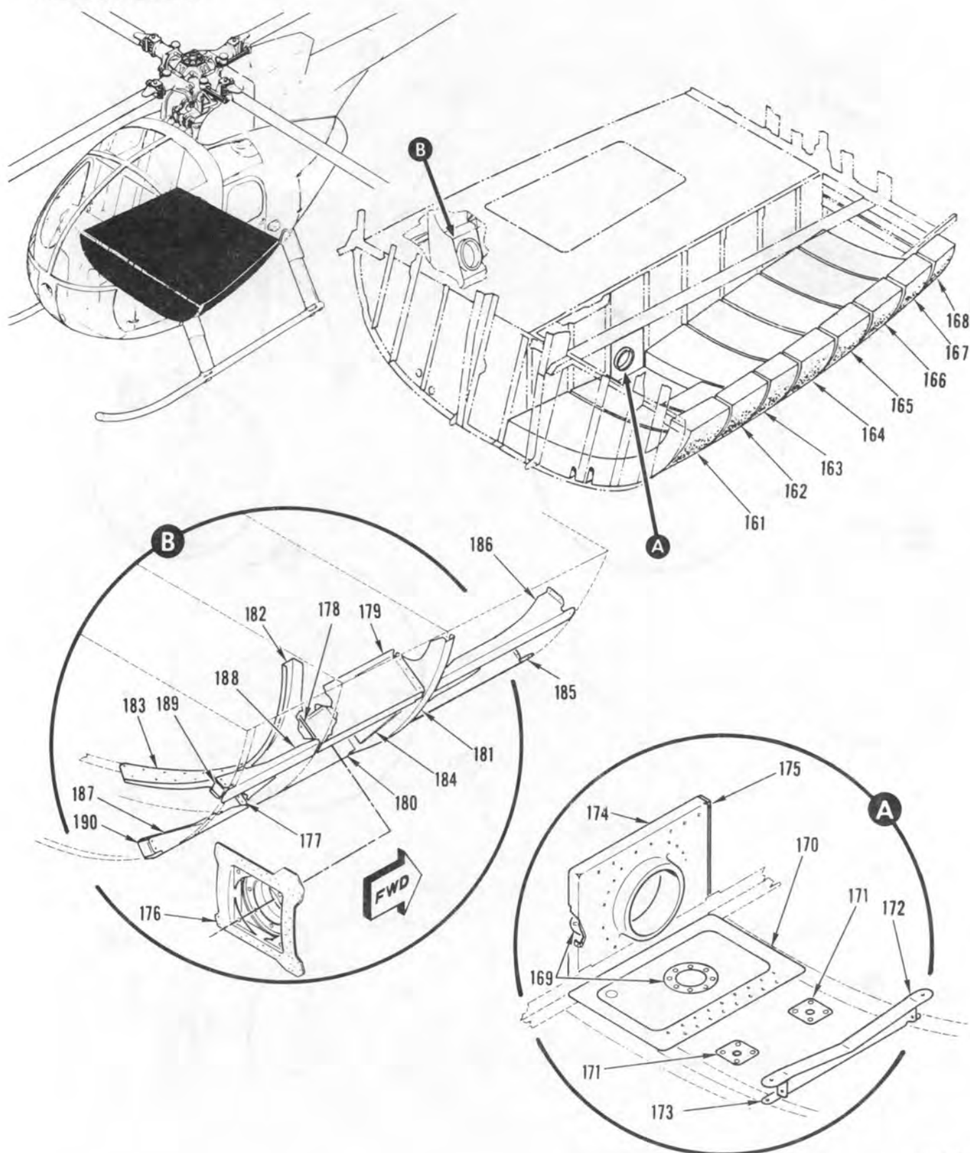
FIGURE 6. LOWER SECTION INSTALLATION, FUSELAGE STRUCTURE (SHEET 5 OF 5)
