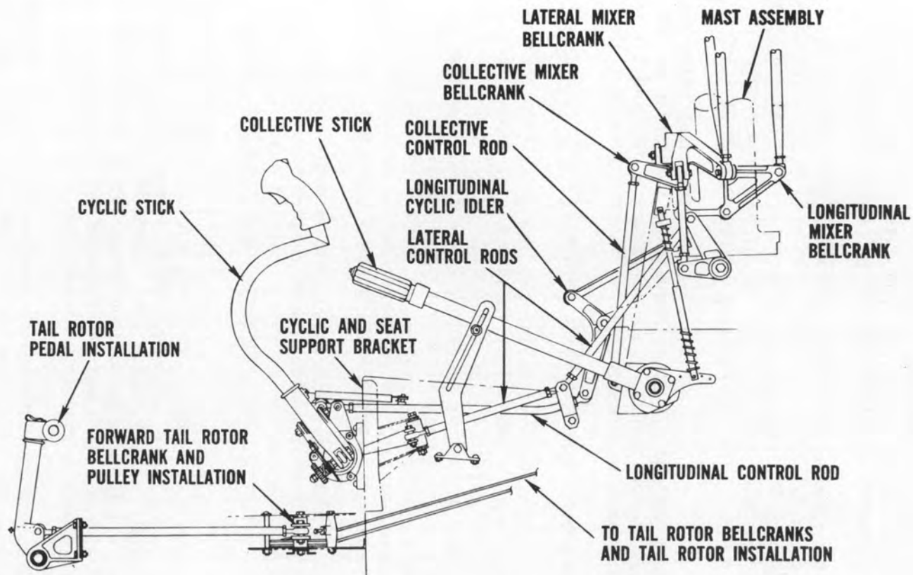
FLIGHT CONTROLS (SIDE VIEW)
