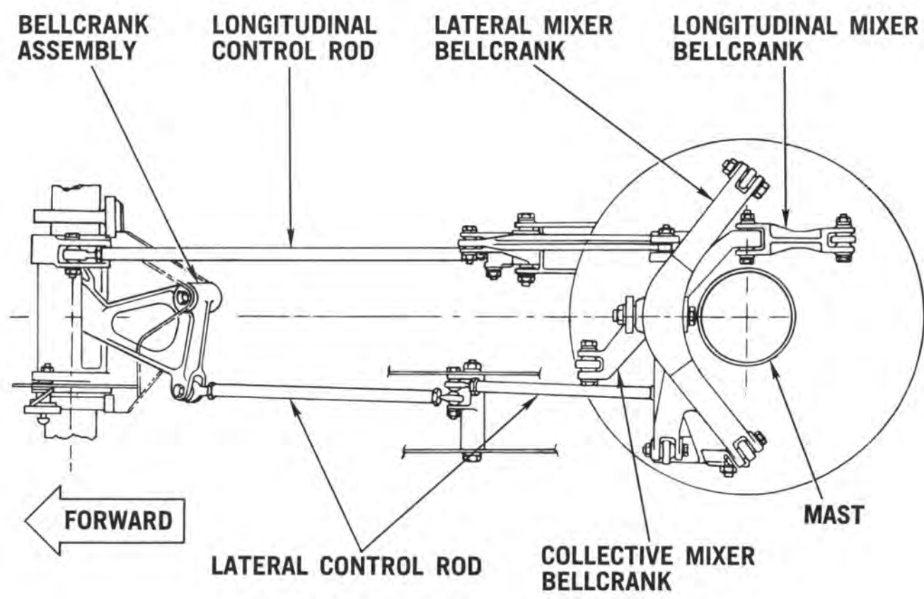
FLIGHT CONTROLS INSTALLATION TOP VIEW
