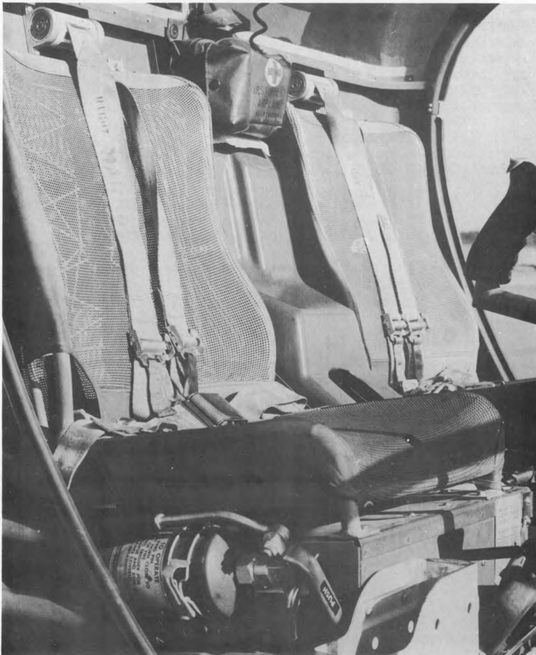
Cockpit View Shows the Location of the Fire Extinguisher, Safety Kit and the Seat Belt-Shoulder Harness Installation: (fig. 2-16)
