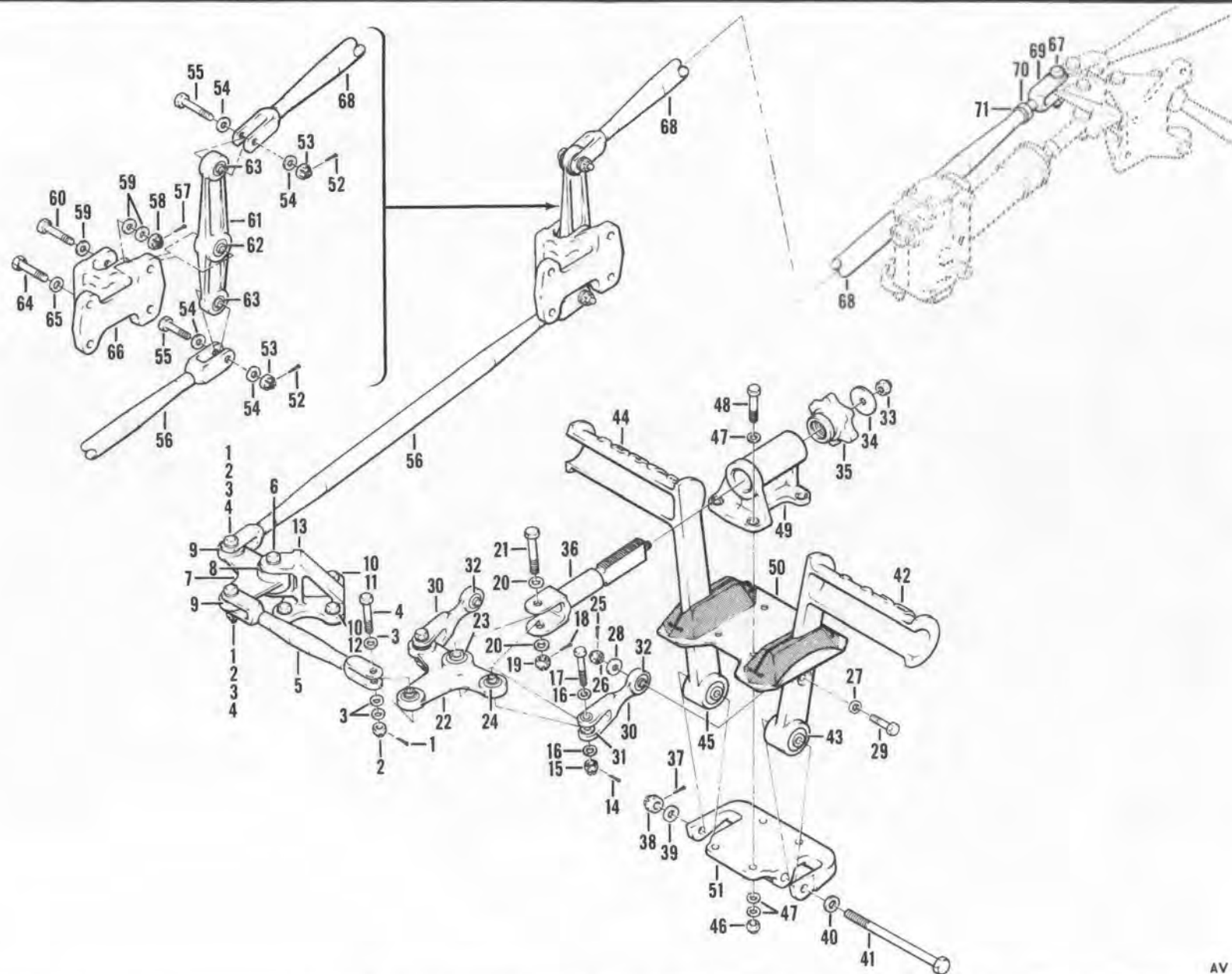
Figure 246. Controls Installation, Anti-Torque, Forward Section
