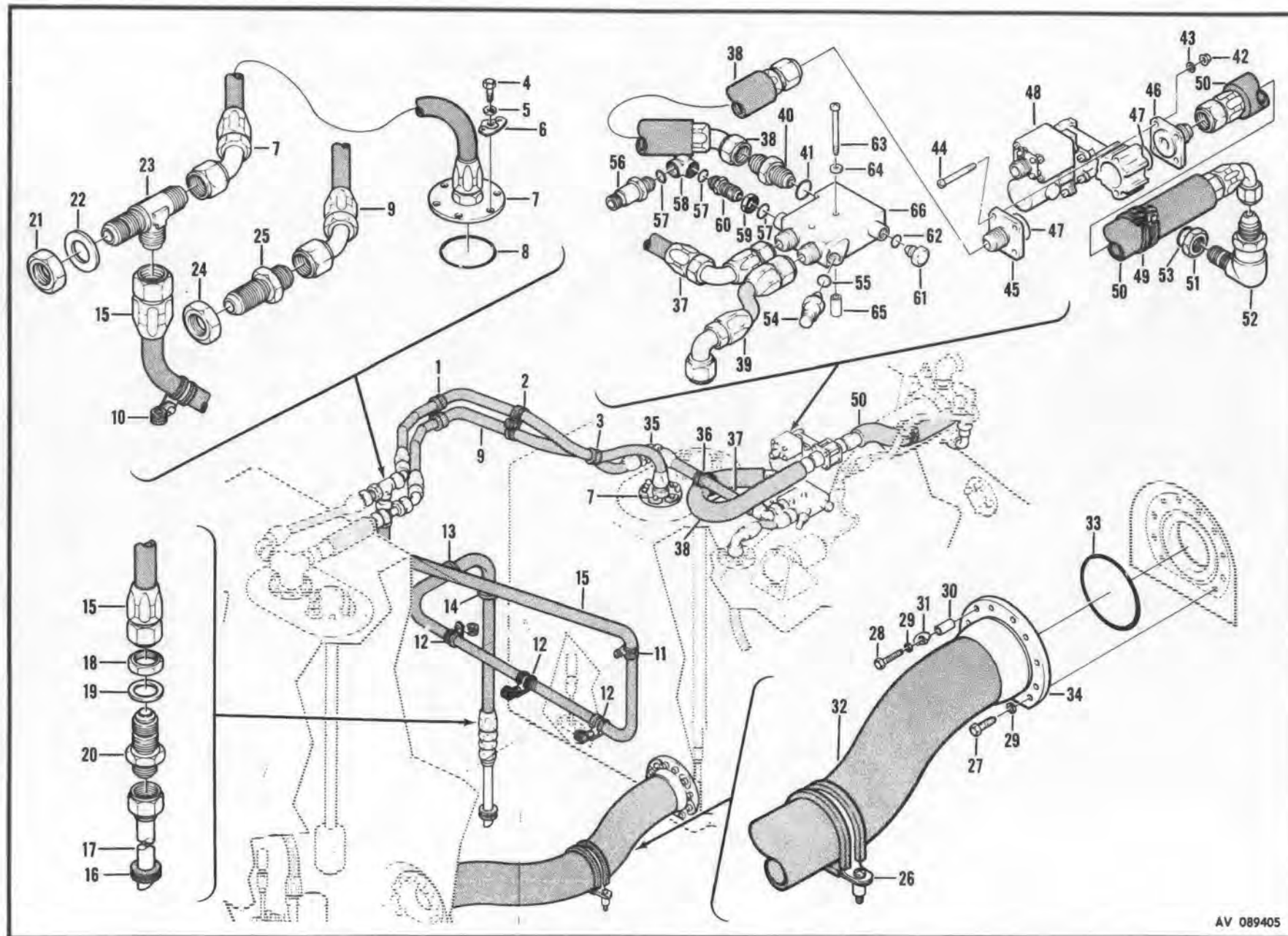
Figure 225. Retrofit Kit, Crashworthy Fuel System
