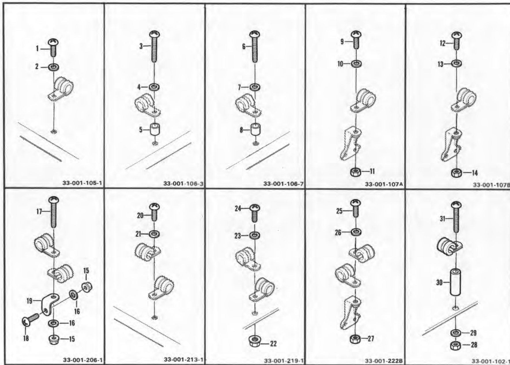
Figure 215E. Modification, Equipment Installation, Aft Section
