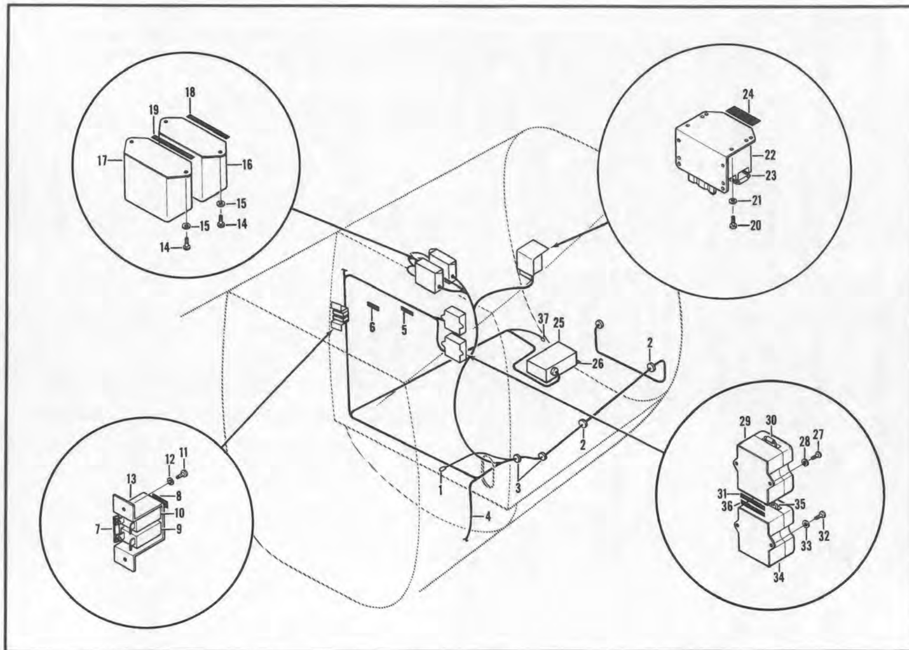
Figure 170A. Modification, Electrical Equipment Installation, Forward Section
