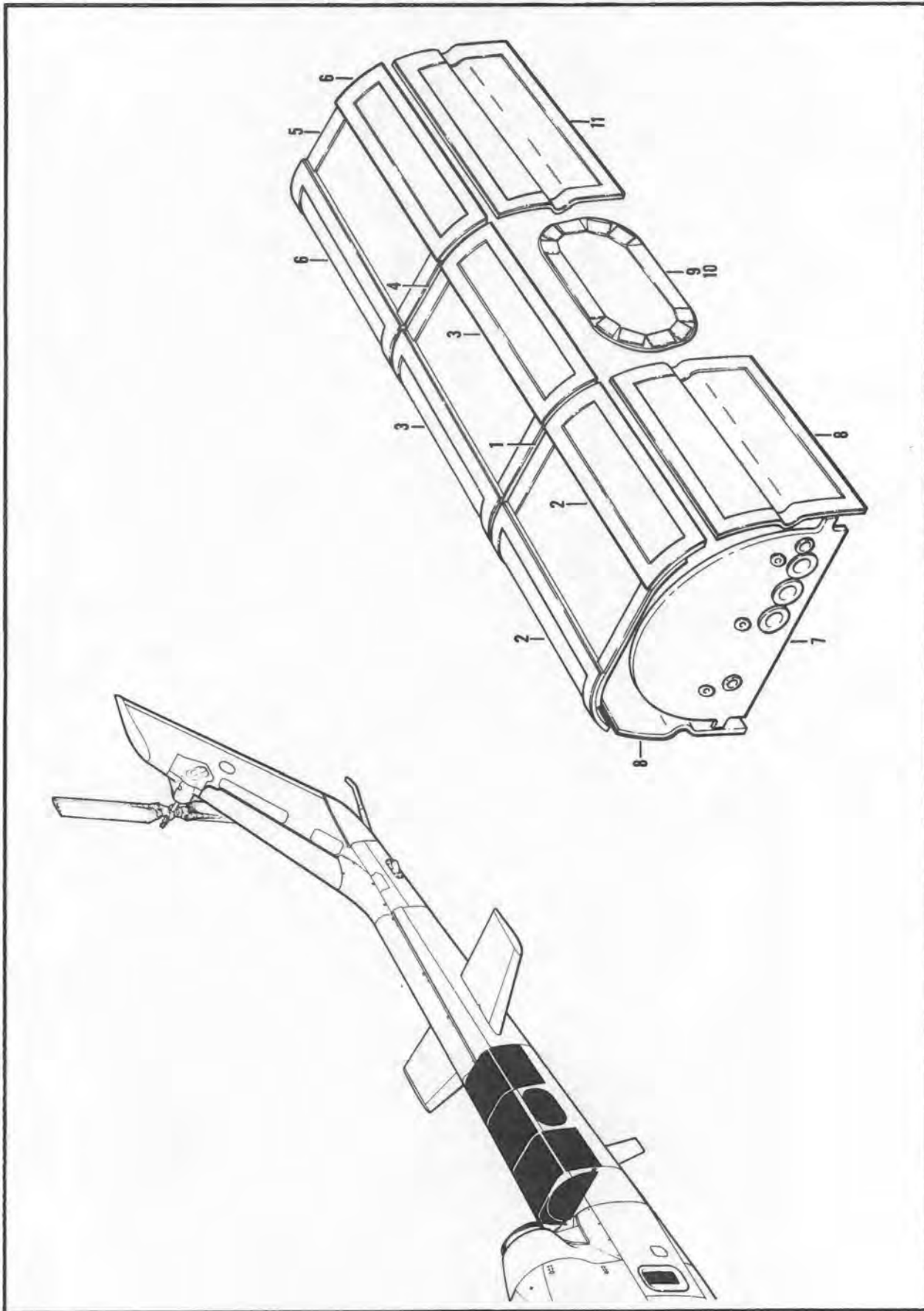
Figure 268B. Modification, Avionics Cooling, Tail Boom
