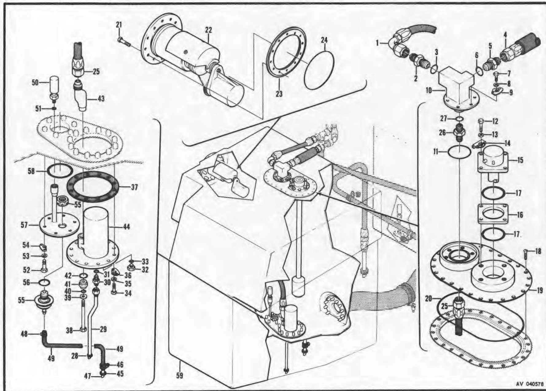
Figure 220. Fuel System Installation (Crashworthy)
