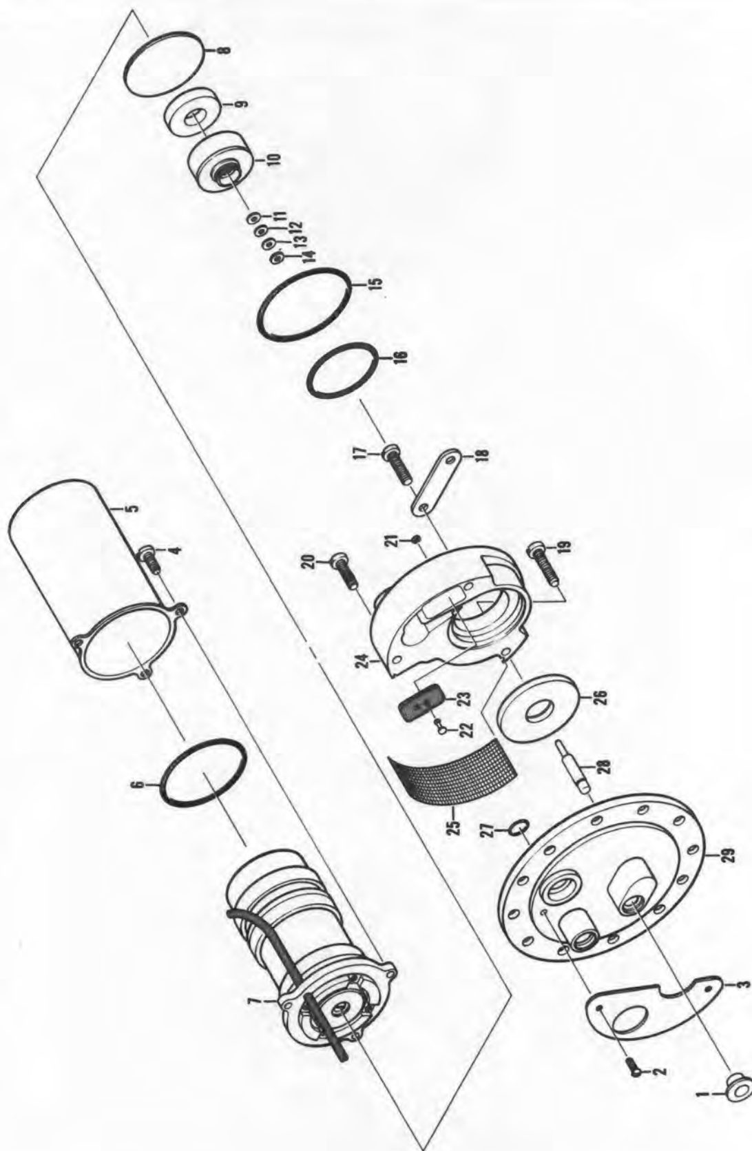
Figure 228A. Pump Assembly, Fuel
