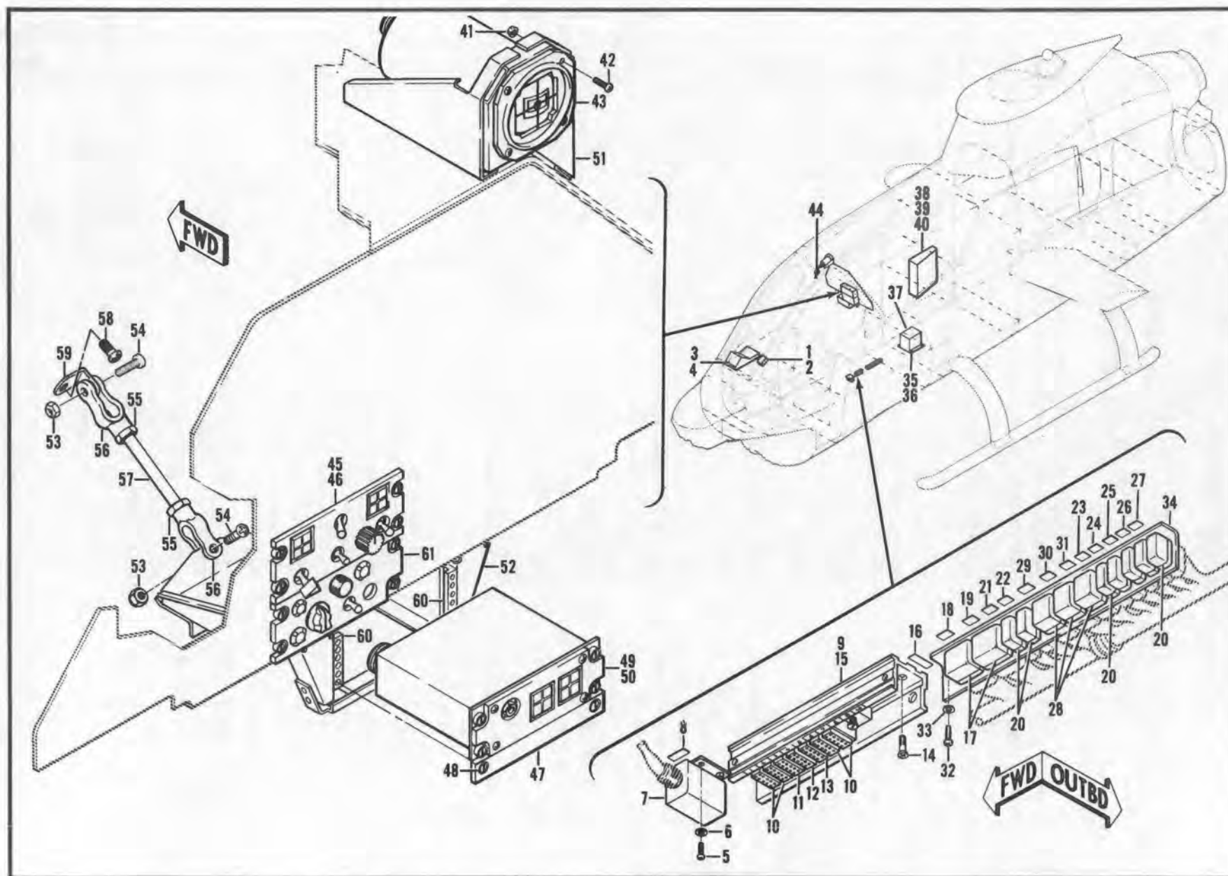
Figure 209B. Modification, Electrical Installation, Armament
