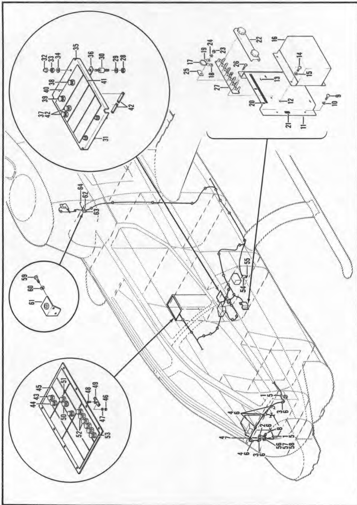
Figure 165A. Modification, Electrical Equipment Installation, Forward Section
