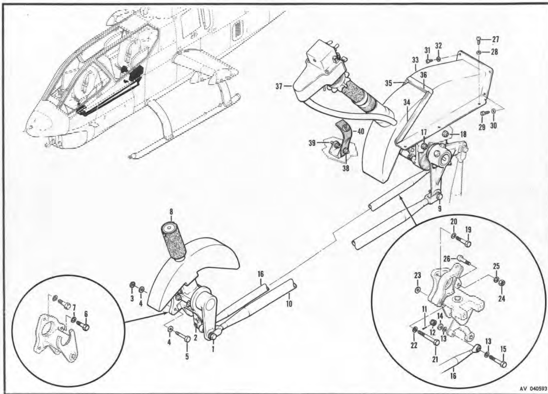
Figure 241. Controls Installation, Collective, Forward Section
