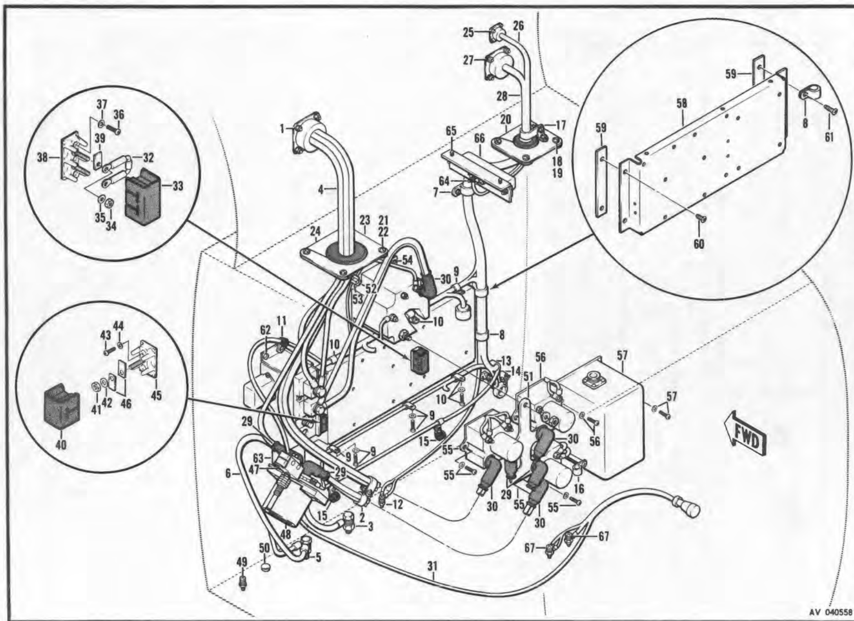
Figure 197. Equipment Installation, Aft Compartment, Forward Section
