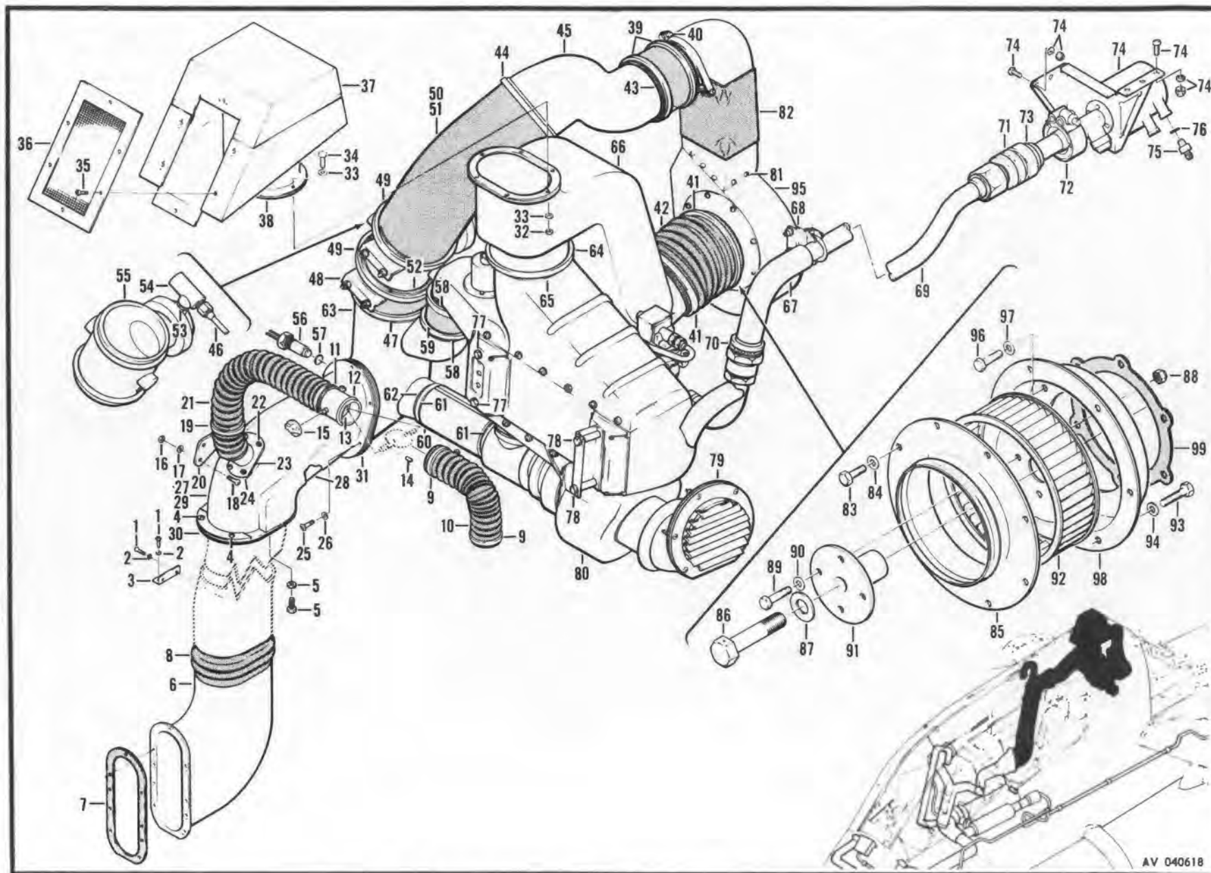
Figure 267. Air Distribution Installation, Heating and Ventilation
