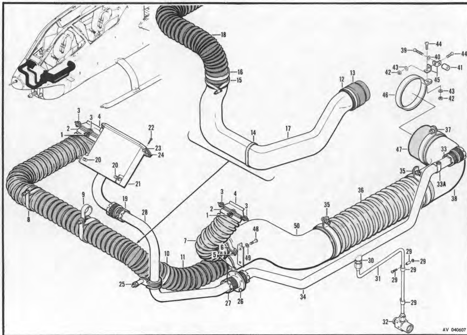
Figure 255. Air Distribution Installation, Heating and Ventilation
