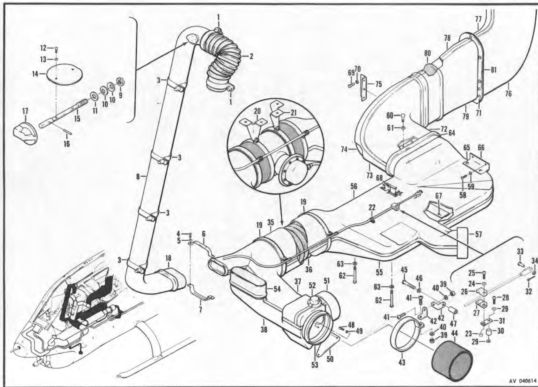
Figure 262. Air Distribution Installation, Heating and Ventilation
