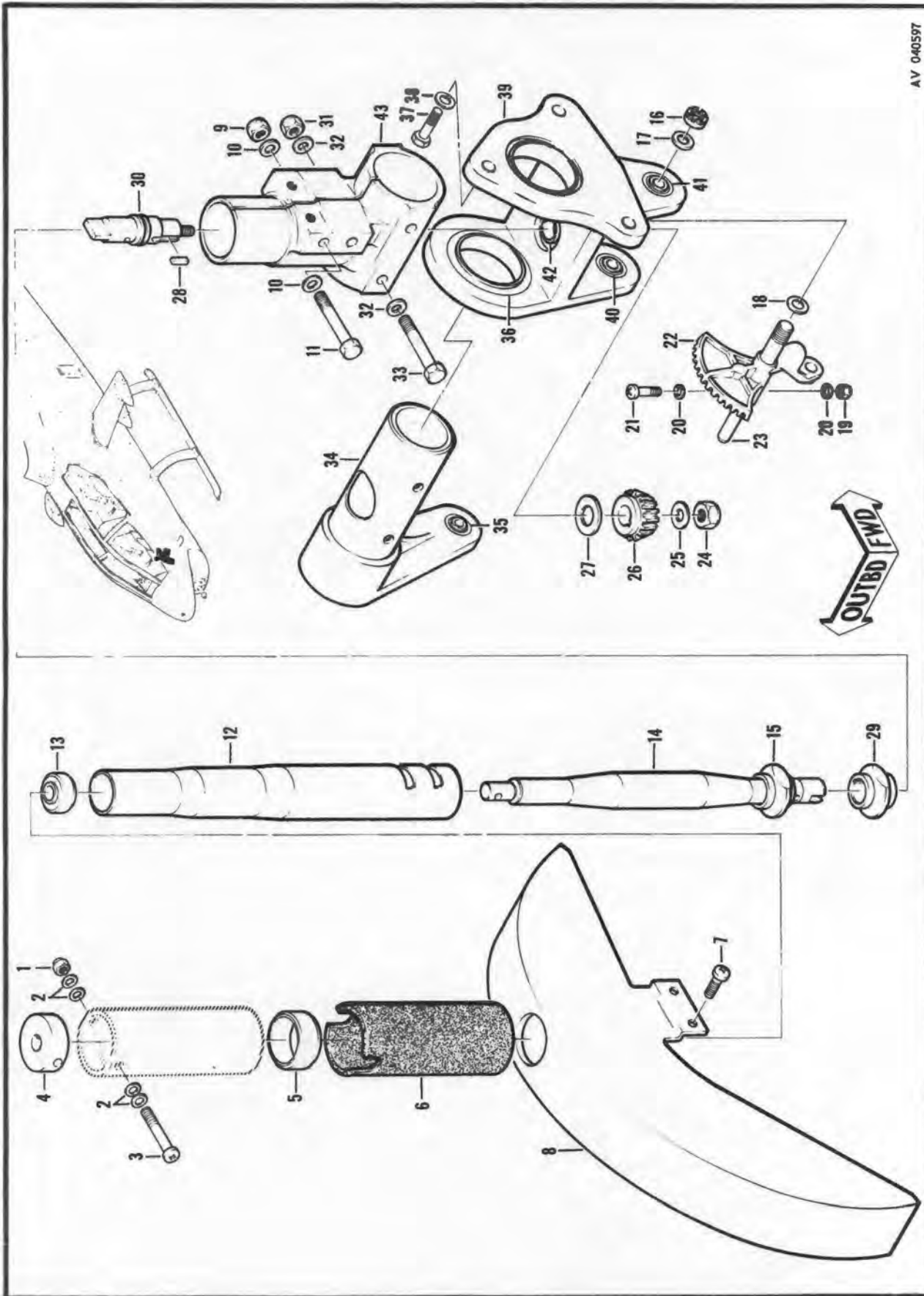
Figure 245. Stick Assembly, Gunner's Collective
