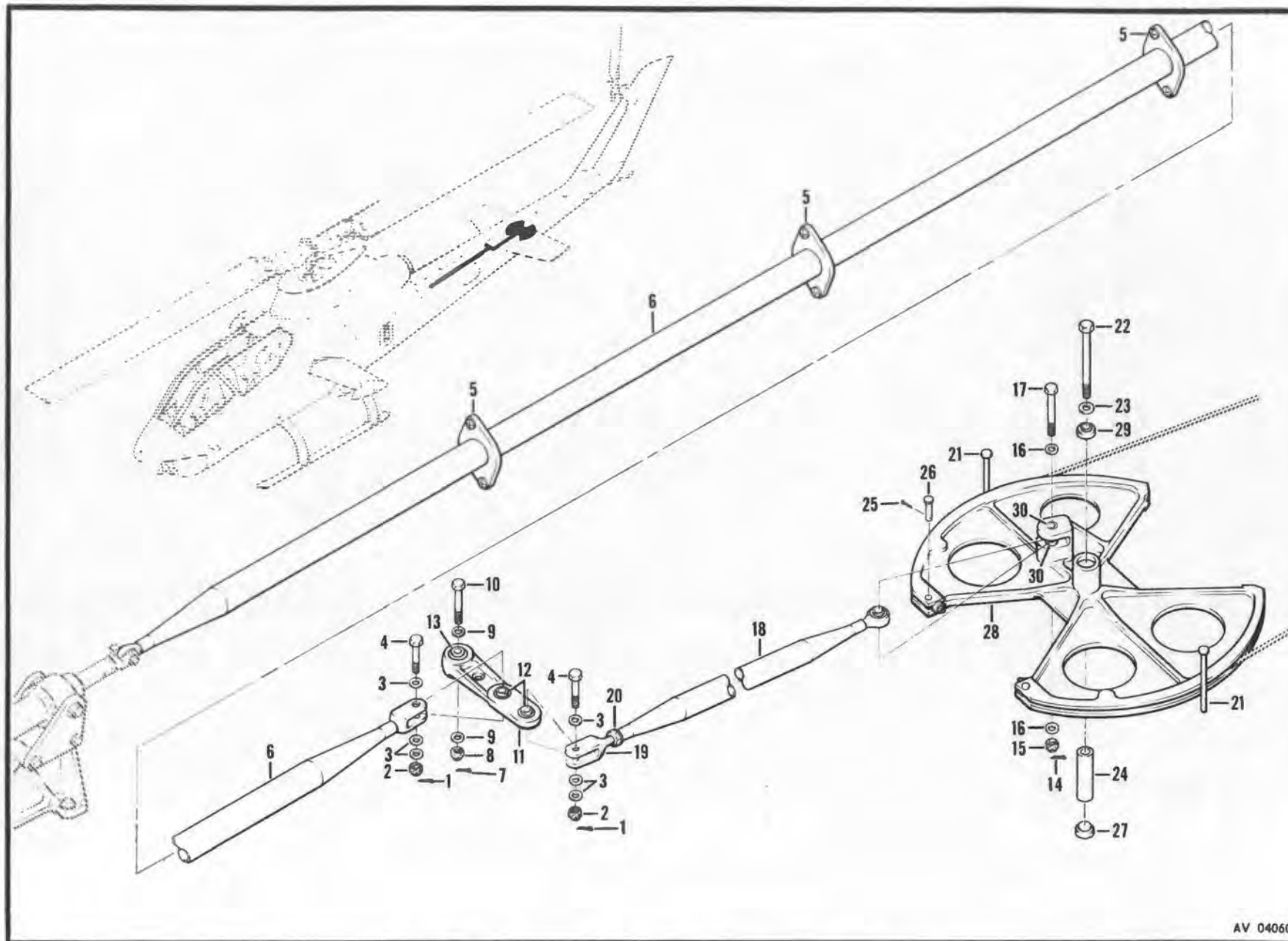
Figure 250. Controls Installation, Anti-Torque, Aft Section
