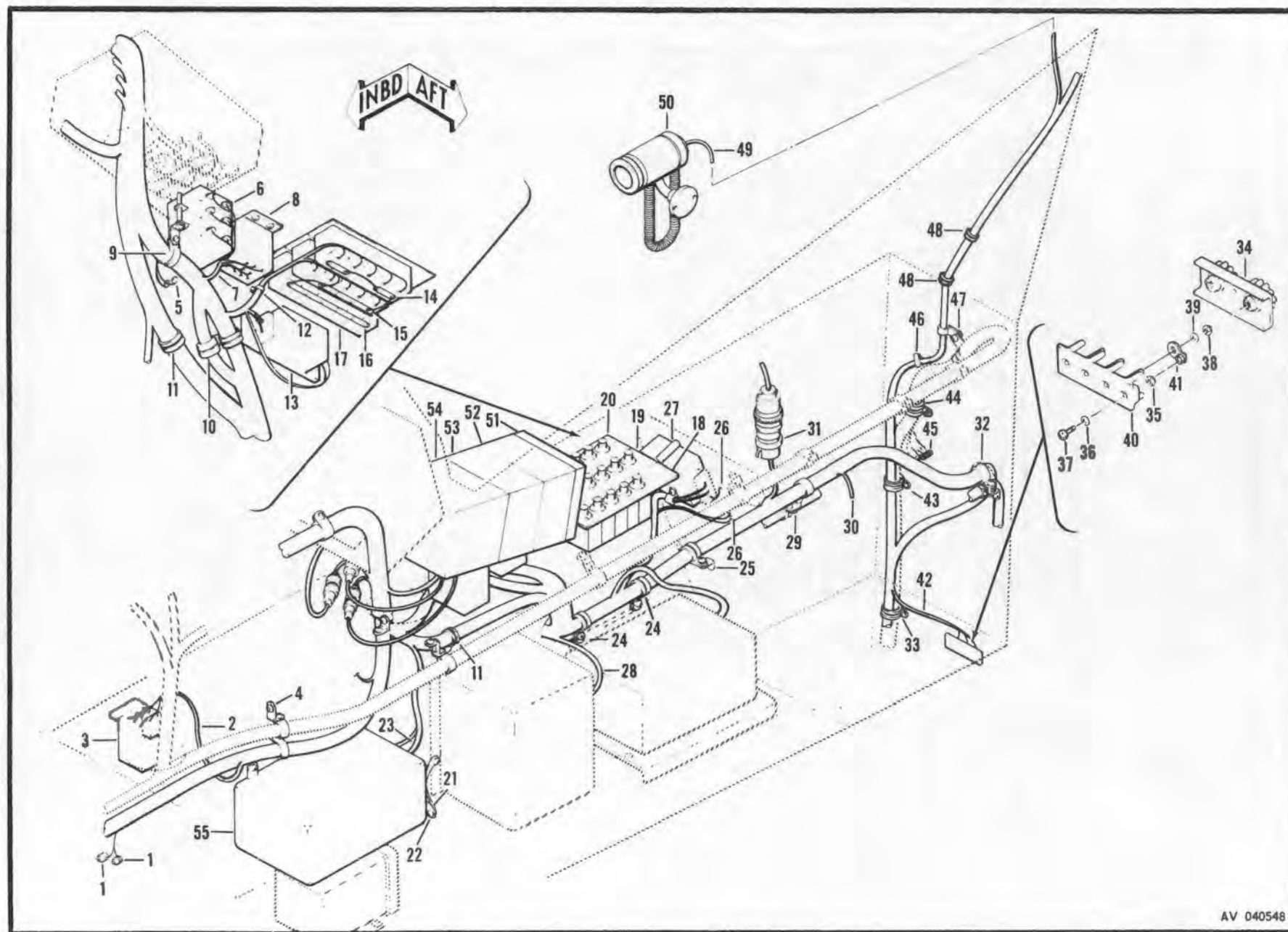
Figure 184. Electrical Installation, Pilot's Section
