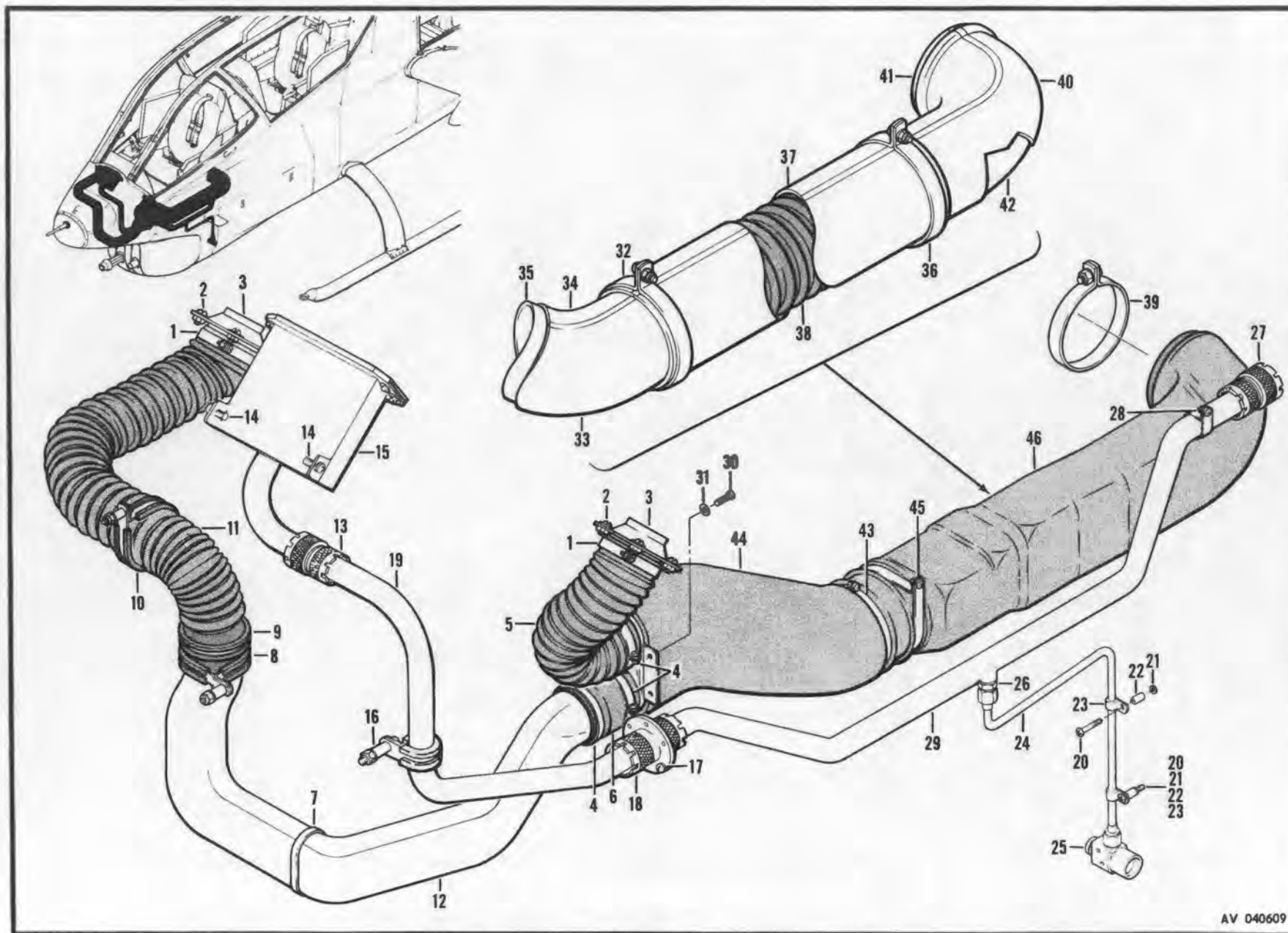
Figure 256. Air Distribution Installation, Heating and Ventilation
