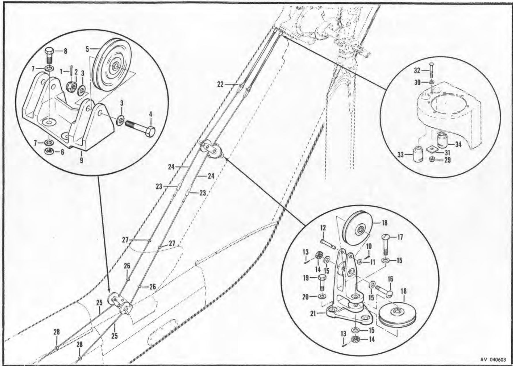
Figure 251. Controls Installation, Anti-Torque, Aft Section
