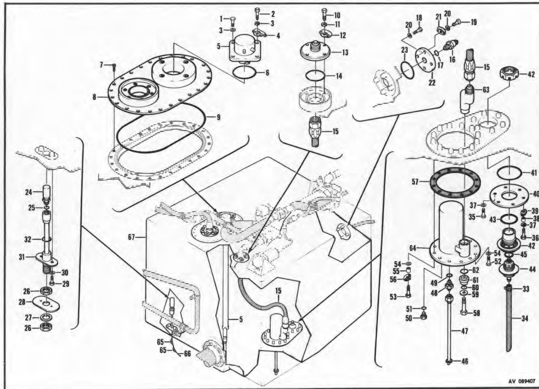
Figure 227. Retrofit Kit, Crashworthy Fuel System
