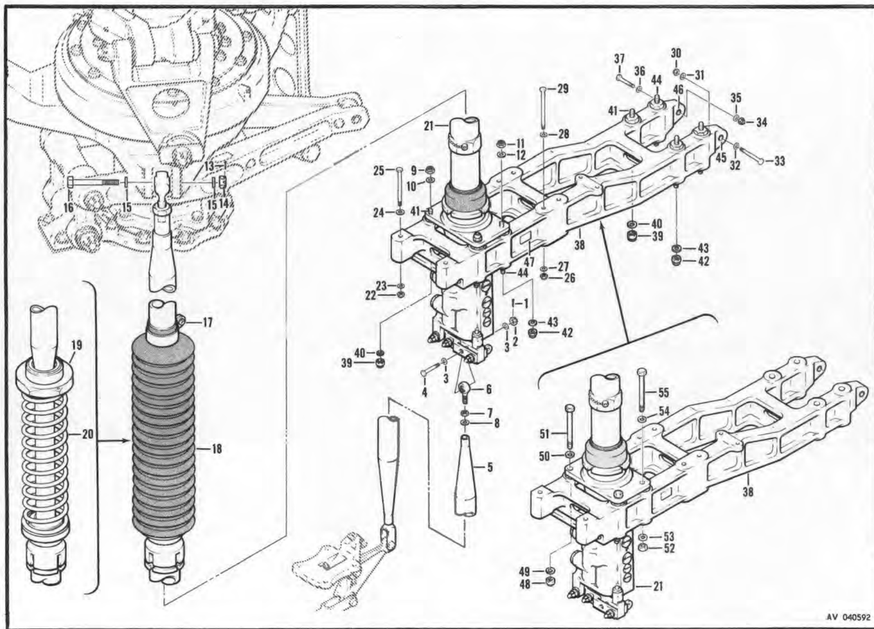
Figure 240. Controls Installation, Lateral Cyclic Controls
