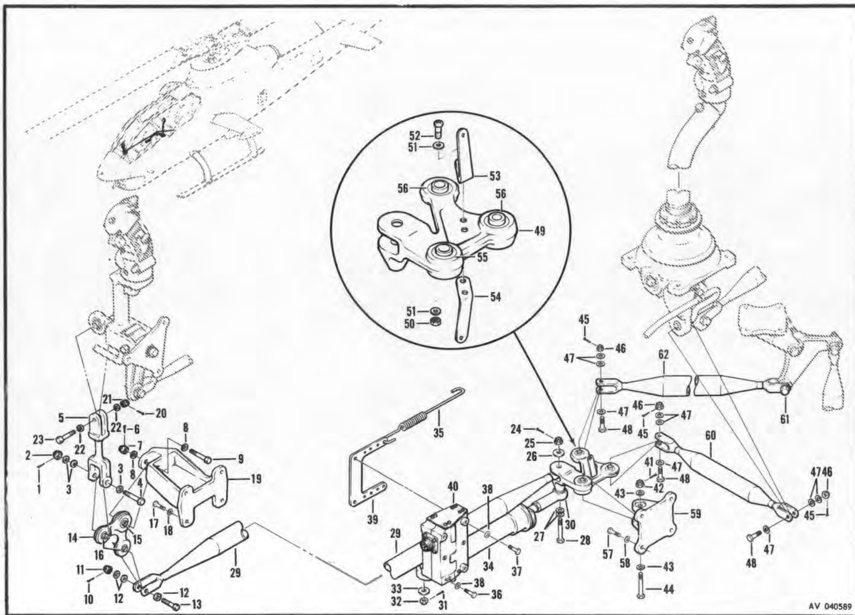
Figure 237. Controls Installation, Lateral Cyclic Controls
