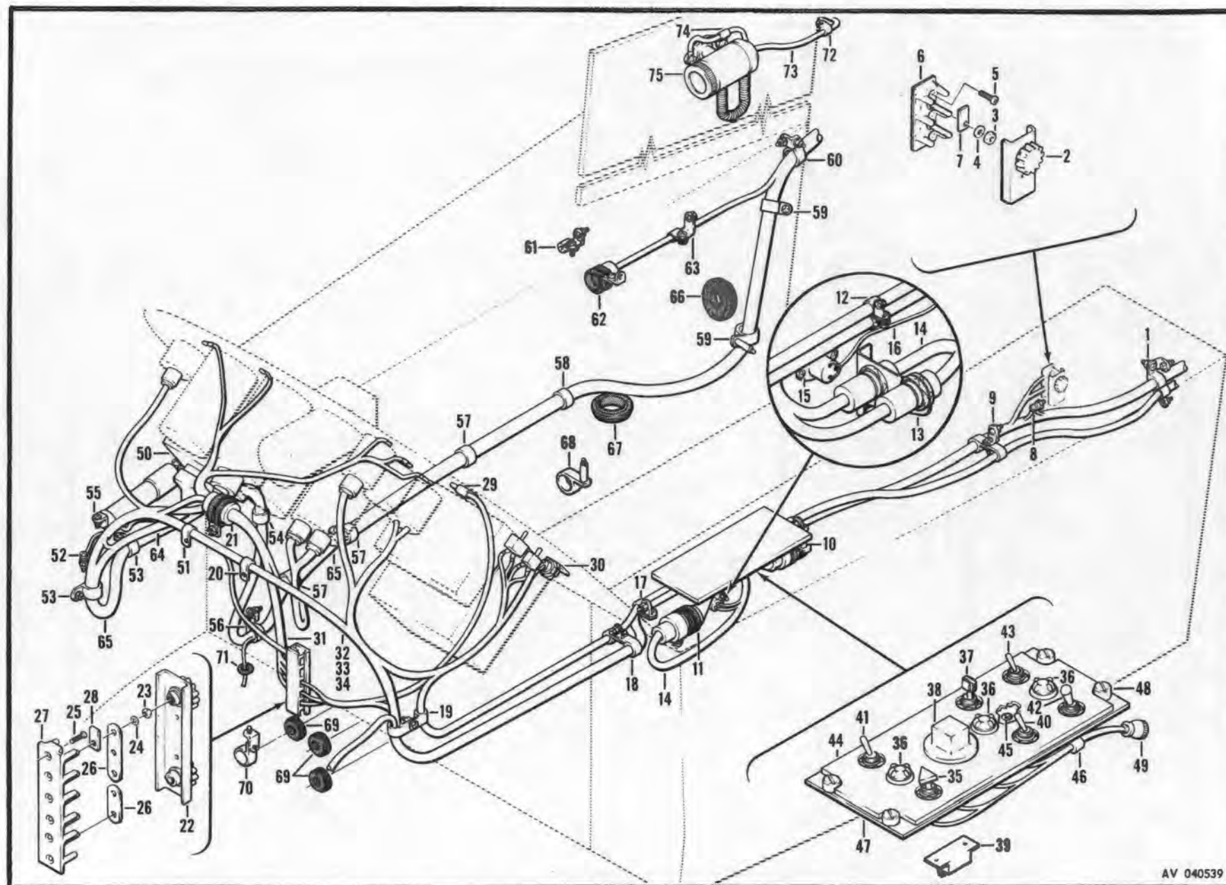
Figure 175. Electrical Installation, Gunner's Section
