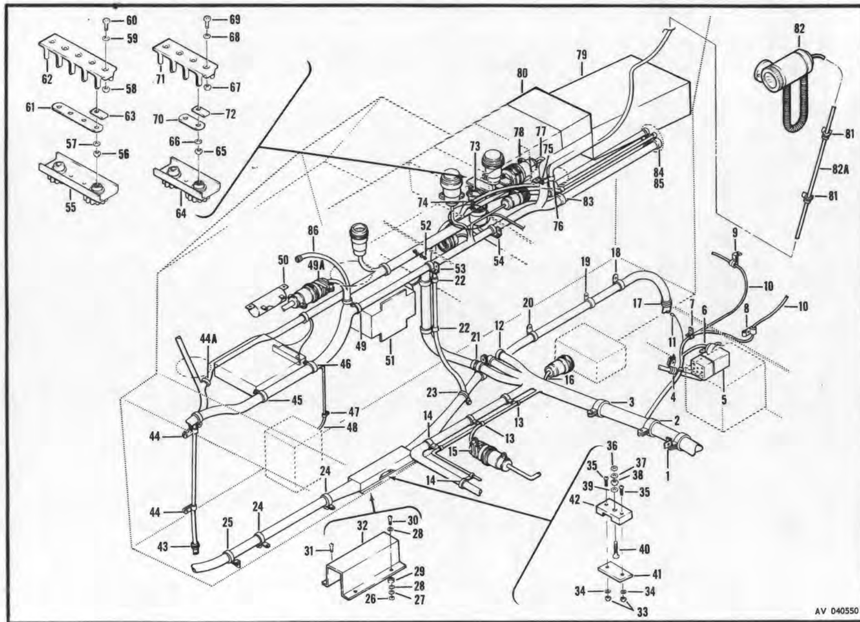
Figure 186. Electrical Installation, Pilot's Section
