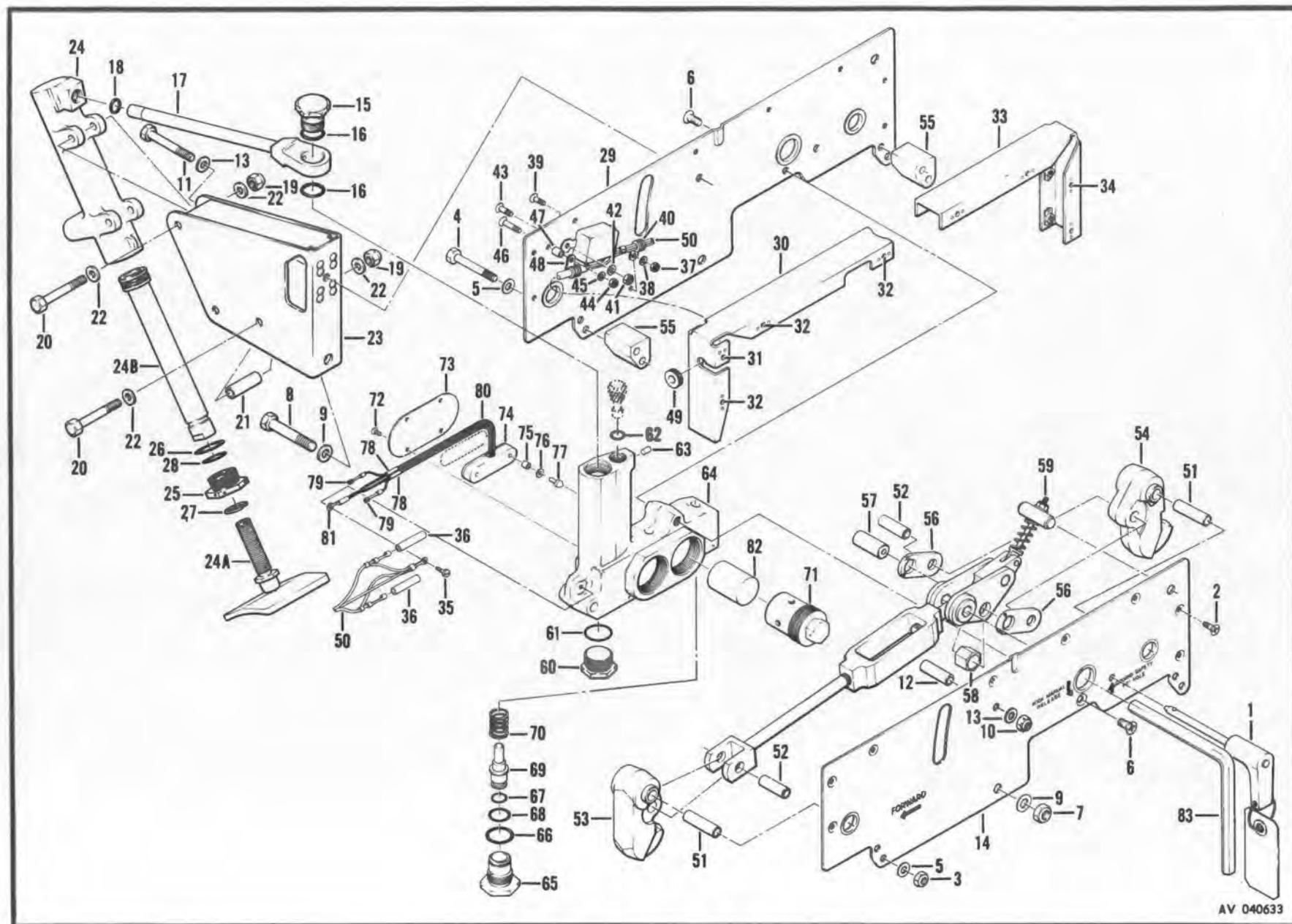
Figure 281. Rack, External Stores Ejector
