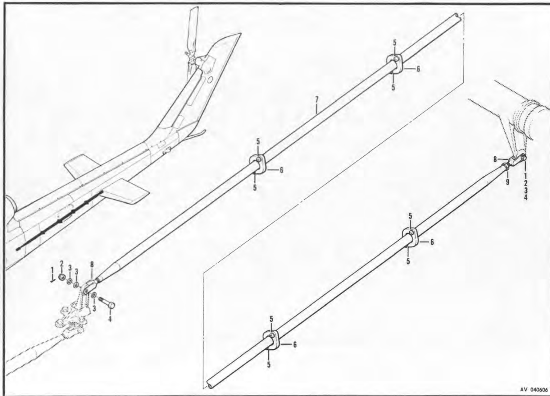
Figure 254. Controls Installation, Elevator, Aft Section
