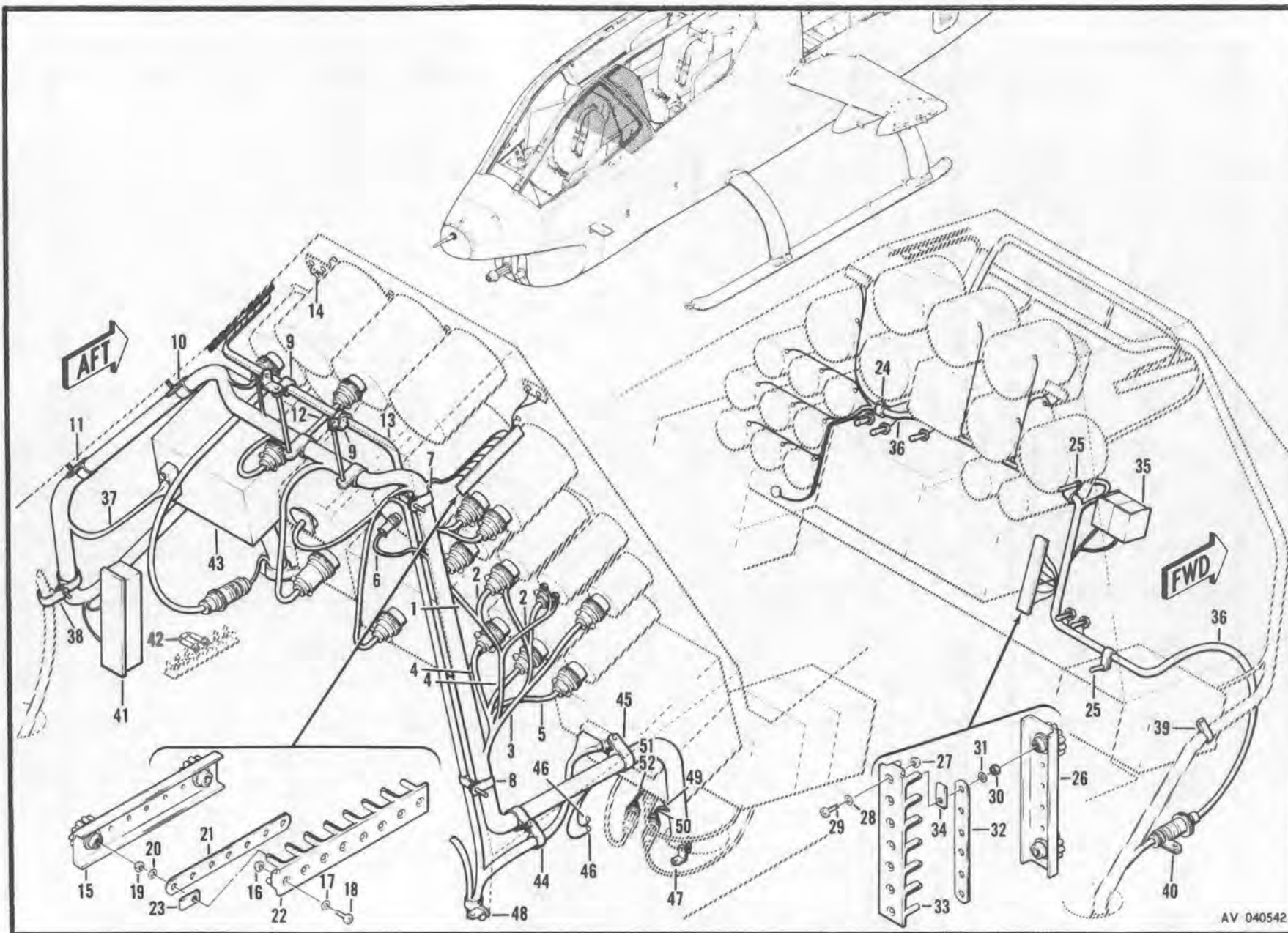
Figure 178. Electrical Installation, Pilot's Section
