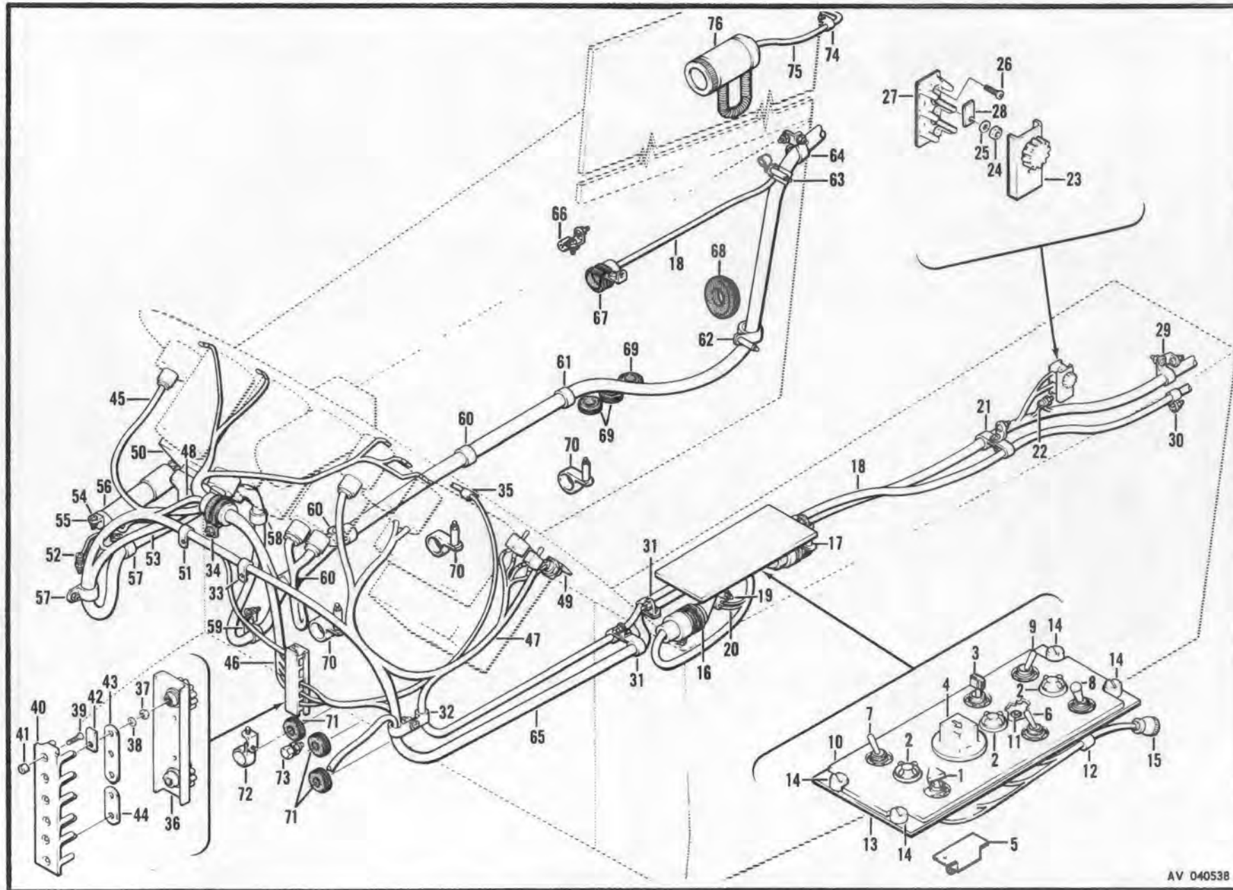
Figure 174. Electrical Installation, Gunner's Section
