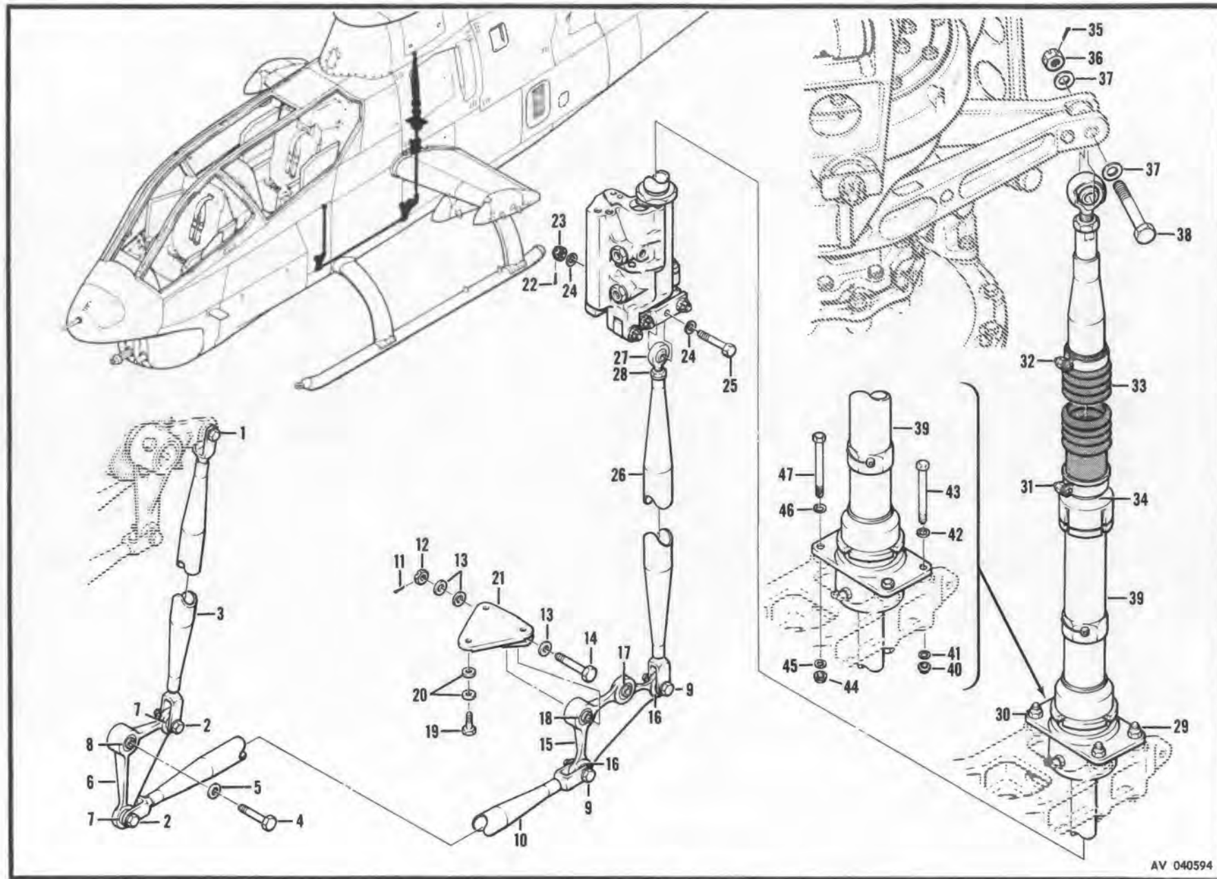
Figure 242. Controls Installation, Collective, Aft Section
