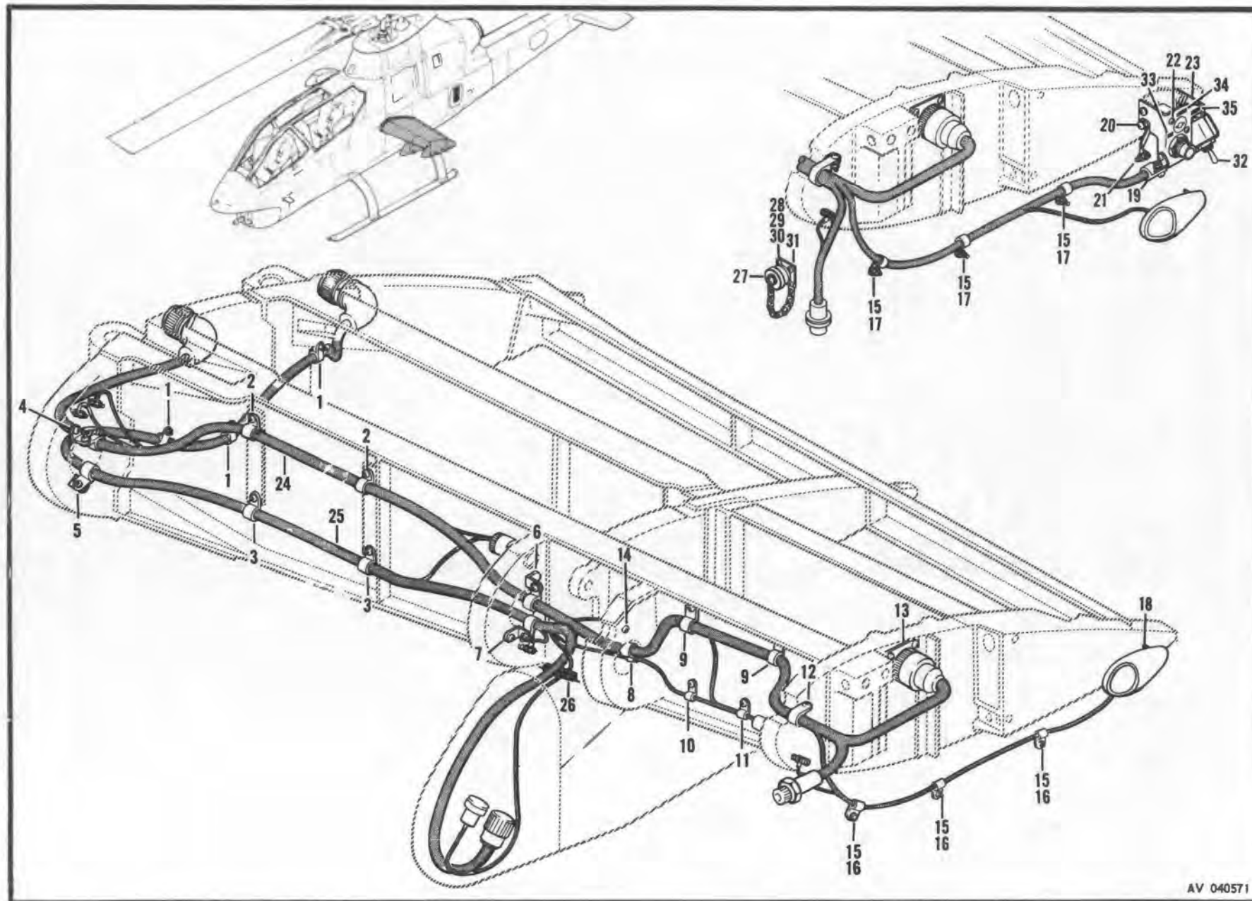
Figure 213. Electrical Installation, Wing
