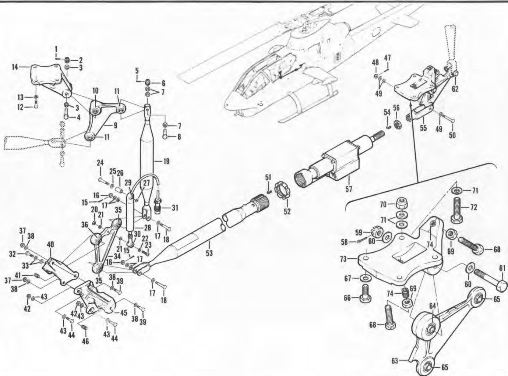
Figure 239. Controls Installation, Lateral Cyclic Controls
