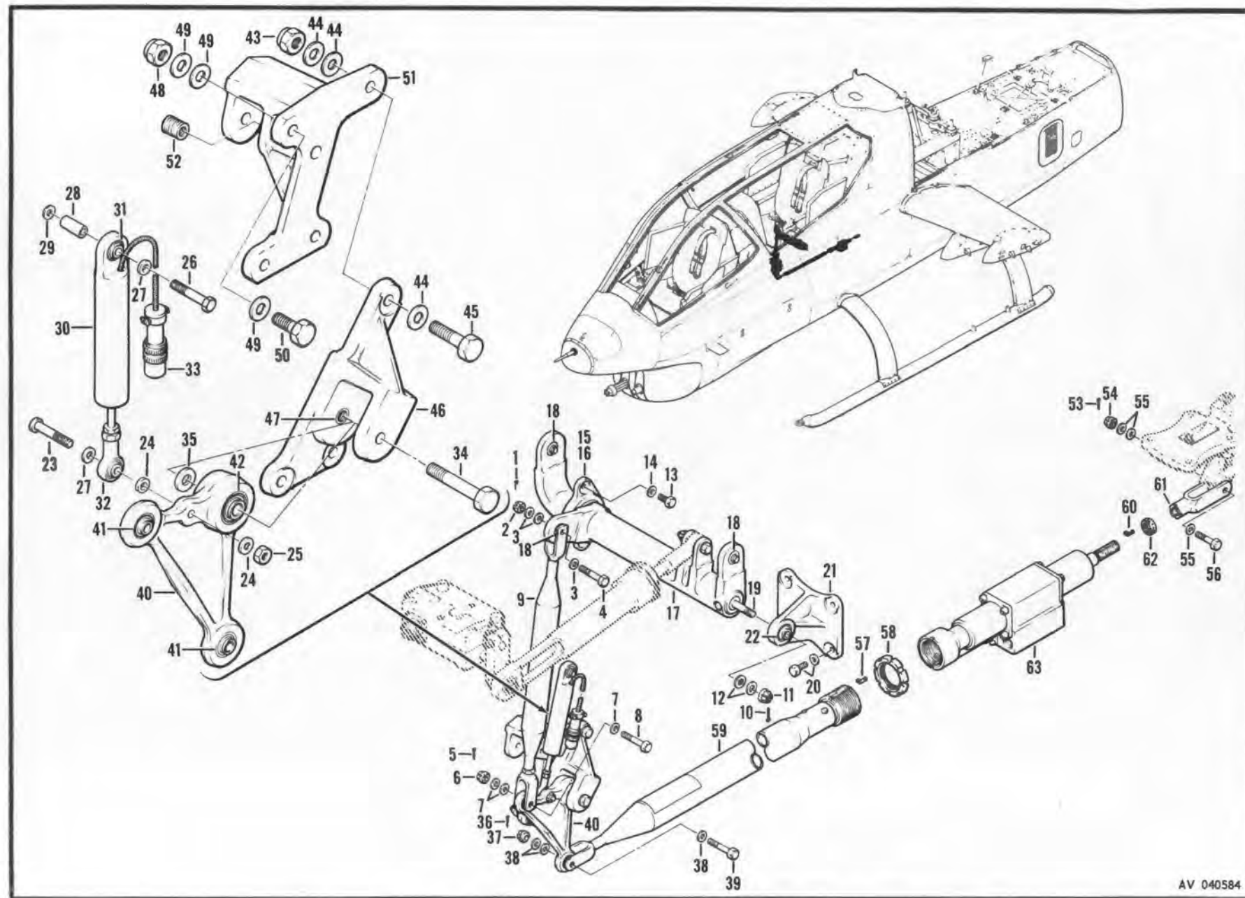
Figure 232. Controls Installation, Fore and Aft, Cyclic Controls, Center Section
