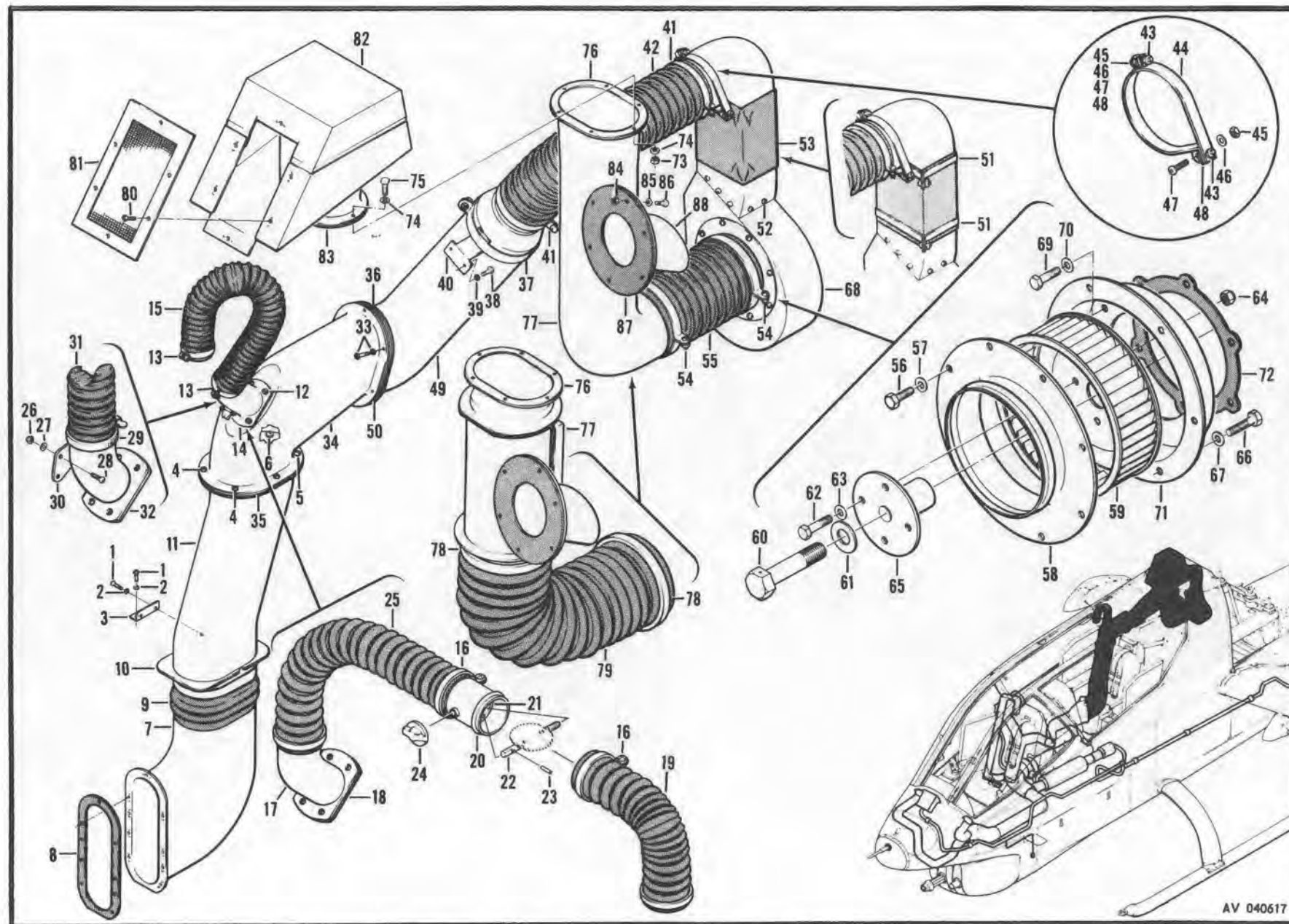
Figure 266. Air Distribution Installation, Heating and Ventilation
