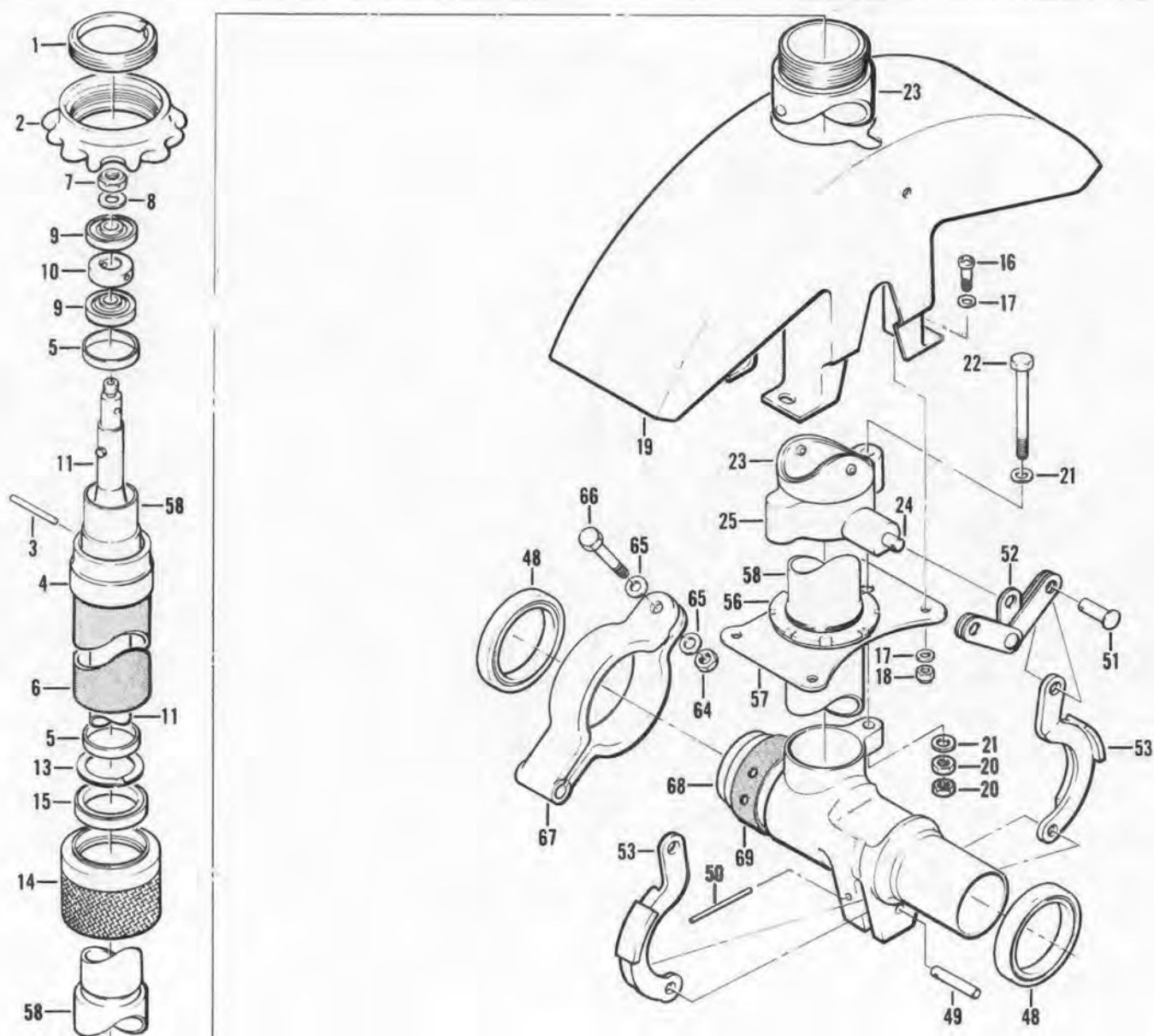
Figure 244. Controller, Grip Assembly (Sheet 1 of 2)
