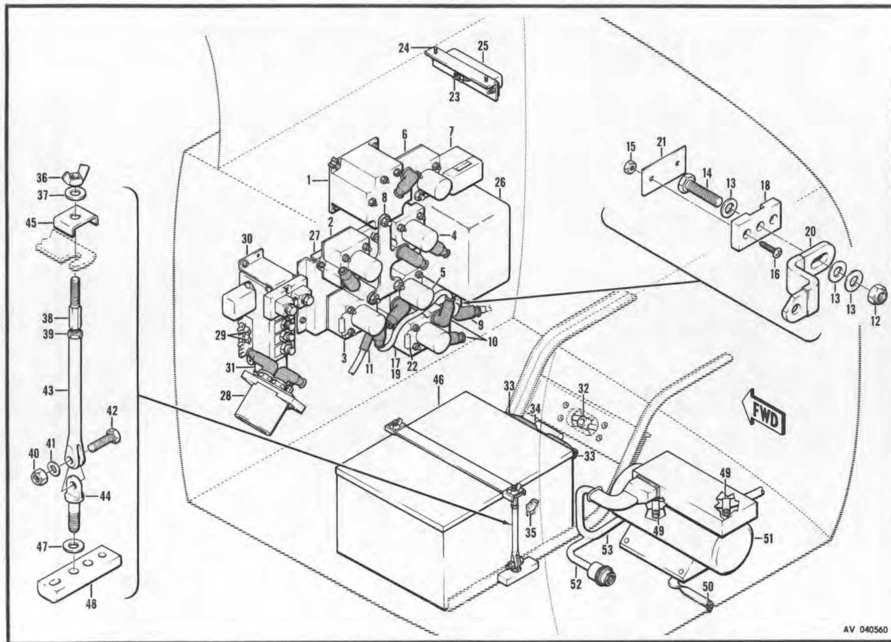
Figure 199. Equipment Installation, Aft Compartment, Forward Section
