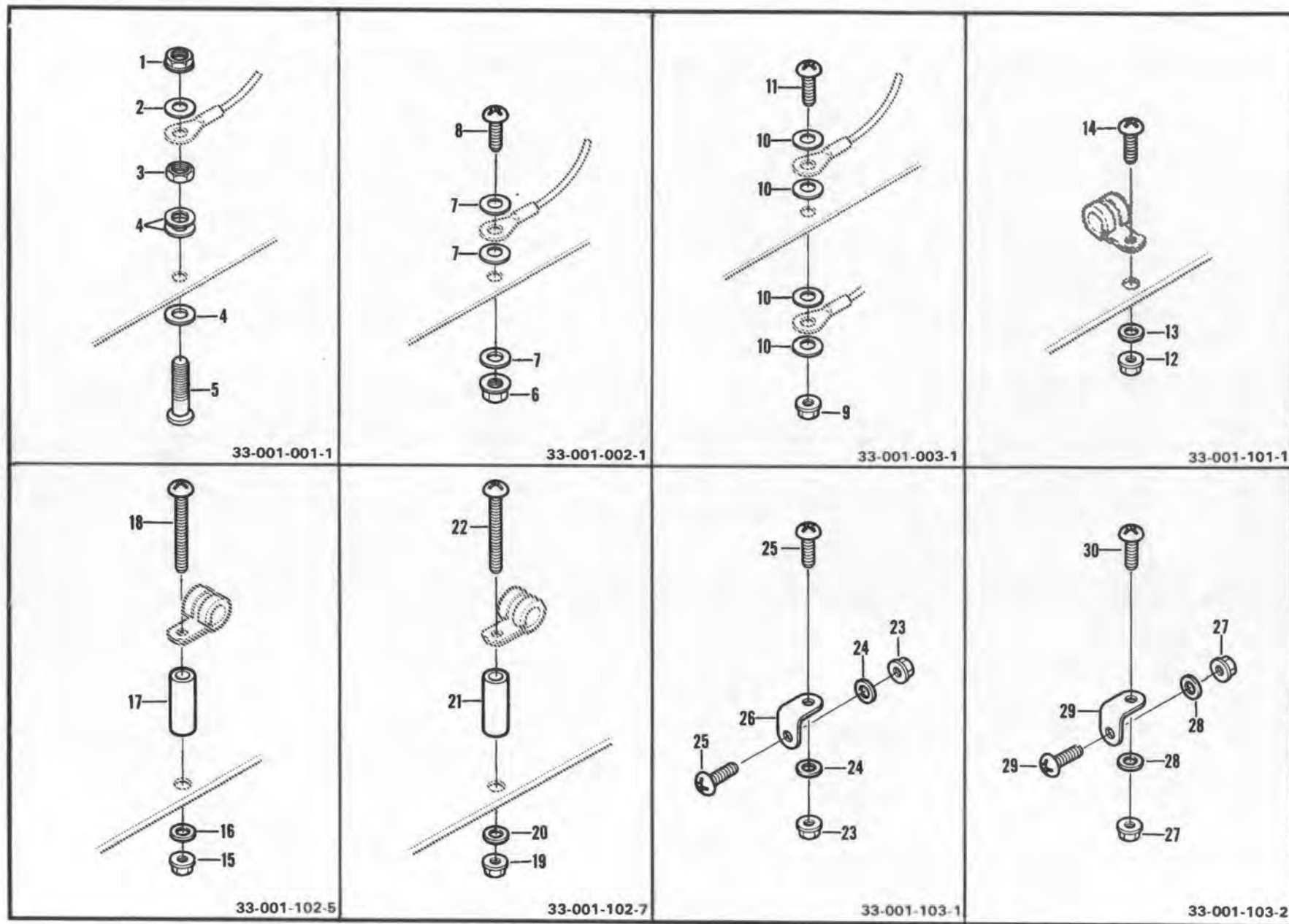
Figure 215D. Modification, Equipment Installation, Aft Section
