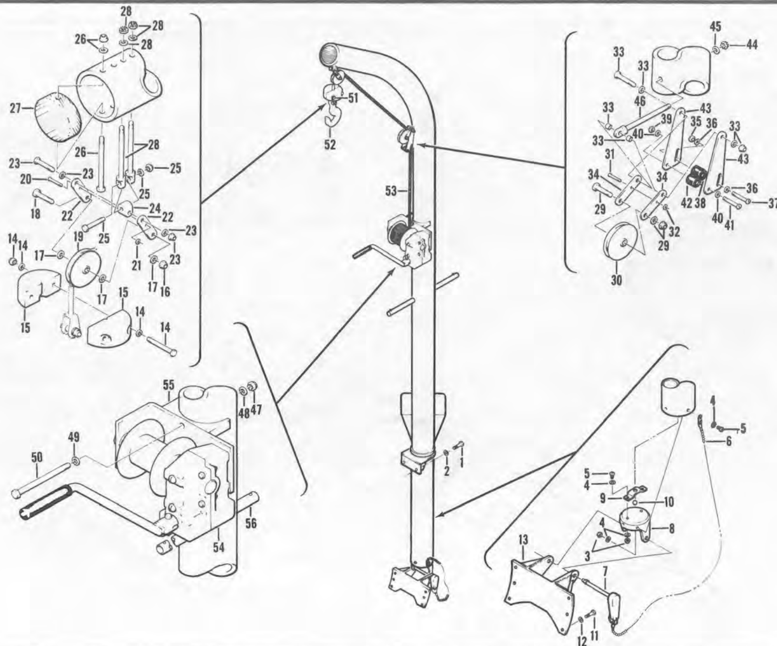
Figure A8. Airframe Tools
