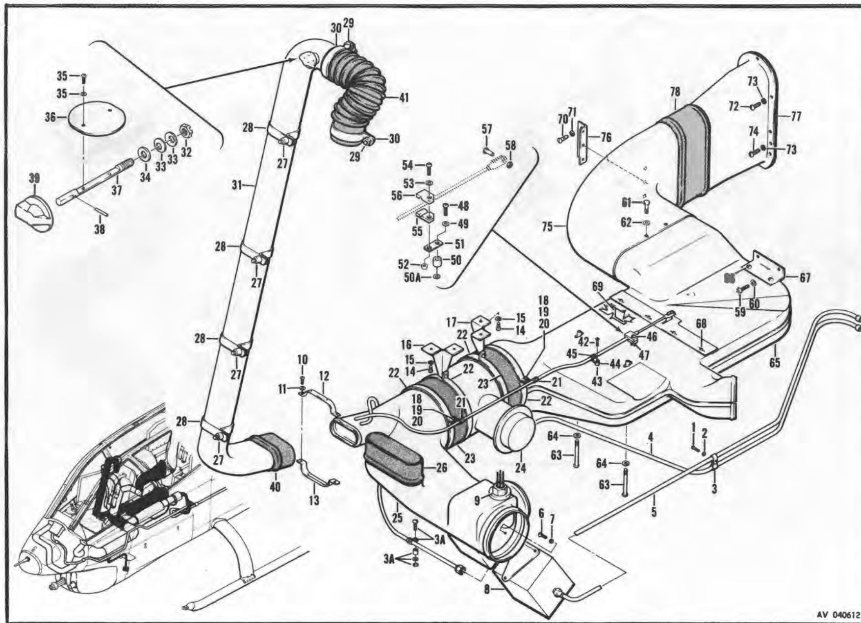
Figure 261. Air Distribution Installation, Heating and Ventilation (Sheet 1 of 2)
