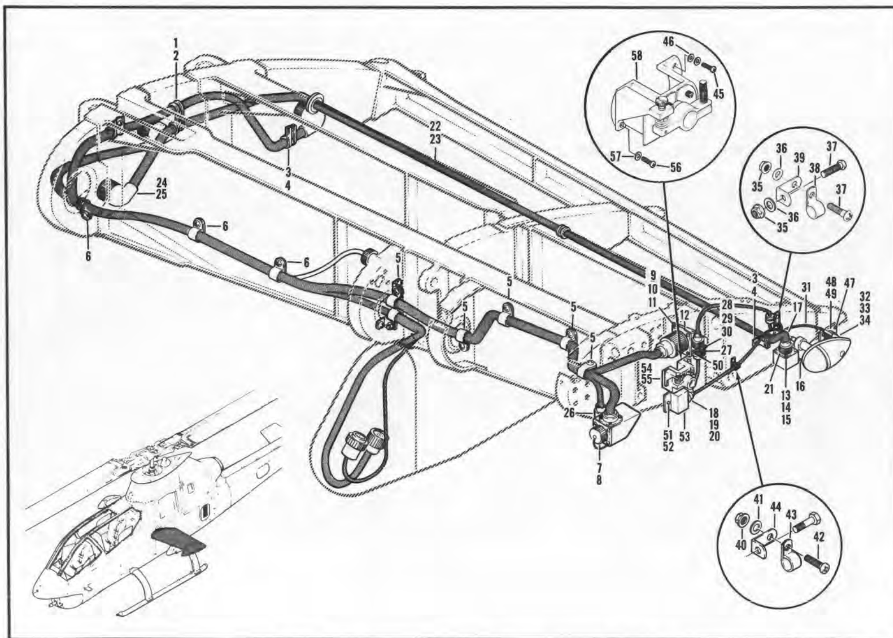
Figure 213A. Modification, Electrical Equipment, Wing L.H. and R.H.
