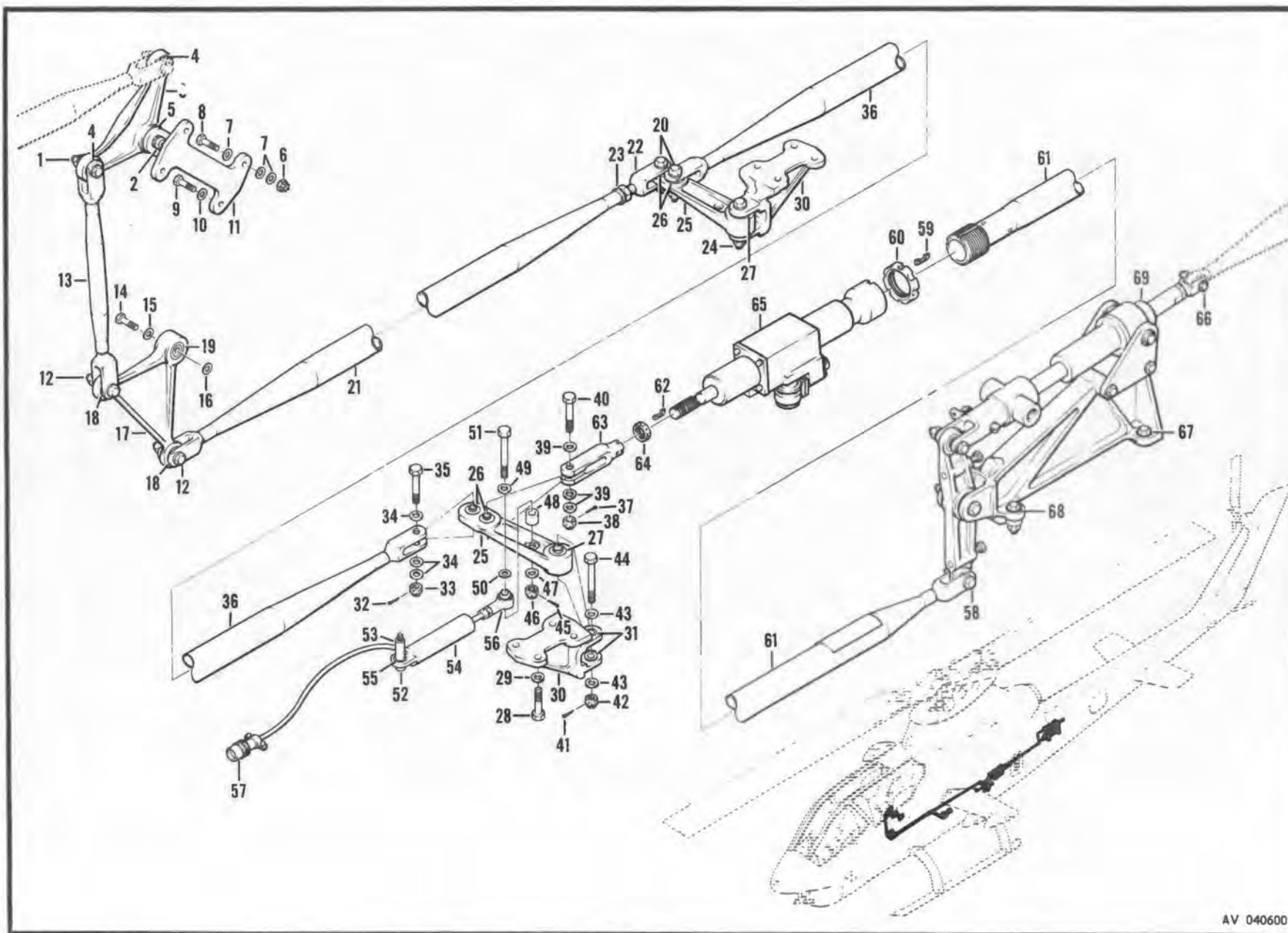
Figure 248. Controls Installation, Anti-Torque, Forward Section
