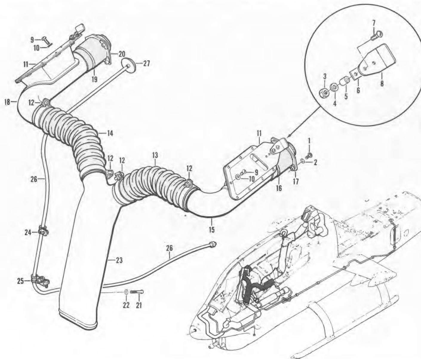
Figure 265. Air Distribution Installation, Heating and Ventilation
