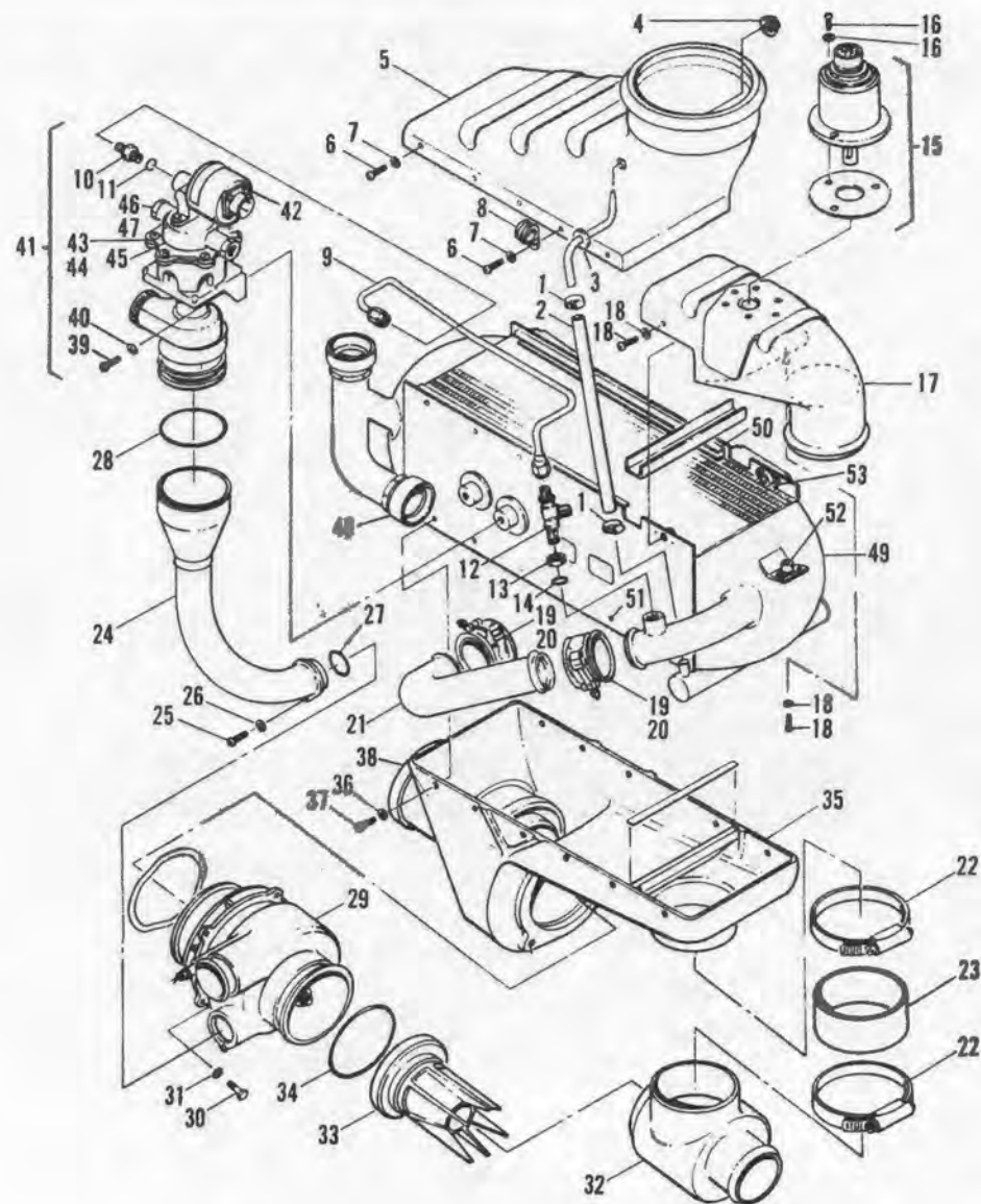
Figure 275. Environmental Control Unit and Regulating Valve Assembly
