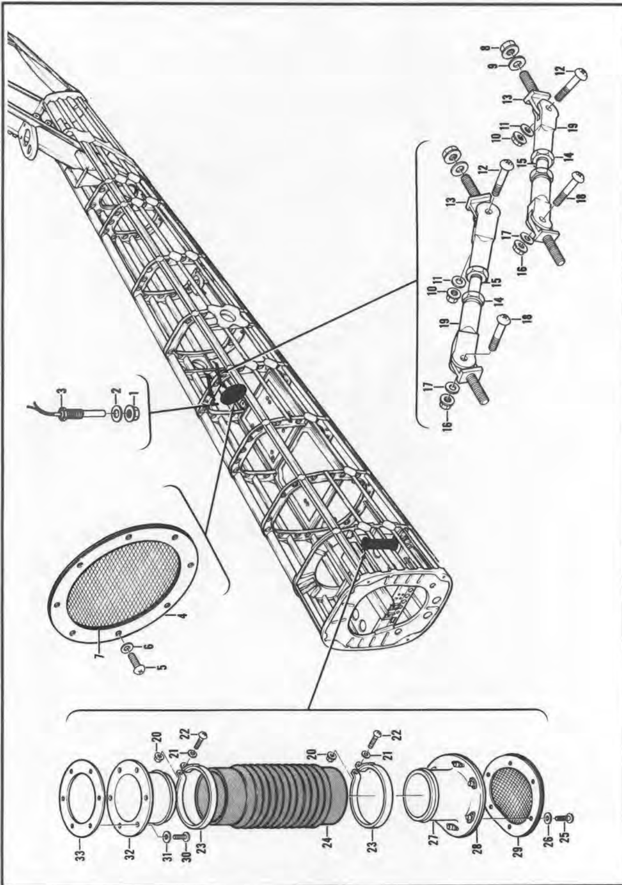
Figure 268C. Modification, Avionics Cooling, Tail Boom
