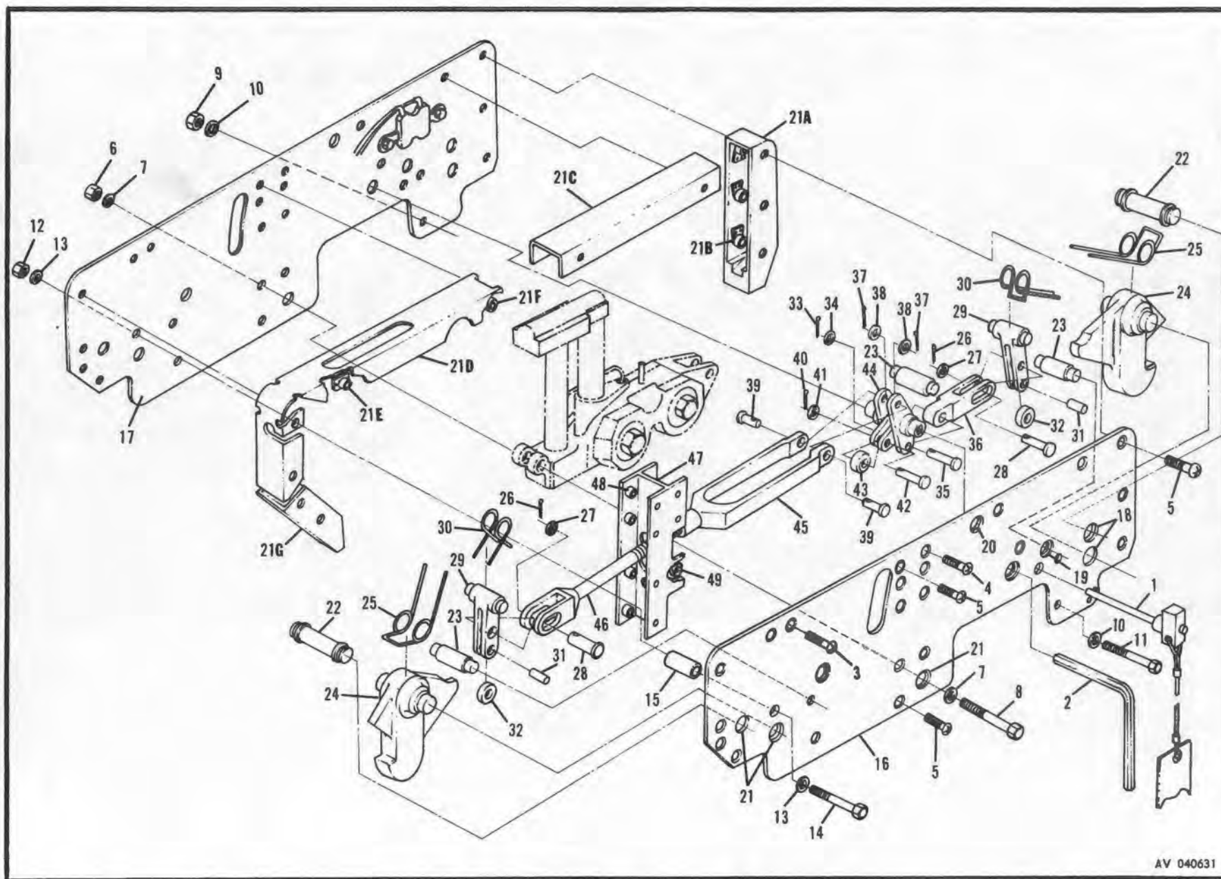
Figure 280. Rack, External Stores Ejector (Sheet 1 of 2)
