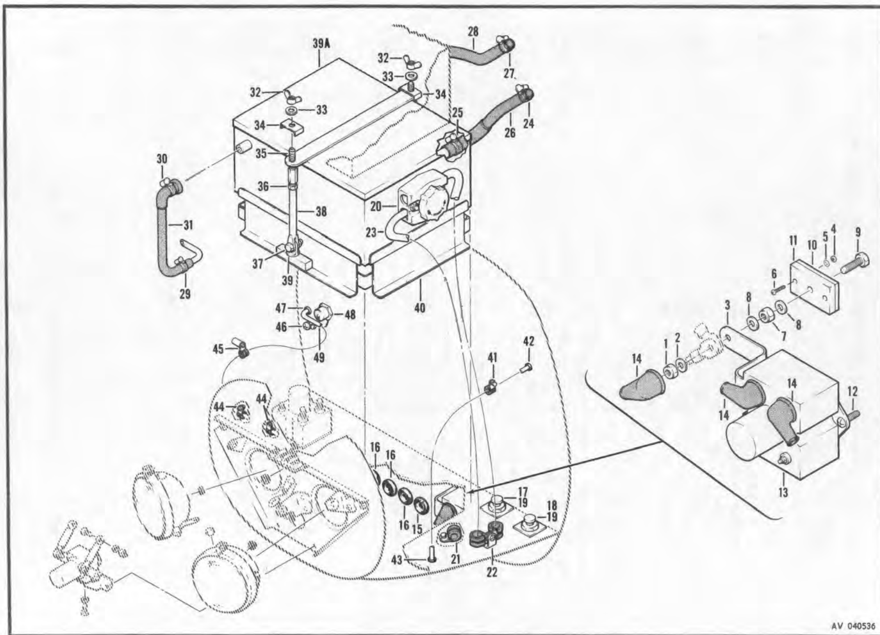
Figure 172. Electrical Installation, Nose Compartment
