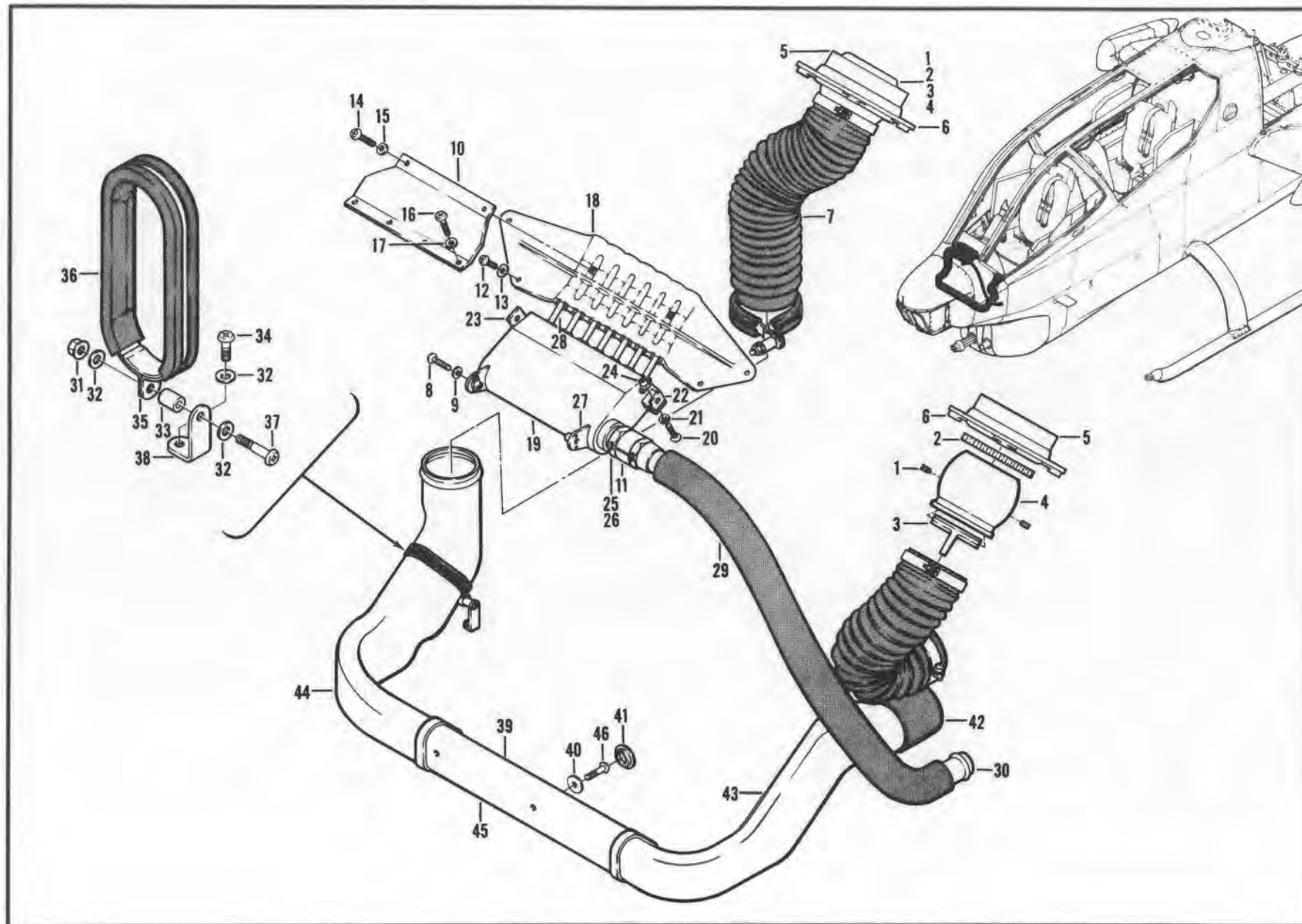
Figure 268A. Modification, Air Distribution System
