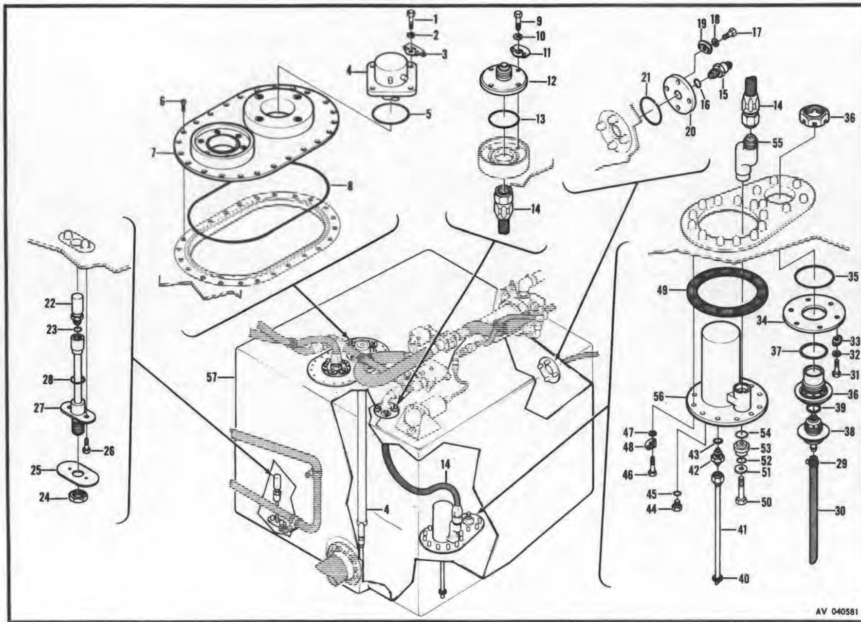
Figure 223. Fuel System Installation (Crashworthy)
