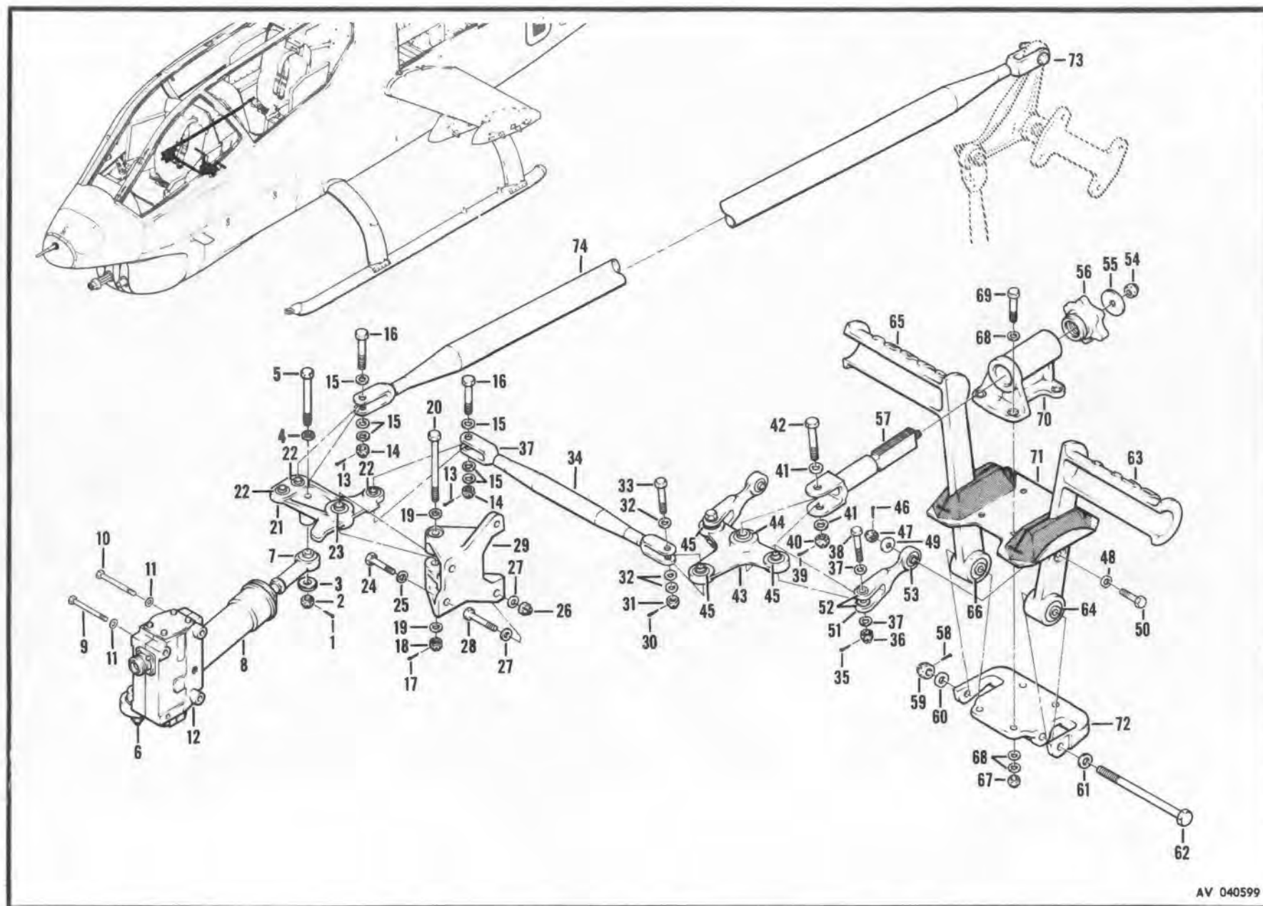
Figure 247. Controls Installation, Anti-Torque, Forward Section
