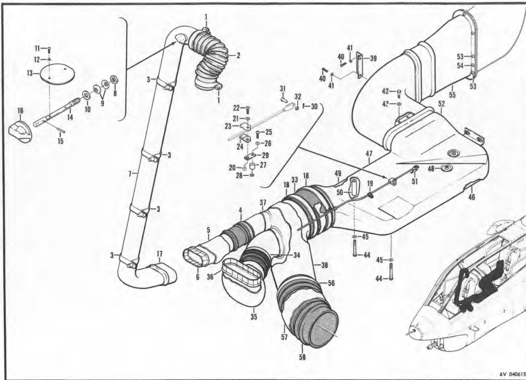
Figure 263. Air Distribution Installation, Heating and Ventilation
