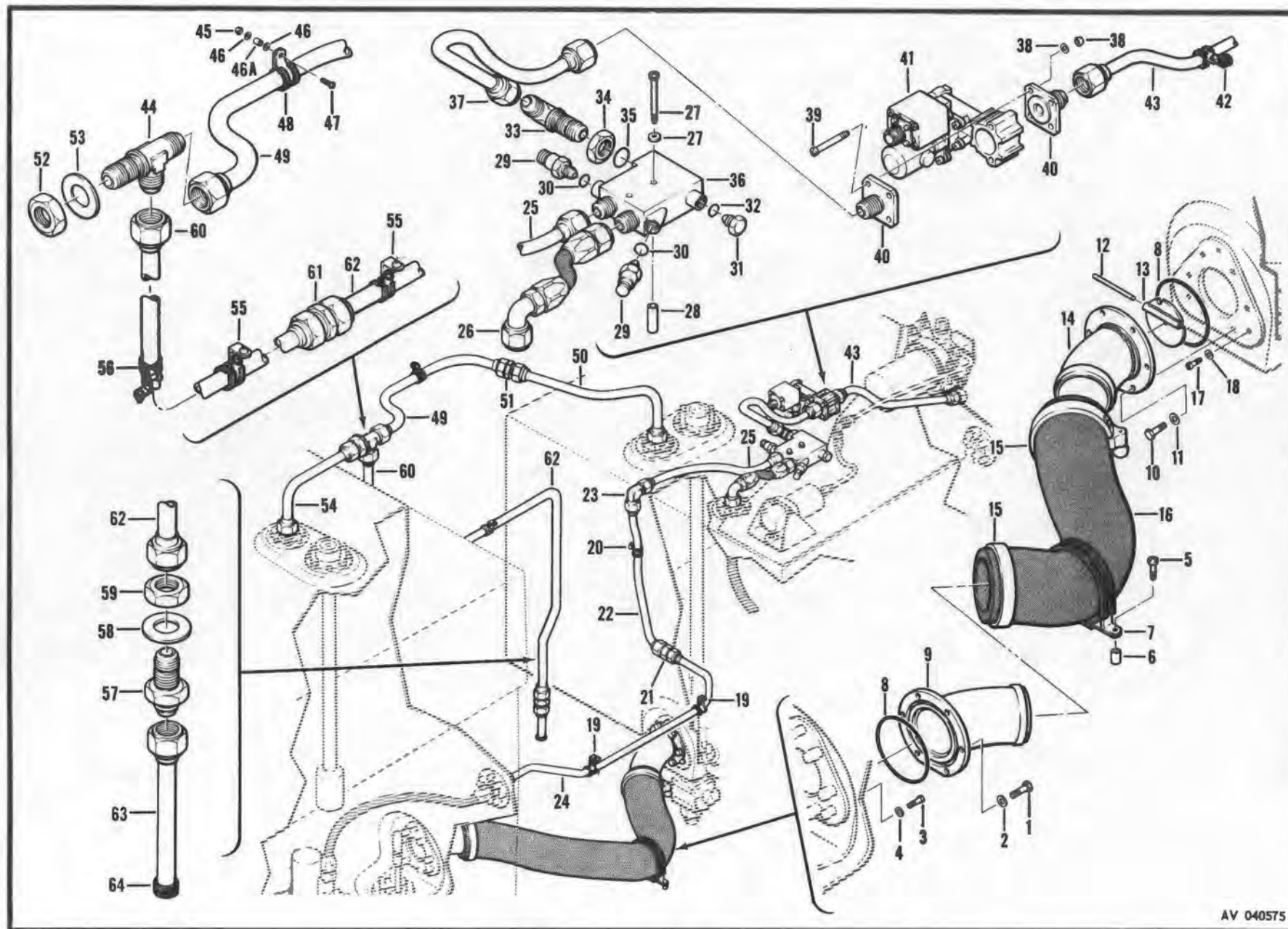
Figure 217. Fuel System Installation (Standard)
