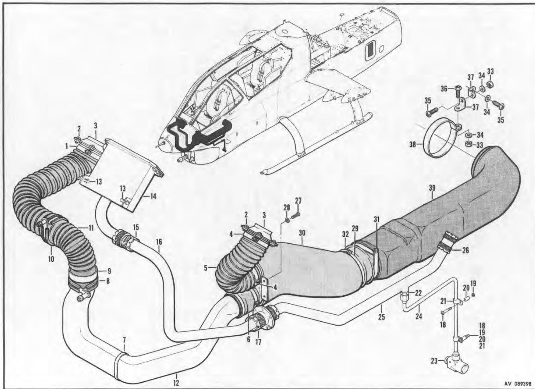
Figure 257. Air Distribution Installation, Heating and Ventilation
