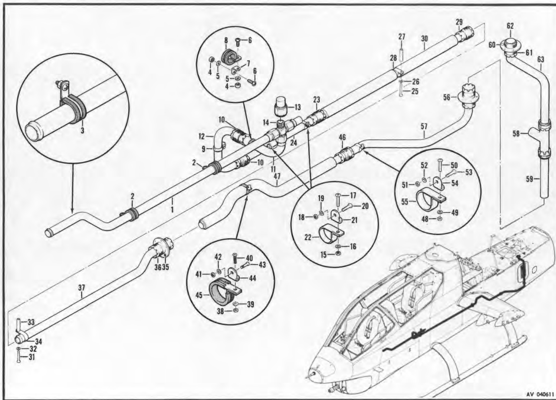
Figure 259. Air Distribution Installation, Heating and Ventilation
