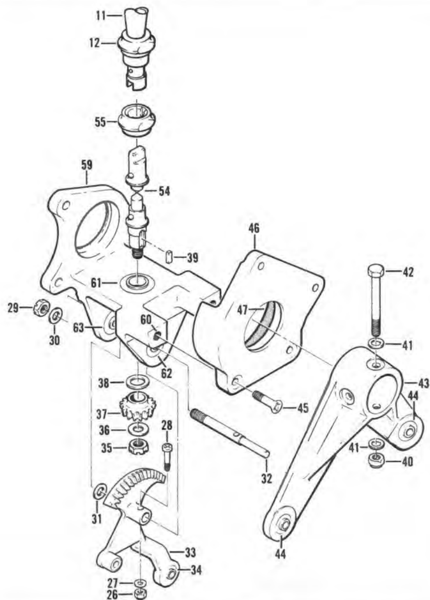
Figure 244. Controller, Grip Assembly (Sheet 2 of 2)
