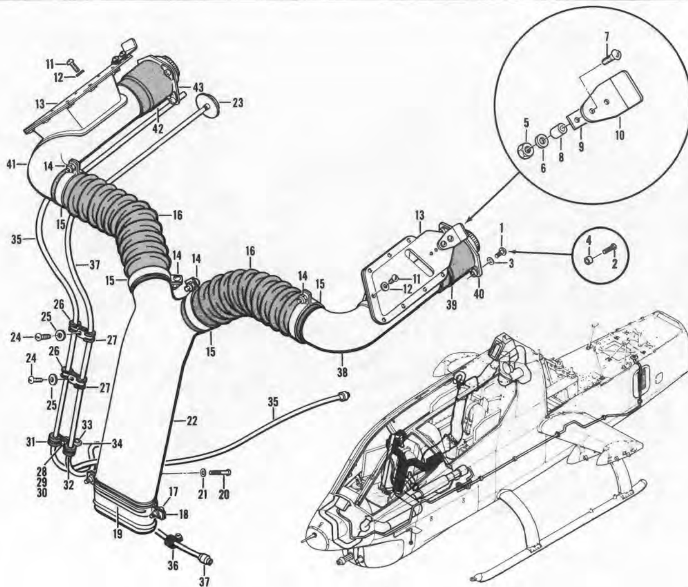
Figure 264. Air Distribution Installation, Heating and Ventilation
