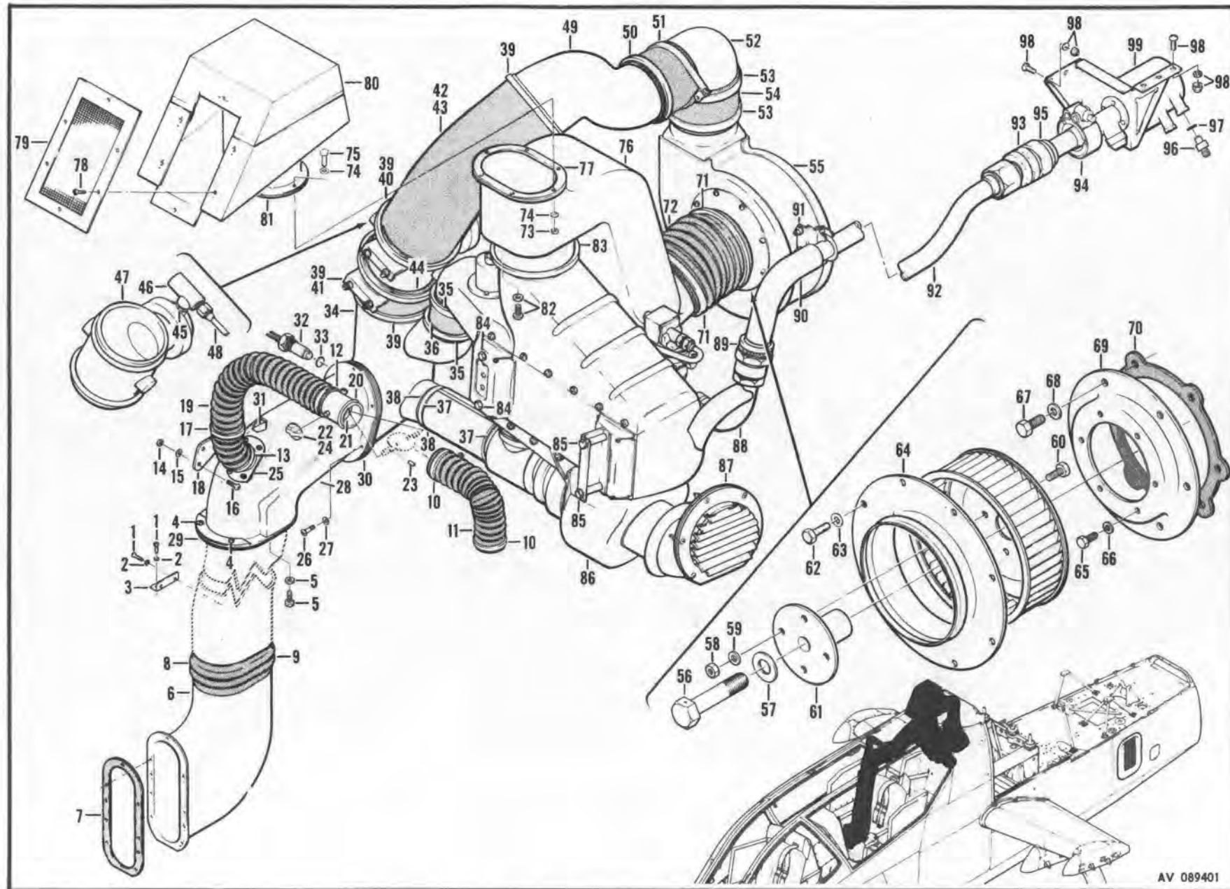
Figure 268. Air Distribution Installation, Heating and Ventilation
