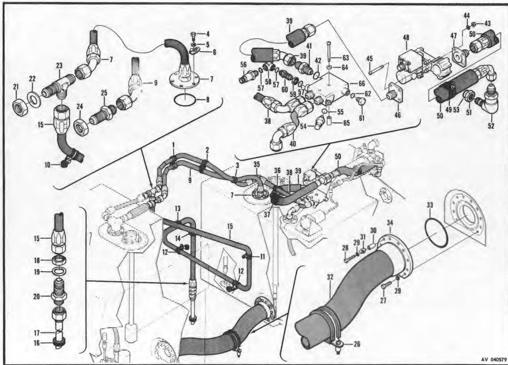
Figure 221. Fuel System Installation (Crashworthy)
