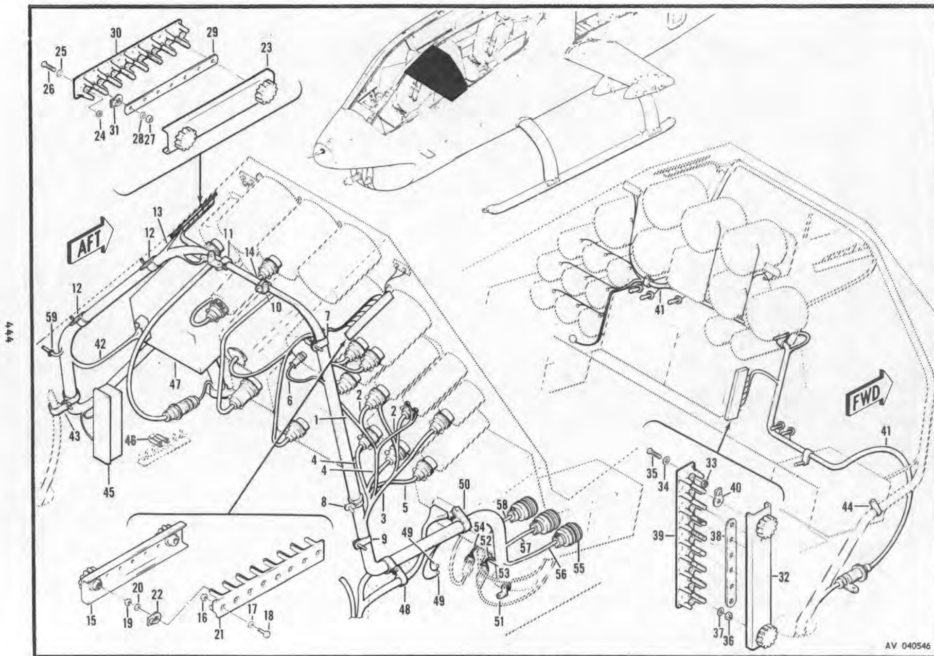
Figure 182. Electrical Installation, Pilot's Section
