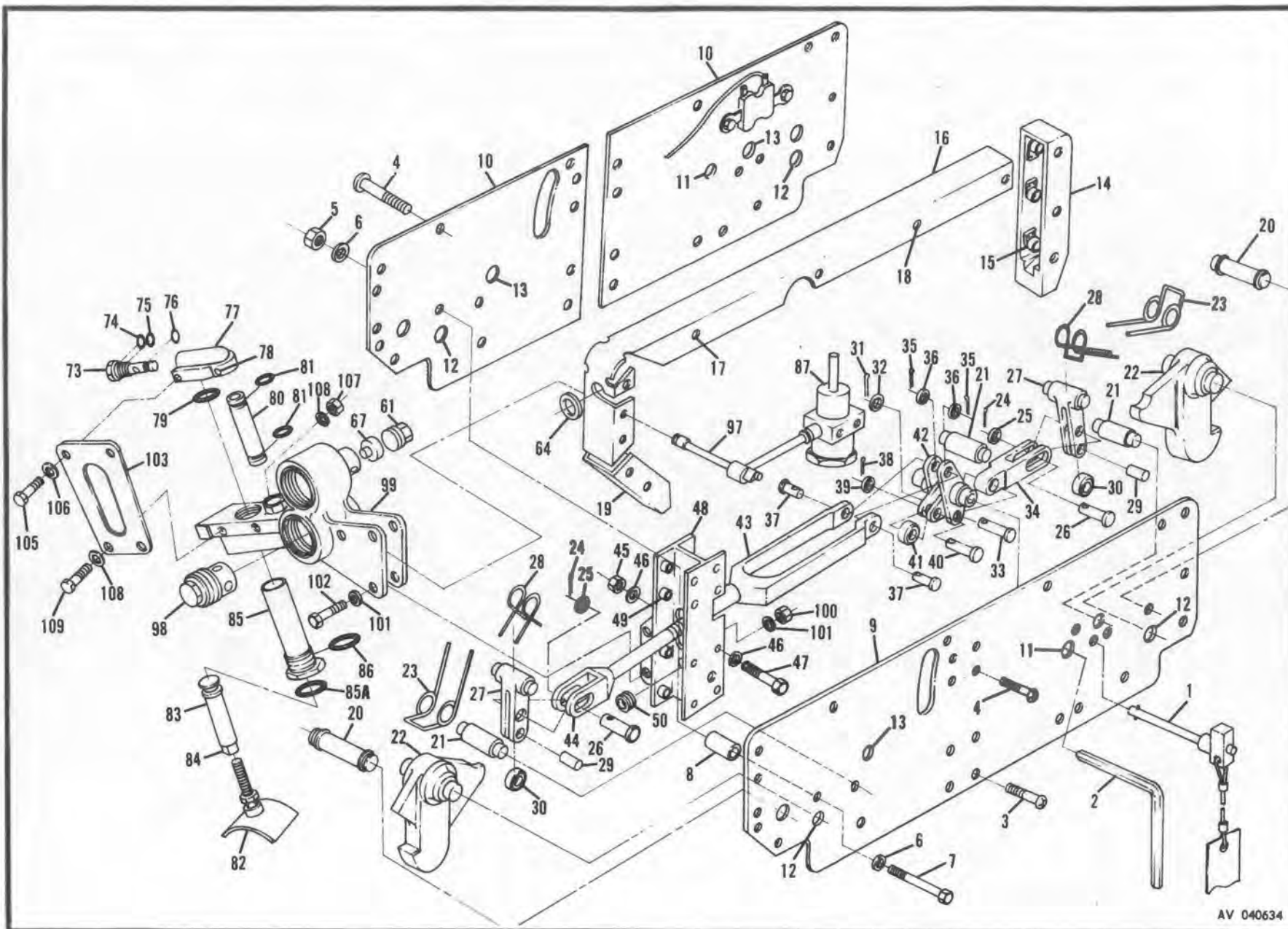
Figure 282. Rack, External Stores Ejector (Sheet 1 of 2)
