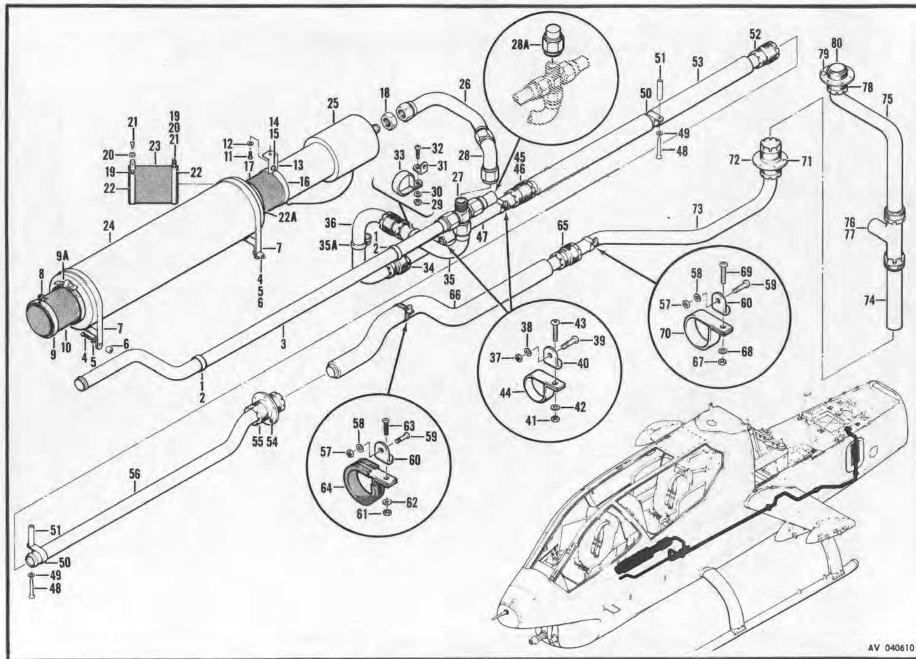
Figure 258. Air Distribution Installation, Heating and Ventilation
