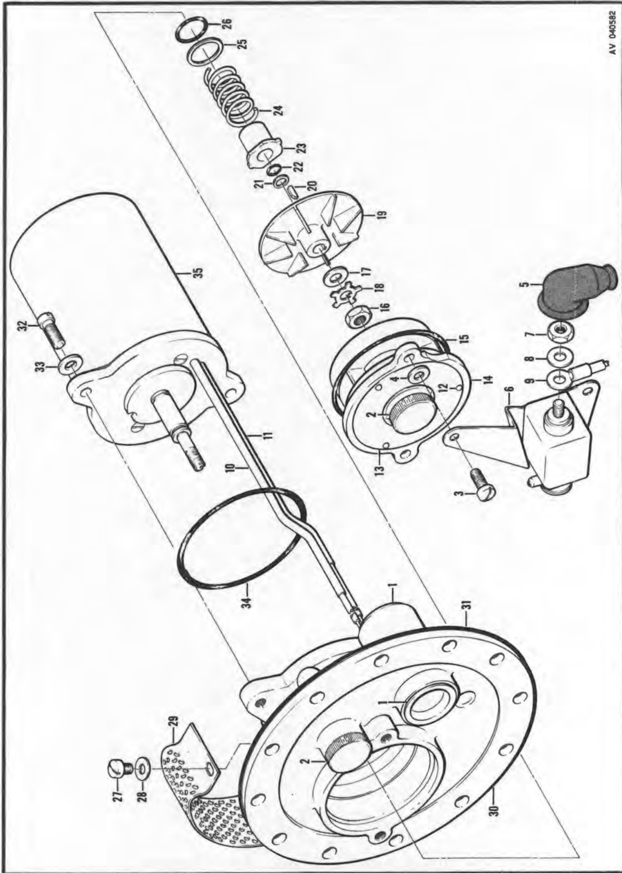
Figure 228. Pump Assembly, Fuel
