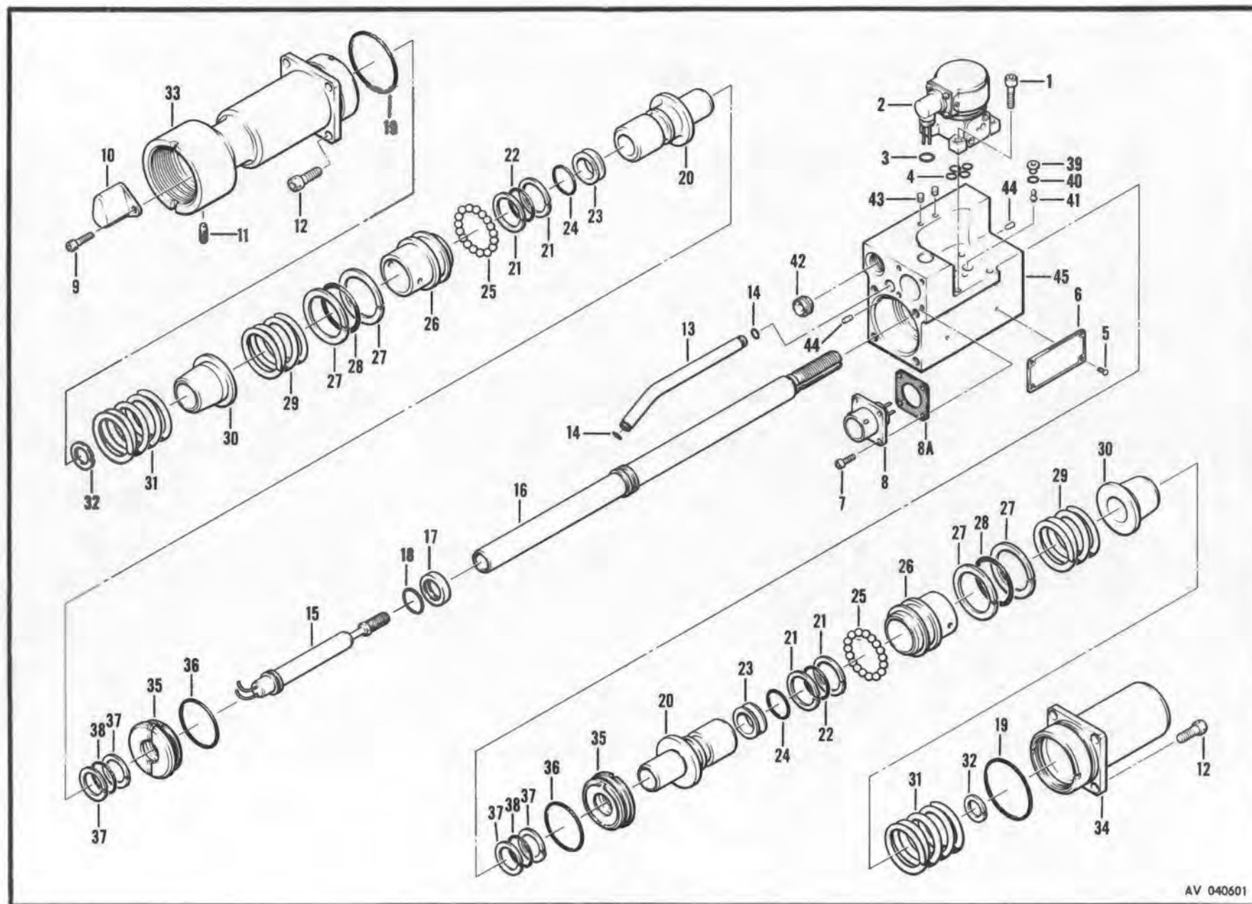
Figure 249. Servo Actuator
