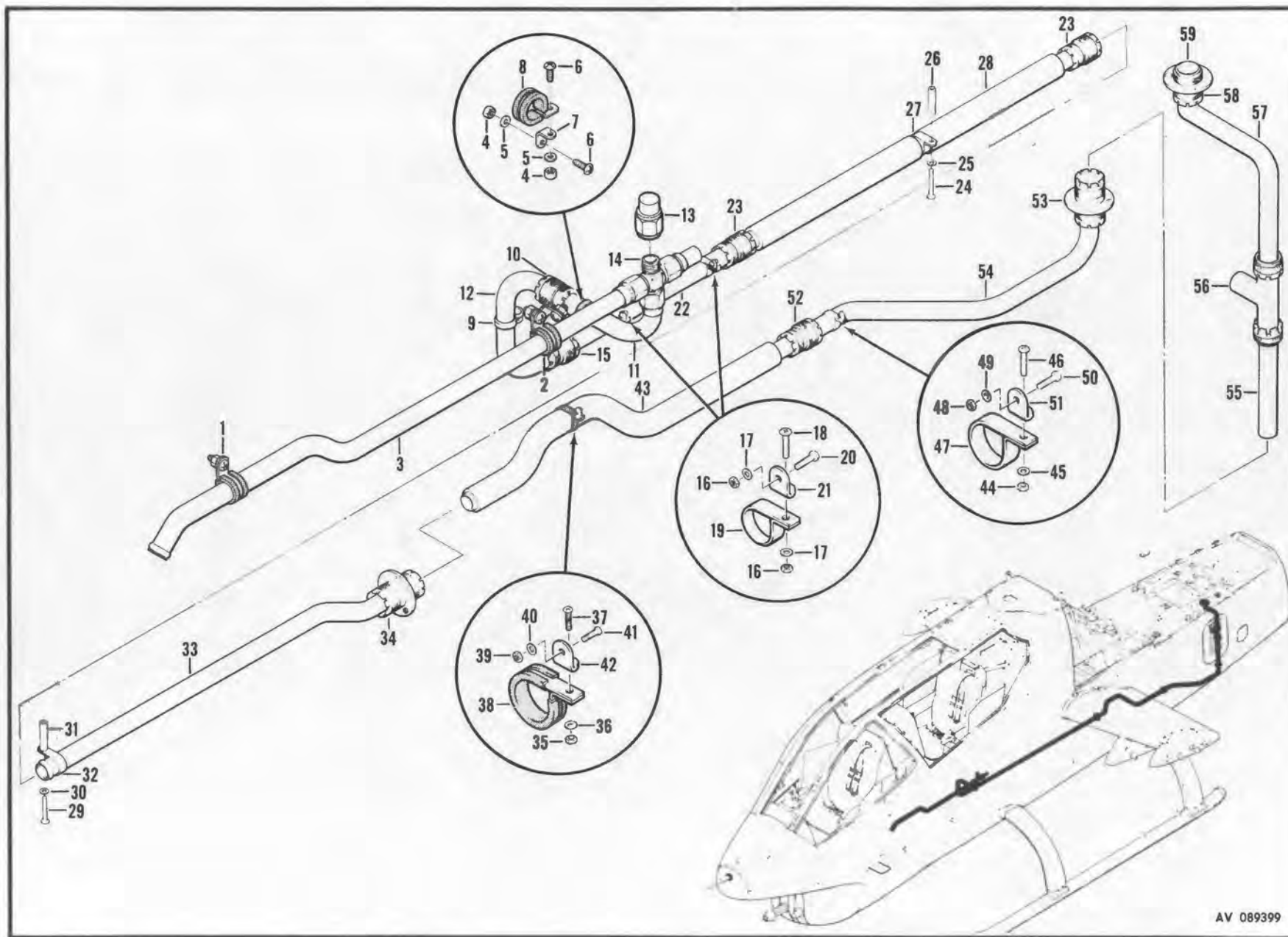
Figure 260. Air Distribution Installation, Heating and Ventilation
