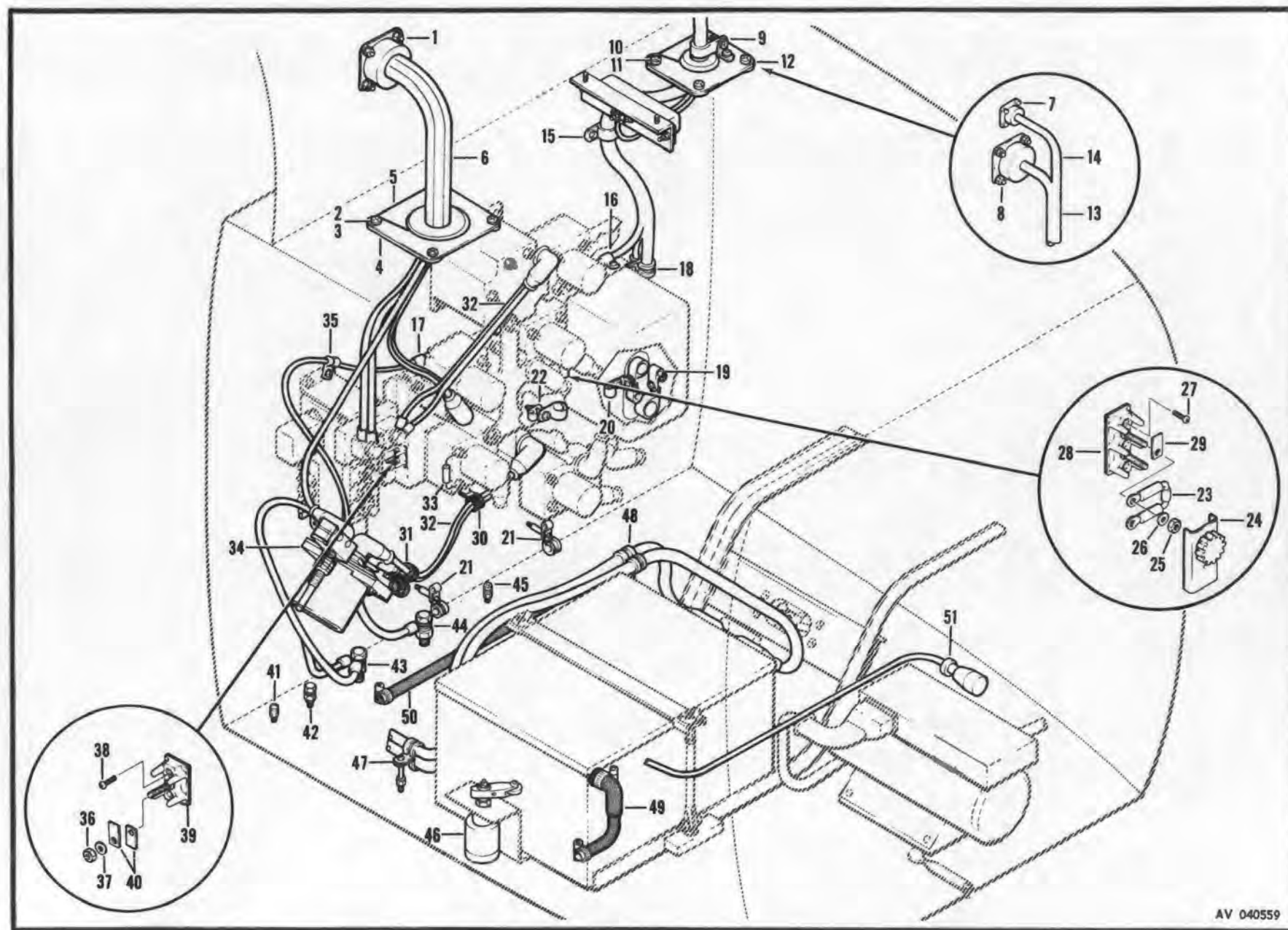
Figure 198. Equipment Installation, Aft Compartment, Forward Section
