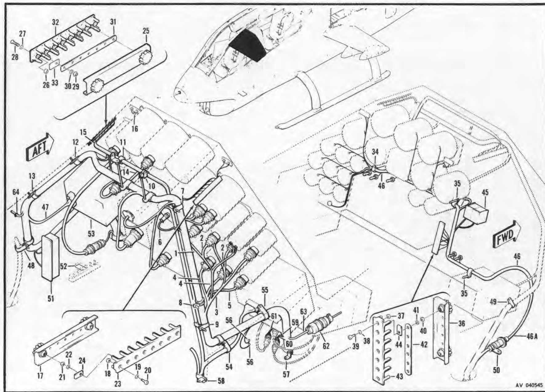
Figure 181. Electrical Installation, Pilot's Section
