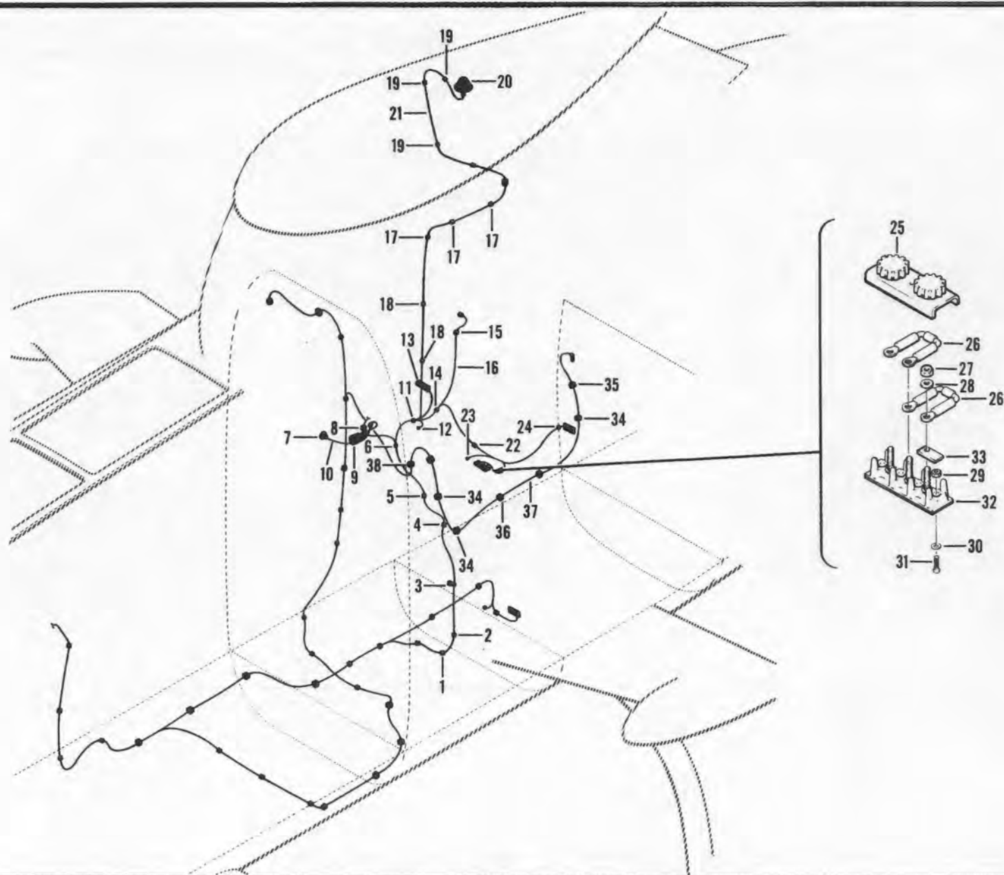
Figure 170. Electrical Installation, Forward Section
